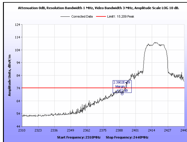
Plot 374. Radiated Restricted Band Edge, Peak, Channel 2, 802.11n 20 MHz, Ant. 1
