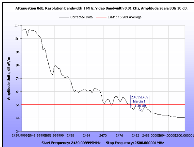
Plot 295. Radiated Restricted Band Edge, Average, Channel 7, 802.11b, Ant. 1
