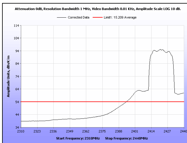
Plot 353. Radiated Restricted Band Edge, Average, Channel 3, 802.11n 20 MHz, Ant. 0
