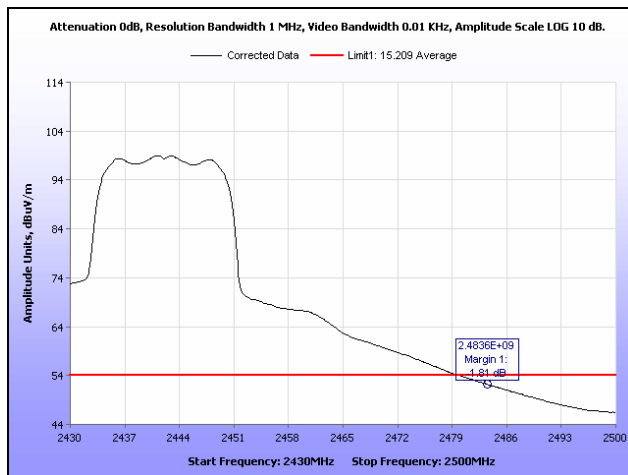
Plot 317. Radiated Restricted Band Edge, Average, Channel 7, 802.11g, Ant. 0
