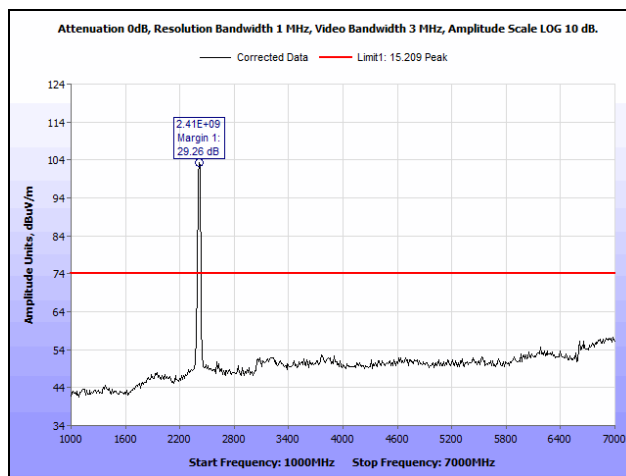
Plot 211. Radiated Spurious Emissions, Low Channel, 802.11n 20 MHz, Ant. 0, 1 GHz – 7 GHz, Peak
