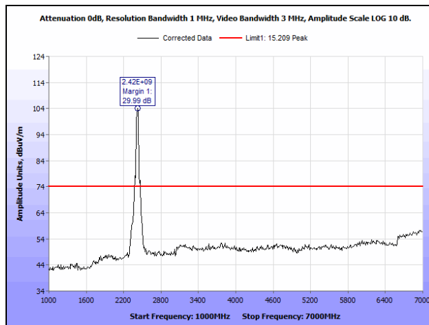
Plot 251. Radiated Spurious Emissions, Mid Channel, 802.11n 40 MHz, Ant. 1, 1 GHz – 7 GHz, Peak
