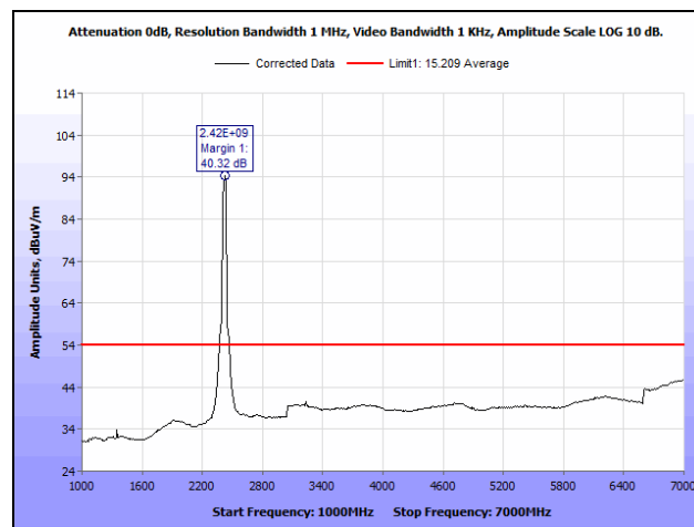
Plot 238. Radiated Spurious Emissions, Mid Channel, 802.11n 40 MHz, Ant. 0, 1 GHz – 7 GHz, Average
