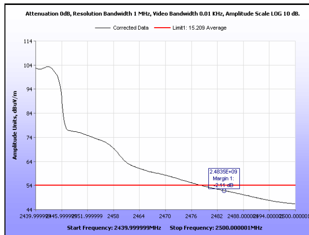
Plot 337. Radiated Restricted Band Edge, Average, Channel 6, 802.11g, Ant. 1
