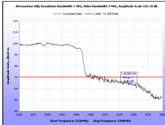
Plot 438. Radiated Restricted Band Edge, Peak, Channel 5, 802.11n 40 MHz, MIMO
