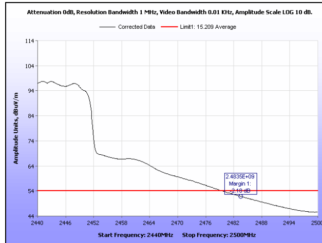
Plot 361. Radiated Restricted Band Edge, Average, Channel 7, 802.11n 20 MHz, Ant. 0
