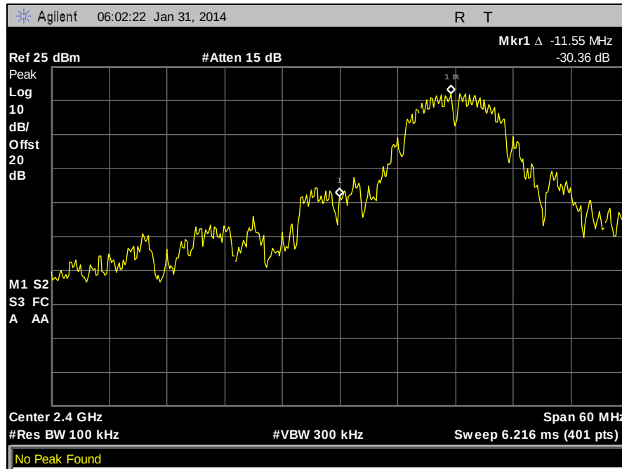
Plot 471. Conducted Band Edge, Low Channel, 802.11b, Ant. 0
