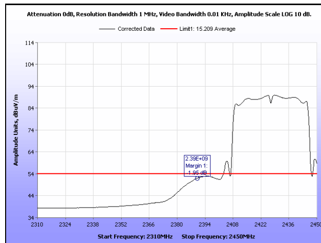
Plot 413. Radiated Restricted Band Edge, Average, Channel 2, 802.11n 40 MHz, Ant. 1
