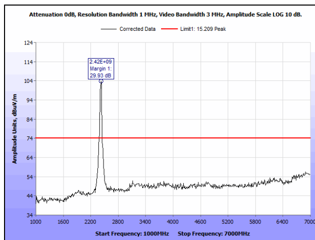
Plot 239. Radiated Spurious Emissions, Mid Channel, 802.11n 40 MHz, Ant. 0, 1 GHz – 7 GHz, Peak
