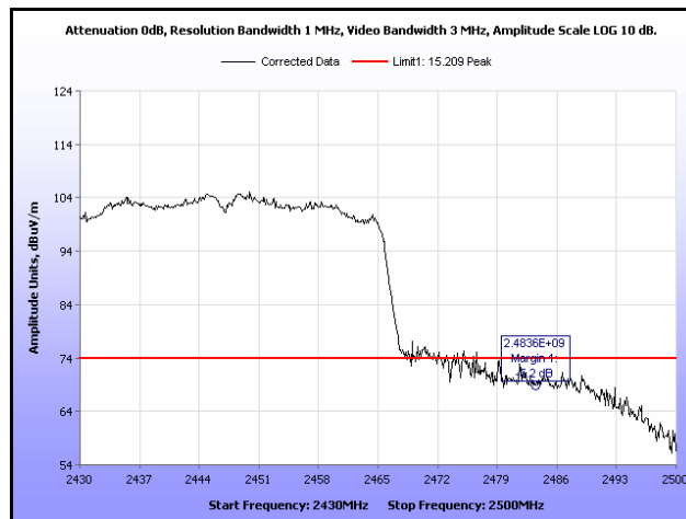
Plot 440. Radiated Restricted Band Edge, Peak, Channel 6, 802.11n 40 MHz, MIMO
