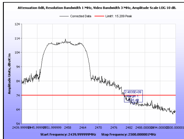
Plot 324. Radiated Restricted Band Edge, Peak, Channel 10, 802.11g, Ant. 0
