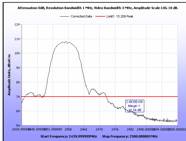
Plot 302. Radiated Restricted Band Edge, Peak, Channel 10, 802.11b, Ant. 1
