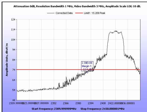
Plot 332. Radiated Restricted Band Edge, Peak, Channel 3, 802.11g, Ant. 1
