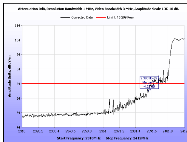
Plot 328. Radiated Restricted Band Edge, Peak, Channel 1, 802.11g, Ant. 1
