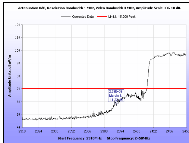
Plot 418. Radiated Restricted Band Edge, Peak, Channel 4, 802.11n 40 MHz, Ant. 1
