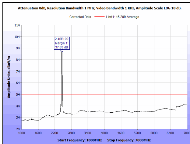
Plot 230. Radiated Spurious Emissions, High Channel, 802.11n 20 MHz, Ant. 1, 1 GHz – 7 GHz, Average
