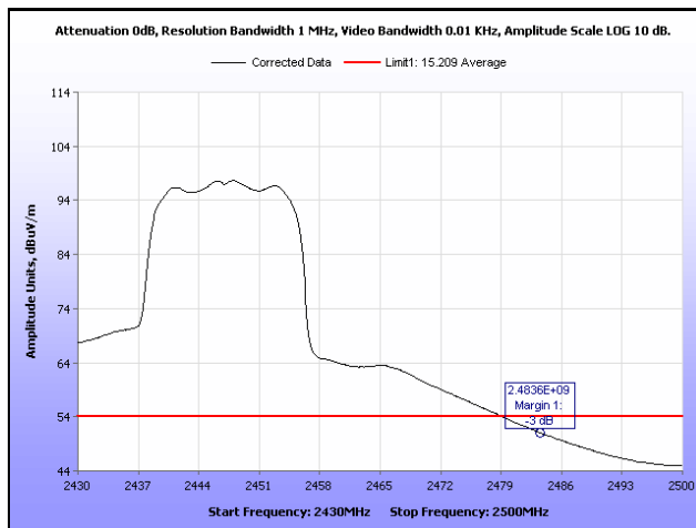
Plot 319. Radiated Restricted Band Edge, Average, Channel 8, 802.11g, Ant. 0
