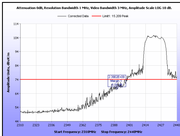
Plot 354. Radiated Restricted Band Edge, Peak, Channel 3, 802.11n 20 MHz, Ant. 0
