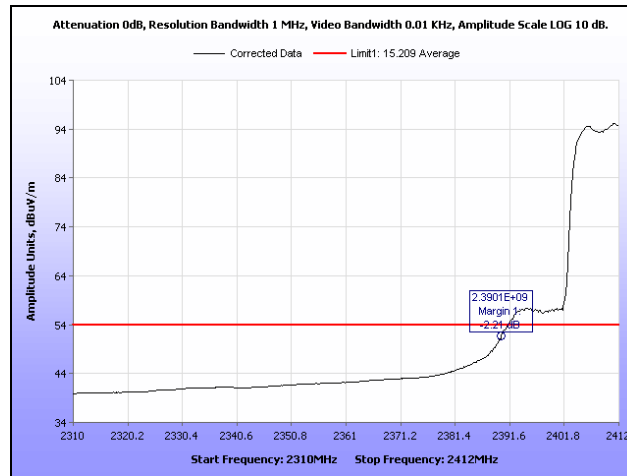
Plot 305. Radiated Restricted Band Edge, Average, Channel 1, 802.11g, Ant. 0
