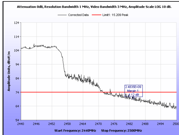
Plot 364. Radiated Restricted Band Edge, Peak, Channel 8, 802.11n 20 MHz, Ant. 0
