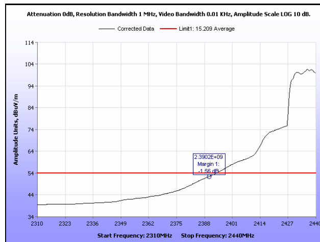
Plot 381. Radiated Restricted Band Edge, Average, Channel 6, 802.11n 20 MHz, Ant. 1
