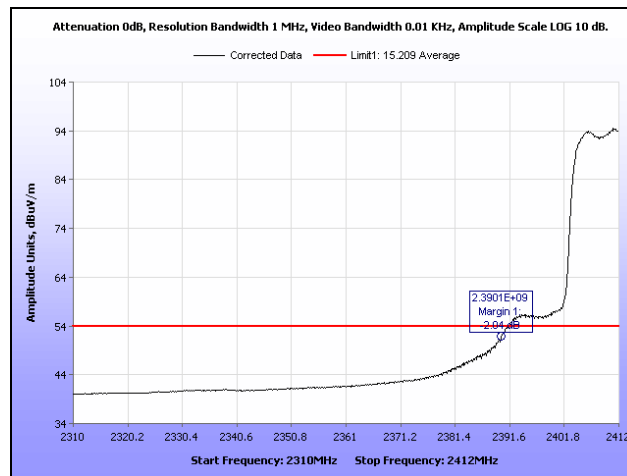
Plot 327. Radiated Restricted Band Edge, Average, Channel 1, 802.11g, Ant. 1
