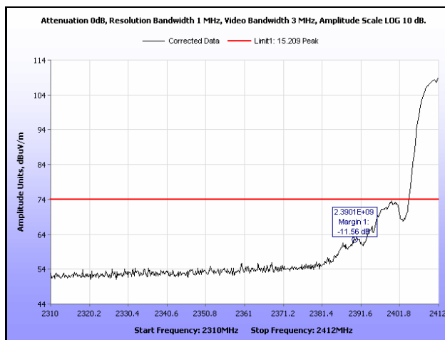
Plot 286. Radiated Restricted Band Edge, Peak, Channel 1, 802.11b, Ant. 1
