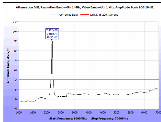
Plot 250. Radiated Spurious Emissions, Mid Channel, 802.11n 40 MHz, Ant. 1, 1 GHz – 7 GHz, Average
