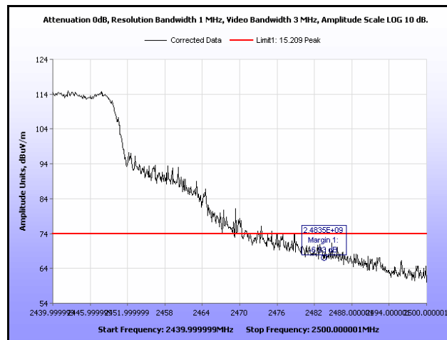
Plot 340. Radiated Restricted Band Edge, Peak, Channel 7, 802.11g, Ant. 1
