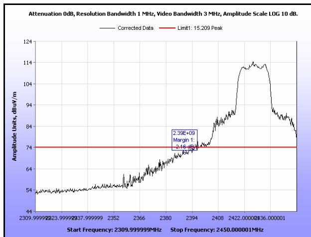
Plot 334. Radiated Restricted Band Edge, Peak, Channel 4, 802.11g, Ant. 1
