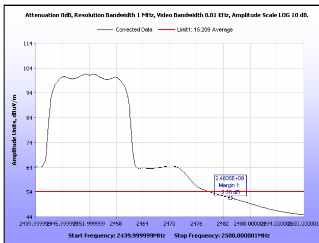
Plot 343. Radiated Restricted Band Edge, Average, Channel 9, 802.11g, Ant. 1
