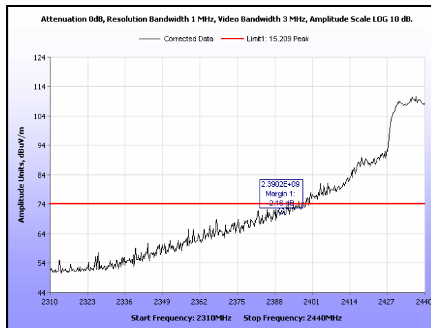
Plot 360. Radiated Restricted Band Edge, Peak, Channel 6, 802.11n 20 MHz, Ant. 0
