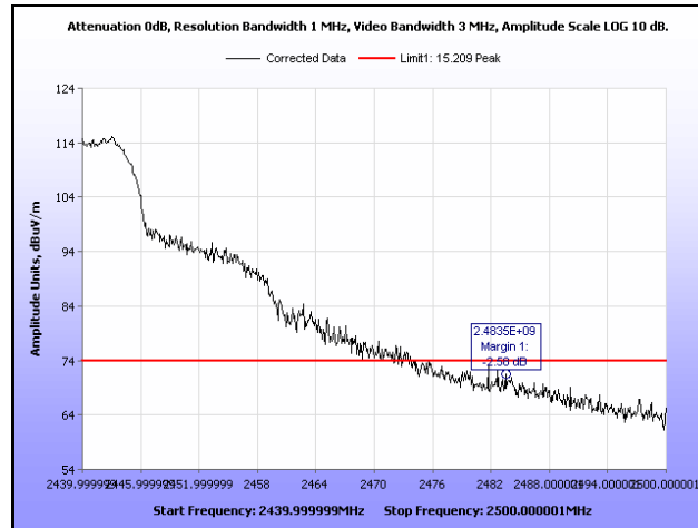
Plot 338. Radiated Restricted Band Edge, Peak, Channel 6, 802.11g, Ant. 1
