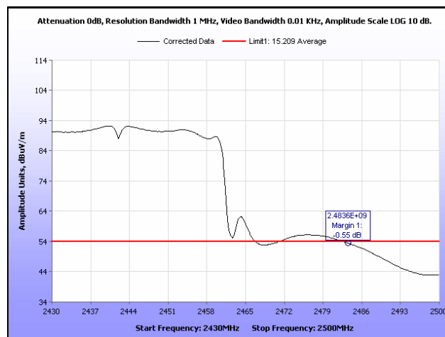
Plot 419. Radiated Restricted Band Edge, Average, Channel 5, 802.11n 40 MHz, Ant. 1
