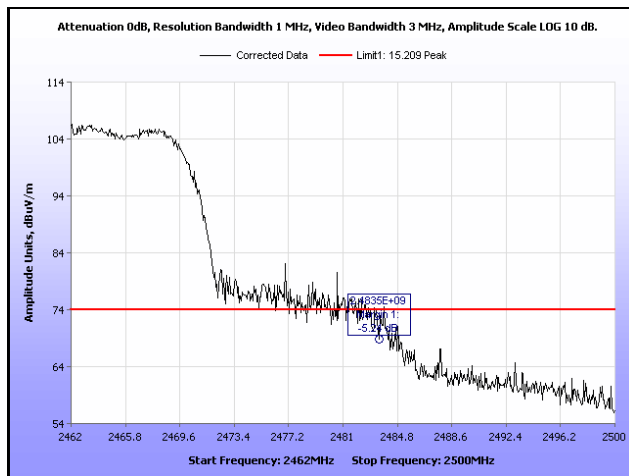
Plot 348. Radiated Restricted Band Edge, Peak, Channel 11, 802.11g, Ant. 1
