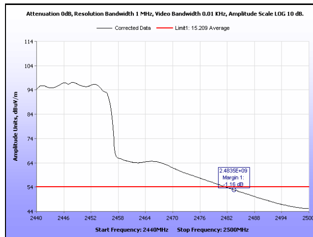
Plot 363. Radiated Restricted Band Edge, Average, Channel 8, 802.11n 20 MHz, Ant. 0
