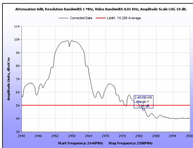
Plot 281. Radiated Restricted Band Edge, Average, Channel 10, 802.11b, Ant. 0
