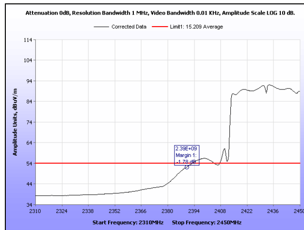
Plot 415. Radiated Restricted Band Edge, Average, Channel 3, 802.11n 40 MHz, Ant. 1
