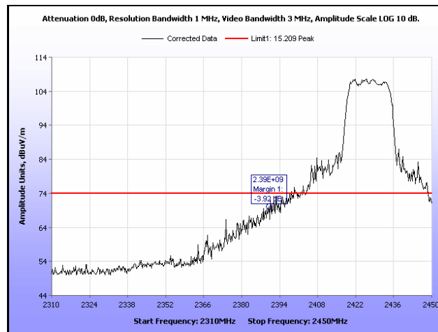
Plot 312. Radiated Restricted Band Edge, Peak, Channel 4, 802.11g, Ant. 0
