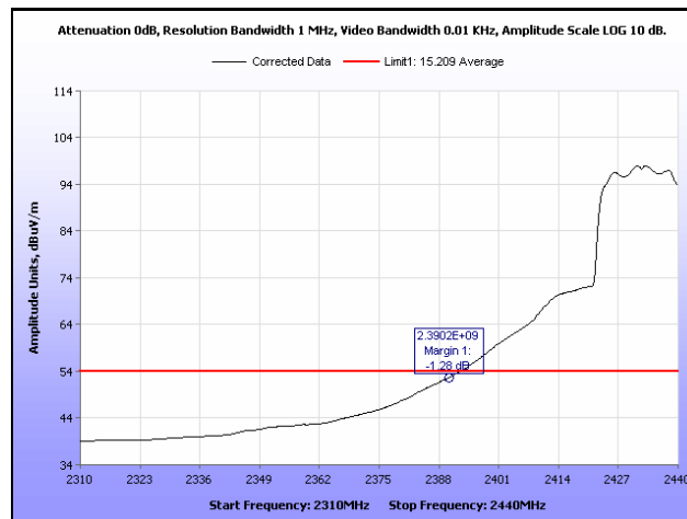
Plot 357. Radiated Restricted Band Edge, Average, Channel 5, 802.11n 20 MHz, Ant. 0
