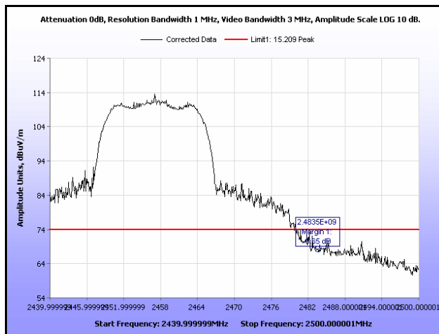
Plot 346. Radiated Restricted Band Edge, Peak, Channel 10, 802.11g, Ant. 1
