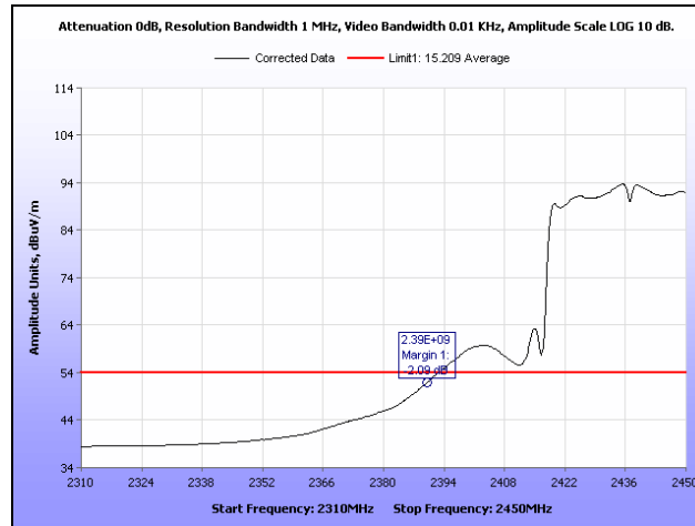
Plot 417. Radiated Restricted Band Edge, Average, Channel 4, 802.11n 40 MHz, Ant. 1
