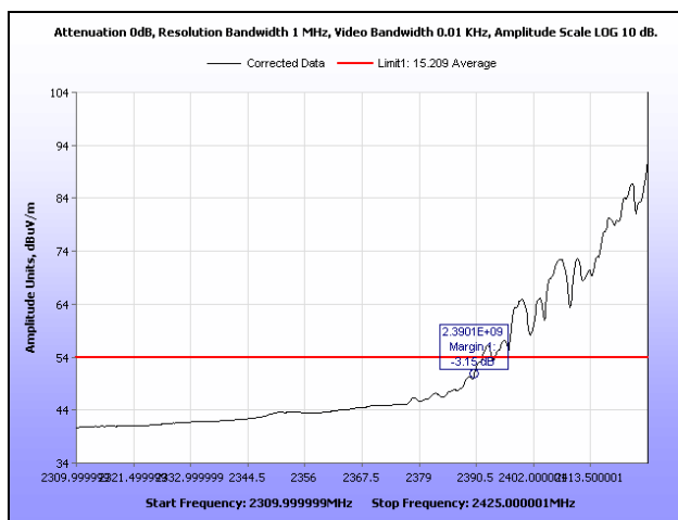
Plot 293. Radiated Restricted Band Edge, Average, Channel 5, 802.11b, Ant. 1
