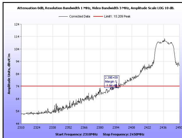
Plot 316. Radiated Restricted Band Edge, Peak, Channel 6, 802.11g, Ant. 0
