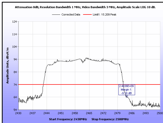
Plot 410. Radiated Restricted Band Edge, Peak, Channel 9, 802.11n 40 MHz, Ant. 0
