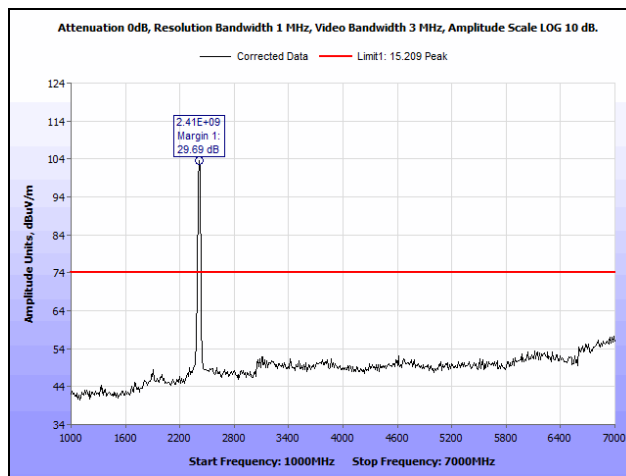
Plot 223. Radiated Spurious Emissions, Low Channel, 802.11n 20 MHz, Ant. 1, 1 GHz – 7 GHz, Peak
