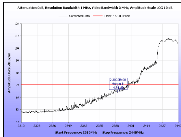
Plot 380. Radiated Restricted Band Edge, Peak, Channel 5, 802.11n 20 MHz, Ant. 1
