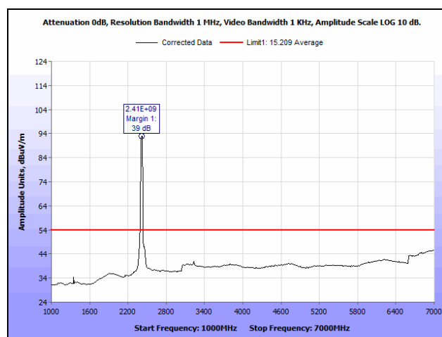
Plot 258. Radiated Spurious Emissions, Low Channel, 802.11n 40 MHz, MIMO, 1 GHz – 7 GHz, Average
