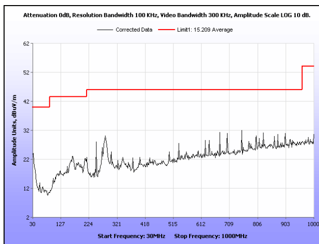
Plot 225. Radiated Spurious Emissions, Mid Channel, 802.11n 20 MHz, Ant. 1, 30 MHz – 1 GHz
