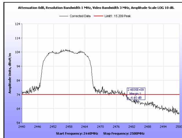
Plot 368. Radiated Restricted Band Edge, Peak, Channel 10, 802.11n 20 MHz, Ant. 0
