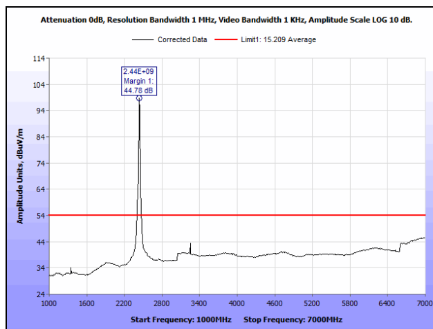
Plot 226. Radiated Spurious Emissions, Mid Channel, 802.11n 20 MHz, Ant. 1, 1 GHz – 7 GHz, Average
