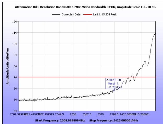
Plot 292. Radiated Restricted Band Edge, Peak, Channel 4, 802.11b, Ant. 1
