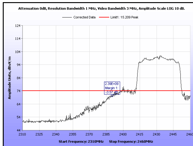
Plot 398. Radiated Restricted Band Edge, Peak, Channel 3, 802.11n 40 MHz, Ant. 0
