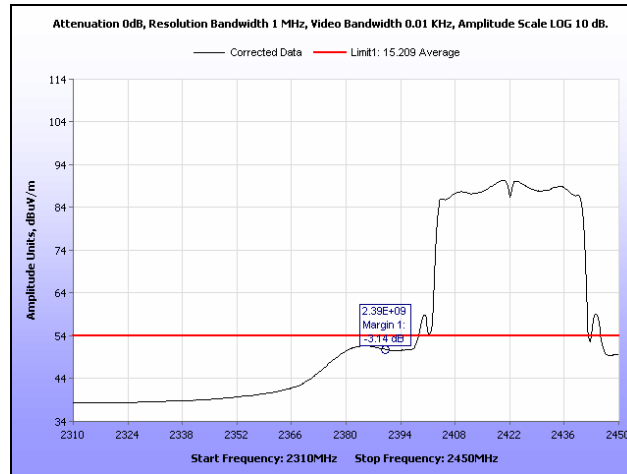
Plot 411. Radiated Restricted Band Edge, Average, Channel 1, 802.11n 40 MHz, Ant. 1
