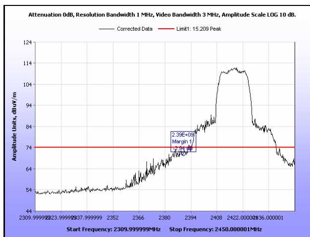
Plot 330. Radiated Restricted Band Edge, Peak, Channel 2, 802.11g, Ant. 1
