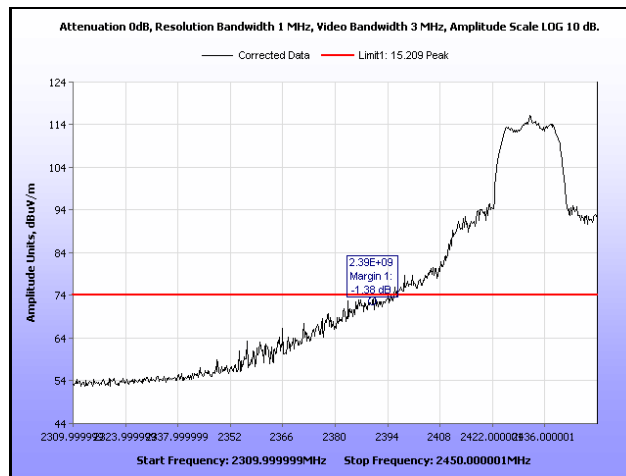
Plot 336. Radiated Restricted Band Edge, Peak, Channel 5, 802.11g, Ant. 1
