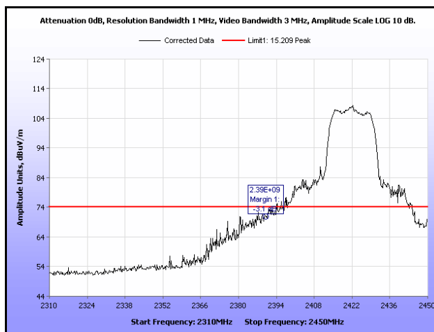
Plot 310. Radiated Restricted Band Edge, Peak, Channel 3, 802.11g, Ant. 0
