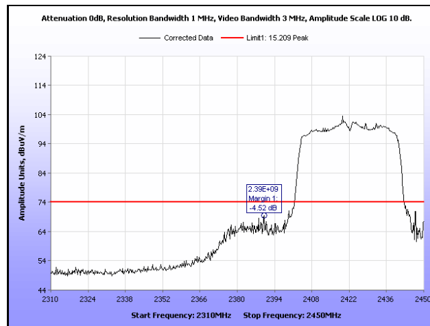
Plot 412. Radiated Restricted Band Edge, Peak, Channel 1, 802.11n 40 MHz, Ant. 1
