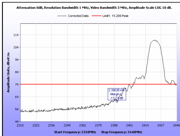
Plot 274. Radiated Restricted Band Edge, Peak, Channel 3, 802.11b, Ant. 0
