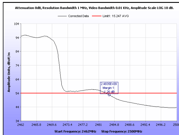
Plot 325. Radiated Restricted Band Edge, Average, Channel 11, 802.11g, Ant. 0
