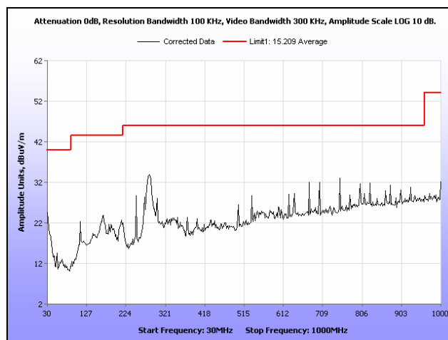
Plot 257. Radiated Spurious Emissions, Low Channel, 802.11n 40 MHz, MIMO, 30 MHz – 1 GHz
