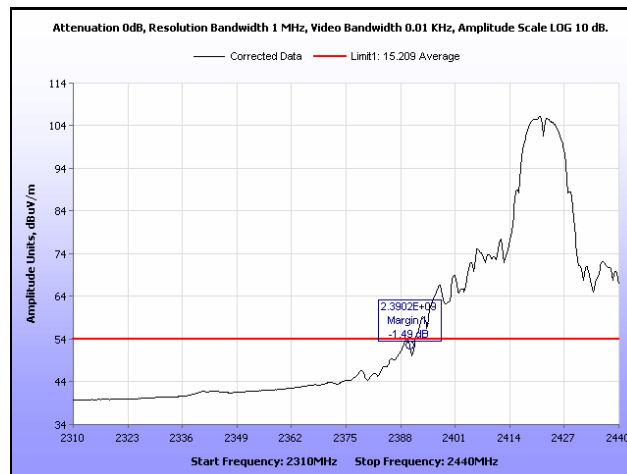
Plot 273. Radiated Restricted Band Edge, Average, Channel 3, 802.11b, Ant. 0
