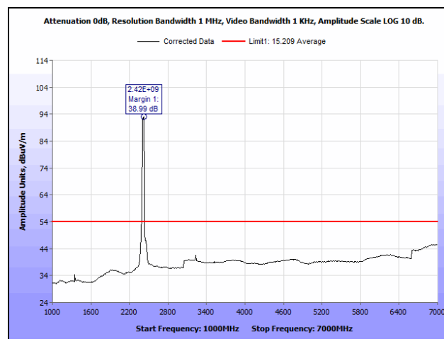
Plot 234. Radiated Spurious Emissions, Low Channel, 802.11n 40 MHz, Ant. 0, 1 GHz – 7 GHz, Average
