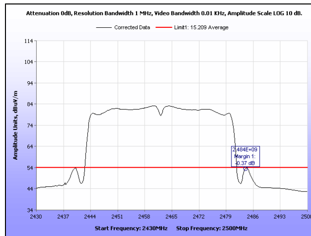
Plot 445. Radiated Restricted Band Edge, Average, Channel 9, 802.11n 40 MHz, MIMO
