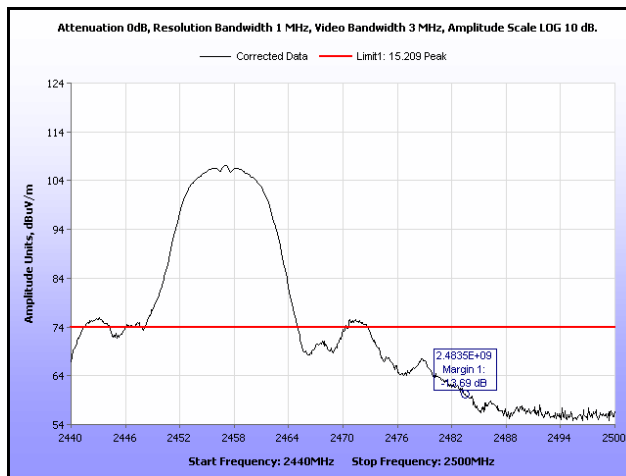
Plot 282. Radiated Restricted Band Edge, Peak, Channel 10, 802.11b, Ant. 0
