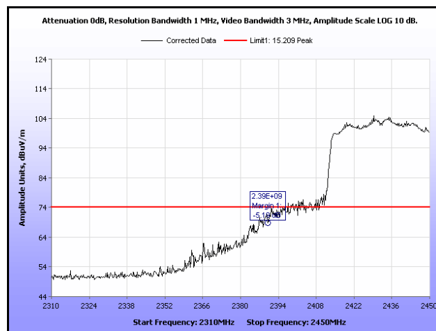
Plot 416. Radiated Restricted Band Edge, Peak, Channel 3, 802.11n 40 MHz, Ant. 1
