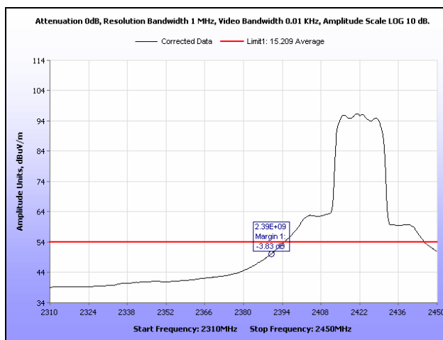
Plot 309. Radiated Restricted Band Edge, Average, Channel 3, 802.11g, Ant. 0
