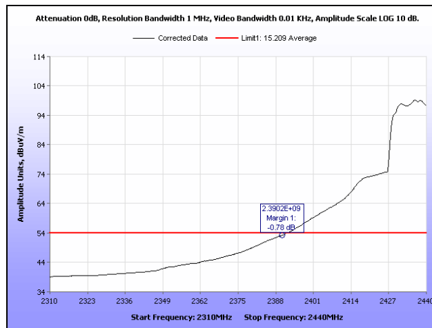
Plot 359. Radiated Restricted Band Edge, Average, Channel 6, 802.11n 20 MHz, Ant. 0
