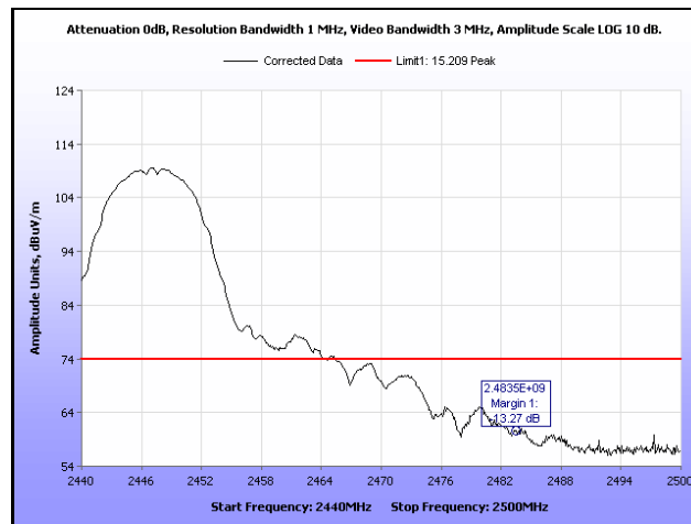
Plot 278. Radiated Restricted Band Edge, Peak, Channel 8, 802.11b, Ant. 0
