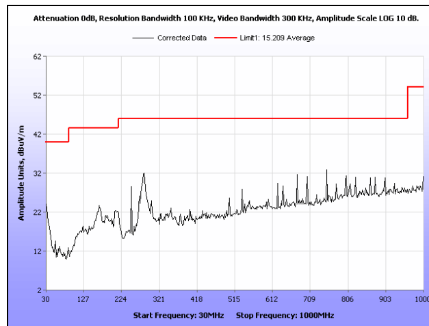
Plot 237. Radiated Spurious Emissions, Mid Channel, 802.11n 40 MHz, Ant. 0, 30 MHz – 1 GHz
