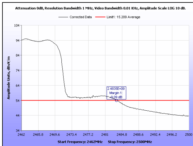
Plot 347. Radiated Restricted Band Edge, Average, Channel 11, 802.11g, Ant. 1
