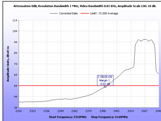
Plot 355. Radiated Restricted Band Edge, Average, Channel 4, 802.11n 20 MHz, Ant. 0
