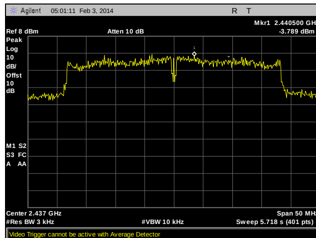
Plot 506. Peak Power Spectral Density, Mid Channel, 802.11n 40 MHz, Ant. 0
