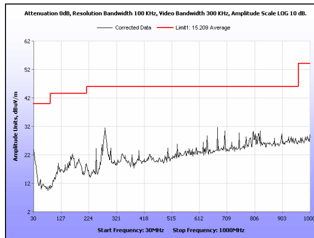
Plot 249. Radiated Spurious Emissions, Mid Channel, 802.11n 40 MHz, Ant. 1, 30 MHz – 1 GHz
