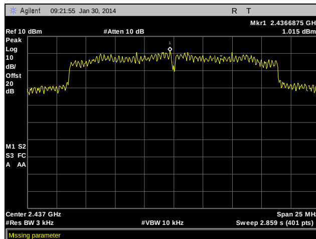
Plot 500. Peak Power Spectral Density, Mid Channel, 802.11n 20 MHz, Ant. 0
