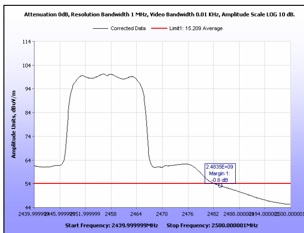
Plot 345. Radiated Restricted Band Edge, Average, Channel 10, 802.11g, Ant. 1
