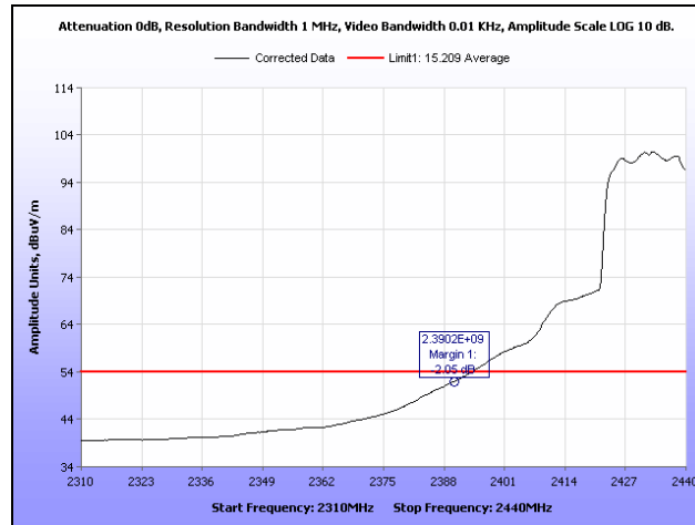
Plot 379. Radiated Restricted Band Edge, Average, Channel 5, 802.11n 20 MHz, Ant. 1
