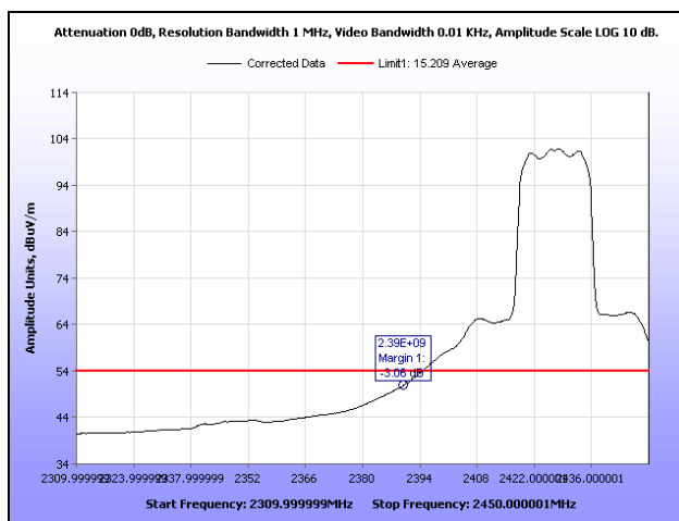
Plot 333. Radiated Restricted Band Edge, Average, Channel 4, 802.11g, Ant. 1
