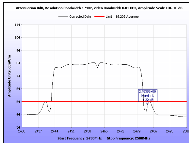
Plot 427. Radiated Restricted Band Edge, Average, Channel 9, 802.11n 40 MHz, Ant. 1
