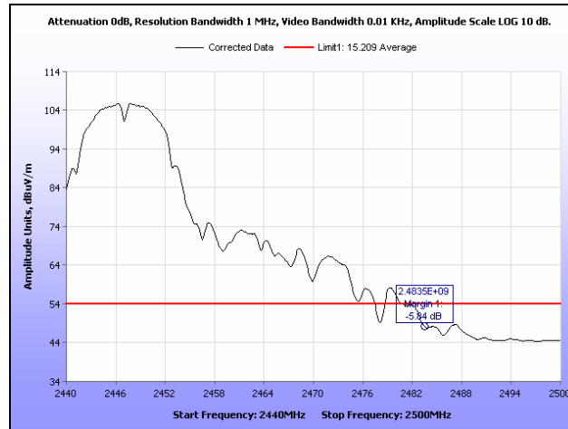
Plot 277. Radiated Restricted Band Edge, Average, Channel 8, 802.11b, Ant. 0
