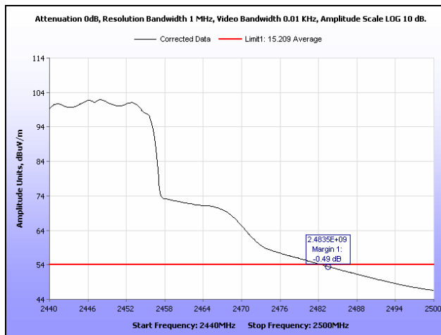
Plot 385. Radiated Restricted Band Edge, Average, Channel 8, 802.11n 20 MHz, Ant. 1
