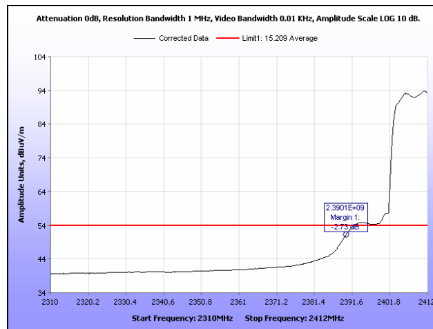
Plot 371. Radiated Restricted Band Edge, Average, Channel 1, 802.11n 20 MHz, Ant. 1
