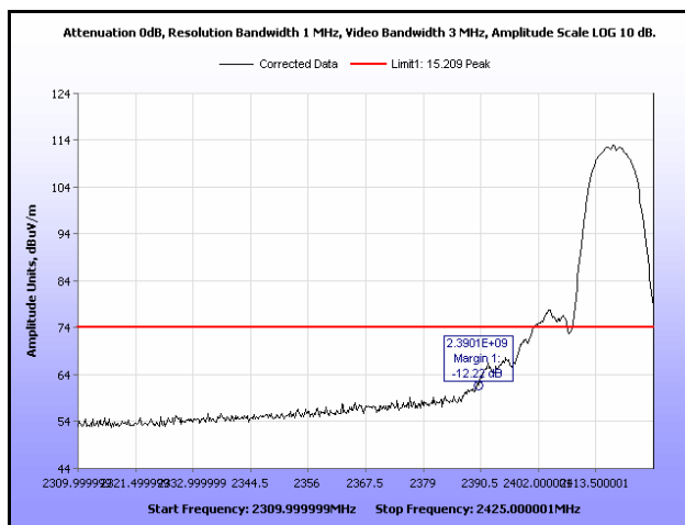
Plot 288. Radiated Restricted Band Edge, Peak, Channel 2, 802.11b, Ant. 1
