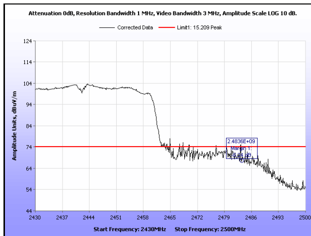
Plot 420. Radiated Restricted Band Edge, Peak, Channel 5, 802.11n 40 MHz, Ant. 1
