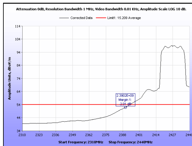
Plot 375. Radiated Restricted Band Edge, Average, Channel 3, 802.11n 20 MHz, Ant. 1
