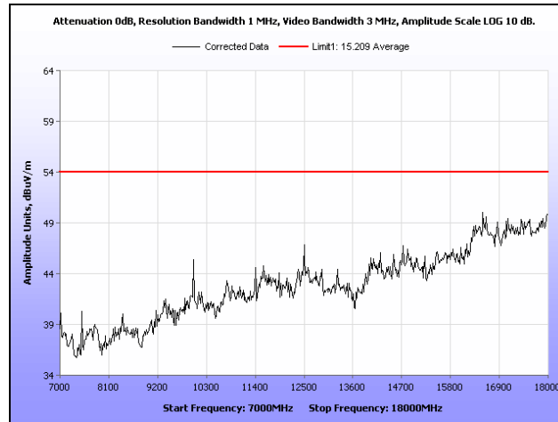
Plot 236. Radiated Spurious Emissions, Low Channel, 802.11n 40 MHz, Ant. 0, 7 GHz – 18 GHz
