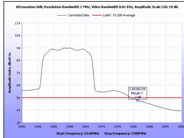
Plot 367. Radiated Restricted Band Edge, Average, Channel 10, 802.11n 20 MHz, Ant. 0
