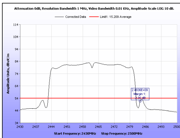
Plot 409. Radiated Restricted Band Edge, Average, Channel 9, 802.11n 40 MHz, Ant. 0
