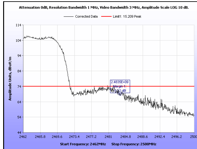
Plot 326. Radiated Restricted Band Edge, Peak, Channel 11, 802.11g, Ant. 0
