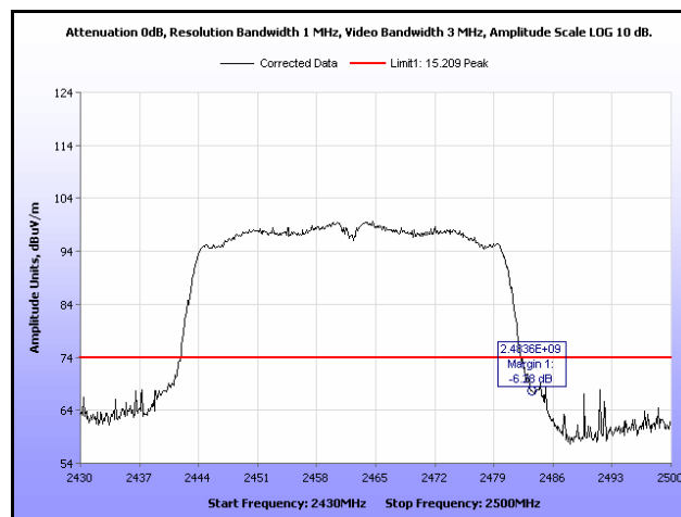
Plot 428. Radiated Restricted Band Edge, Peak, Channel 9, 802.11n 40 MHz, Ant. 1
