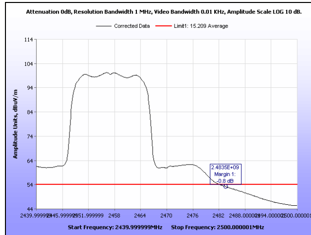
Plot 323. Radiated Restricted Band Edge, Average, Channel 10, 802.11g, Ant. 0
