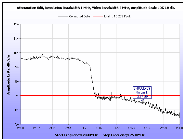
Plot 402. Radiated Restricted Band Edge, Peak, Channel 5, 802.11n 40 MHz, Ant. 0
