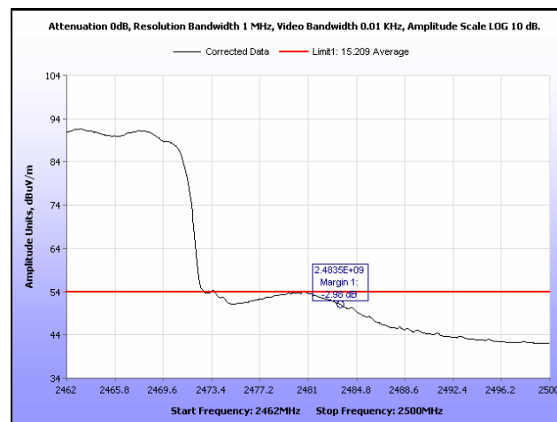
Plot 369. Radiated Restricted Band Edge, Average, Channel 11, 802.11n 20 MHz, Ant. 0
