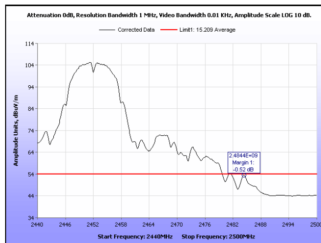
Plot 279. Radiated Restricted Band Edge, Average, Channel 9, 802.11b, Ant. 0
