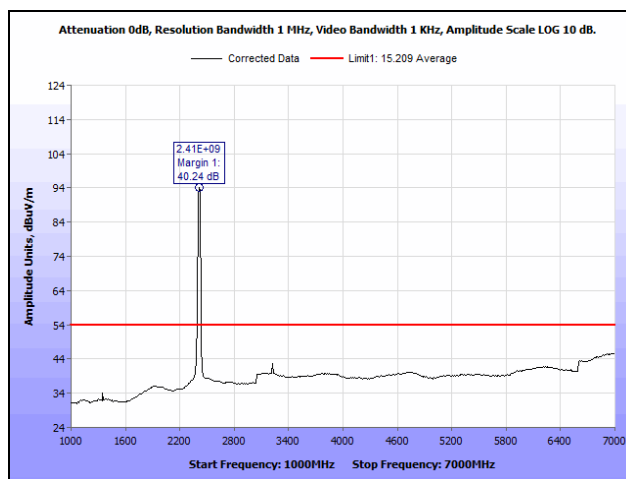
Plot 210. Radiated Spurious Emissions, Low Channel, 802.11n 20 MHz, Ant. 0, 1 GHz – 7 GHz, Average
