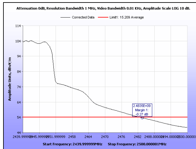
Plot 339. Radiated Restricted Band Edge, Average, Channel 7, 802.11g, Ant. 1
