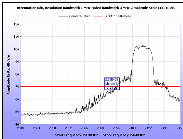
Plot 308. Radiated Restricted Band Edge, Peak, Channel 2, 802.11g, Ant. 0
