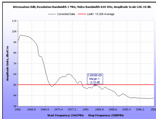
Plot 303. Radiated Restricted Band Edge, Average, Channel 11, 802.11b, Ant. 1
