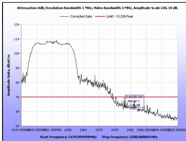
Plot 344. Radiated Restricted Band Edge, Peak, Channel 9, 802.11g, Ant. 1
