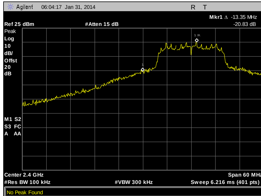
Plot 475. Conducted Band Edge, Low Channel, 802.11g, Ant. 0
