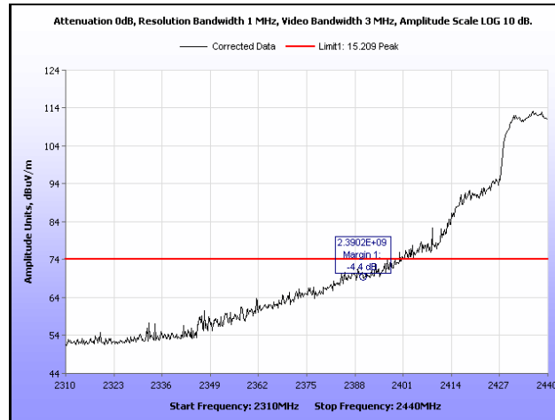
Plot 382. Radiated Restricted Band Edge, Peak, Channel 6, 802.11n 20 MHz, Ant. 1
