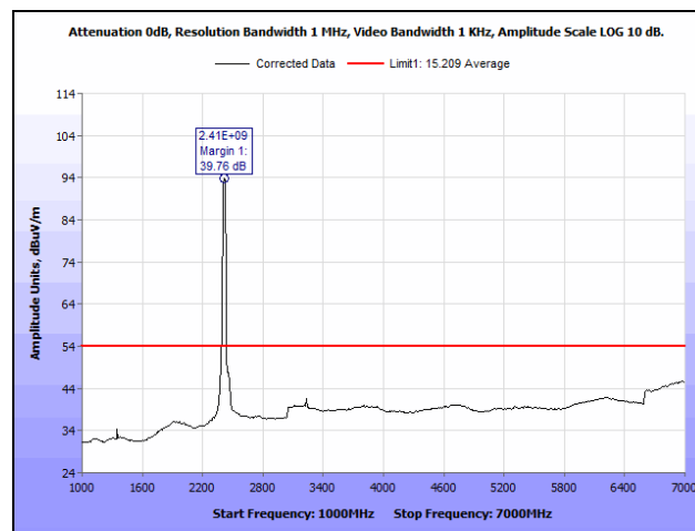
Plot 246. Radiated Spurious Emissions, Low Channel, 802.11n 40 MHz, Ant. 1, 1 GHz – 7 GHz, Average
