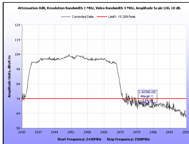
Plot 424. Radiated Restricted Band Edge, Peak, Channel 7, 802.11n 40 MHz, Ant. 1
