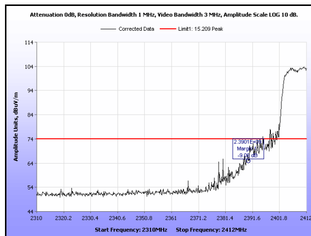
Plot 372. Radiated Restricted Band Edge, Peak, Channel 1, 802.11n 20 MHz, Ant. 1
