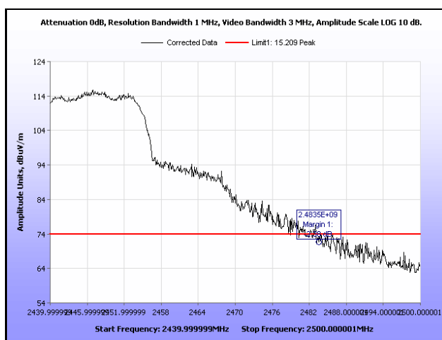
Plot 342. Radiated Restricted Band Edge, Peak, Channel 8, 802.11g, Ant. 1
