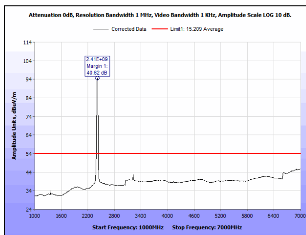
Plot 222. Radiated Spurious Emissions, Low Channel, 802.11n 20 MHz, Ant. 1, 1 GHz – 7 GHz, Average
