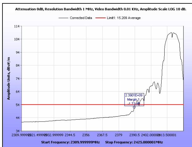
Plot 287. Radiated Restricted Band Edge, Average, Channel 2, 802.11b, Ant. 1
