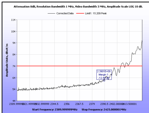
Plot 294. Radiated Restricted Band Edge, Peak, Channel 5, 802.11b, Ant. 1
