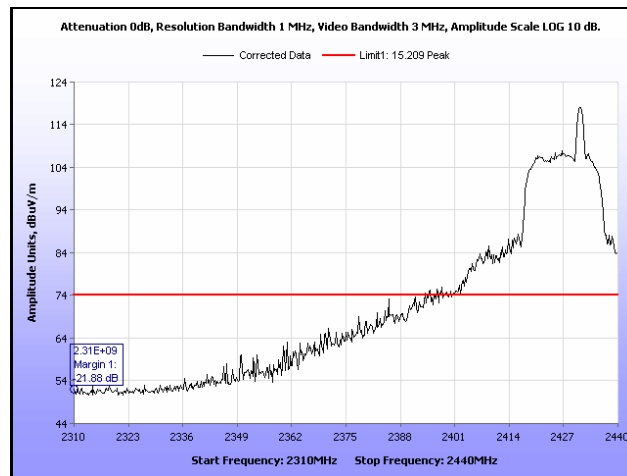
Plot 356. Radiated Restricted Band Edge, Peak, Channel 4, 802.11n 20 MHz, Ant. 0
