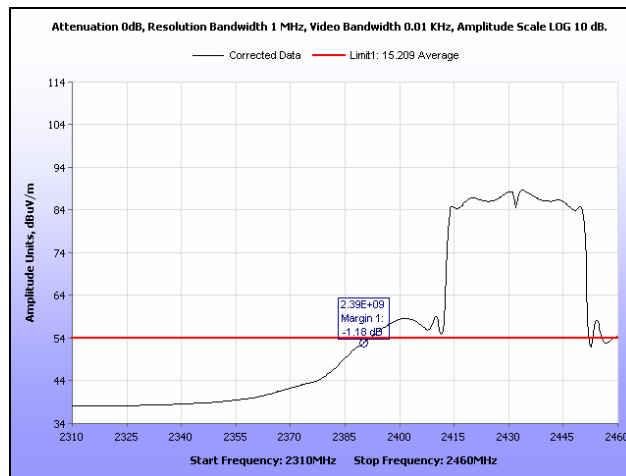
Plot 397. Radiated Restricted Band Edge, Average, Channel 3, 802.11n 40 MHz, Ant. 0
