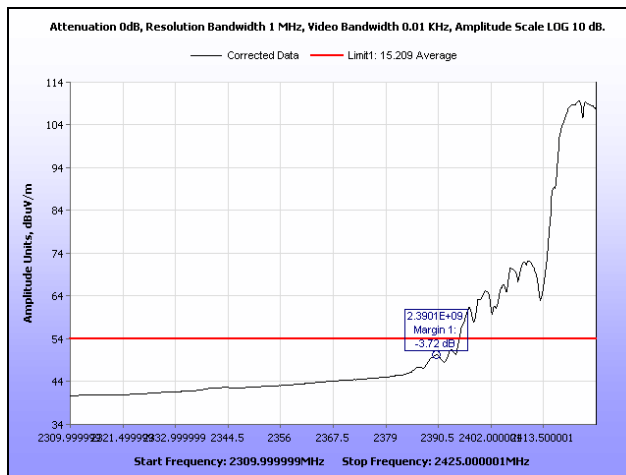
Plot 289. Radiated Restricted Band Edge, Average, Channel 3, 802.11b, Ant. 1
