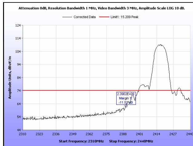
Plot 272. Radiated Restricted Band Edge, Peak, Channel 2, 802.11b, Ant. 0
