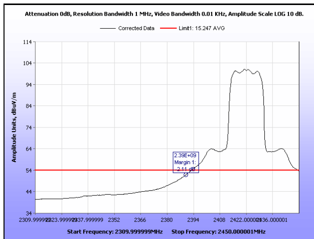
Plot 331. Radiated Restricted Band Edge, Average, Channel 3, 802.11g, Ant. 1
