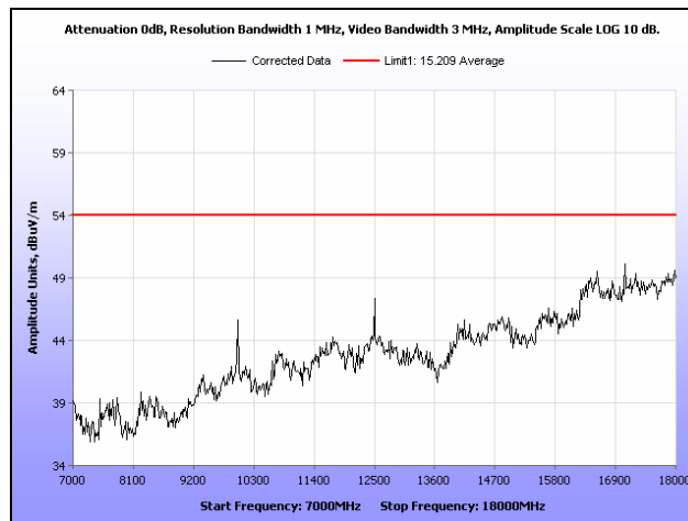
Plot 244. Radiated Spurious Emissions, High Channel, 802.11n 40 MHz, Ant. 0, 7 GHz – 18 GHz
