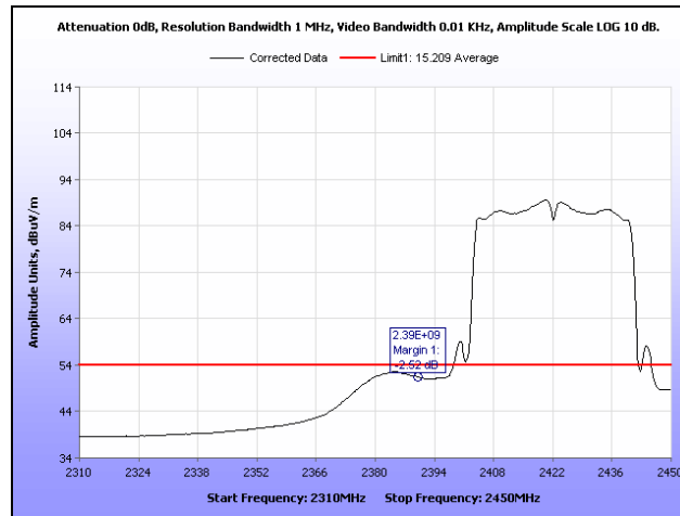
Plot 429. Radiated Restricted Band Edge, Average, Channel 1, 802.11n 40 MHz, MIMO
