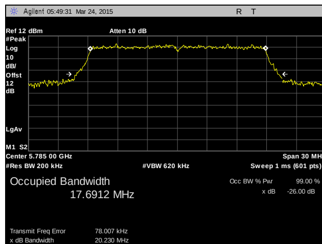
Plot 30. 26 dB Occupied Bandwidth, Mid Channel, 802.11ac 20 MHz, MIMO, Transmitting Beam-Forming
