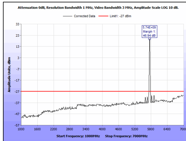
Plot 119. Radiated Spurious Emissions, Low Channel, 802.11a 20 MHz, MIMO, Non-TX BF, 1 GHz – 7 GHz
