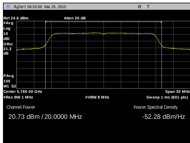
Plot 69. RF Output Power, Mid Channel, 802.11ac 20 MHz, MIMO, Transmitting Beam-Forming
