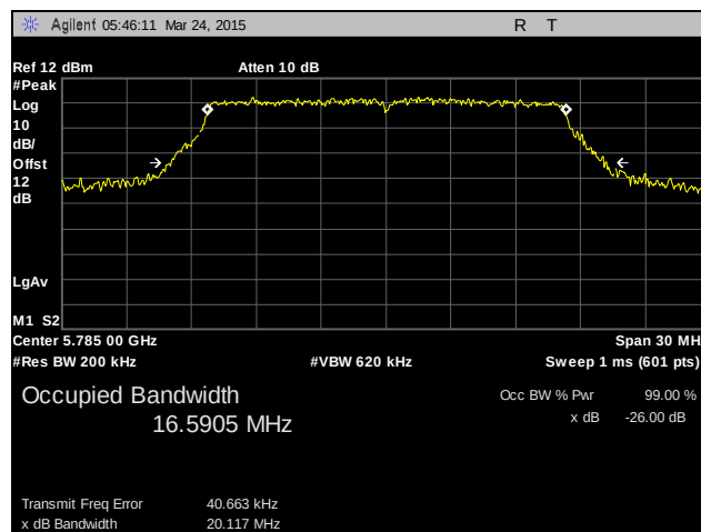
Plot 2. 26 dB Occupied Bandwidth, Mid Channel, 802.11a 20 MHz, MIMO, Non-Transmitting Beam-Forming
