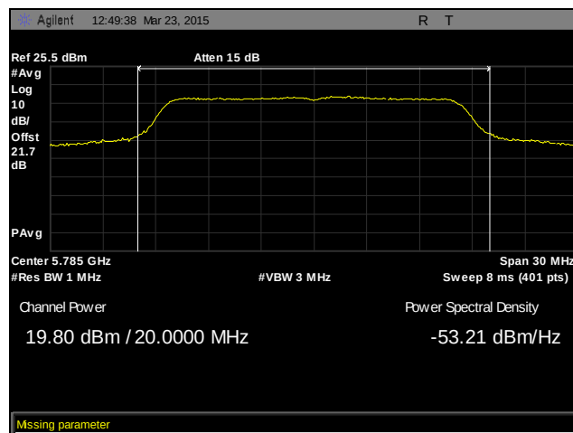
Plot 55. RF Output Power, Mid Channel, 802.11a 20 MHz, SISO, Non-Transmitting Beam-Forming
