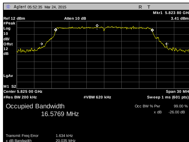
Plot 3. 26 dB Occupied Bandwidth, High Channel, 802.11a 20 MHz, MIMO, Non-Transmitting Beam-Forming
