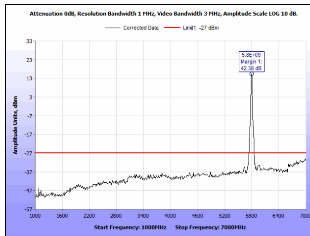
Plot 155. Radiated Spurious Emissions, High Channel, 802.11n 40 MHz, MIMO, Non-TX BF, 1 GHz – 7 GHz
