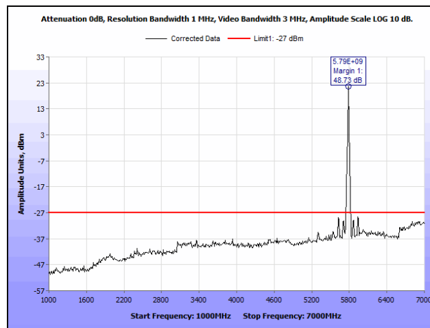
Plot 206. Radiated Spurious Emissions, Mid Channel, 802.11ac 20 MHz, MIMO, TX BF, 1 GHz – 7 GHz
