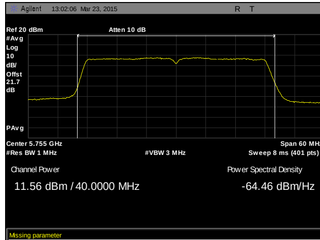
Plot 49. RF Output Power, Low Channel, 802.11ac 40 MHz, MIMO, Non-Transmitting Beam-Forming
