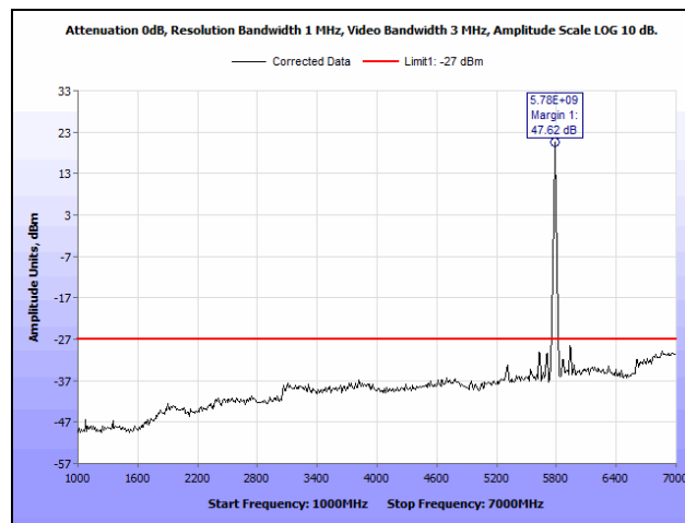
Plot 122. Radiated Spurious Emissions, Mid Channel, 802.11a 20 MHz, MIMO, Non-TX BF, 1 GHz – 7 GHz
