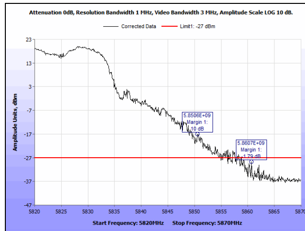
Plot 236. Radiated Band Edge, High Channel, 802.11a 20 MHz, MIMO, Non-Transmitting Beam-Forming
