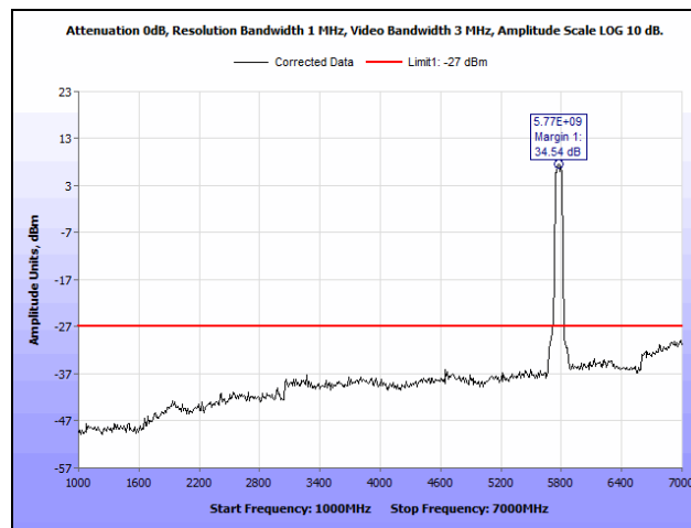
Plot 158. Radiated Spurious Emissions, 802.11ac 80 MHz, MIMO, Non-TX BF, 1 GHz – 7 GHz
