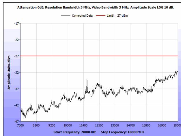
Plot 126. Radiated Spurious Emissions, High Channel, 802.11a 20 MHz, MIMO, Non-TX BF, 7 GHz – 18 GHz
