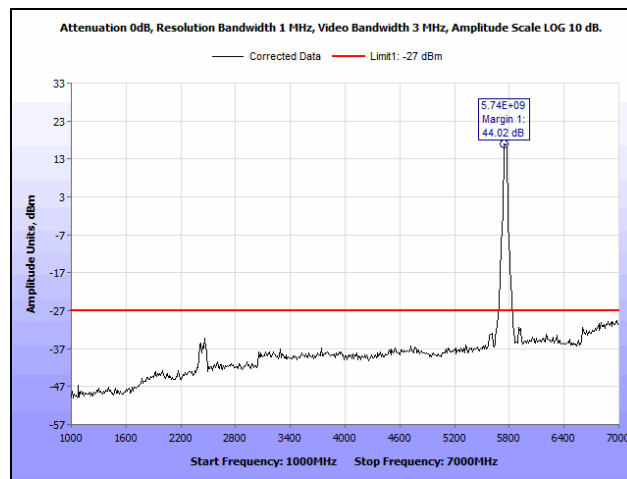
Plot 194. Radiated Spurious Emissions, Low Channel, 802.11n 40 MHz, SISO, Non-TX BF, 1 GHz – 7 GHz
