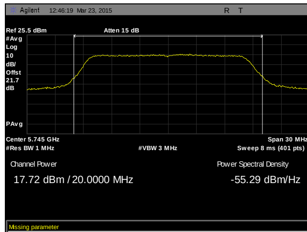
Plot 54. RF Output Power, Low Channel, 802.11a 20 MHz, SISO, Non-Transmitting Beam-Forming
