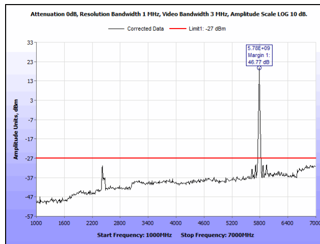
Plot 173. Radiated Spurious Emissions, Mid Channel, 802.11ac 20 MHz, SISO, Non-TX BF, 1 GHz – 7 GHz
