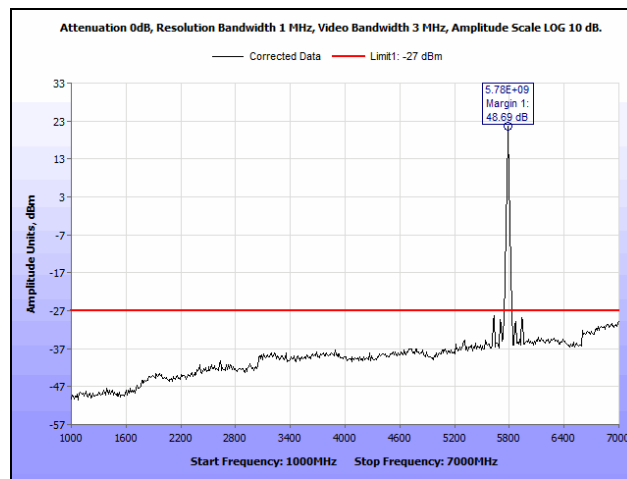
Plot 215. Radiated Spurious Emissions, Mid Channel, 802.11n 20 MHz, MIMO, TX BF, 1 GHz – 7 GHz
