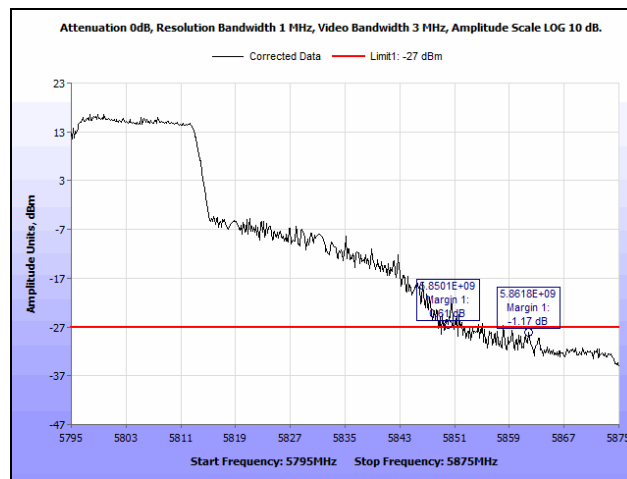
Plot 253. Radiated Band Edge, High Channel, 802.11ac 40 MHz, SISO, Non-Transmitting Beam-Forming
