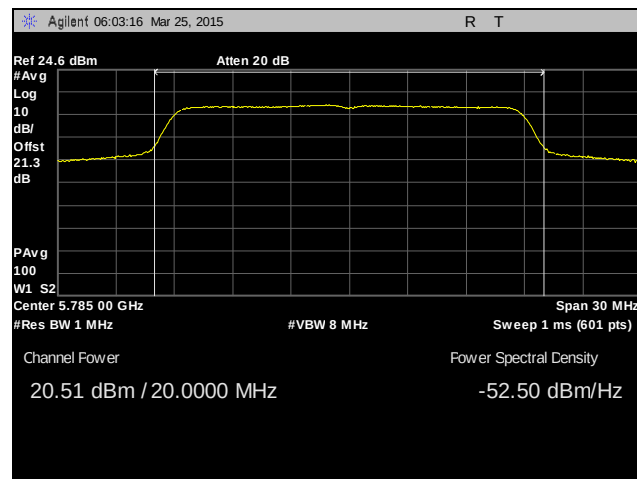
Plot 72. RF Output Power, Mid Channel, 802.11n 20 MHz, MIMO, Transmitting Beam-Forming
