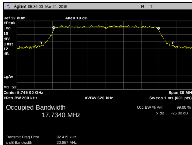
Plot 29. 26 dB Occupied Bandwidth, Low Channel, 802.11ac 20 MHz, MIMO, Transmitting Beam-Forming
