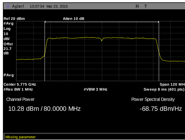
Plot 53. RF Output Power, 802.11ac 80 MHz, MIMO, Non-Transmitting Beam-Forming
