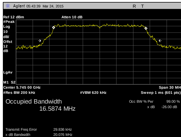
Plot 1. 26 dB Occupied Bandwidth, Low Channel, 802.11a 20 MHz, MIMO, Non-Transmitting Beam-Forming
