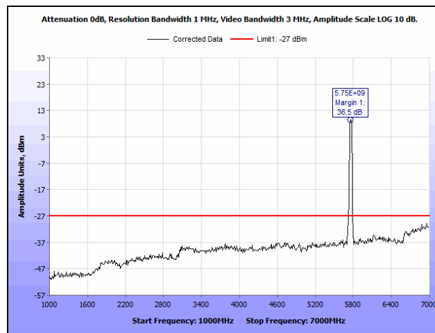
Plot 227. Radiated Spurious Emissions, Low Channel, 802.11n 40 MHz, MIMO, TX BF, 1 GHz – 7 GHz
