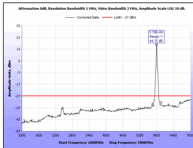
Plot 197. Radiated Spurious Emissions, High Channel, 802.11n 40 MHz, SISO, Non-TX BF, 1 GHz – 7 GHz
