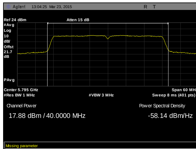
Plot 50. RF Output Power, High Channel, 802.11ac 40 MHz, MIMO, Non-Transmitting Beam-Forming
