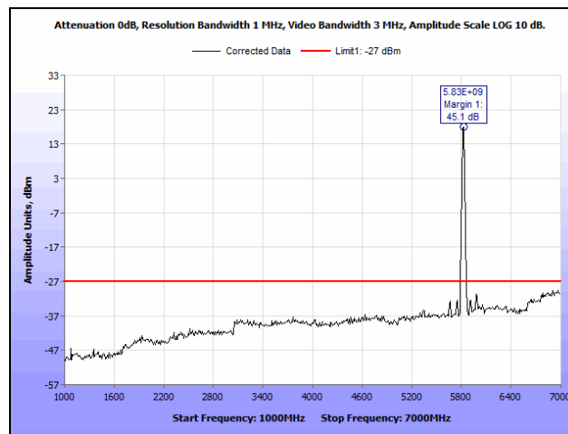
Plot 143. Radiated Spurious Emissions, High Channel, 802.11n 20 MHz, MIMO, Non-TX BF, 1 GHz – 7 GHz
