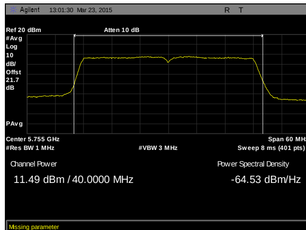
Plot 51. RF Output Power, Low Channel, 802.11n 40 MHz, MIMO, Non-Transmitting Beam-Forming
