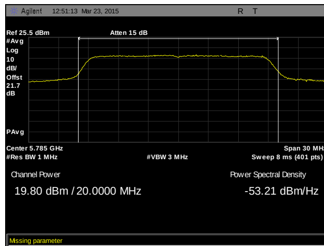
Plot 44. RF Output Power, Mid Channel, 802.11ac 20 MHz, MIMO, Non-Transmitting Beam-Forming
