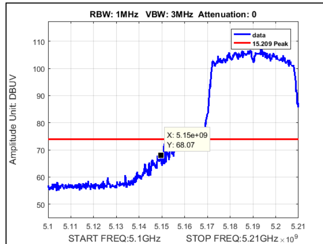
Plot 85. Peak Band Edge Spurious, BW 40M, Ch. 5190M, 80211n, MCS24, P3230
