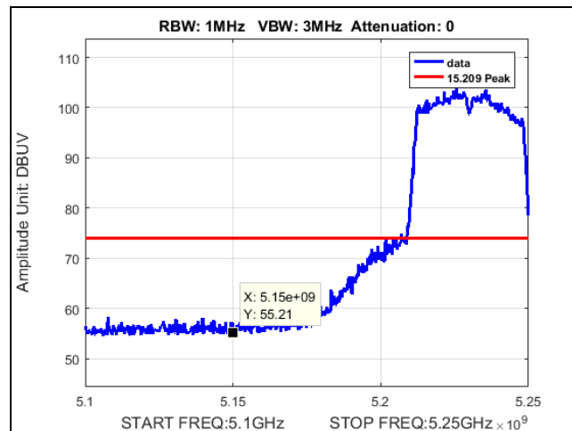
Plot 87. Peak Band Edge Spurious, BW 40M, Ch. 5230M, 80211n, MCS24, P3230
