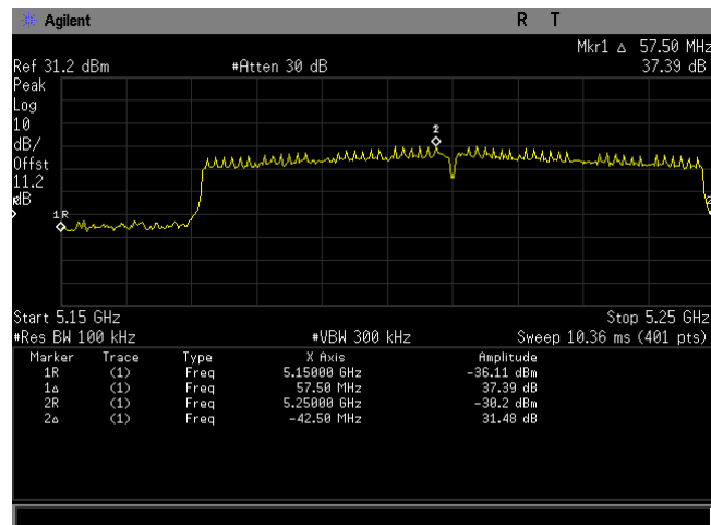
Plot 96. Frequency Stability, 80211ac BW 80MHz
