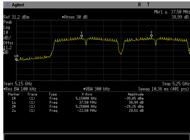
Plot 94. Frequency Stability, 80211n BW 40MHz
