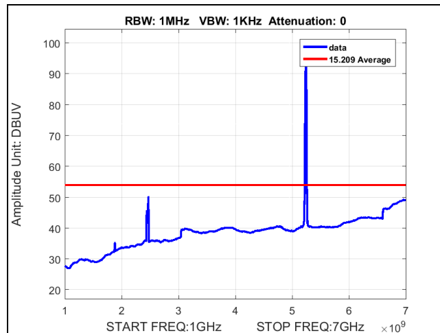
Plot 45. Average Spurious Emission, 1-7 GHz, BW 20M, Ch. 5240M, 80211a, MCS0, P3230
