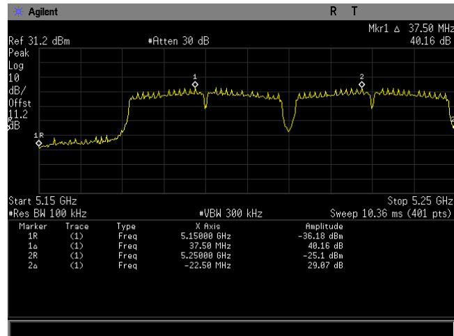
Plot 106. Frequency Stability, 80211n BW 40MHz
