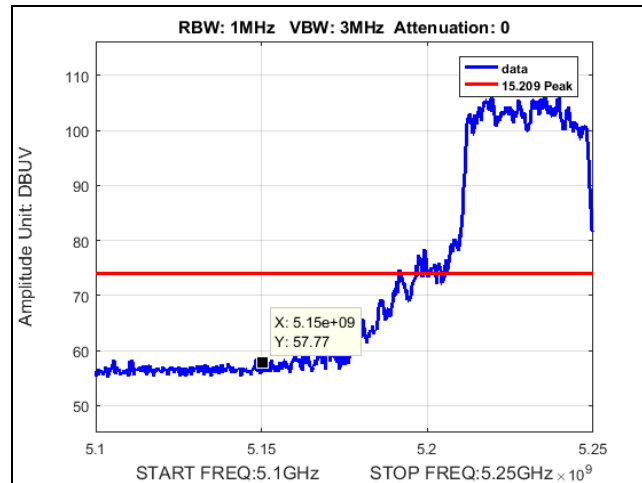
Plot 86. Peak Band Edge Spurious, BW 40M, Ch. 5230M, 80211ac, MCS24, P3230
