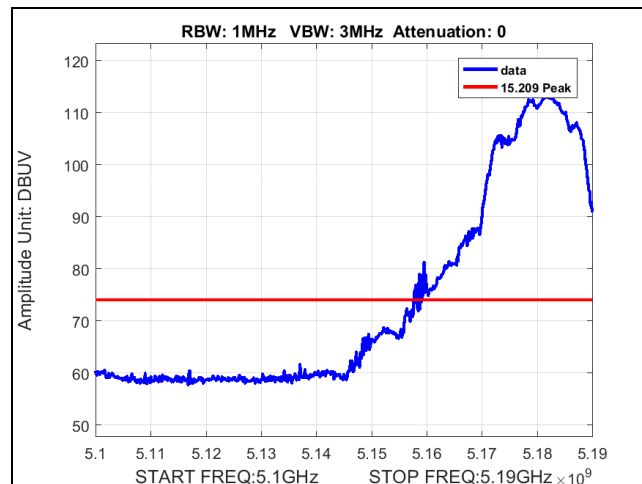
Plot 78. Peak Band Edge Spurious, BW 20M, Ch. 5180M, 80211a, MCS0, P3230
