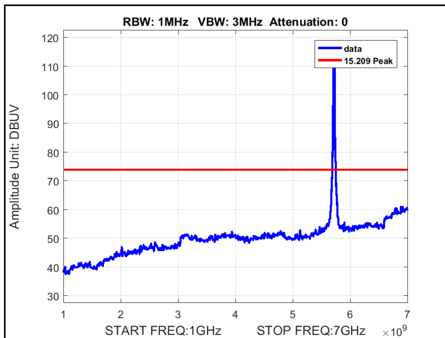
Plot 101. Radiated Spurious Emissions, 5700 MHz, 802.11a, 1 GHz – 7 GHz, Peak
