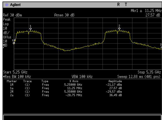
Plot 189. Frequency Stability, 802.11a, UNII2A, 40°C/133V
