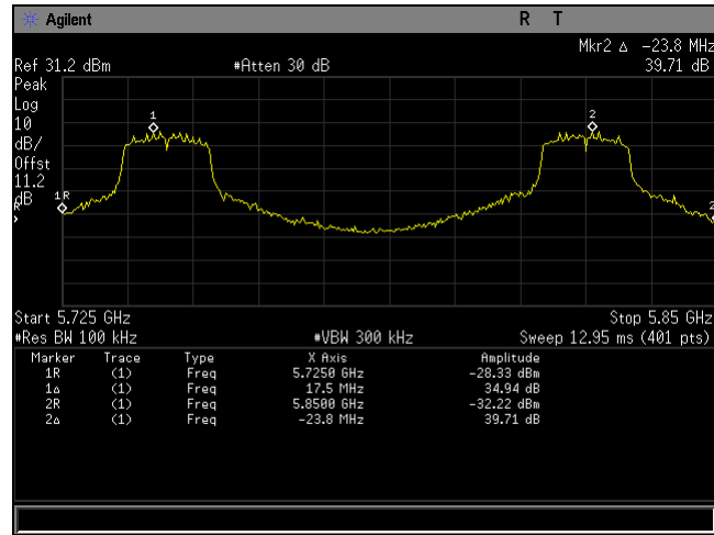
Plot 76. Frequency Stability, 80211a BW 20MHz
