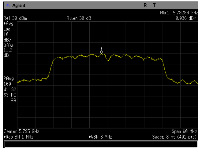
Plot 27. Power Spectral Density, BW 40M, Ch 5795M, 80211n, MSC24, P3230, CH0
