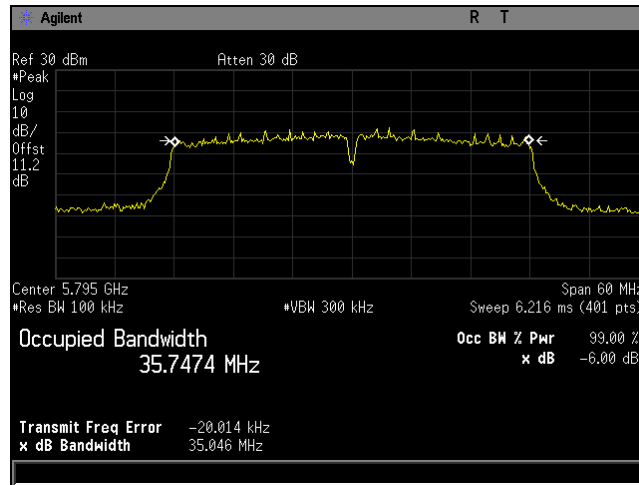
Plot 68. 6 dB Bandwidth, BW 40M, Ch 5795M, 80211n, MCS16, P3230, CH0
