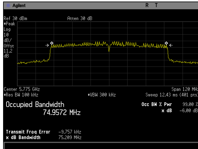
Plot 69. 6 dB Bandwidth, BW 80M, Ch 5775M, 80211ac, MCS24, P3230, CH0
