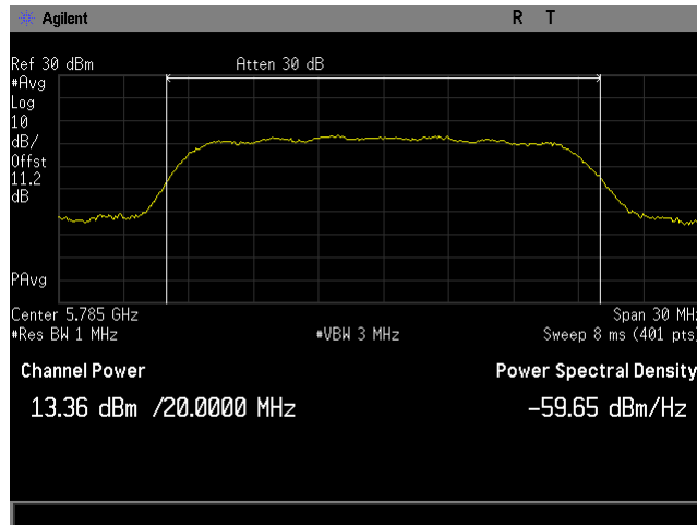
Plot 5. Maximum Conducted Output Power, BW 20M, Ch 5785M, 80211ac, MCS24, P3230, CH0
