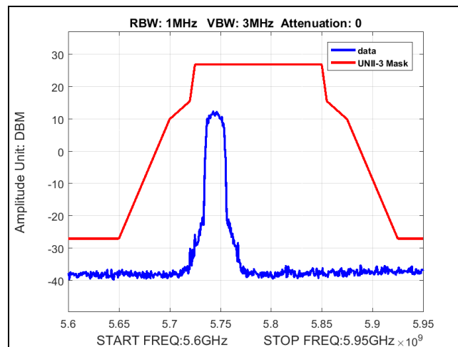
Plot 45. Band Edge, BW 20M, Ch 5745M, 80211n, MCS24, P3230
