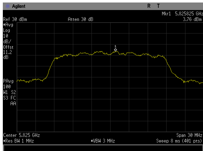
Plot 23. Power Spectral Density, BW 20M, Ch 5825M, 80211n, MSC24, P3230, CH0
