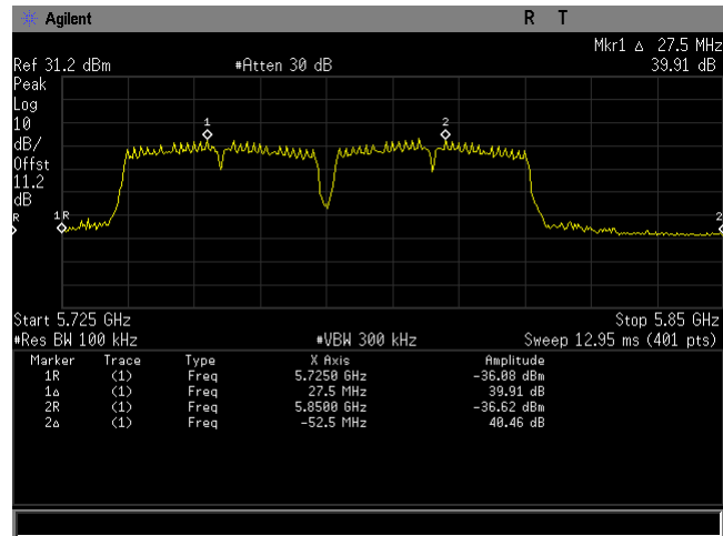
Plot 73. Frequency Stability, 80211n BW 40MHz
