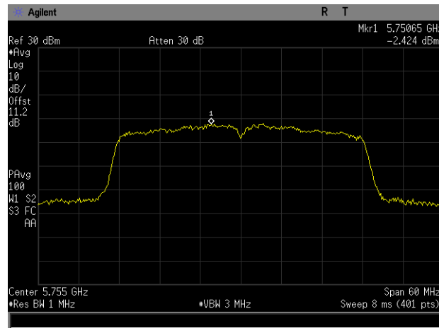
Plot 24. Power Spectral Density, BW 40M, Ch 5755M, 80211ac, MCS24, P3230 CH0
