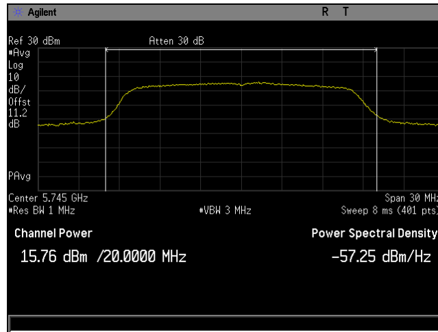
Plot 1. Maximum Conducted Output Power, BW 20M, Ch 5745M, 80211a, MSC0, P3230, CH0
