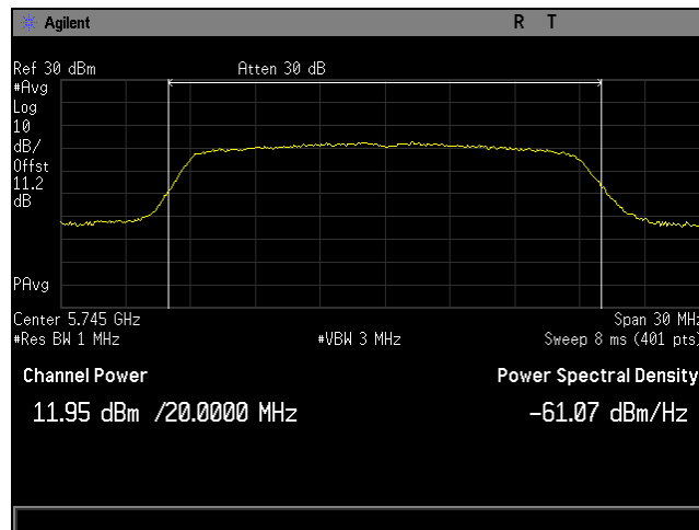
Plot 3. Maximum Conducted Output Power, BW 20M, Ch 5745M, 80211n, MSC24, P3230, CH0
