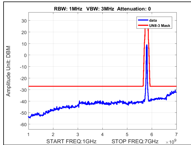
Plot 38. Undesirable Emissions, BW 40M, Ch 5795M, 80211n, MCS24, P3230
