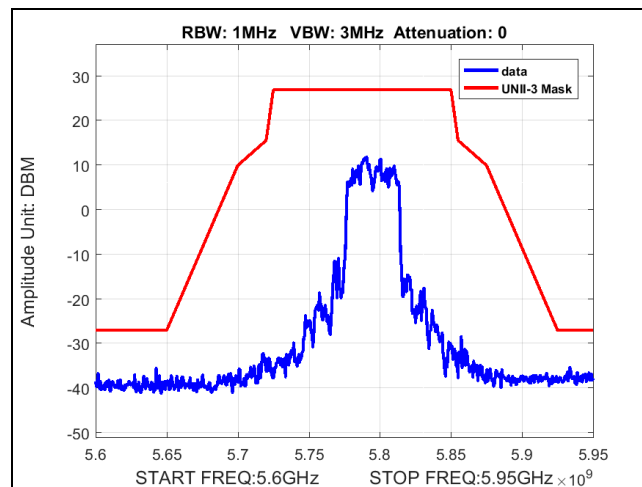
Plot 51. Band Edge, BW 40M, Ch 5795M, 80211ac, MCS24, P3230
