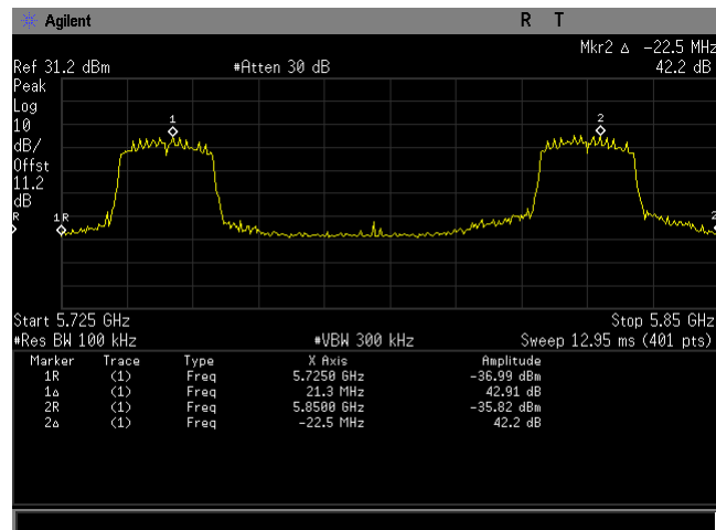
Plot 72. Frequency Stability, 80211n BW 20MHz
