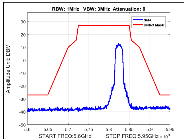
Plot 47. Band Edge, BW 20M, Ch 5825M, 80211ac, MCS24, P3230
