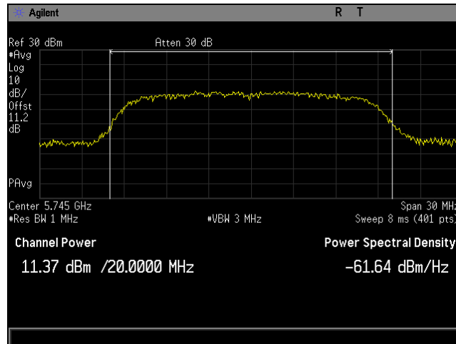
Plot 2. Maximum Conducted Output Power, BW 20M, Ch 5745M, 80211ac, MCS24, P3230 CH0
