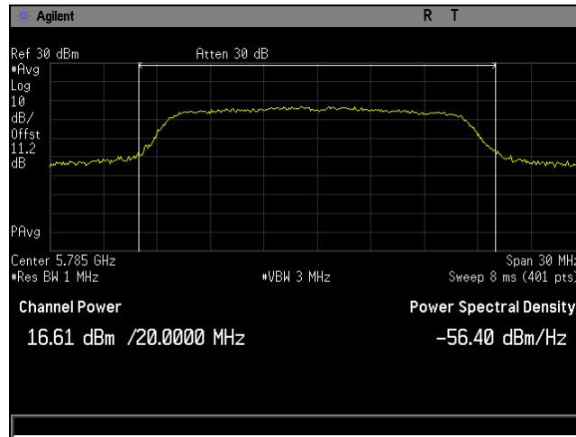
Plot 4. Maximum Conducted Output Power, BW 20M, Ch 5785M, 80211a, MSC0, P3230, CH0
