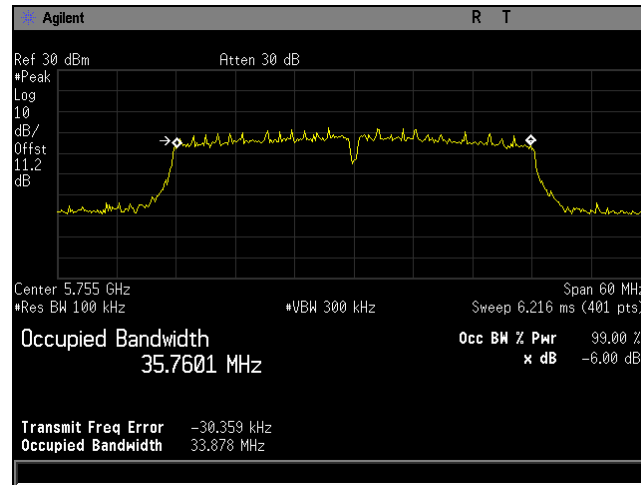
Plot 65. 6 dB Bandwidth, BW 40M, Ch 5755M, 80211ac, MCS24, P3230, CH0
