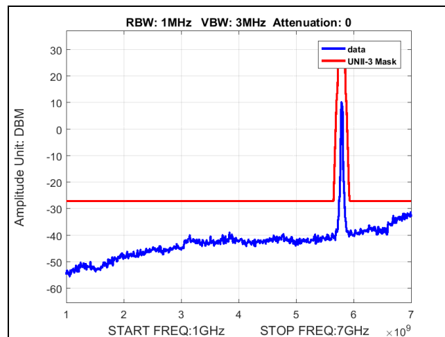
Plot 37. Undesirable Emissions, BW 40M, Ch 5795M, 80211ac, MCS24, P3230
