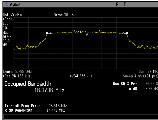
Plot 59. 6 dB Bandwidth, BW 20M, Ch 5785M, 80211a, MCS0, P3230, CH0
