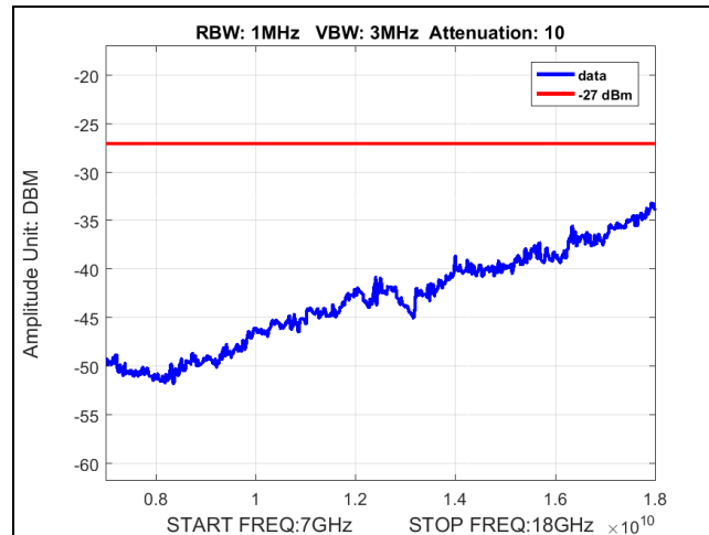
Plot 39. Undesirable Emissions, BW 80M, Ch 5775M, 7-18GHz
