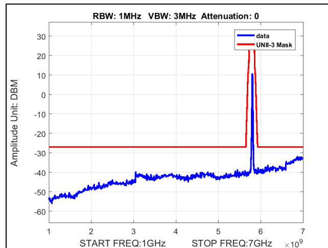
Plot 33. Undesirable Emissions, BW 20M, Ch 5825M, 80211ac, MCS24, P3230
