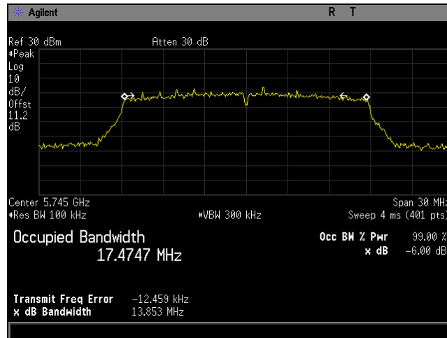
Plot 57. 6 dB Bandwidth, BW 20M, Ch 5745M, 80211ac, MCS24, P3230, CH0
