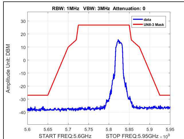
Plot 46. Band Edge, BW 20M, Ch 5825M, 80211a, MCS0, P3230
