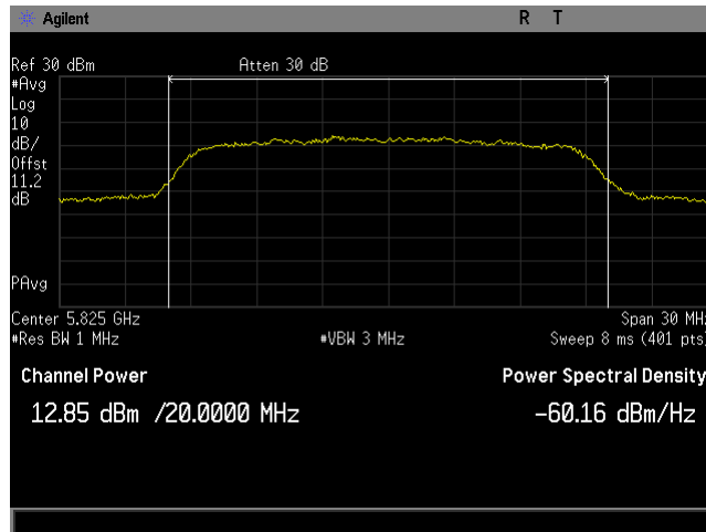
Plot 8. Maximum Conducted Output Power, BW 20M, Ch 5825M, 80211ac, MSC24, P3230, CH0
