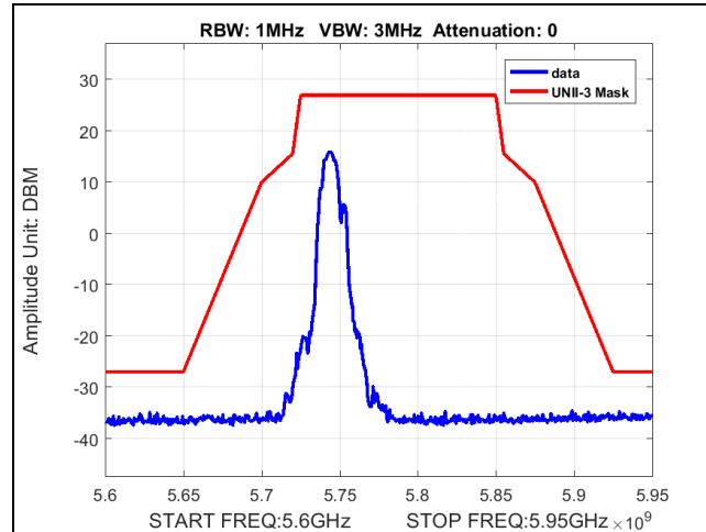
Plot 43. Band Edge, BW 20M, Ch 5745M, 80211a, MCS0, P3230
