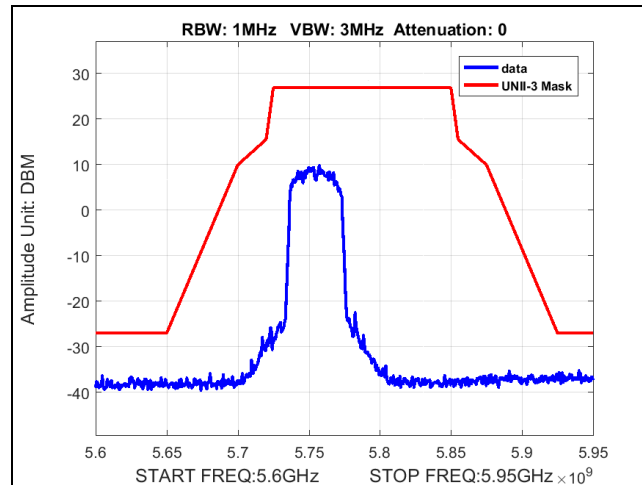
Plot 50. Band Edge, BW 40M, Ch 5755M, 80211n, MCS24, P3230
