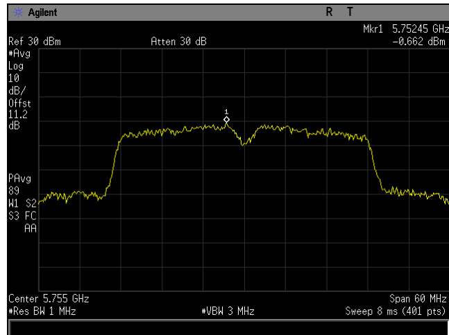
Plot 25. Power Spectral Density, BW 40M, Ch 5755M, 80211n, MCS24, P3230, CH0
