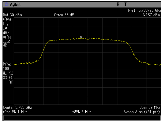
Plot 18. Power Spectral Density, BW 20M, Ch 5785M, 80211a, MSC0, P3230, CH0
