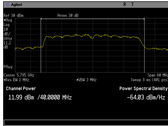
Plot 13. Maximum Conducted Output Power, BW 40M, Ch 5795M, 80211n, MSC24, P3230, CH0
