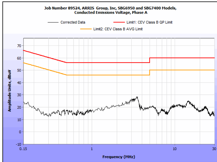
Plot 55. Conducted Emissions, Phase
