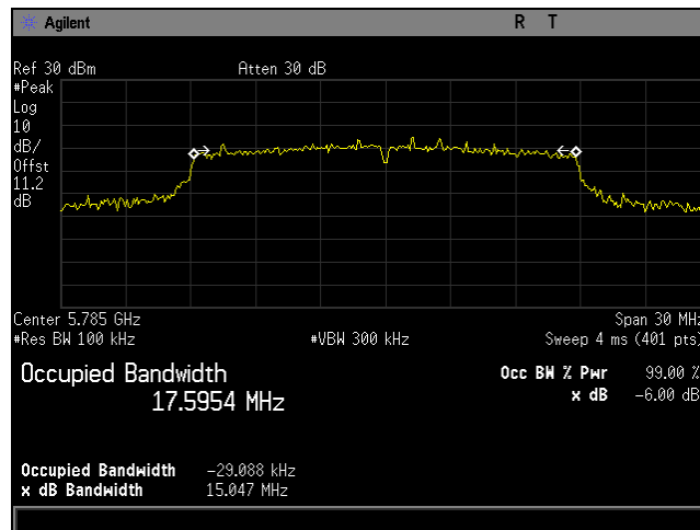
Plot 61. 6 dB Bandwidth, BW 20M, Ch 5785M, 80211n, MCS16, P3230, CH0
