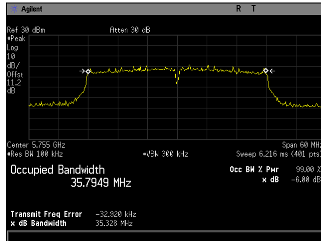
Plot 66. 6 dB Bandwidth, BW 40M, Ch 5755M, 80211n, MCS16, P3230, CH0
