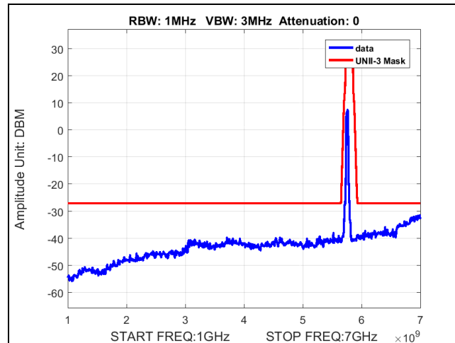
Plot 36. Undesirable Emissions, BW 40M, Ch 5755M, 80211n, MCS24, P3230
