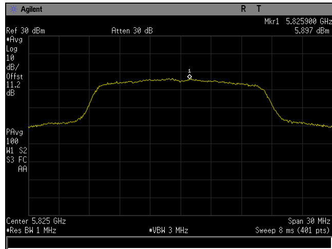
Plot 21. Power Spectral Density, BW 20M, Ch 5825M, 80211a, MSC0, P3230, CH0
