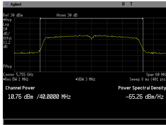
Plot 10. Maximum Conducted Output Power, BW 40M, Ch 5755M, 80211ac, MCS24 P3230, CH0
