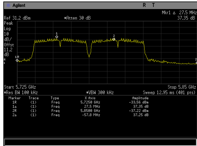
Plot 85. Frequency Stability, 80211n BW 40MHz
