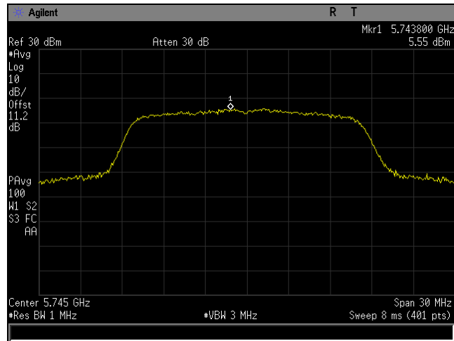
Plot 15. Power Spectral Density, BW 20M, Ch 5745M, 80211a, MSC0, P3230, CH0
