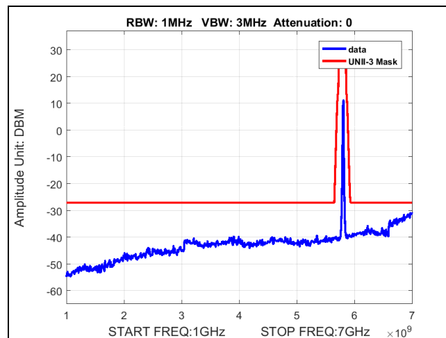
Plot 34. Undesirable Emissions, BW 20M, Ch 5825M, 80211n, MCS24, P3230
