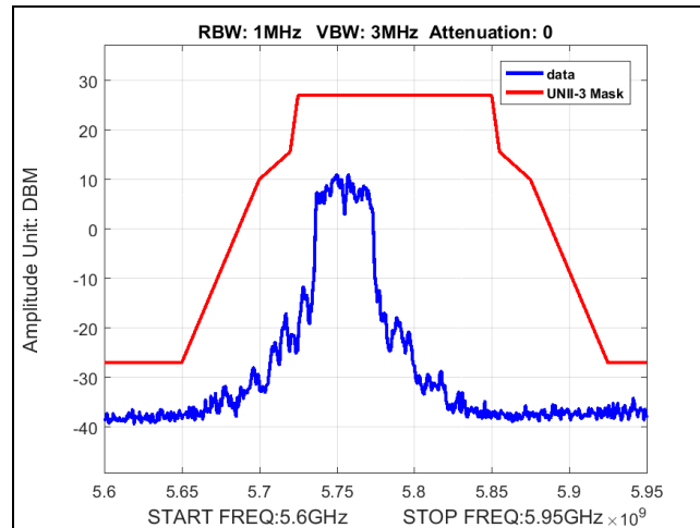
Plot 49. Band Edge, BW 40M, Ch 5755M, 80211ac, MCS24, P3230
