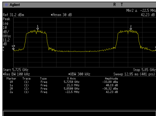
Plot 71. Frequency Stability, 80211ac BW 20MHz
