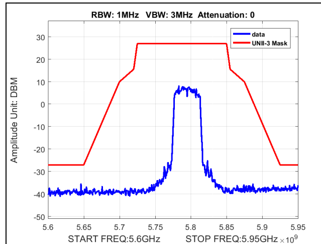
Plot 52. Band Edge, BW 40M, Ch 5795M, 80211n, MCS24, P3230
