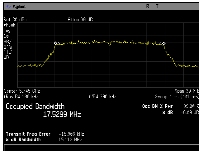
Plot 58. 6 dB Bandwidth, BW 20M, Ch 5745M, 80211n, MCS16, P3230, CH0
