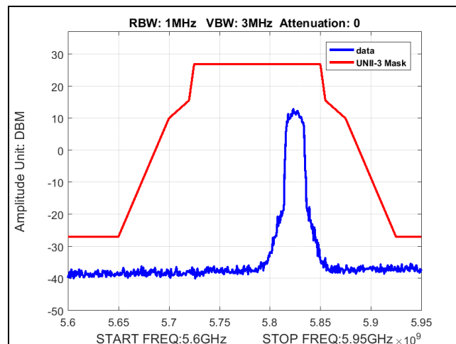
Plot 48. Band Edge, BW 20M, Ch 5825M, 80211n, MCS24, P3230
