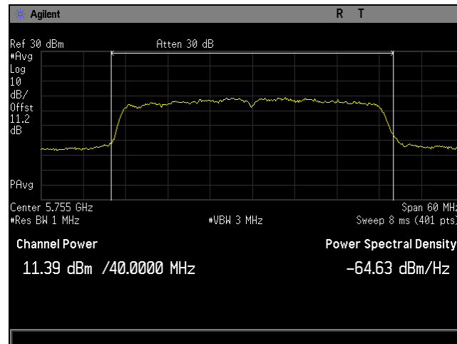
Plot 11. Maximum Conducted Output Power, BW 40M, Ch 5755M, 80211n, MSC24 P3230, CH0
