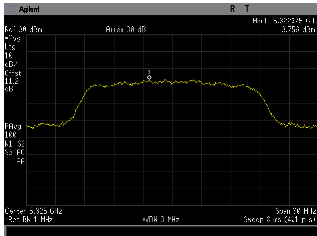
Plot 22. Power Spectral Density, BW 20M, Ch 5825M, 80211ac, MSC24, P3230, CH0
