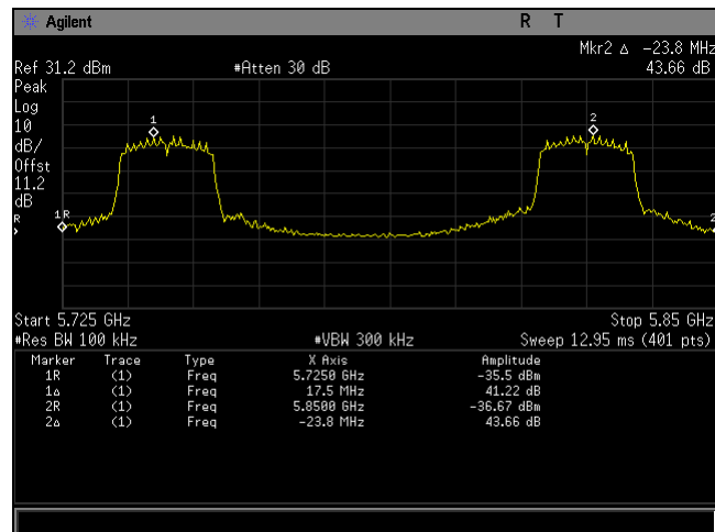
Plot 77. Frequency Stability, 80211ac BW 20MHz
