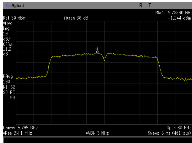
Plot 26. Power Spectral Density, BW 40M, Ch 5795M, 80211ac, MCS24, P3230, CH0
