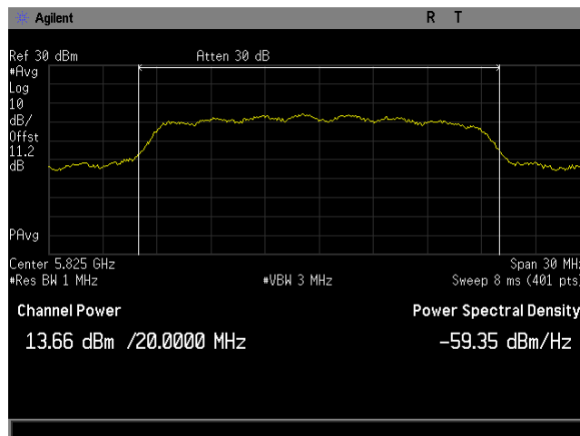
Plot 9. Maximum Conducted Output Power, BW 20M, Ch 5825M, 80211n MSC24, P3230, CH0
