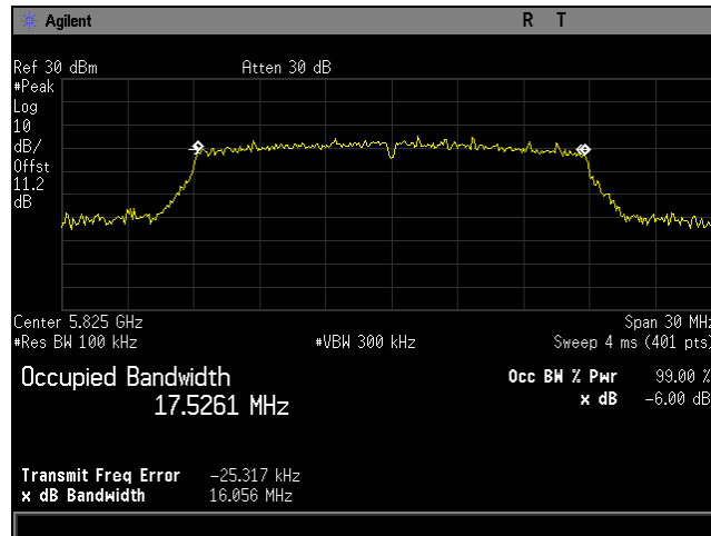
Plot 64. 6 dB Bandwidth, BW 20M, Ch 5825M, 80211n, MCS16, P3230, CH0
