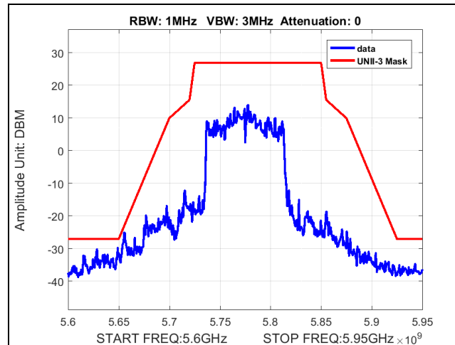
Plot 53. Band Edge, BW 80M, Ch 5775M, 80211ac, MCS24, P3230
