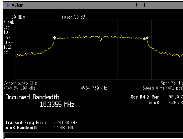
Plot 56. 6 dB Bandwidth, BW 20M, Ch 5745M, 80211a, MCS0, P3230, CH0
