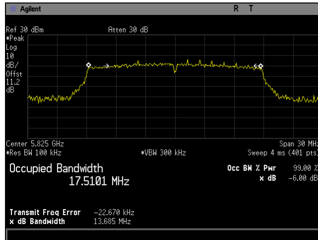
Plot 63. 6 dB Bandwidth, BW 20M, Ch 5825M, 80211ac, MCS24, P3230, CH0
