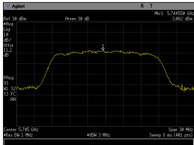
Plot 17. Power Spectral Density, BW 20M, Ch 5745M, 80211n, MSC24, P3230, CH0
