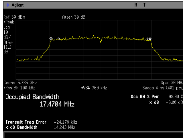
Plot 60. 6 dB Bandwidth, BW 20M, Ch 5785M, 80211ac, MCS24, P3230, CH0
