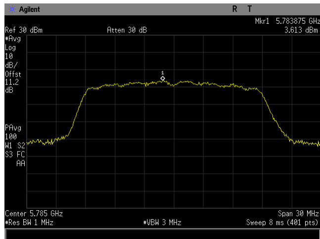
Plot 19. Power Spectral Density, BW 20M, Ch 5785M, 80211ac, MCS24, P3230, CH0
