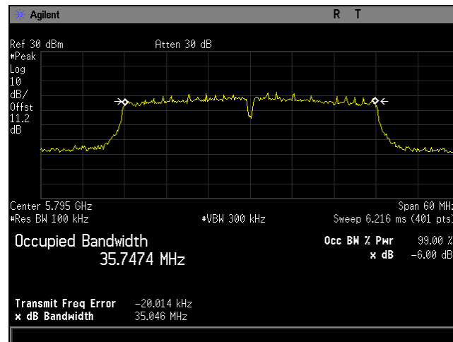
Plot 67. 6 dB Bandwidth, BW 40M, Ch 5795M, 80211ac, MCS24, P3230, CH0
