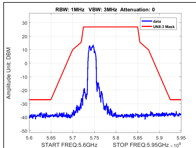
Plot 44. Band Edge, BW 20M, Ch 5745M, 80211ac, MCS24, P3230
