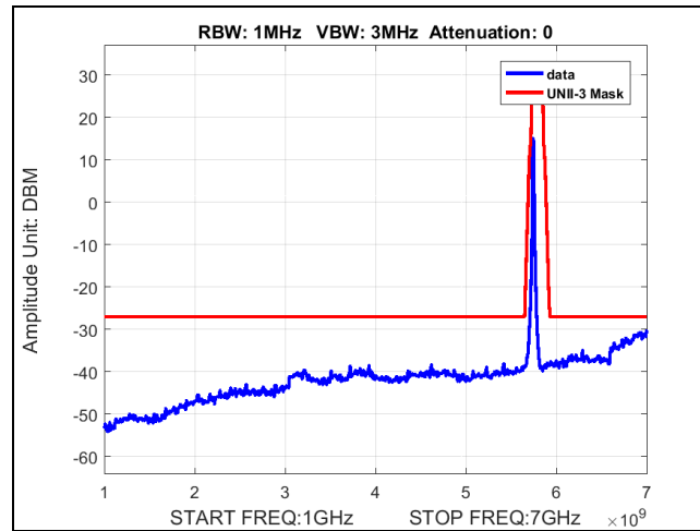
Plot 29. Undesirable Emissions, BW 20M, Ch 5745M, 80211a, MCS0, P3230
