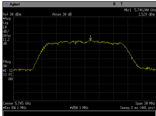
Plot 16. Power Spectral Density, BW 20M, Ch 5745M, 80211ac, MCS24, P3230, CH0
