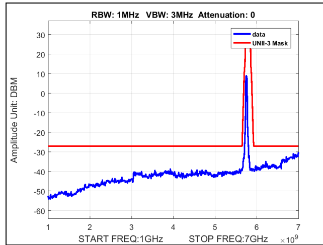
Plot 35. Undesirable Emissions, BW 40M, Ch 5755M, 80211ac, MCS24, P3230
