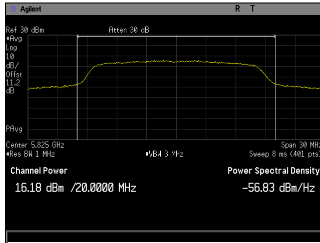
Plot 7. Maximum Conducted Output Power, BW 20M, Ch 5825M, 80211a MSC0 P3230, CH0
