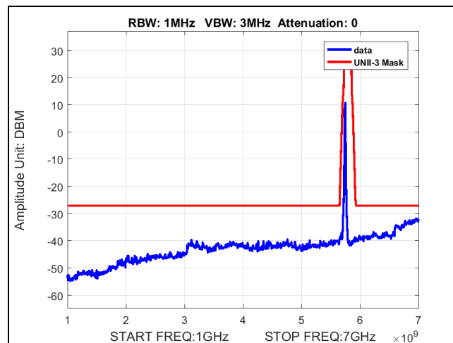
Plot 31. Undesirable Emissions, BW 20M, Ch 5745M, 80211n, MCS24, P3230
