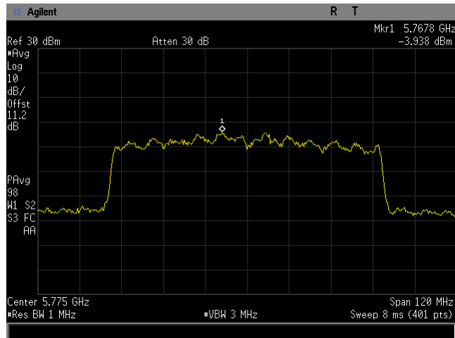
Plot 28. Power Spectral Density, BW 80M, Ch 5775M, 80211ac, MSC24, P3230, CH0
