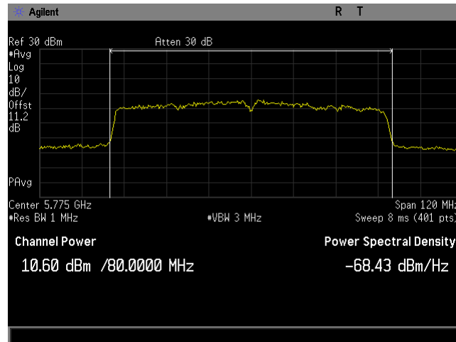
Plot 14. Maximum Conducted Output Power, BW 80M, Ch 5775M, 80211ac, MSC24, P3230, CH0
