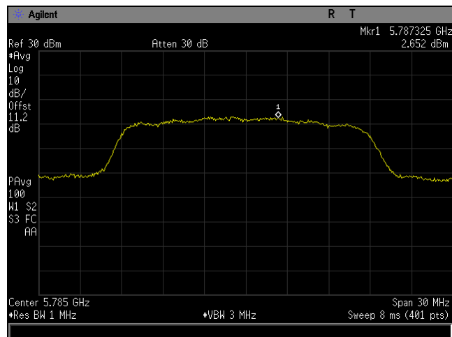
Plot 20. Power Spectral Density, BW 20M, Ch 5785M, 80211n, MSC24, P3230, CH0
