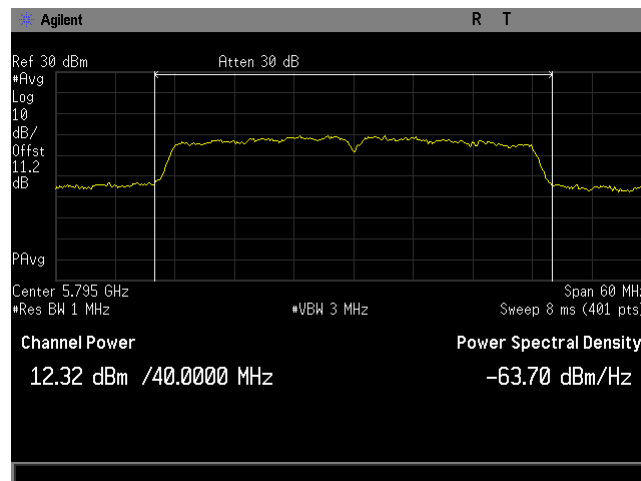
Plot 12. Maximum Conducted Output Power, BW 40M, Ch 5795M, 80211ac, MCS24, P3230, CH0
