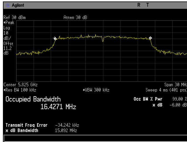
Plot 62. 6 dB Bandwidth, BW 20M, Ch 5825M, 80211a, MCS0, P3230, CH0
