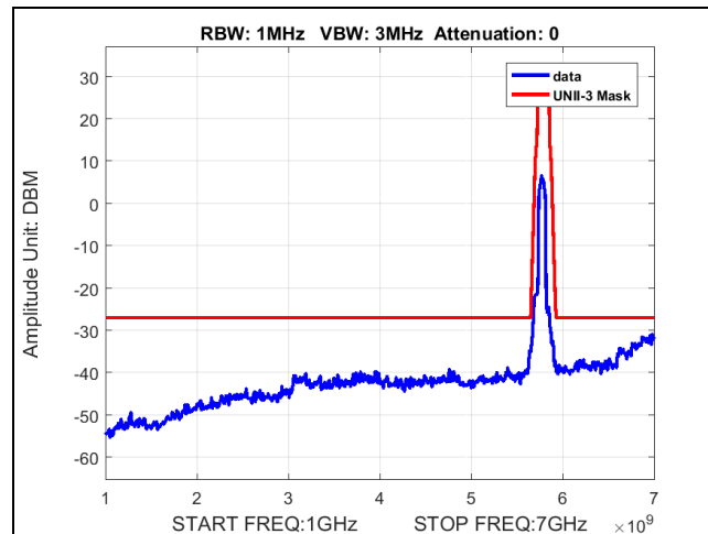
Plot 40. Undesirable Emissions, BW 80M, Ch 5775M, 80211ac, MCS24, P3230
