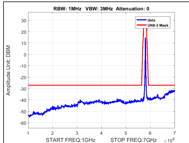
Plot 32. Undesirable Emissions, BW 20M, Ch 5825M, 80211a, MCS0, P3230
