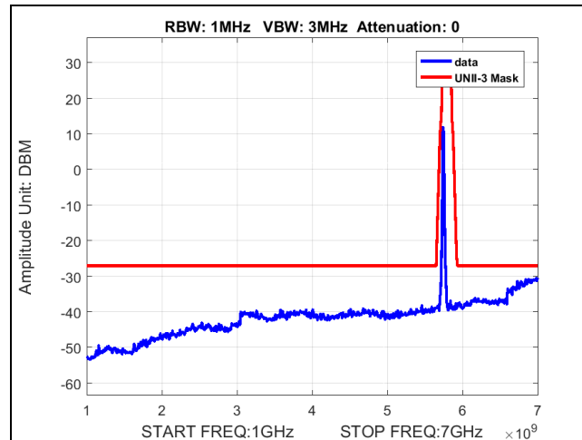
Plot 30. Undesirable Emissions, BW 20M, Ch 5745M, 80211ac, MCS24, P3230
