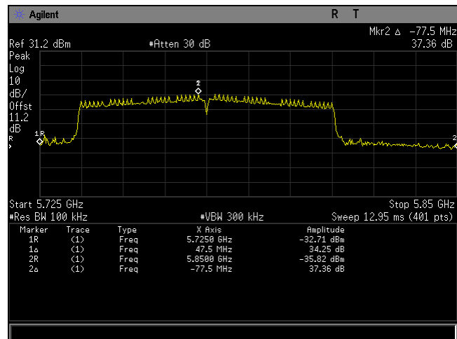
Plot 87. Frequency Stability, 80211ac BW 80MHz
