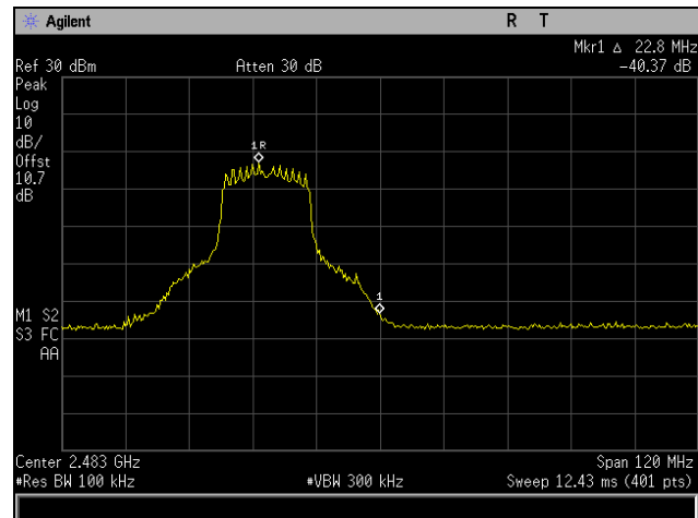
Plot 74. Conducted Band Edge, High Channel, 802.11g
