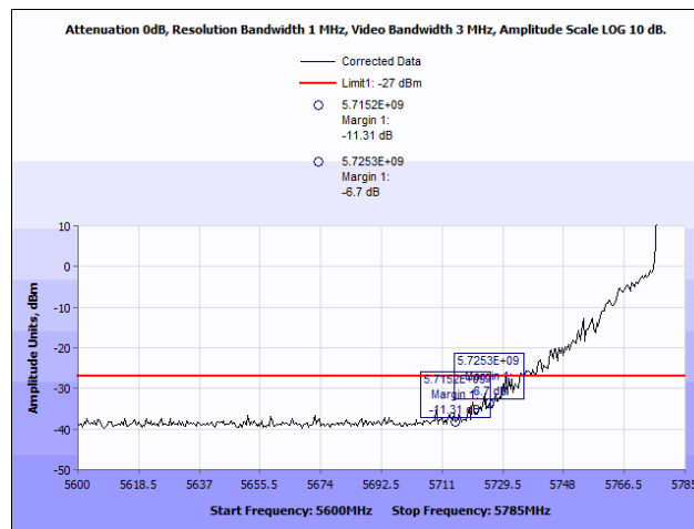
Plot 117. Radiated Band Edge, Mid Channel, 802.11n 20 MHz
