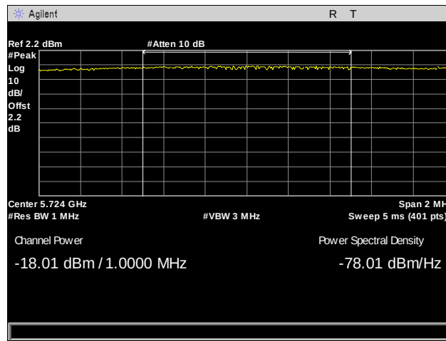
Plot 123. Radiated Band Edge, Channel 149, 802.11n 20 MHz, Integration at 5725 MHz
