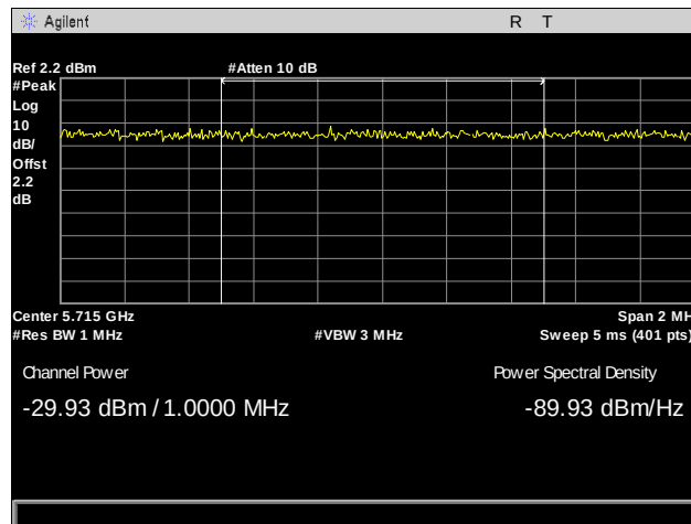
Plot 129. Radiated Band Edge, Channel 149, 802.11n 40 MHz, Integration at 5715 MHz
