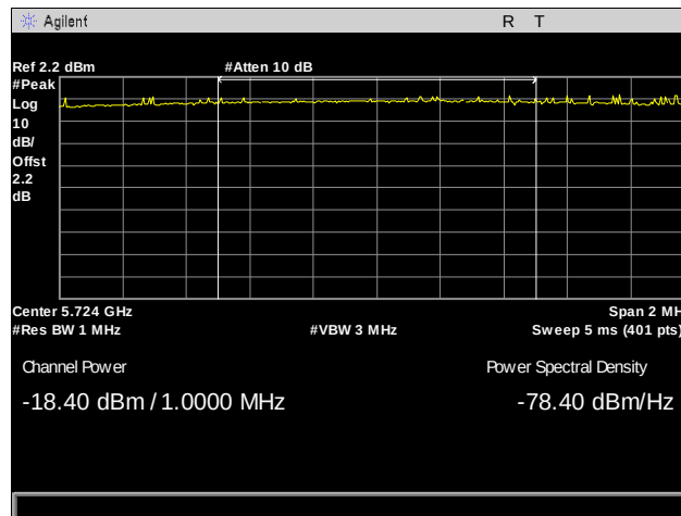
Plot 104. Radiated Band Edge, Channel 149, 802.11ac 20 MHz, Integration at 5725 MHz
