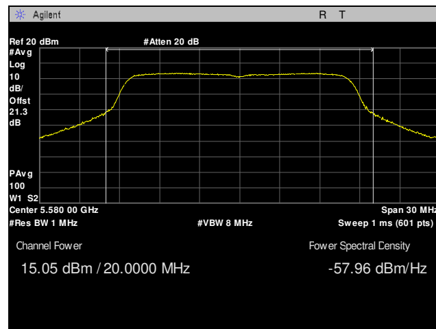
Plot 7. Maximum Conducted Output Power, Channel 116, 802.11a 20 MHz
