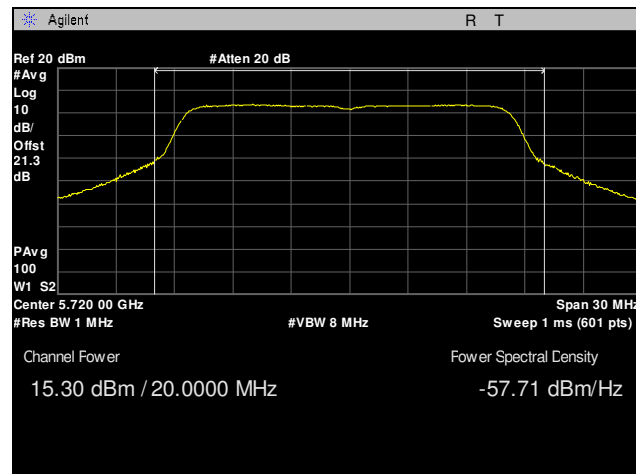
Plot 8. Maximum Conducted Output Power, Channel 144, 802.11a 20 MHz
