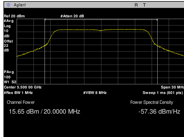
Plot 6. Maximum Conducted Output Power, Channel 100, 802.11a 20 MHz
