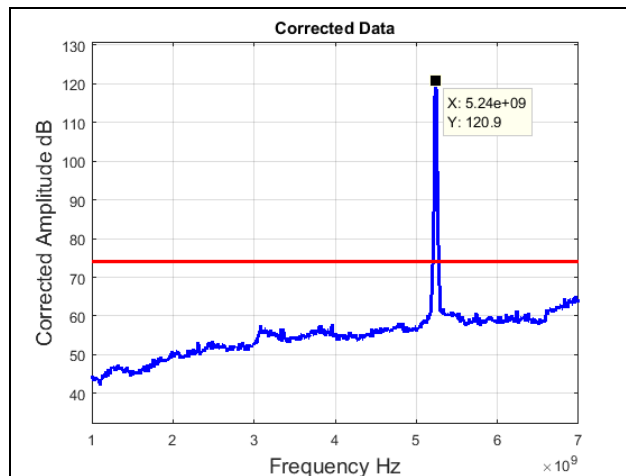
Plot 35. Radiated Spurious Emissions, High Channel, 802.11a 20 MHz, 1 GHz – 7 GHz, Peak
