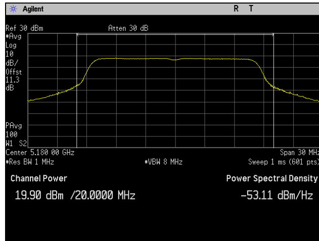
Plot 1. Conducted Output Power, Low Channel, 802.11a 20 MHz
