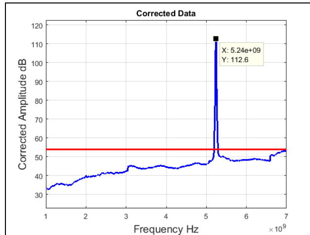
Plot 46. Radiated Spurious Emissions, High Channel, 802.11n 20 MHz, 1 GHz – 7 GHz, Average
