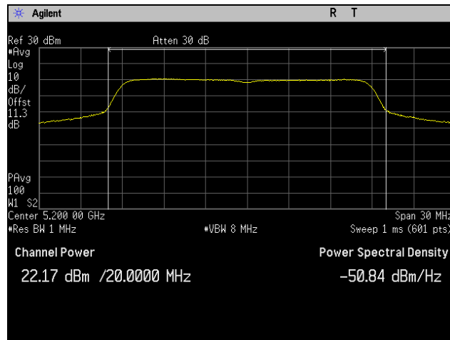
Plot 2. Conducted Output Power, Mid Channel, 802.11a 20 MHz
