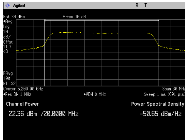
Plot 8. Conducted Output Power, Mid Channel, 802.11n 20 MHz
