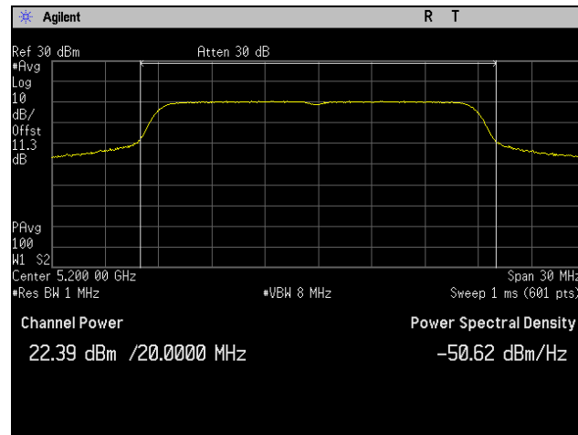
Plot 5. Conducted Output Power, Mid Channel, 802.11ac 20 MHz
