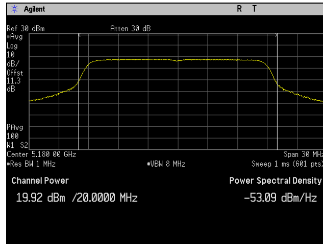
Plot 4. Conducted Output Power, Low Channel, 802.11ac 20 MHz
