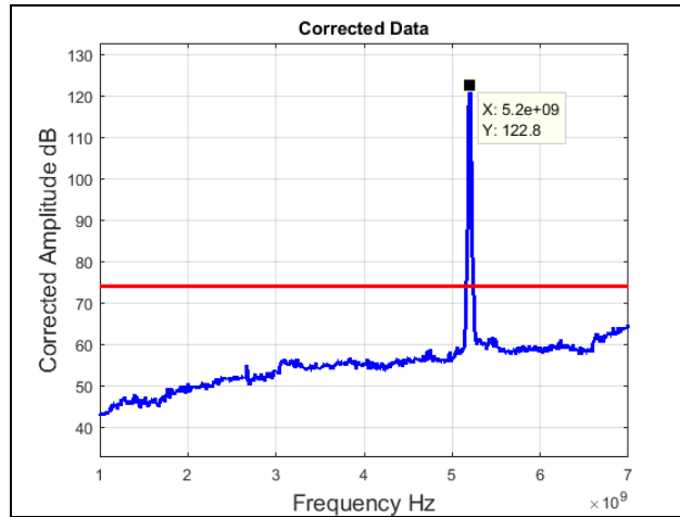
Plot 33. Radiated Spurious Emissions, Mid Channel, 802.11a 20 MHz, 1 GHz – 7 GHz, Peak
