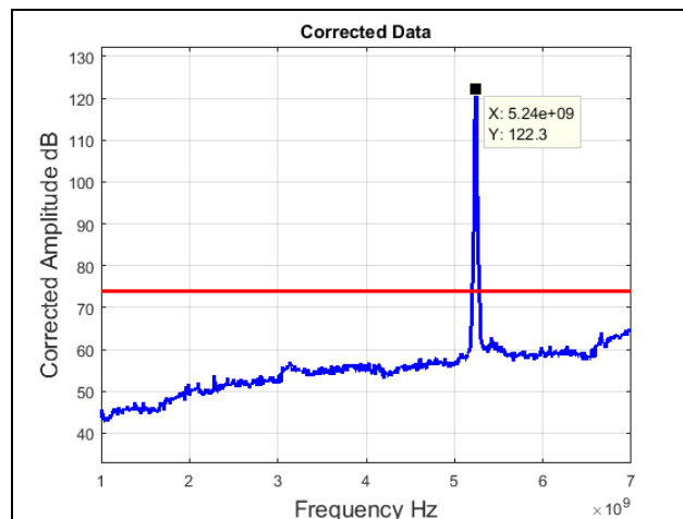
Plot 41. Radiated Spurious Emissions, High Channel, 802.11ac 20 MHz, 1 GHz – 7 GHz, Peak
