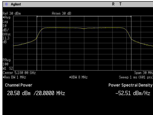
Plot 7. Conducted Output Power, Low Channel, 802.11n 20 MHz
