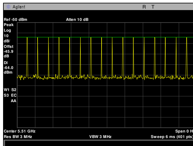
Plot 358. Radar Waveform Calibration, 5510 MHz, Type 3
