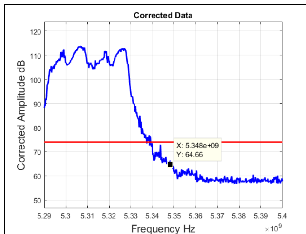
Plot 332. Radiated Band Edge, 5310 MHz, 802.11ac 40 MHz, Peak
