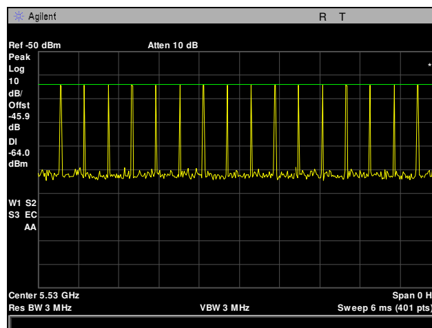
Plot 359. Radar Waveform Calibration, 5530 MHz, Type 3
