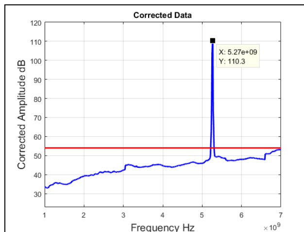
Plot 240. Radiated Spurious Emissions, 5260 MHz, 802.11ac 20 MHz, 1 GHz – 7 GHz, Average
