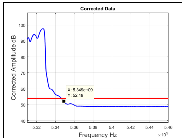
Plot 331. Radiated Band Edge, 5310 MHz, 802.11ac 40 MHz, Average
