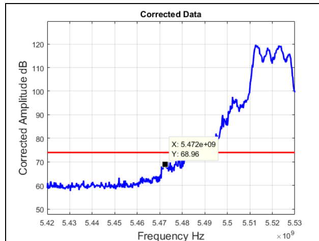
Plot 311. Radiated Band Edge, 5520 MHz, 802.11a 20 MHz, Peak
