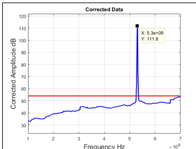
Plot 256. Radiated Spurious Emissions, 5300 MHz, 802.11n 20 MHz, 1 GHz – 7 GHz, Average
