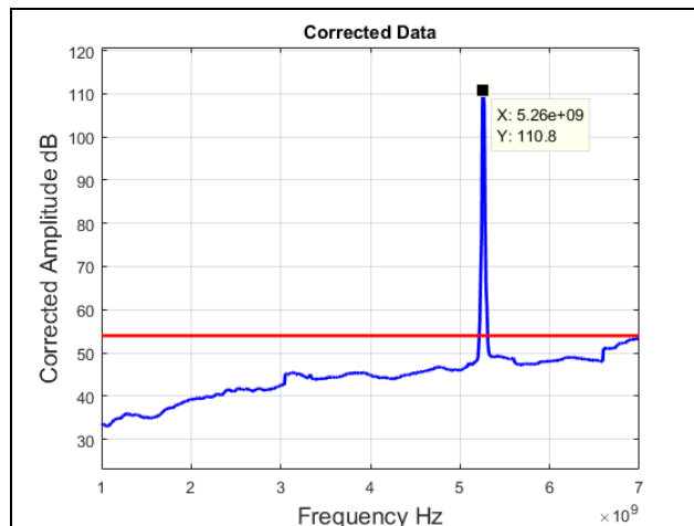
Plot 224. Radiated Spurious Emissions, 5260 MHz, 802.11a 20 MHz, 1 GHz – 7 GHz, Average
