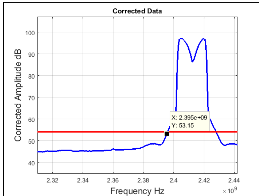
Plot 60. Radiated Restricted Band Edge, Low Channel, 802.11n 20 MHz, Average
