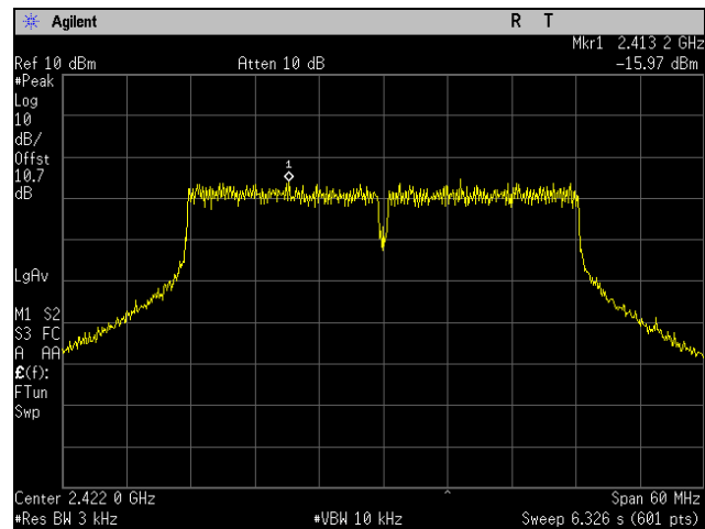
Plot 97. Peak Power Spectral Density, Low Channel, 802.11n 40 MHz, Port 1
