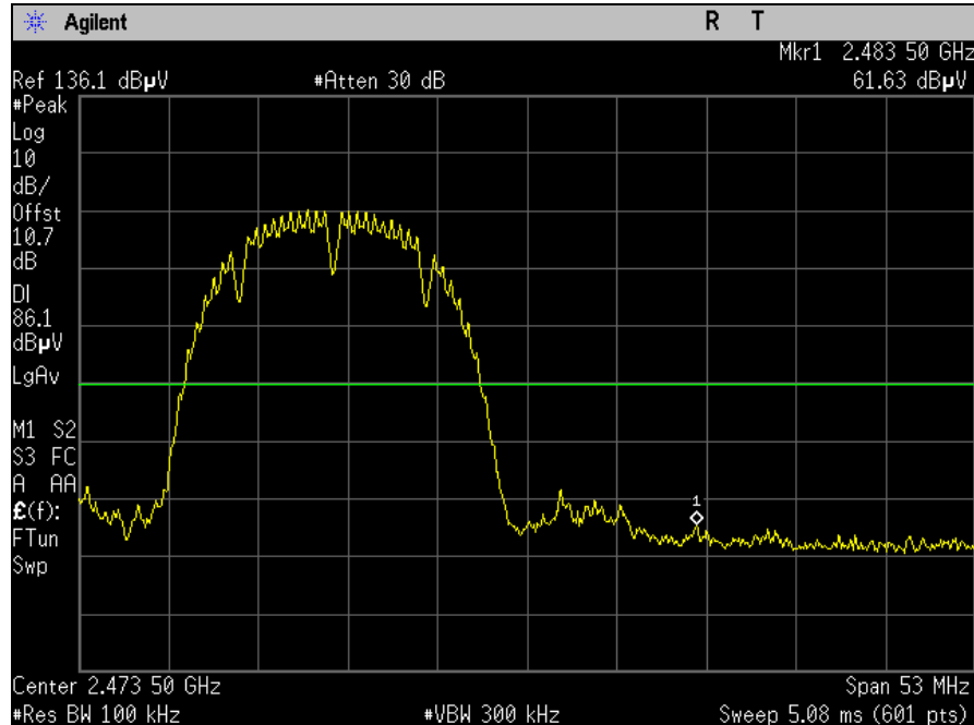
Plot 81. Conducted Band Edge, High Channel, 802.11b 20 MHz, 30 dBc
