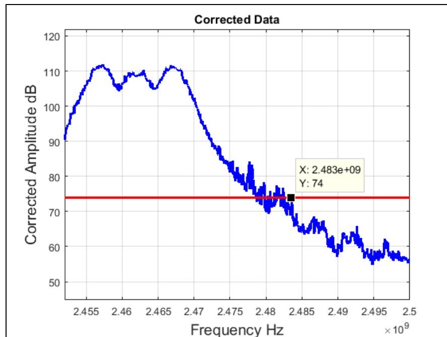
Plot 59. Radiated Restricted Band Edge, High Channel, 802.11g 20 MHz, Peak
