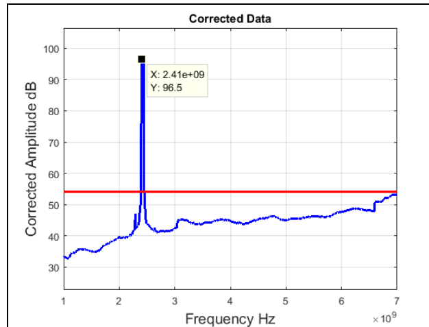
Plot 46. Radiated Spurious Emissions, Low Channel, 802.11n 40 MHz, 1 GHz – 7 GHz, Average
