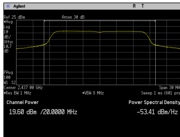
Plot 19. Peak Power Output, Mid Channel, 802.11g 20 MHz, Port 2
