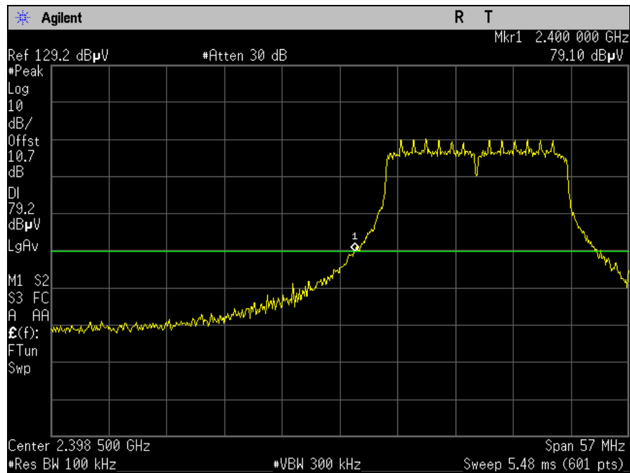
Plot 84. Conducted Band Edge, Low Channel, 802.11n 20 MHz, 30 dBc
