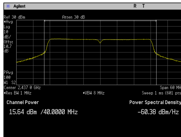
Plot 13. Peak Power Output, Mid Channel, 802.11n 40 MHz, Port 1
