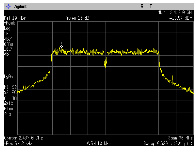
Plot 98. Peak Power Spectral Density, Mid Channel, 802.11n 40 MHz, Port 1
