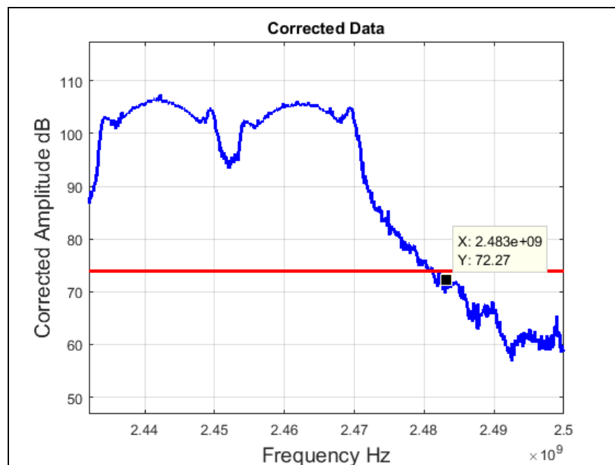
Plot 67. Radiated Restricted Band Edge, High Channel, 802.11n 40 MHz, Peak
