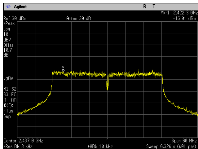
Plot 110. Peak Power Spectral Density, Mid Channel, 802.11n 40 MHz, Port 2
