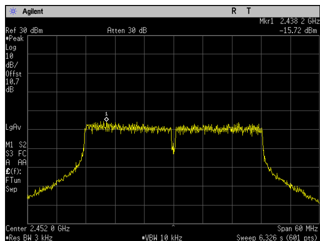
Plot 111. Peak Power Spectral Density, High Channel, 802.11n 40 MHz, Port 2
