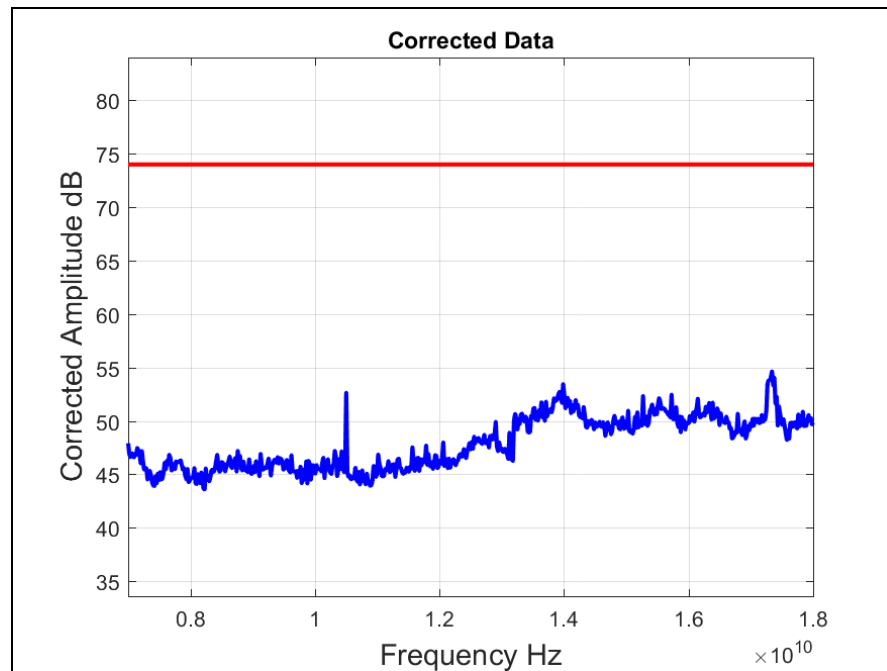
Plot. Radiated Spurious Emissions, Worst Case, 7 GHz – 18 GHz, Peak
