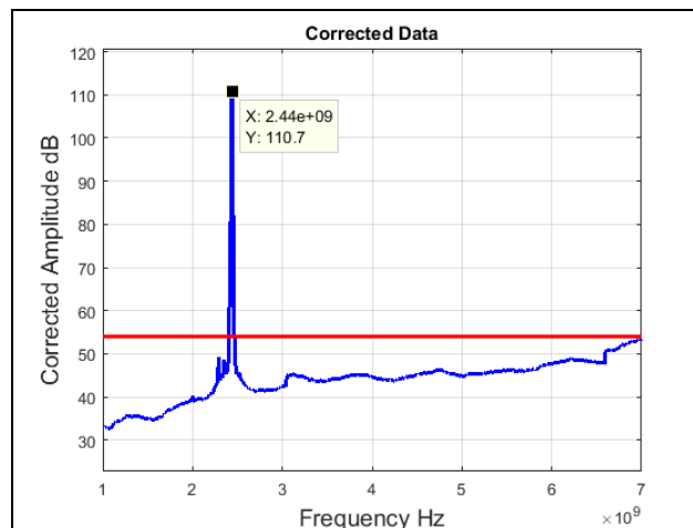
Plot 30. Radiated Spurious Emissions, Mid Channel, 802.11b 20 MHz, 1 GHz – 7 GHz, Average
