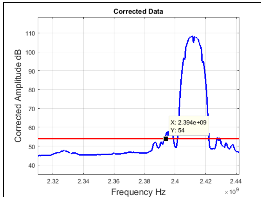
Plot 52. Radiated Restricted Band Edge, Low Channel, 802.11b 20 MHz, Average
