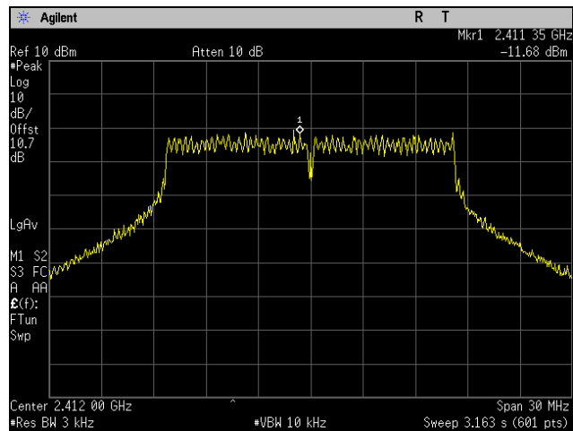
Plot 106. Peak Power Spectral Density, Low Channel, 802.11n 20 MHz, Port 2
