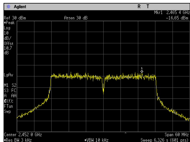
Plot 99. Peak Power Spectral Density, High Channel, 802.11n 40 MHz, Port 1
