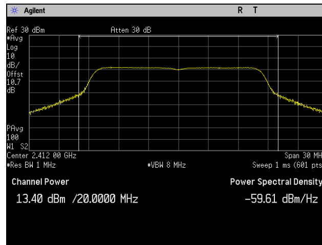
Plot 6. Peak Power Output, Low Channel, 802.11g 20 MHz, Port 1
