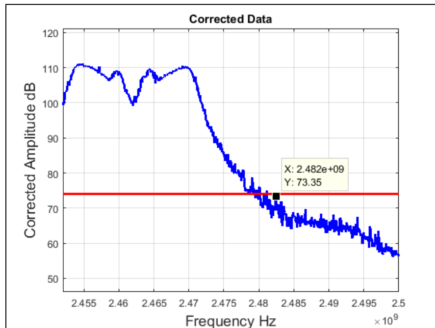
Plot 63. Radiated Restricted Band Edge, High Channel, 802.11n 20 MHz, Peak
