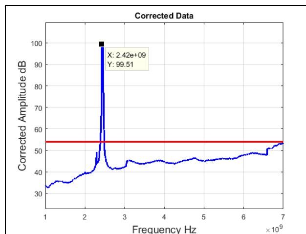
Plot 48. Radiated Spurious Emissions, Mid Channel, 802.11n 40 MHz, 1 GHz – 7 GHz, Average
