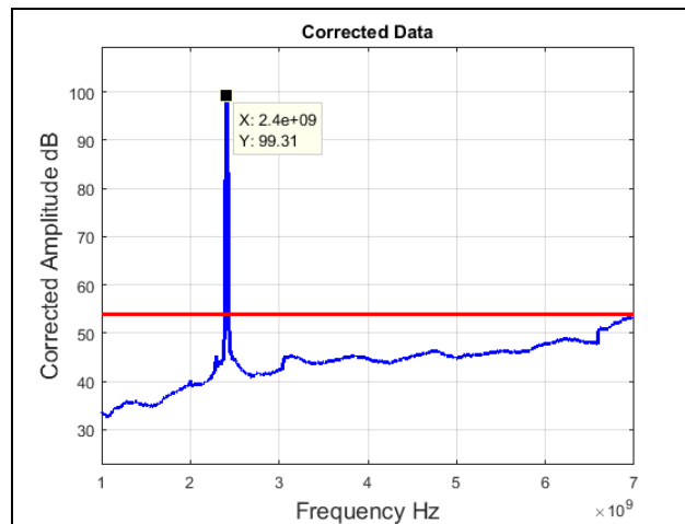
Plot 40. Radiated Spurious Emissions, Low Channel, 802.11n 20 MHz, 1 GHz – 7 GHz, Average
