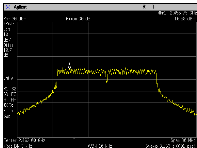
Plot 93. Peak Power Spectral Density, High Channel, 802.11g 20 MHz, Port 1
