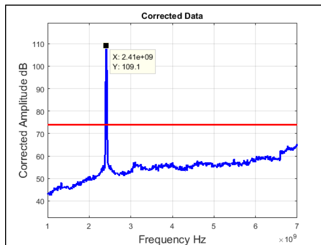
Plot 41. Radiated Spurious Emissions, Low Channel, 802.11n 20 MHz, 1 GHz – 7 GHz, Peak
