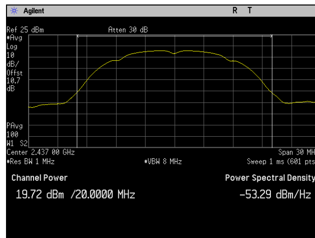
Plot 16. Peak Power Output, Mid Channel, 802.11b 20 MHz, Port 2
