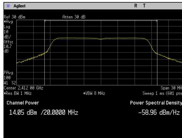
Plot 18. Peak Power Output, Low Channel, 802.11g 20 MHz, Port 2
