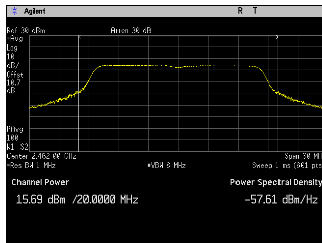
Plot 20. Peak Power Output, High Channel, 802.11g 20 MHz, Port 2
