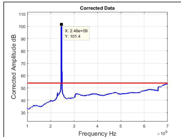
Plot 44. Radiated Spurious Emissions, High Channel, 802.11n 20 MHz, 1 GHz – 7 GHz, Average
