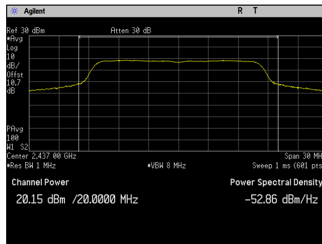
Plot 7. Peak Power Output, Mid Channel, 802.11g 20 MHz, Port 1
