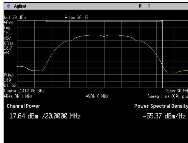
Plot 15. Peak Power Output, Low Channel, 802.11b 20 MHz, Port 2
