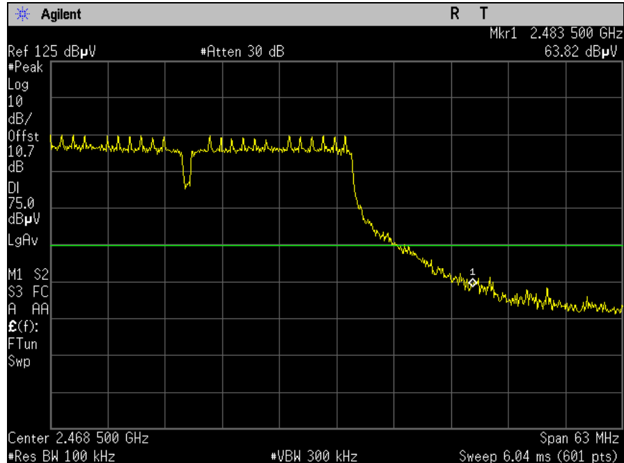
Plot 87. Conducted Band Edge, High Channel, 802.11n 40 MHz, 30 dBc
