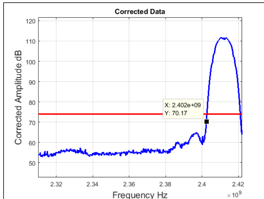
Plot 53. Radiated Restricted Band Edge, Low Channel, 802.11b 20 MHz, Peak
