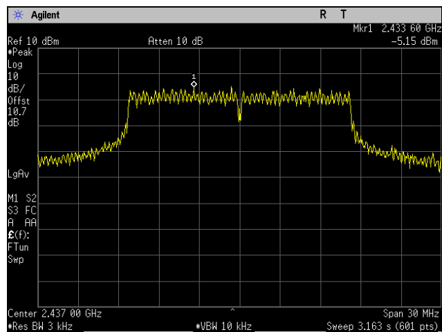
Plot 95. Peak Power Spectral Density, Mid Channel, 802.11n 20 MHz, Port 1
