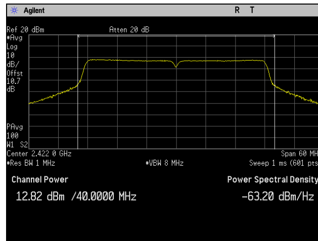
Plot 12. Peak Power Output, Low Channel, 802.11n 40 MHz, Port 1
