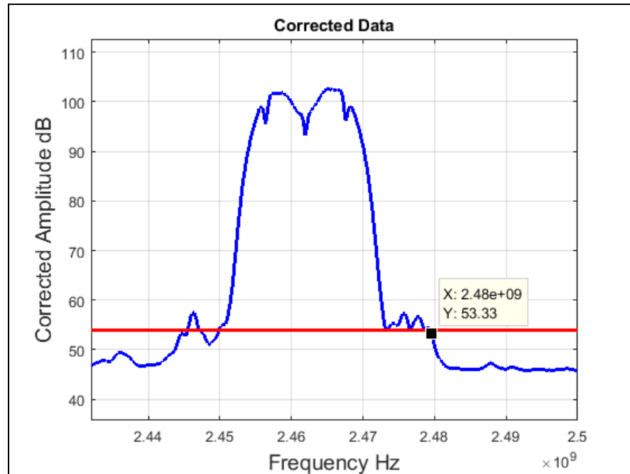
Plot 54. Radiated Restricted Band Edge, High Channel, 802.11b 20 MHz, Average
