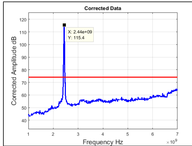
Plot 37. Radiated Spurious Emissions, Mid Channel, 802.11g 20 MHz, 1 GHz – 7 GHz, Peak
