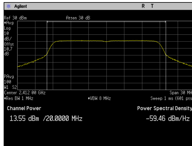
Plot 9. Peak Power Output, Low Channel, 802.11n 20 MHz, Port 1
