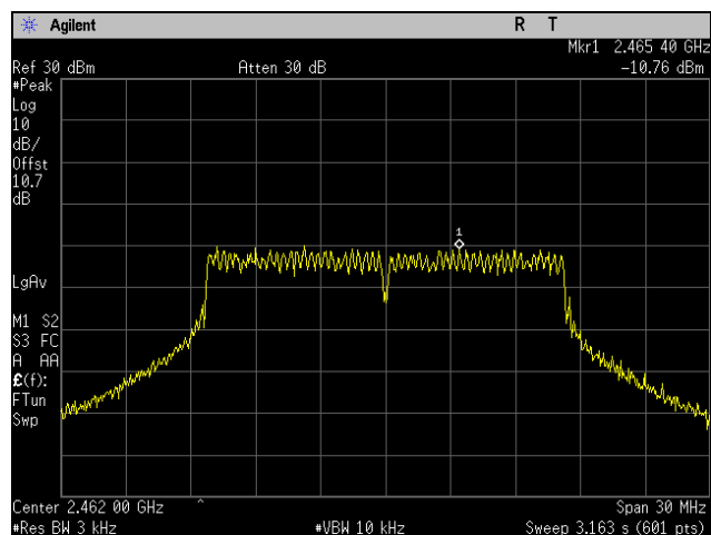
Plot 96. Peak Power Spectral Density, High Channel, 802.11n 20 MHz, Port 1
