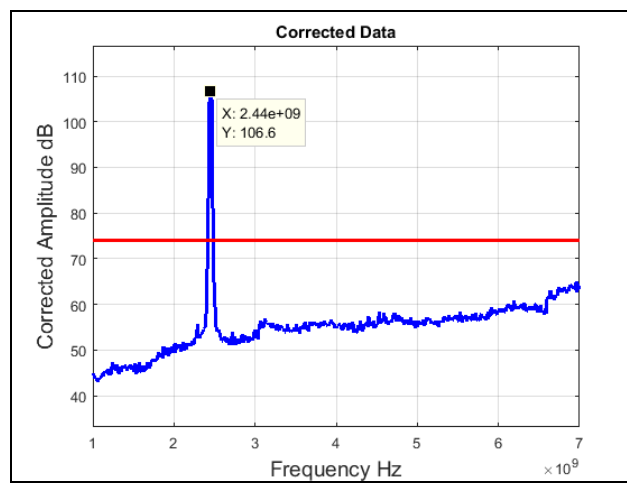
Plot 51. Radiated Spurious Emissions, High Channel, 802.11n 40 MHz, 1 GHz – 7 GHz, Peak
