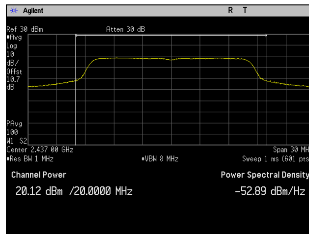
Plot 10. Peak Power Output, Mid Channel, 802.11n 20 MHz, Port 1
