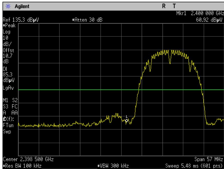
Plot 80. Conducted Band Edge, Low Channel, 802.11b 20 MHz, 30 dBc
