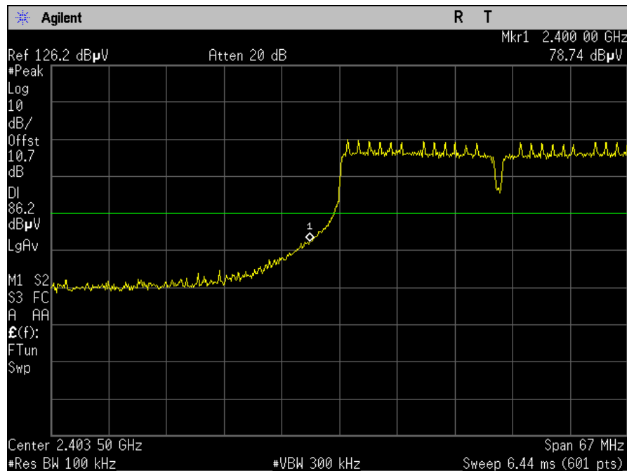
Plot 86. Conducted Band Edge, Low Channel, 802.11n 40 MHz, 30 dBc
