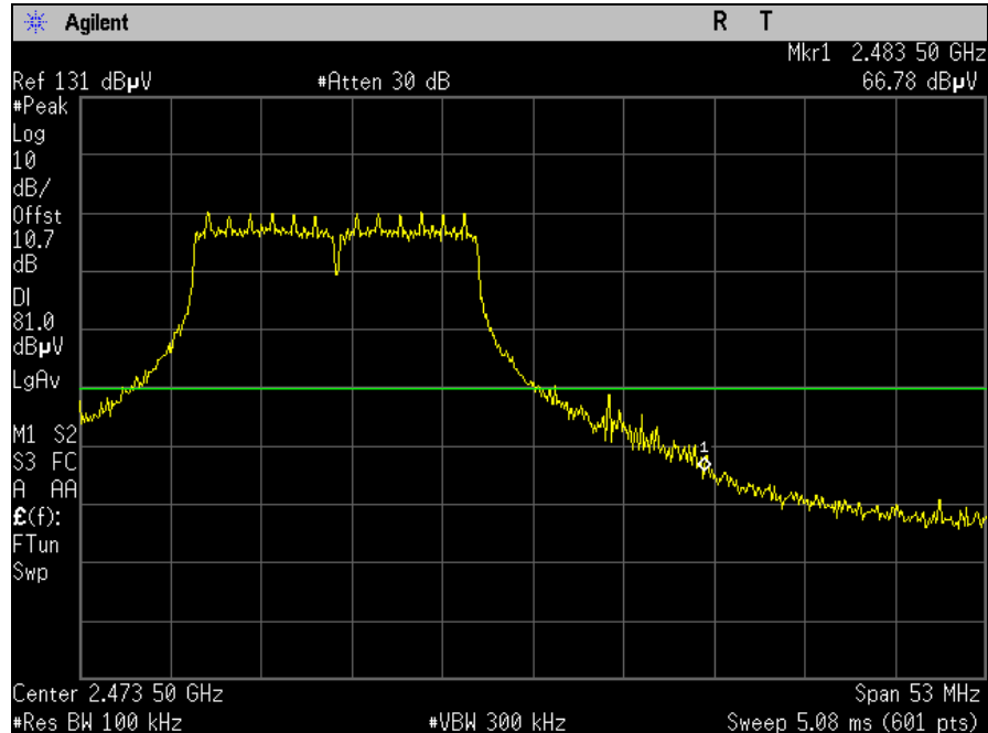
Plot 83. Conducted Band Edge, High Channel, 802.11g 20 MHz, 30 dBc
