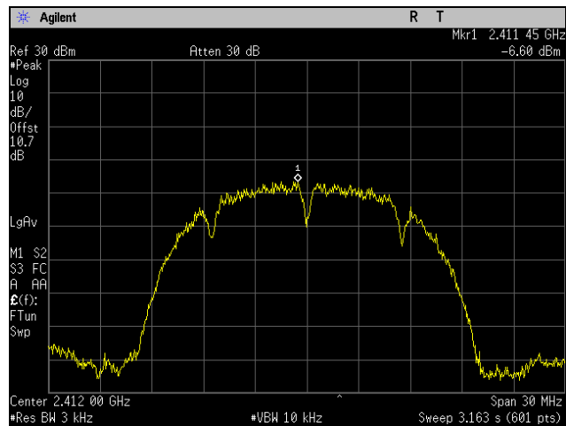
Plot 88. Peak Power Spectral Density, Low Channel, 802.11b 20 MHz, Port 1
