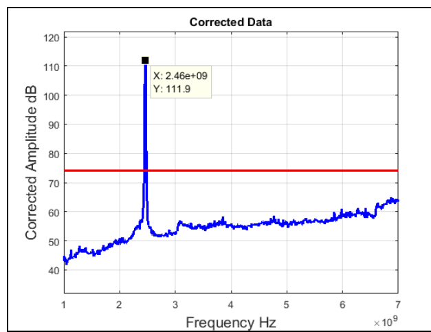
Plot 39. Radiated Spurious Emissions, High Channel, 802.11g 20 MHz, 1 GHz – 7 GHz, Peak
