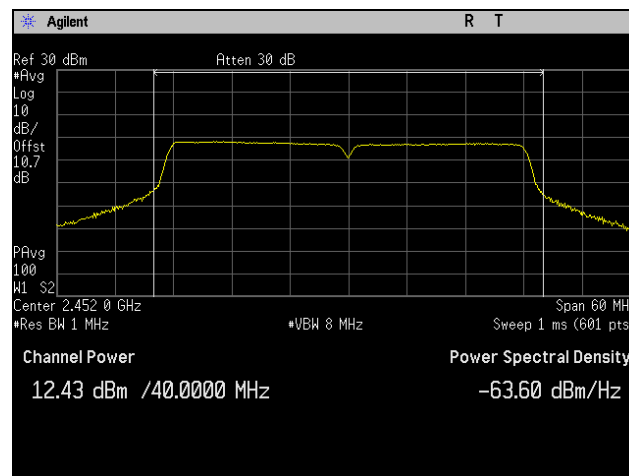
Plot 26. Peak Power Output, High Channel, 802.11n 40 MHz, Port 2
