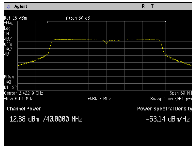
Plot 24. Peak Power Output, Low Channel, 802.11n 40 MHz, Port 2
