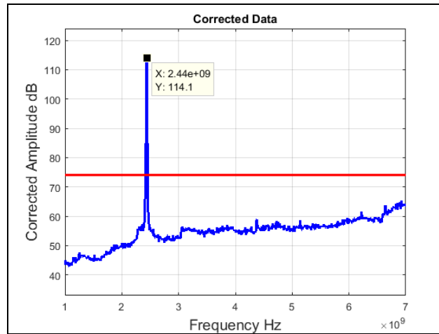
Plot 31. Radiated Spurious Emissions, Mid Channel, 802.11b 20 MHz, 1 GHz – 7 GHz, Peak
