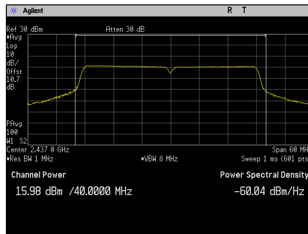
Plot 25. Peak Power Output, Mid Channel, 802.11n 40 MHz, Port 2
