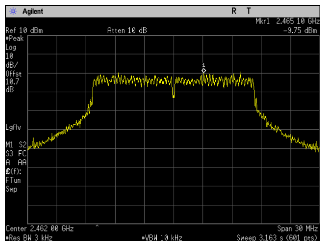
Plot 105. Peak Power Spectral Density, High Channel, 802.11g 20 MHz, Port 2
