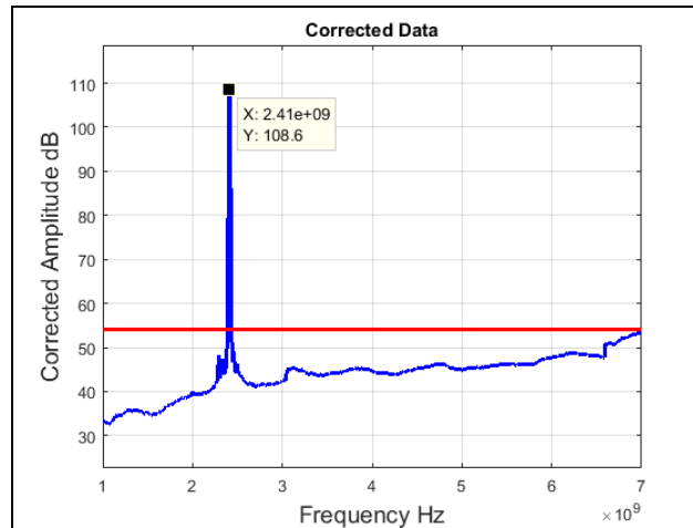
Plot 28. Radiated Spurious Emissions, Low Channel, 802.11b 20 MHz, 1 GHz – 7 GHz, Average
