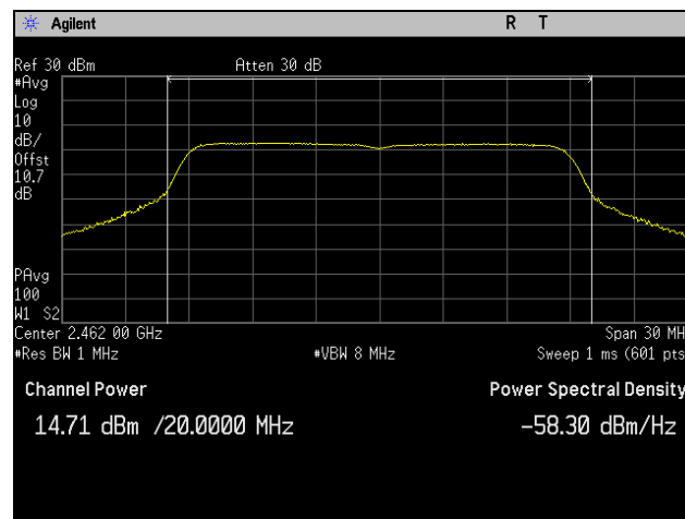
Plot 23. Peak Power Output, High Channel, 802.11n 20 MHz, Port 2
