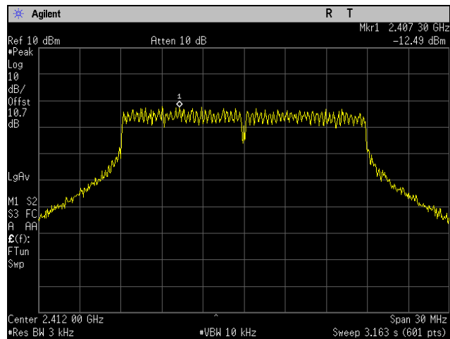
Plot 94. Peak Power Spectral Density, Low Channel, 802.11n 20 MHz, Port 1
