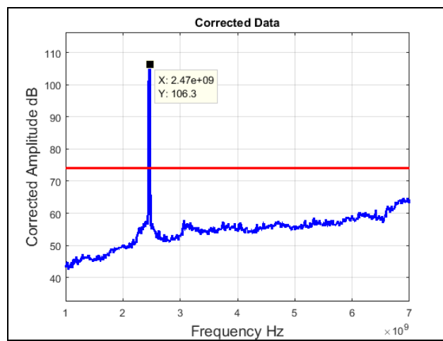
Plot 33. Radiated Spurious Emissions, High Channel, 802.11b 20 MHz, 1 GHz – 7 GHz, Peak
