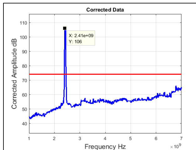
Plot 47. Radiated Spurious Emissions, Low Channel, 802.11n 40 MHz, 1 GHz – 7 GHz, Peak
