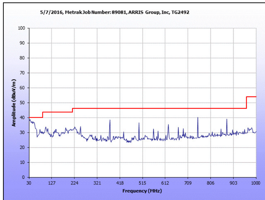
Plot 27. Radiated Spurious Emissions, 30 MHz – 1 GHz, Worst Case Mode
