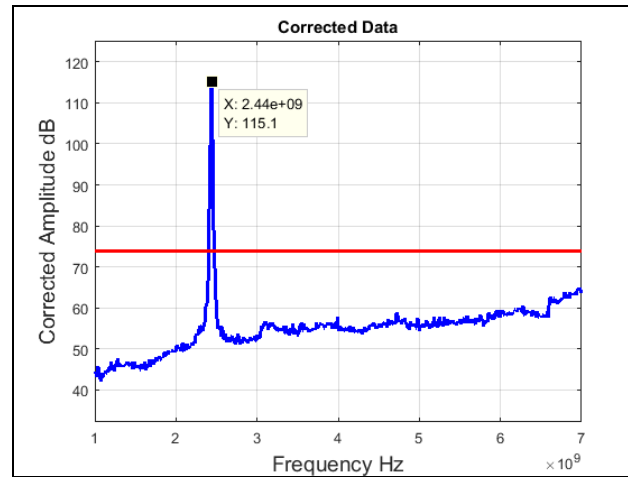
Plot 43. Radiated Spurious Emissions, Mid Channel, 802.11n 20 MHz, 1 GHz – 7 GHz, Peak
