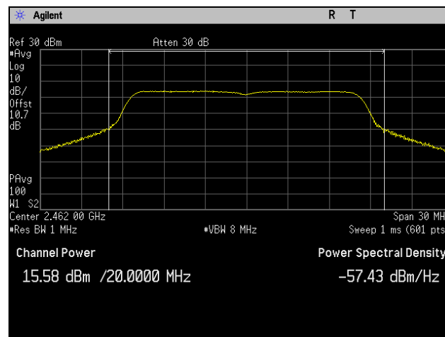
Plot 11. Peak Power Output, High Channel, 802.11n 20 MHz, Port 1
