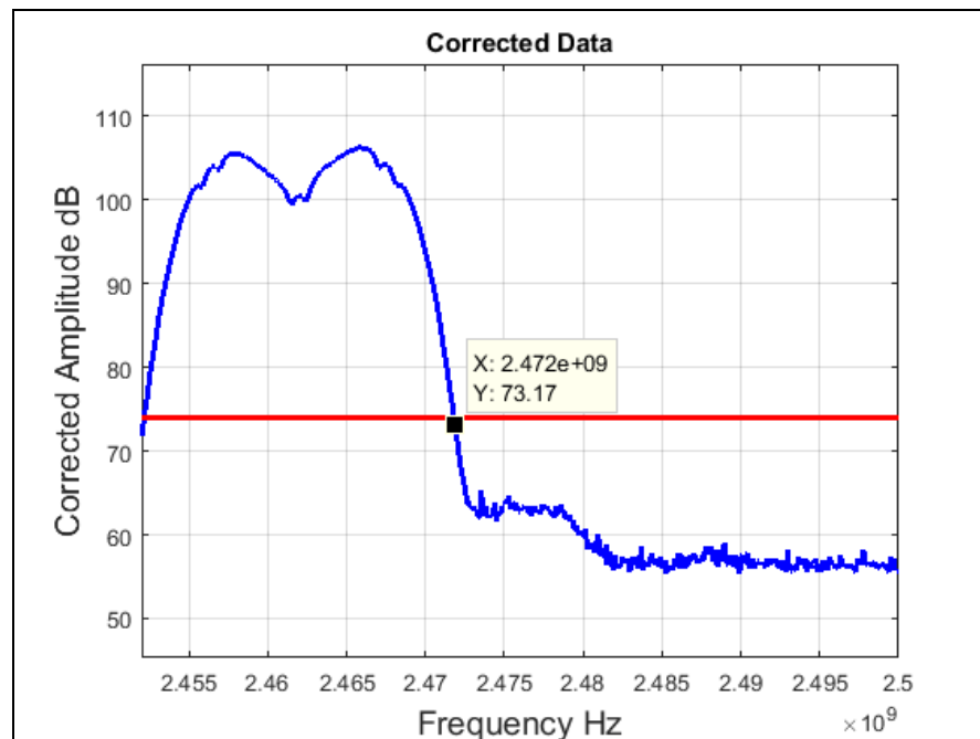
Plot 55. Radiated Restricted Band Edge, High Channel, 802.11b 20 MHz, Peak
