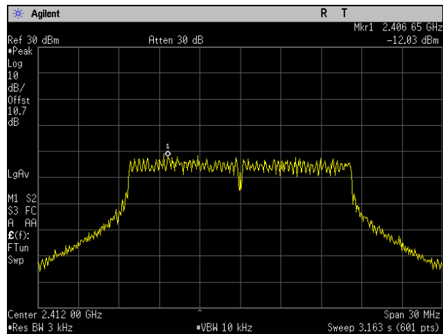
Plot 103. Peak Power Spectral Density, Low Channel, 802.11g 20 MHz, Port 2
