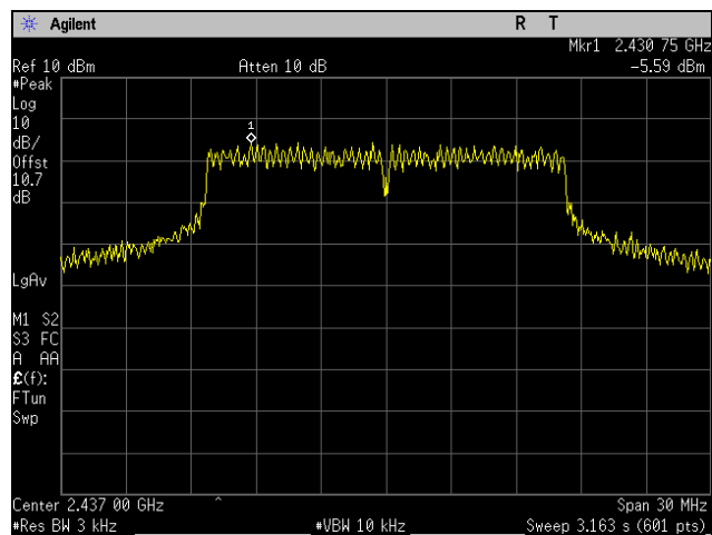
Plot 92. Peak Power Spectral Density, Mid Channel, 802.11g 20 MHz, Port 1
