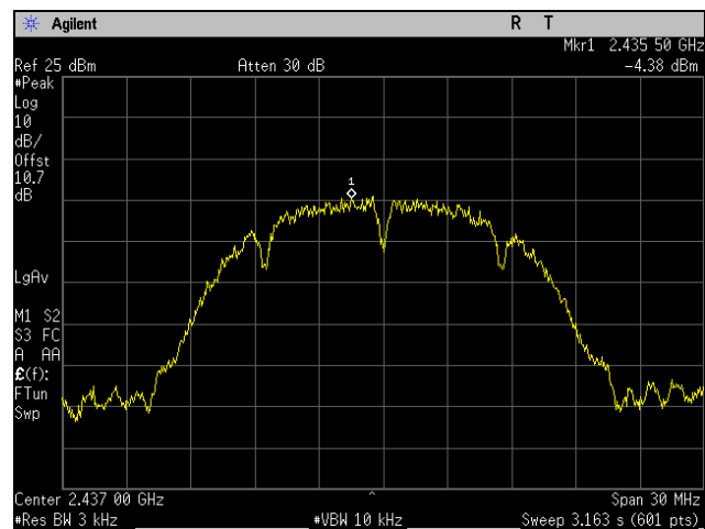
Plot 101. Peak Power Spectral Density, Mid Channel, 802.11b 20 MHz, Port 2
