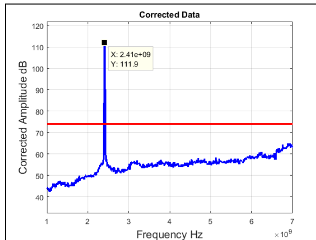
Plot 29. Radiated Spurious Emissions, Low Channel, 802.11b 20 MHz, 1 GHz – 7 GHz, Peak
