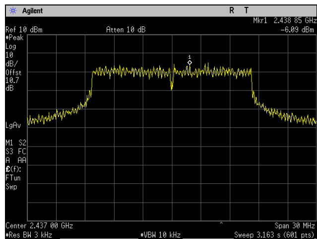
Plot 104. Peak Power Spectral Density, Mid Channel, 802.11g 20 MHz, Port 2
