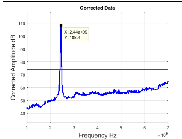
Plot 49. Radiated Spurious Emissions, Mid Channel, 802.11n 40 MHz, 1 GHz – 7 GHz, Peak
