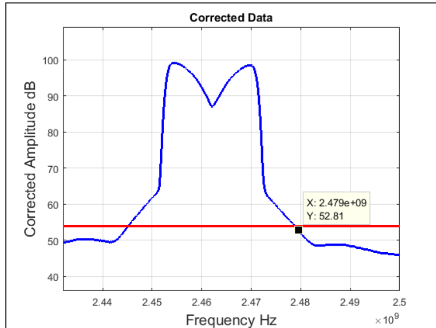
Plot 62. Radiated Restricted Band Edge, High Channel, 802.11n 20 MHz, Average
