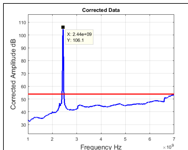
Plot 42. Radiated Spurious Emissions, Mid Channel, 802.11n 20 MHz, 1 GHz – 7 GHz, Average
