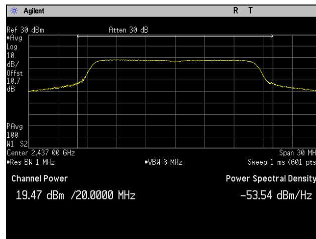
Plot 22. Peak Power Output, Mid Channel, 802.11n 20 MHz, Port 2
