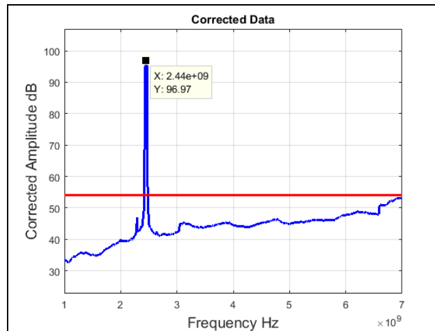
Plot 50. Radiated Spurious Emissions, High Channel, 802.11n 40 MHz, 1 GHz – 7 GHz, Average
