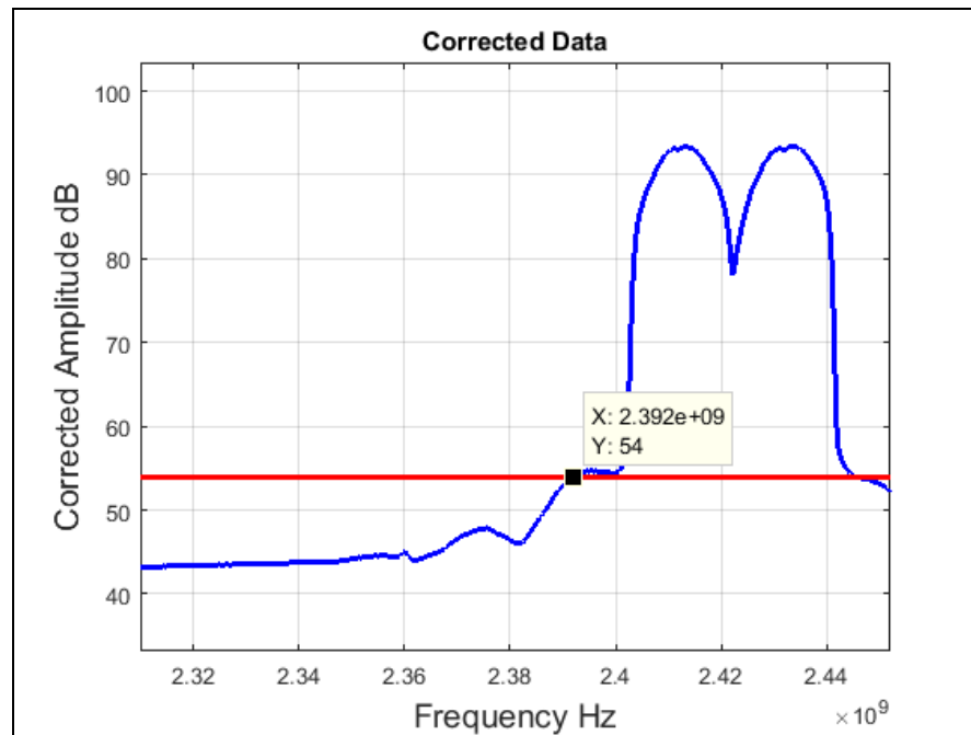
Plot 64. Radiated Restricted Band Edge, Low Channel, 802.11n 40 MHz, Average
