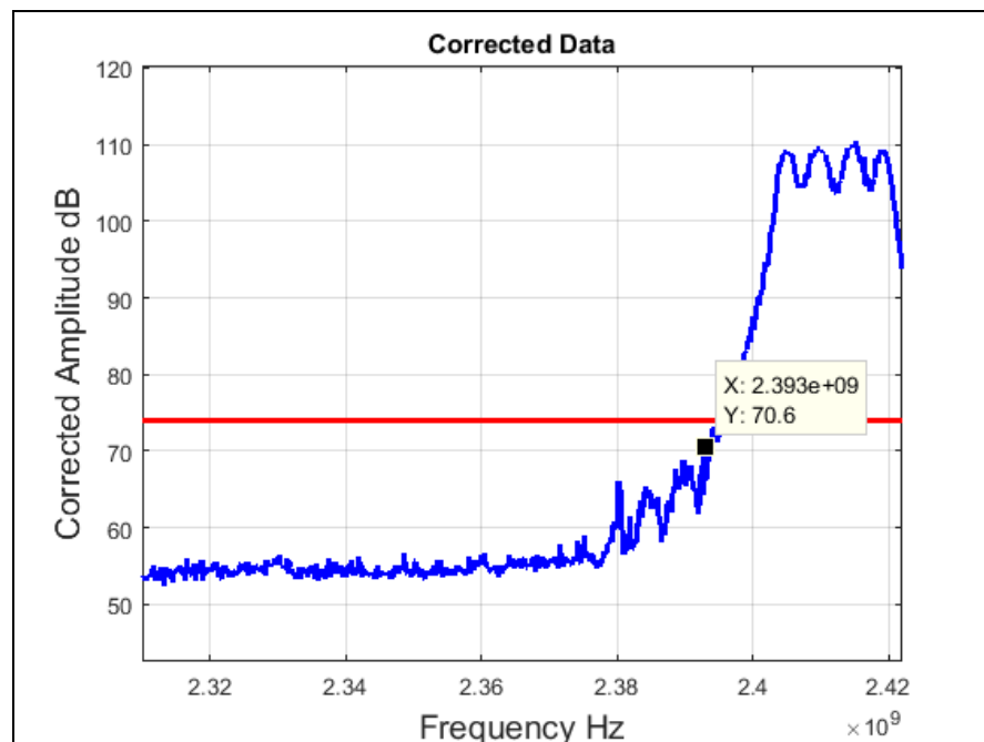
Plot 61. Radiated Restricted Band Edge, Low Channel, 802.11n 20 MHz, Peak
