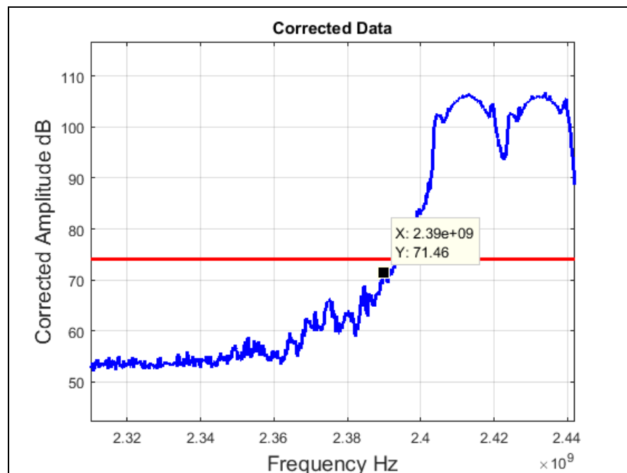
Plot 65. Radiated Restricted Band Edge, Low Channel, 802.11n 40 MHz, Peak
