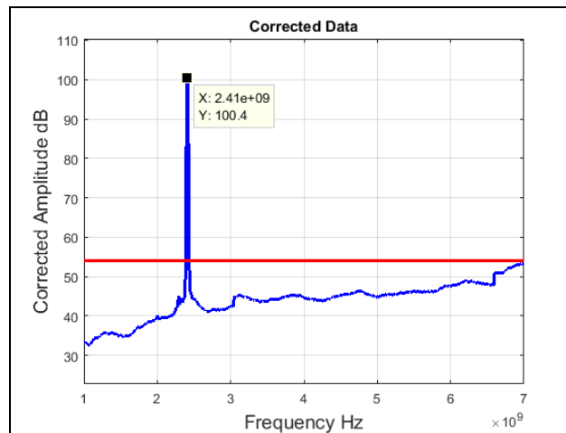
Plot 34. Radiated Spurious Emissions, Low Channel, 802.11g 20 MHz, 1 GHz – 7 GHz, Average
