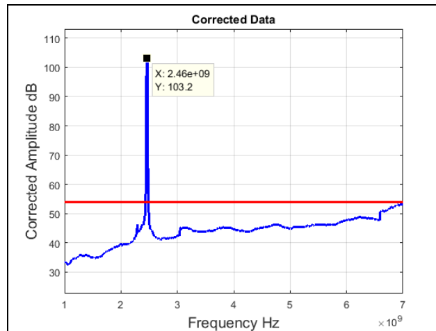
Plot 38. Radiated Spurious Emissions, High Channel, 802.11g 20 MHz, 1 GHz – 7 GHz, Average
