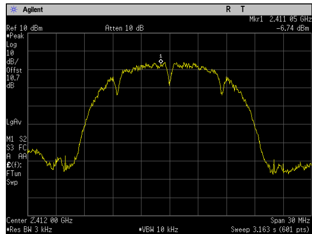
Plot 100. Peak Power Spectral Density, Low Channel, 802.11b 20 MHz, Port 2
