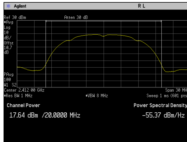
Plot 3. Peak Power Output, Low Channel, 802.11b 20 MHz, Port 1
