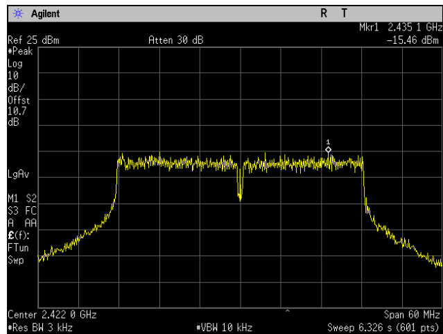
Plot 109. Peak Power Spectral Density, Low Channel, 802.11n 40 MHz, Port 2
