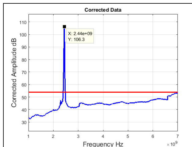
Plot 36. Radiated Spurious Emissions, Mid Channel, 802.11g 20 MHz, 1 GHz – 7 GHz, Average
