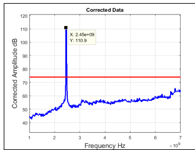
Plot 45. Radiated Spurious Emissions, High Channel, 802.11n 20 MHz, 1 GHz – 7 GHz, Peak
