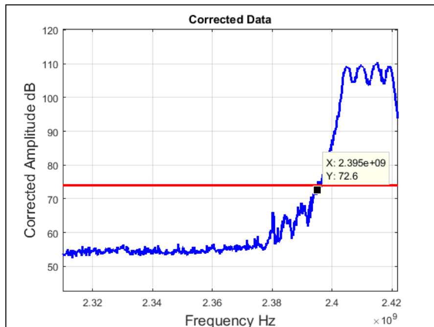
Plot 57. Radiated Restricted Band Edge, Low Channel, 802.11g 20 MHz, Peak
