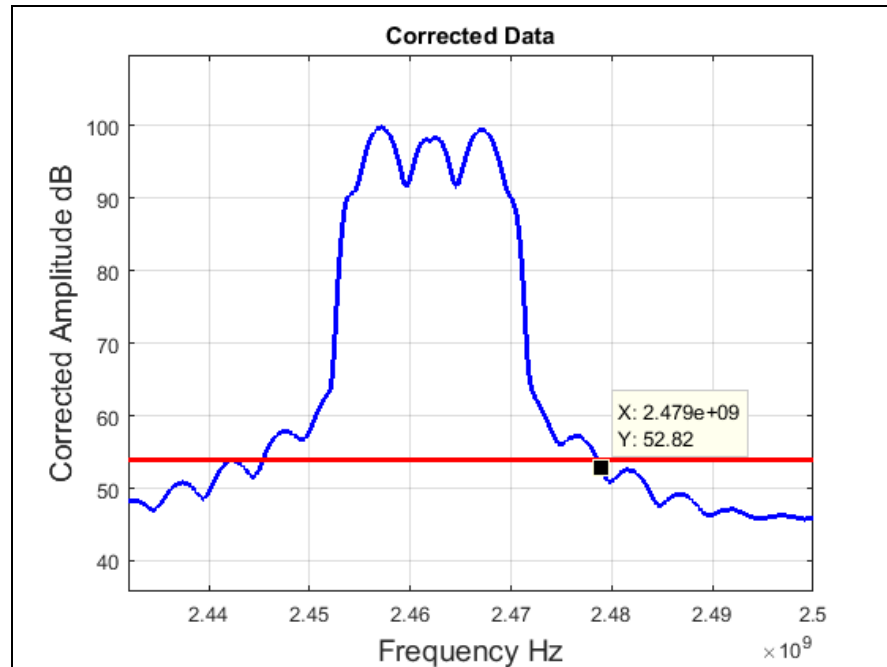
Plot 58. Radiated Restricted Band Edge, High Channel, 802.11g 20 MHz, Average
