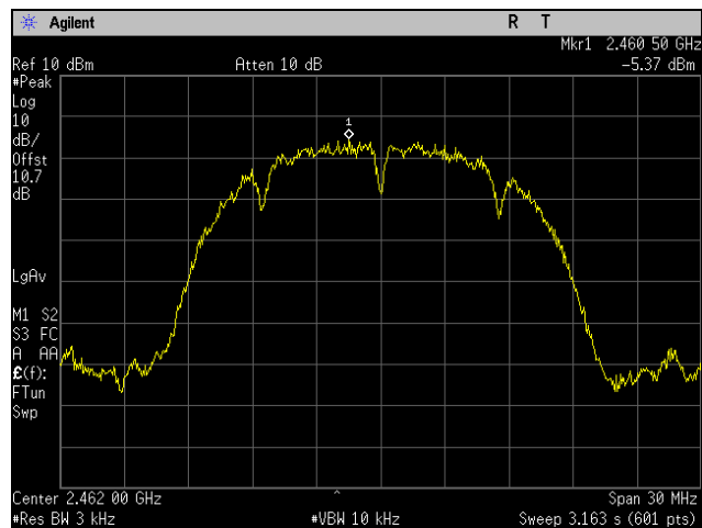
Plot 90. Peak Power Spectral Density, High Channel, 802.11b 20 MHz, Port 1
