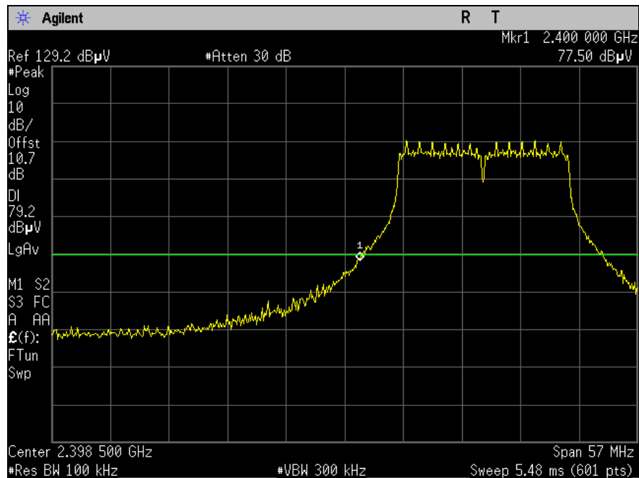
Plot 82. Conducted Band Edge, Low Channel, 802.11g 20 MHz, 30 dBc
