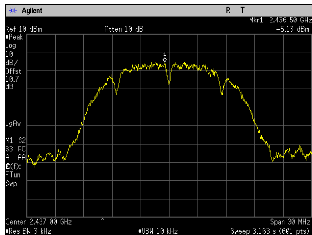
Plot 89. Peak Power Spectral Density, Mid Channel, 802.11b 20 MHz, Port 1
