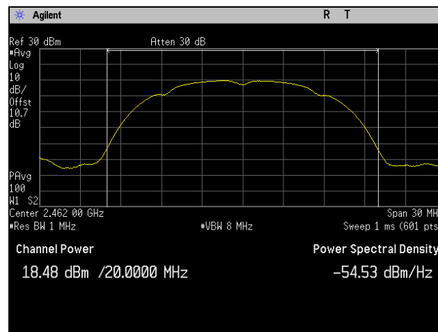
Plot 17. Peak Power Output, High Channel, 802.11b 20 MHz, Port 2
