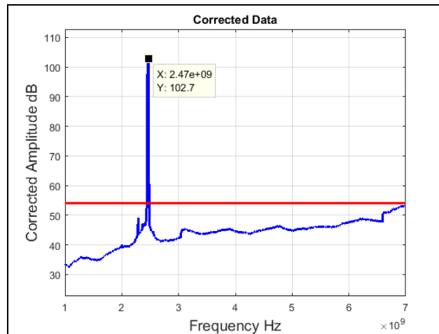
Plot 32. Radiated Spurious Emissions, High Channel, 802.11b 20 MHz, 1 GHz – 7 GHz, Average
