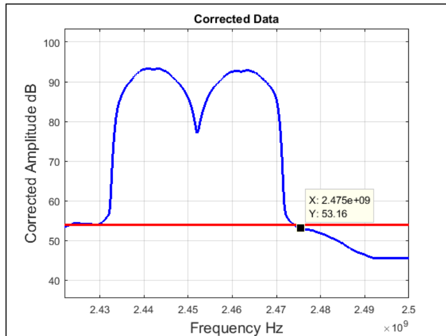
Plot 66. Radiated Restricted Band Edge, High Channel, 802.11n 40 MHz, Average
