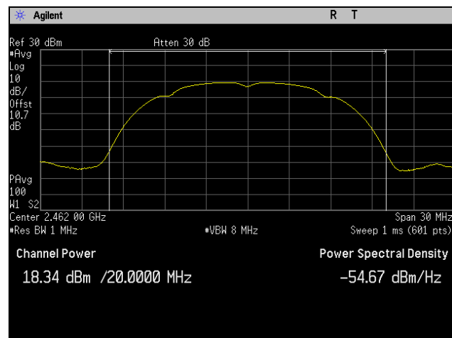
Plot 5. Peak Power Output, High Channel, 802.11b 20 MHz, Port 1
