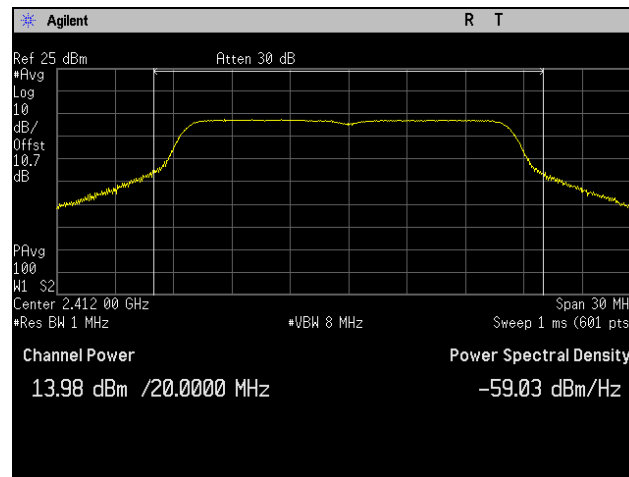
Plot 21. Peak Power Output, Low Channel, 802.11n 20 MHz, Port 2
