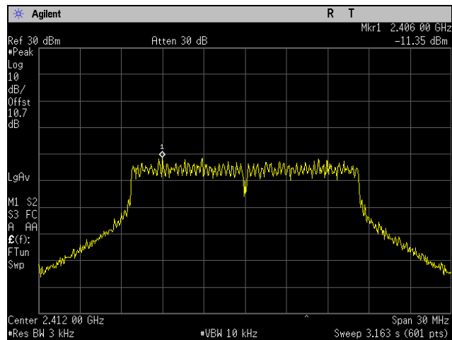
Plot 91. Peak Power Spectral Density, Low Channel, 802.11g 20 MHz, Port 1
