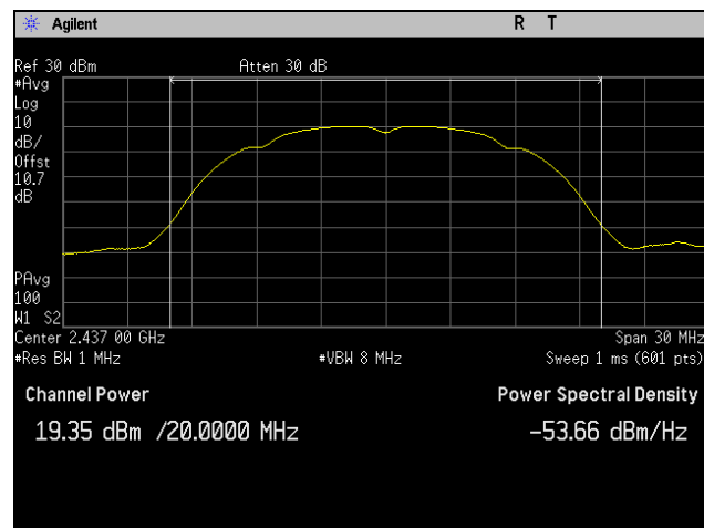
Plot 4. Peak Power Output, Mid Channel, 802.11b 20 MHz, Port 1
