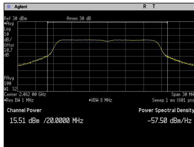
Plot 8. Peak Power Output, High Channel, 802.11g 20 MHz, Port 1
