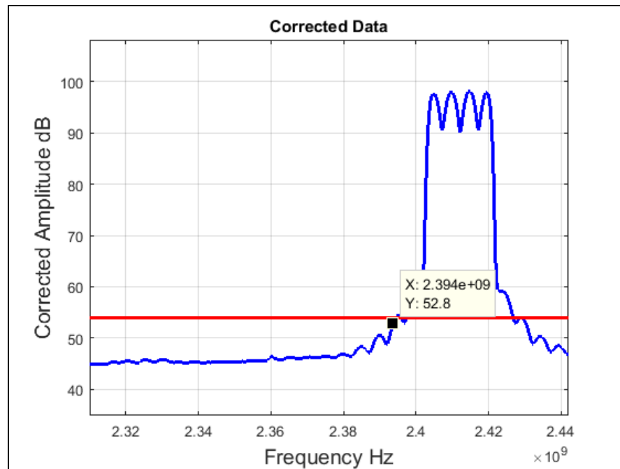
Plot 56. Radiated Restricted Band Edge, Low Channel, 802.11g 20 MHz, Average
