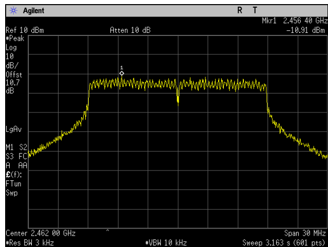
Plot 108. Peak Power Spectral Density, High Channel, 802.11n 20 MHz, Port 2
