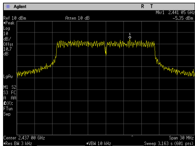
Plot 107. Peak Power Spectral Density, Mid Channel, 802.11n 20 MHz, Port 2
