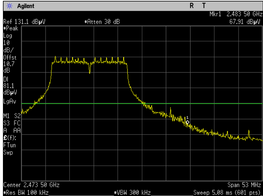
Plot 85. Conducted Band Edge, High Channel, 802.11n 20 MHz, 30 dBc
