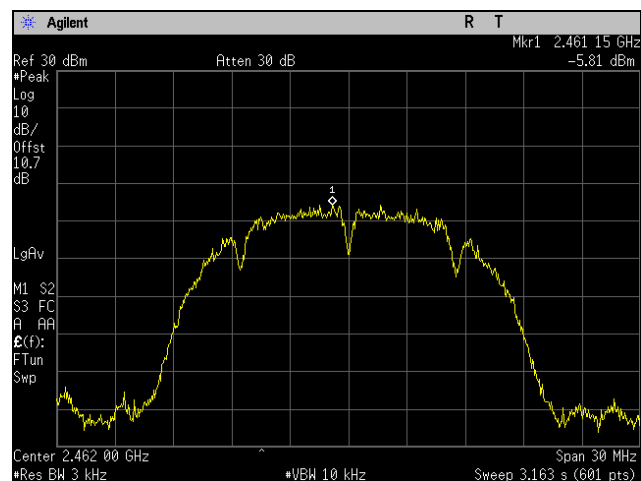
Plot 102. Peak Power Spectral Density, High Channel, 802.11b 20 MHz, Port 2
