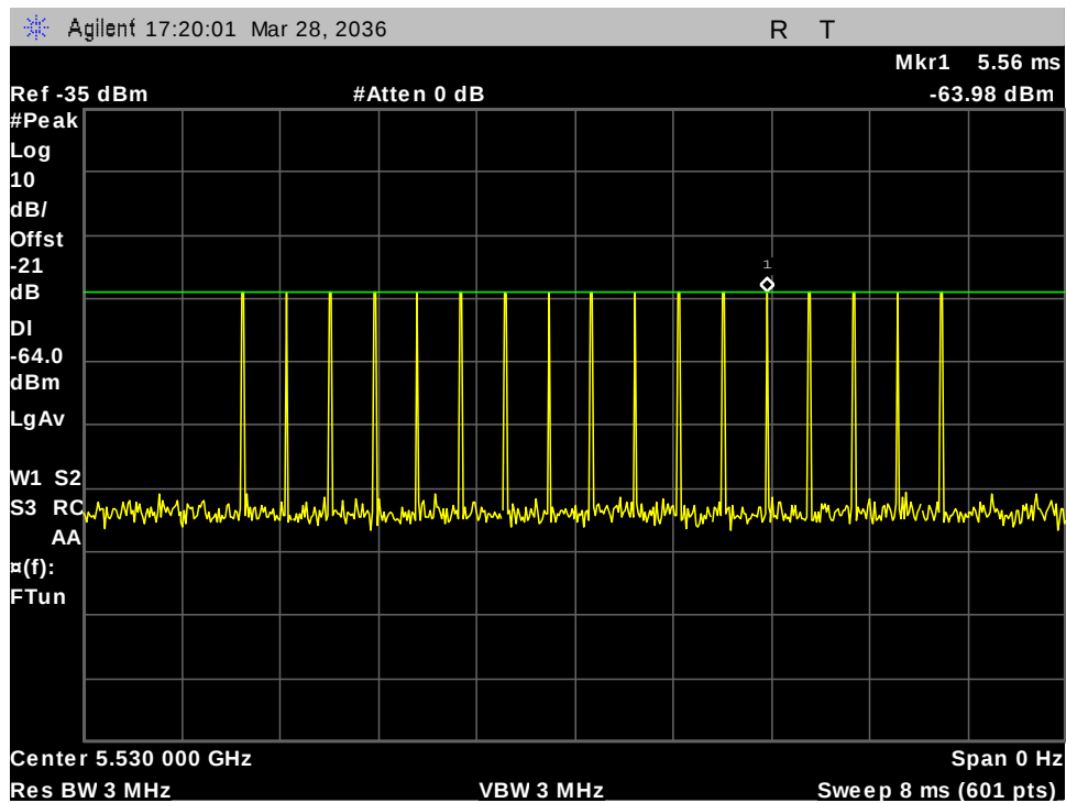
Figure 31: 5530MHz 80M Type -3 Calibration
