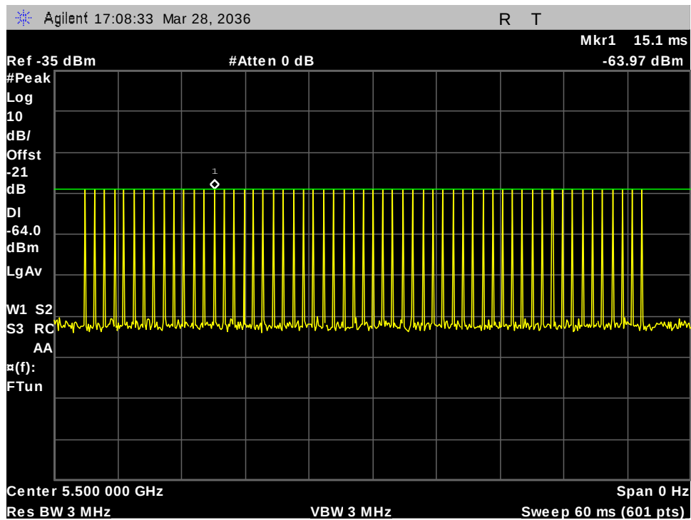
Figure 15: 5500MHz 20M Type -1 Calibration
