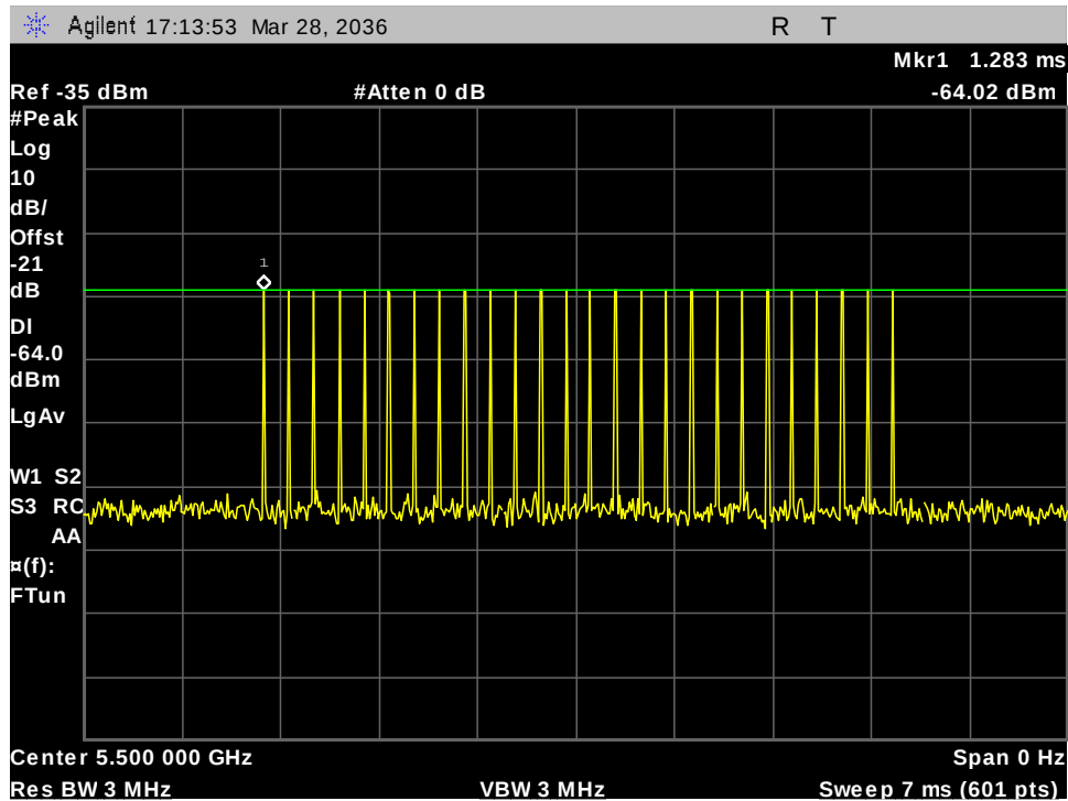
Figure 16: 5500MHz 20M Type -2 Calibration
