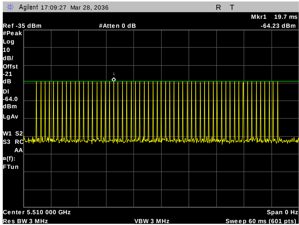
Figure 22: 5510MHz 40M Type -1 Calibration
