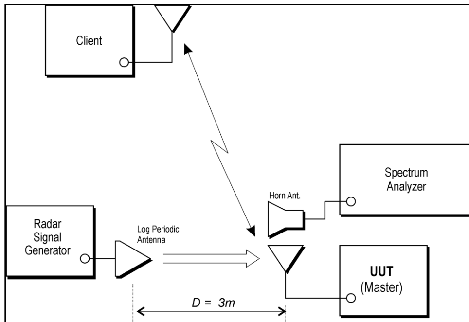
Figure 35: Test Setup Diagram
