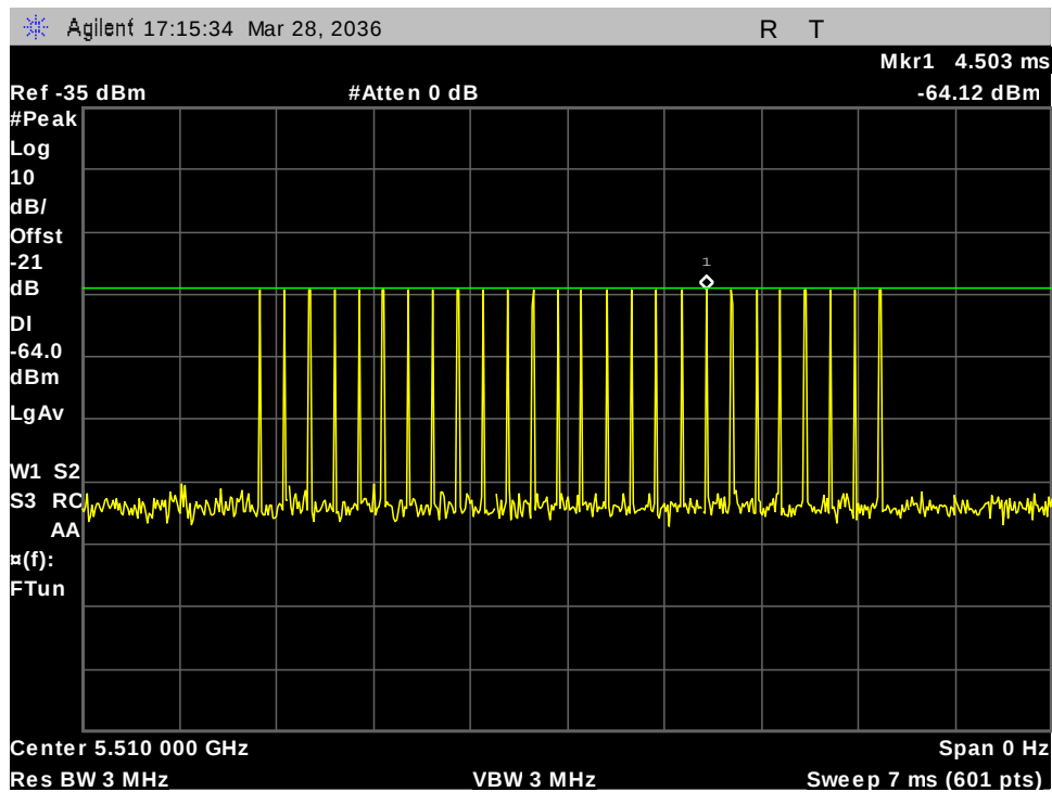
Figure 23: 5510MHz 40M Type -2 Calibration
