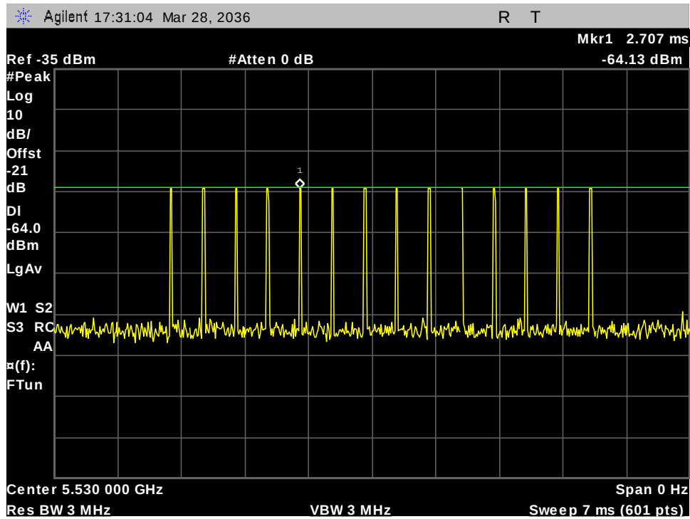
Figure 32: 5530MHz 80M Type -4 Calibration
