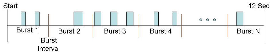
Figure 11: Long Pulse Radar Test Signal Waveform
