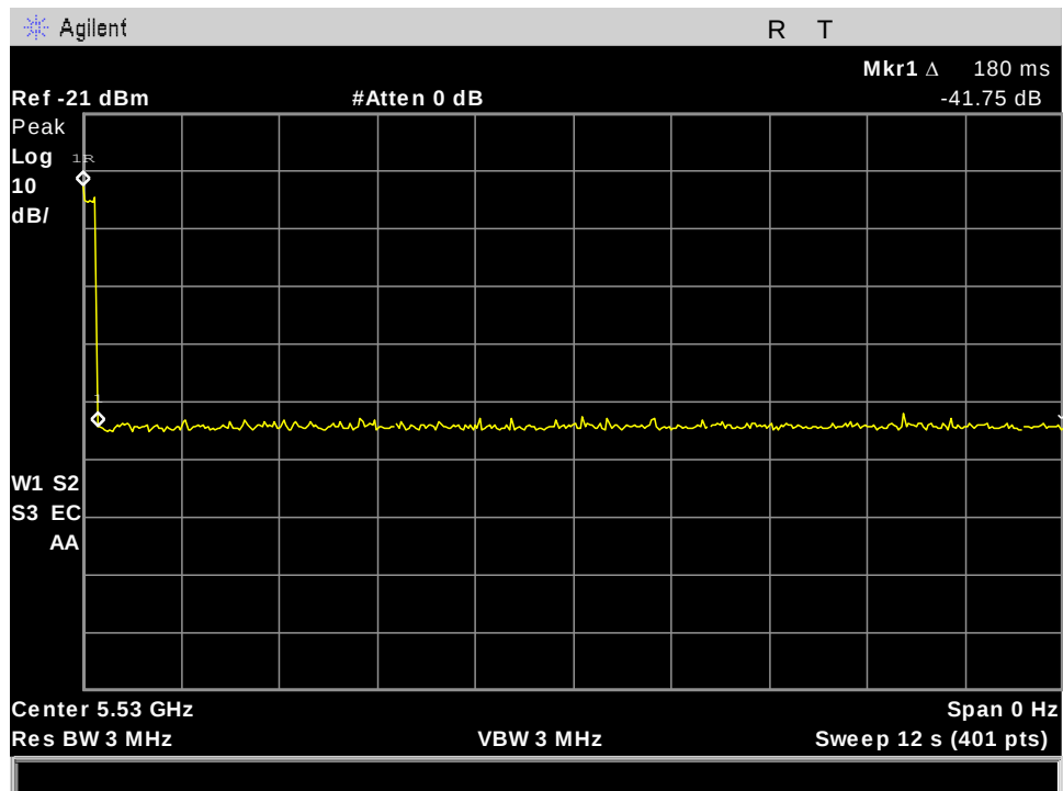
Figure 40: 5530 MHz channel move time
