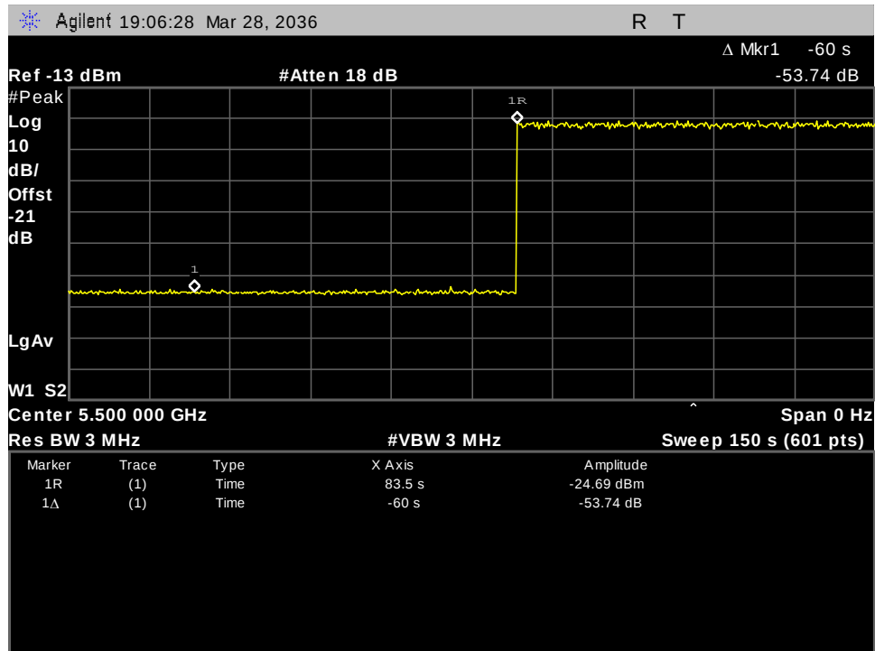
Figure 36: 5500 MHz Channel Availability Check
