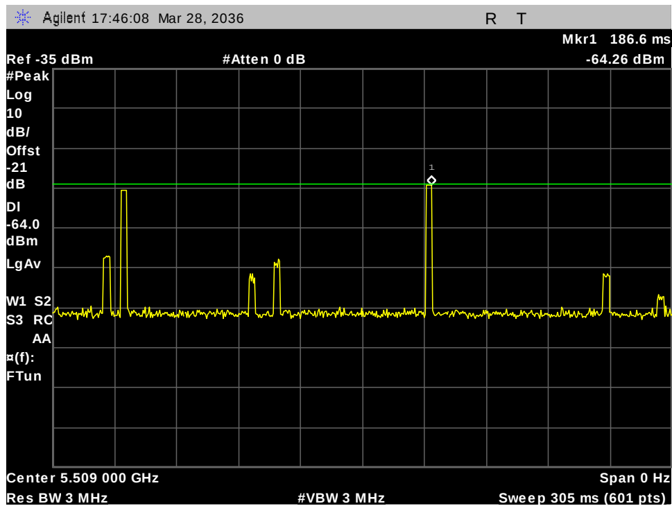
Figure 27: 5510MHz 40M Type -6 hop at 5509MHz Calibration
