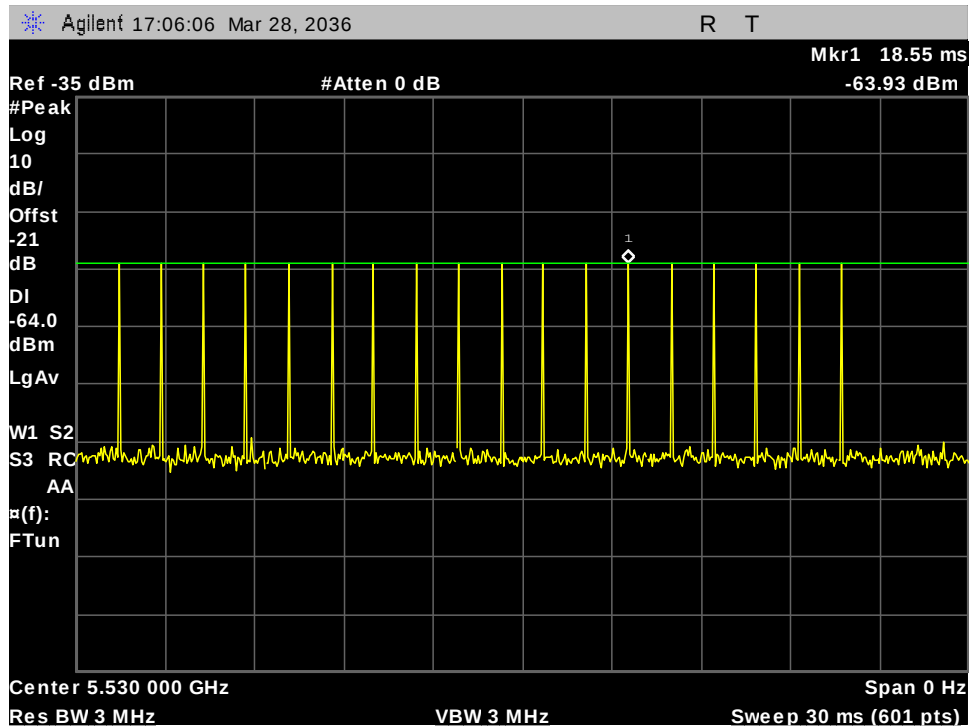
Figure 28: 5530MHz 80M Type -0 Calibration
