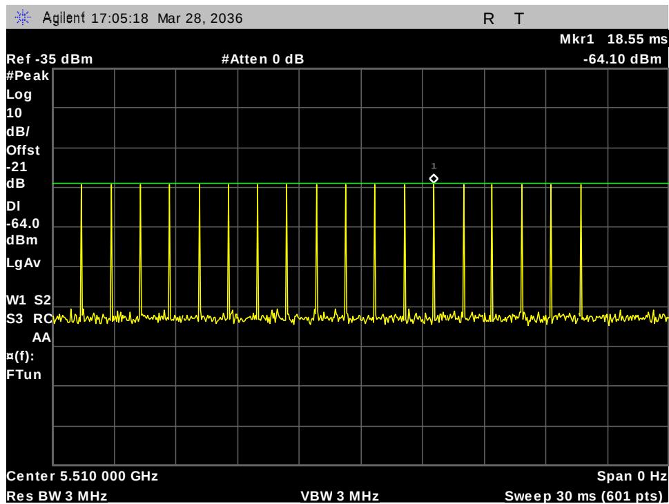
Figure 21: 5510MHz 40M Type -0 Calibration
