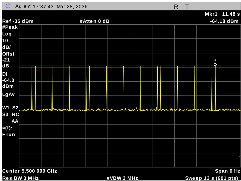
Figure 19: 5500MHz 20M Type -5 Calibration
