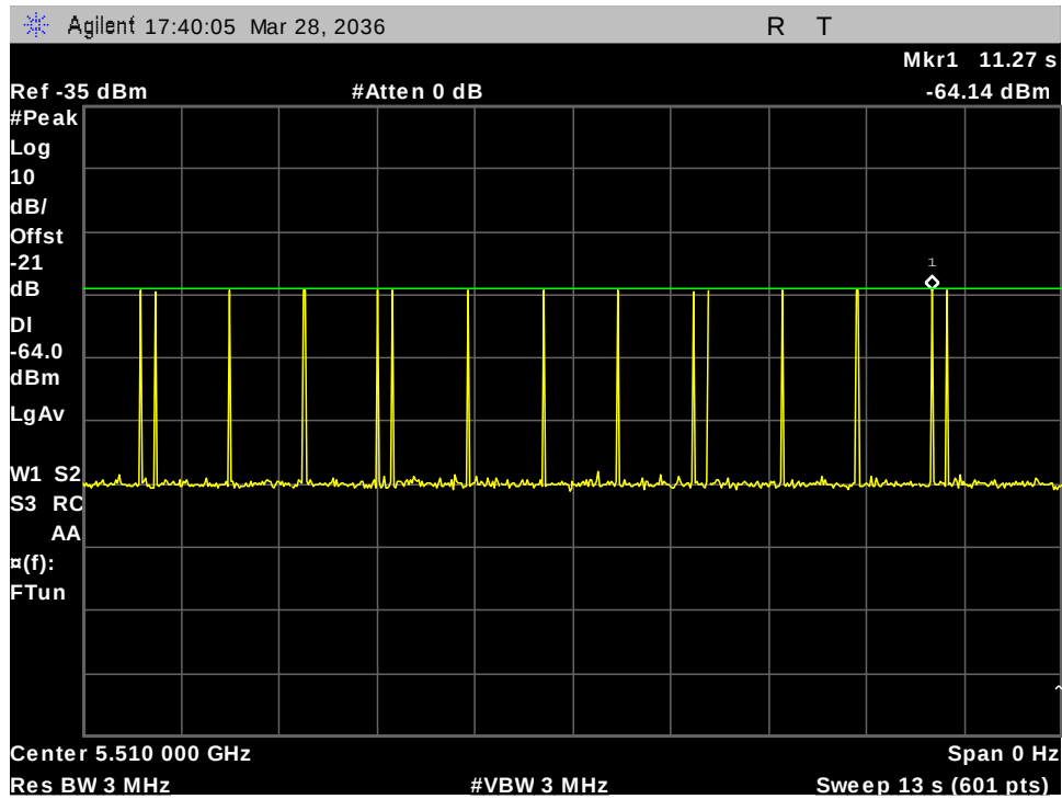
Figure 26: 5510MHz 40M Type -5 Calibration
