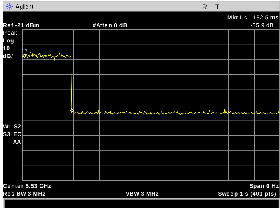
Figure 39: 5530 MHz channel close time
