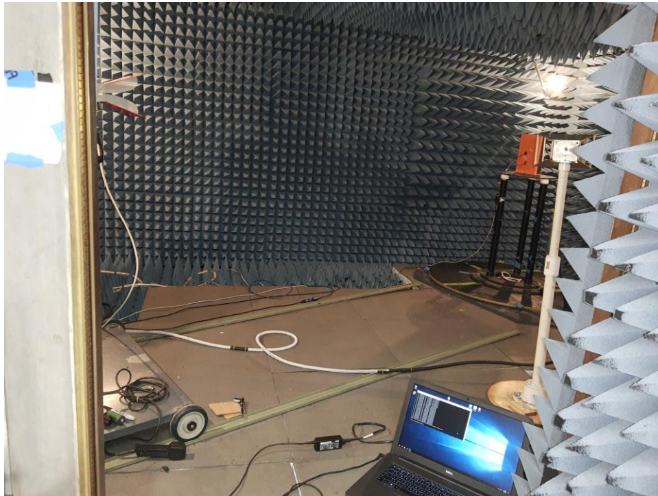
Figure 42: DFS Test Setup
