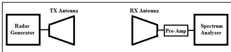
Figure 12: Radiated DFS Calibration Block Diagram
