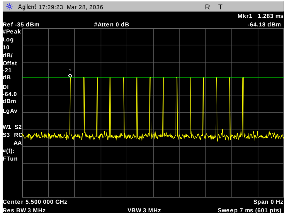
Figure 18: 5500MHz 20M Type -4 Calibration
