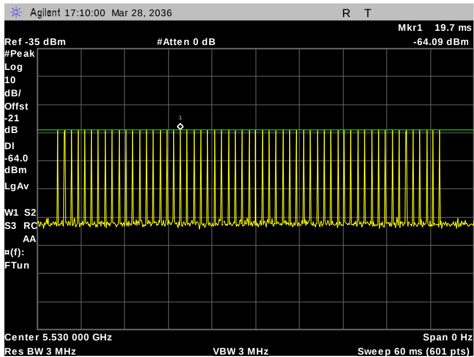
Figure 29: 5530MHz 80M Type -1 Calibration
