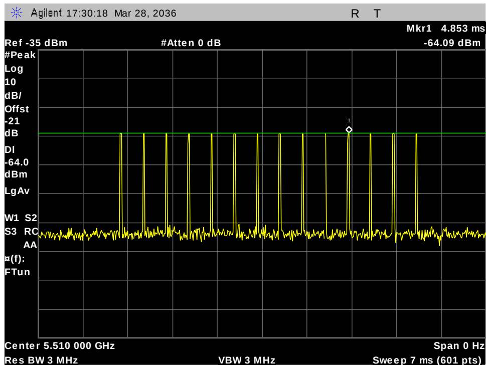
Figure 25: 5510MHz 40M Type -4 Calibration
