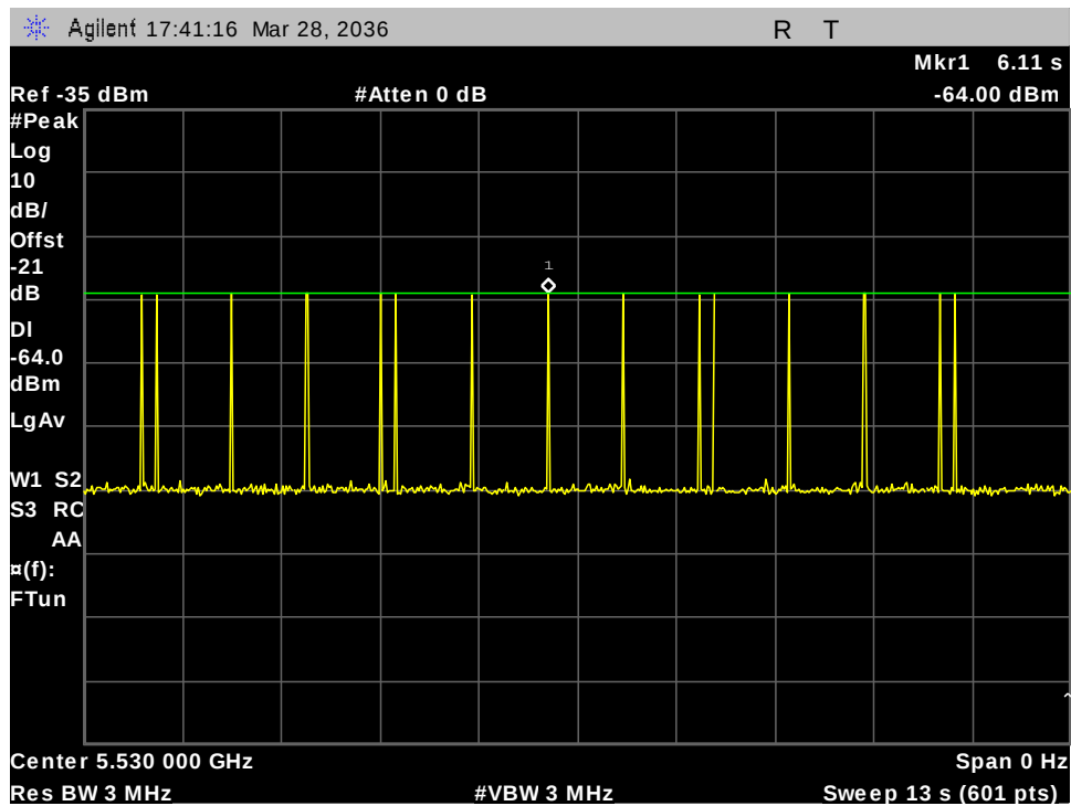
Figure 33: 5530MHz 80M Type -5 Calibration
