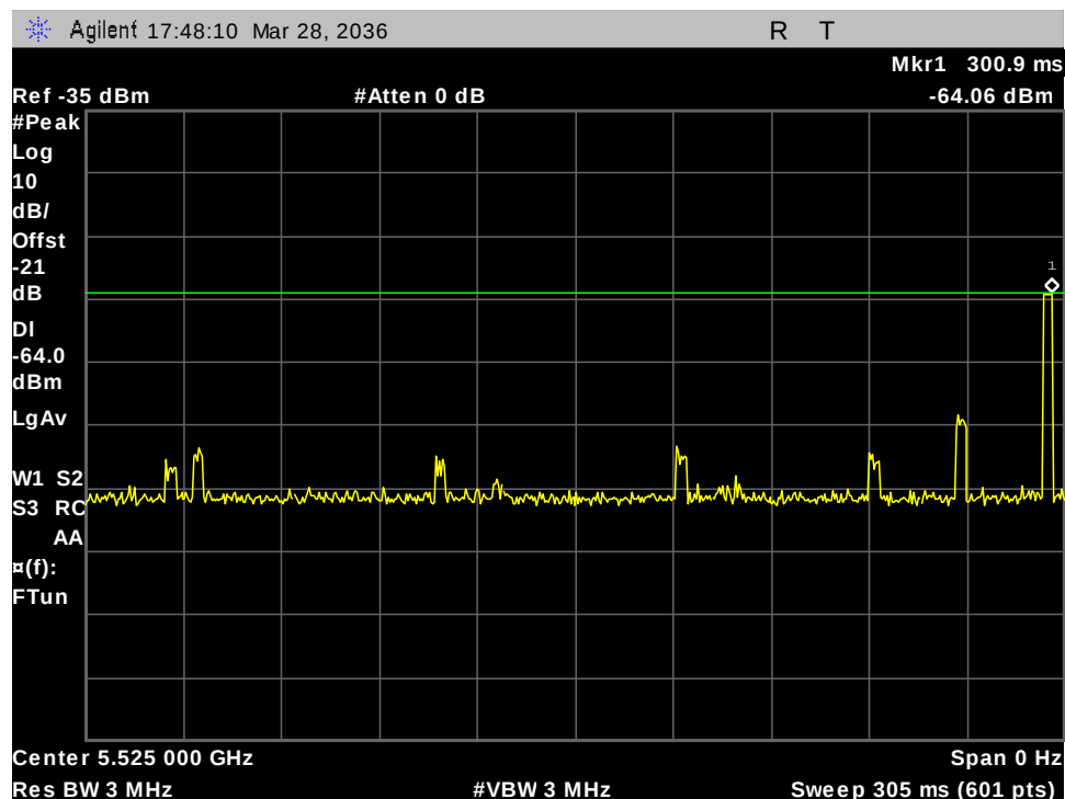
Figure 34: 5530MHz 80M Type -6 hop at 5525MHz Calibration
