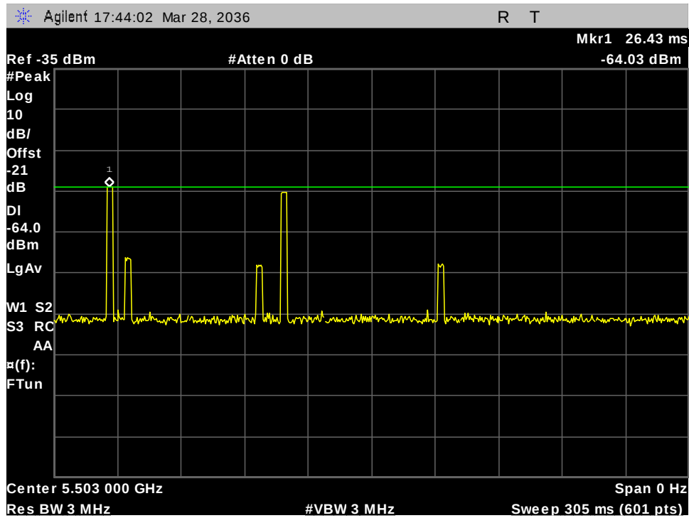
Figure 20: 5500MHz 20M Type -6 hop at 5503MHz Calibration
