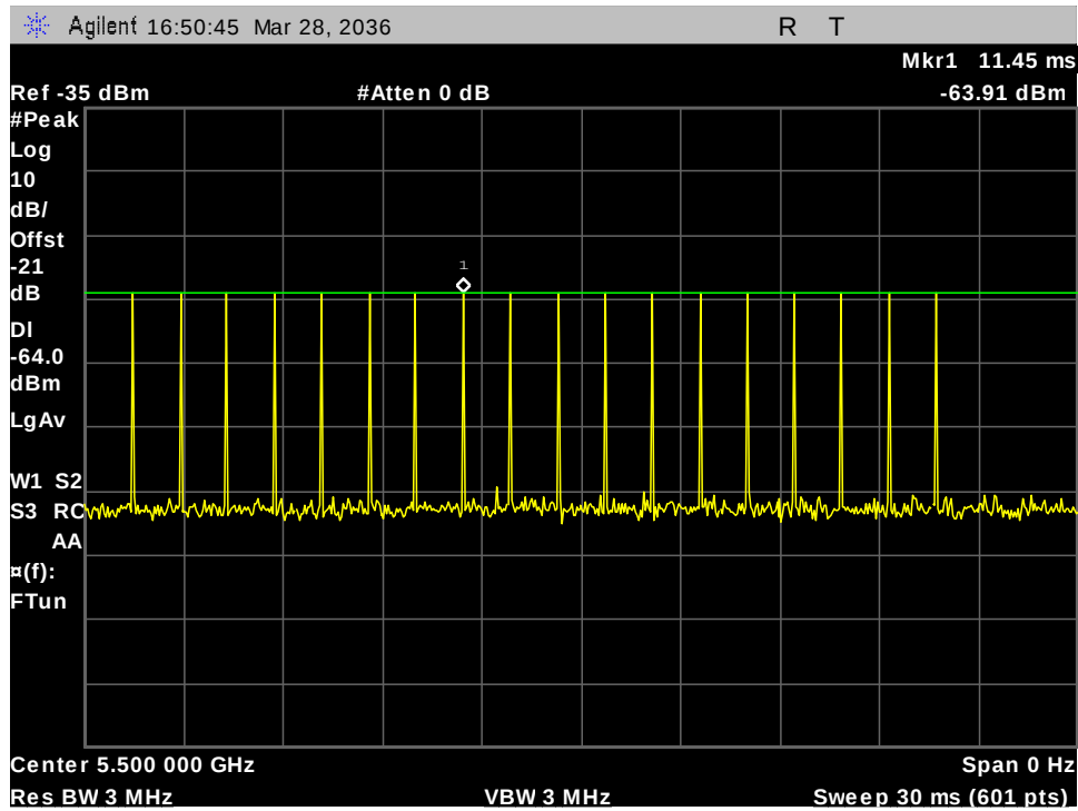
Figure 14: 5500MHz 20M Type -0 Calibration
