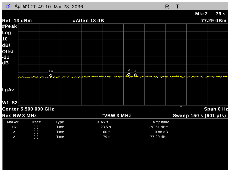
Figure 38: 5500 MHz Radar at Channel Availability Check End
