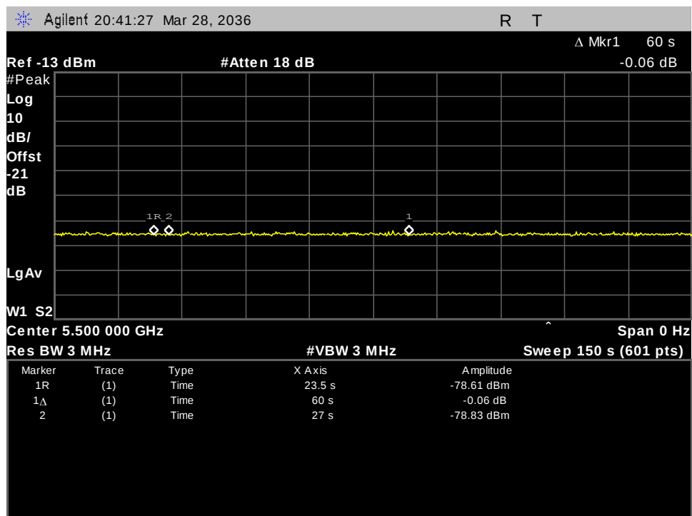
Figure 37: 5500 MHz Radar at Channel Availability Check Start
