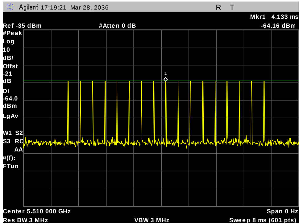
Figure 24: 5510MHz 40M Type -3 Calibration
