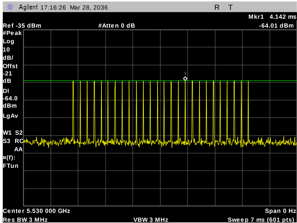
Figure 30: 5530MHz 80M Type -2 Calibration
