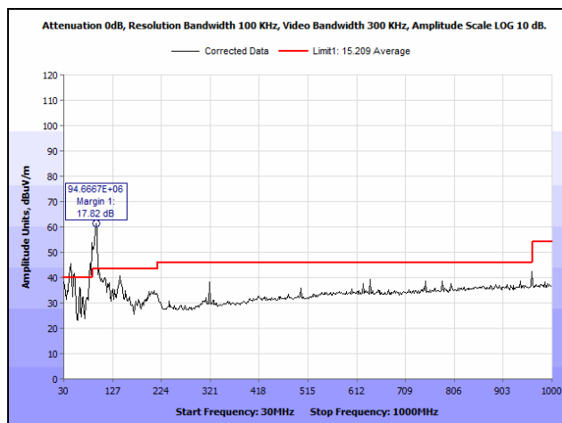
Plot 18. Radiated Spurious Emissions, Radio off, Average
