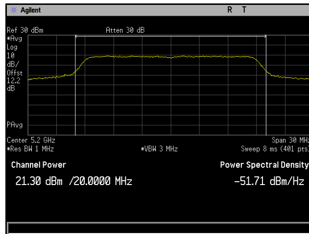
Plot 51. Output Power, 802.11ac 20 MHz, Channel 5200 MHz, 4x8 MCS0 CH6
