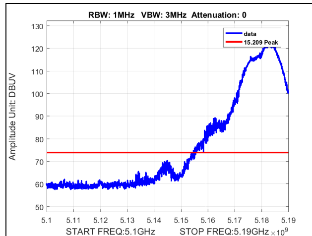
Plot 396. Radiated Band Edge, 802.11n 20 MHz, Channel 5180 MHz, 6x8, Peak, NSS1, P20-17
