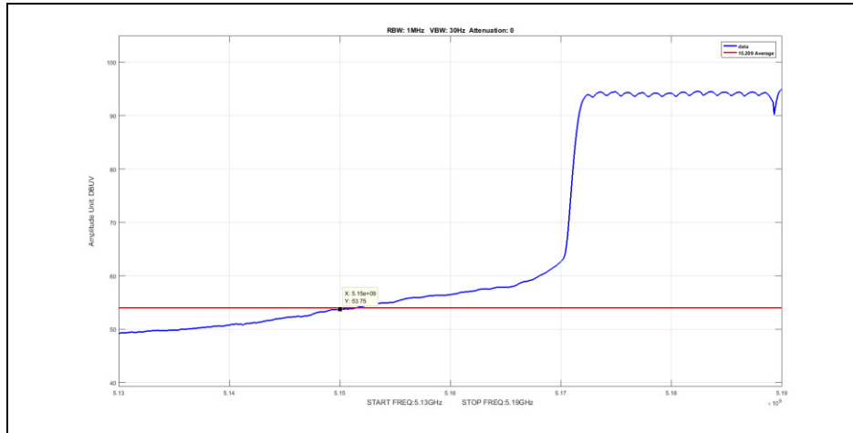
Plot 366. Radiated Band Edge, 802.11ac 40 MHz, Channel 5190 MHz, 4x8, Average, MCS0 NSS1, P17-14
