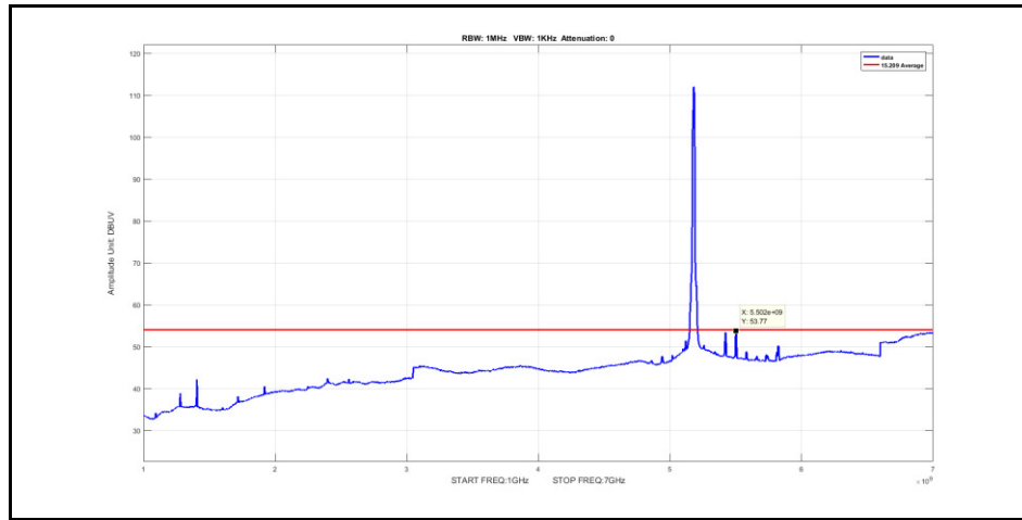
Plot 349. Radiated Spurious Emissions, 802.11n 20 MHz, 5180 MHz, 6x8, MCS0, 1 GHz – 7 GHz, Average
