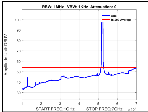
Plot 345. Radiated Spurious Emissions, 802.11ac 80 MHz, 5210 MHz, 6x8, MCS0 NSS1, 1 GHz – 7 GHz, Average
