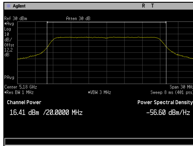
Plot 71. Output Power, 802.11n 20 MHz, Channel 5180 MHz, 4x8 MCS0 CH5
