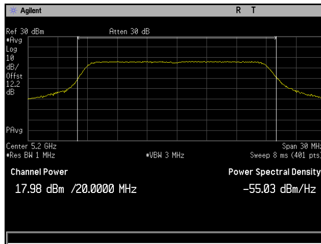
Plot 146. Output Power, 802.11n 20 MHz, Channel 5200 MHz, 6x8 MCS0 CH4
