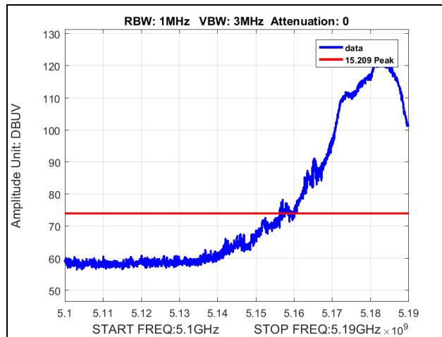
Plot 381. Radiated Band Edge, 802.11a, Channel 5180 MHz, 6x8, Peak, P20-17
