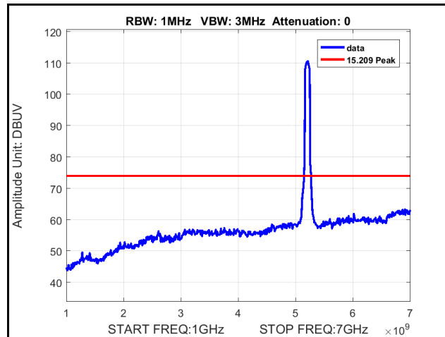
Plot 346. Radiated Spurious Emissions, 802.11ac 80 MHz, 5210 MHz, 6x8, MCS0 NSS1, 1 GHz – 7 GHz, Peak
