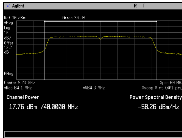
Plot 128. Output Power, 802.11ac 40 MHz, Channel 5230 MHz, 6x8 MCS0 NSS1 CH5
