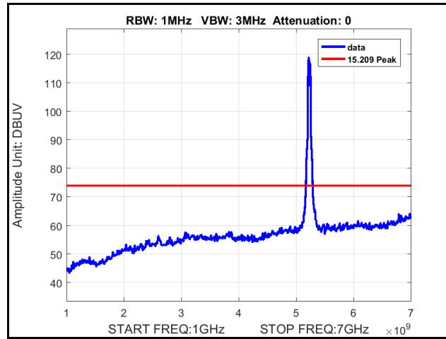
Plot 356. Radiated Spurious Emissions, 802.11n 40 MHz, 5230 MHz, 6x8, MCS0, 1 GHz – 7 GHz, Peak
