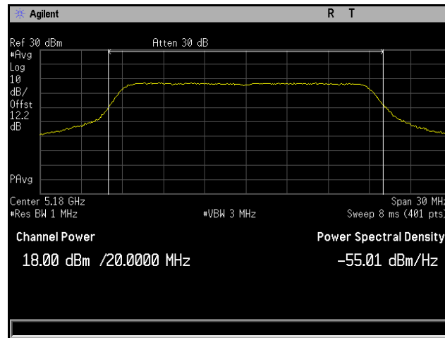
Plot 139. Output Power, 802.11n 20 MHz, Channel 5180 MHz, 6x8 MCS0 CH2
