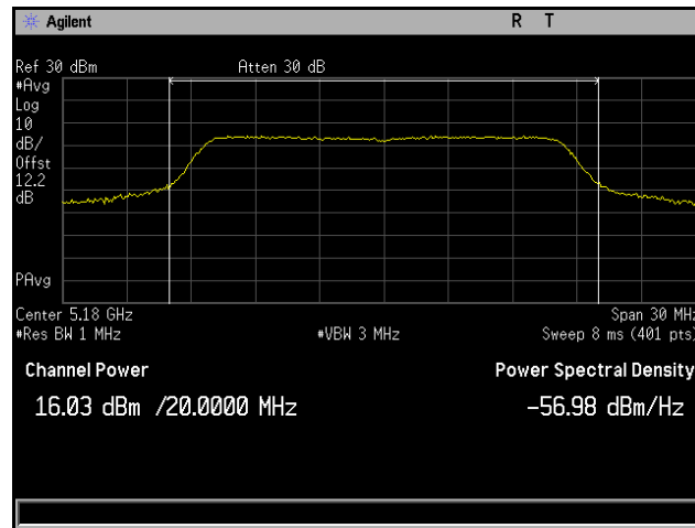
Plot 100. Output Power, 802.11a, Channel 5180 MHz, 6x8 MCS0 CH7
