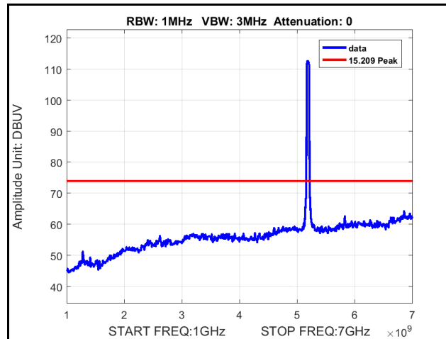
Plot 342. Radiated Spurious Emissions, 802.11ac 40 MHz, 5190 MHz, 6x8, MCS0 NSS1, 1 GHz – 7 GHz, Peak
