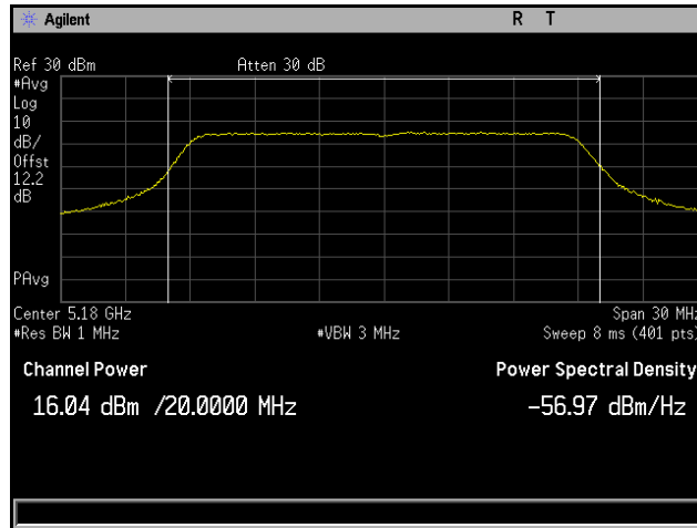
Plot 145. Output Power, 802.11n 20 MHz, Channel 5180 MHz, 6x8 MCS0 CH4
