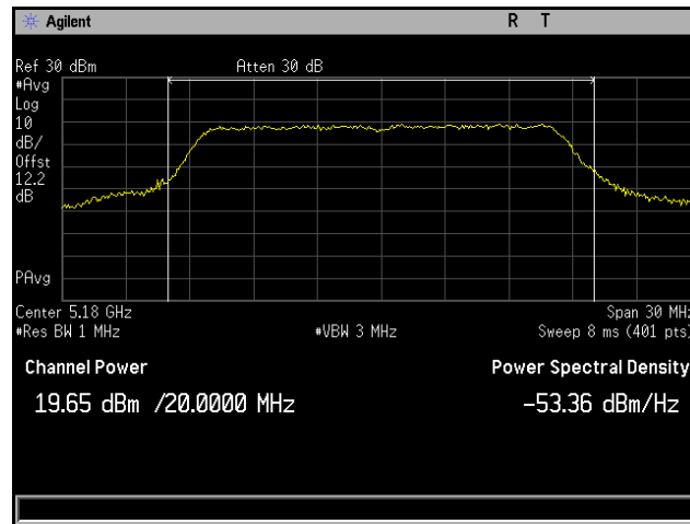
Plot 29. Output Power, 802.11a, Channel 5180 MHz, 4x8 MCS0 CH3
