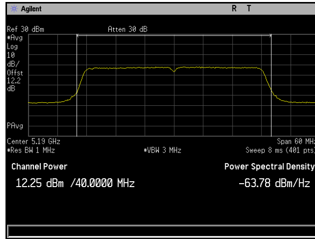
Plot 127. Output Power, 802.11ac 40 MHz, Channel 5190 MHz, 6x8 MCS0 NSS1 CH5
