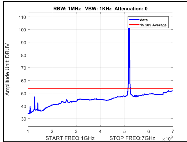
Plot 341. Radiated Spurious Emissions, 802.11ac 40 MHz, 5190 MHz, 6x8, MCS0 NSS1, 1 GHz – 7 GHz, Average
