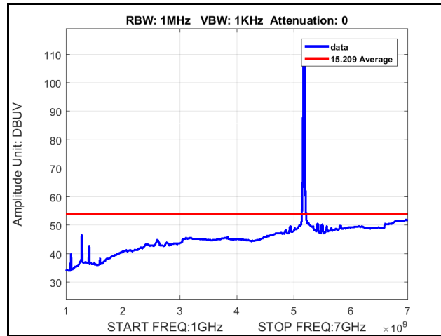
Plot 313. Radiated Spurious Emissions, 802.11ac 20 MHz, 5180 MHz, 4x8, MCS0 NSS1, 1 GHz – 7 GHz, Average
