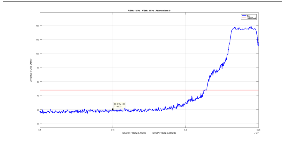
Plot 361. Radiated Band Edge, 802.11a, Channel 5240 MHz, 4x8, Peak, MCS0, P21-21
