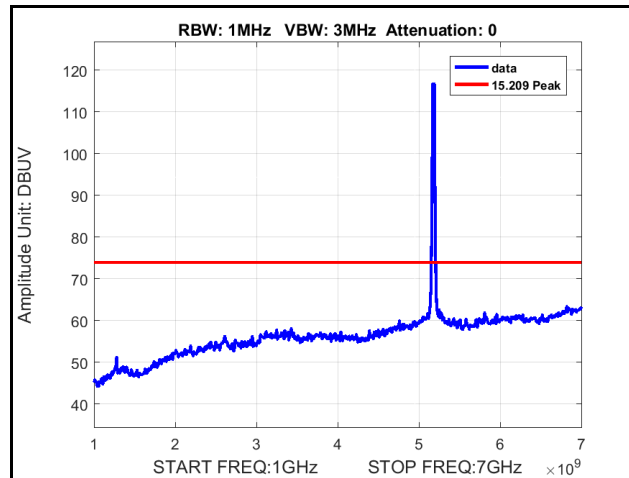
Plot 314. Radiated Spurious Emissions, 802.11ac 20 MHz, 5180 MHz, 4x8, MCS0 NSS1, 1 GHz – 7 GHz, Peak
