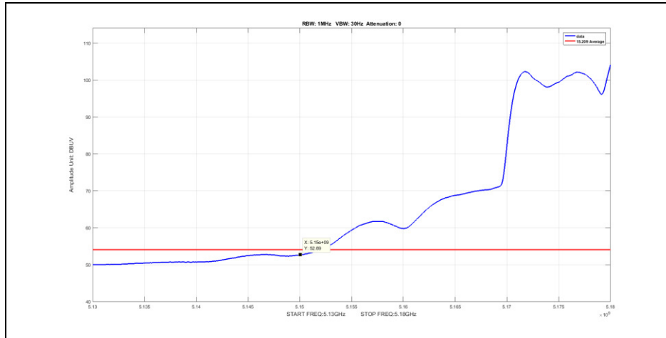
Plot 384. Radiated Band Edge, 802.11ac 20 MHz, Channel 5180 MHz, 6x8, Average, P20-17
