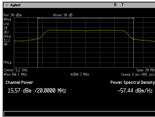
Plot 101. Output Power, 802.11a, Channel 5200 MHz, 6x8 MCS0 CH7
