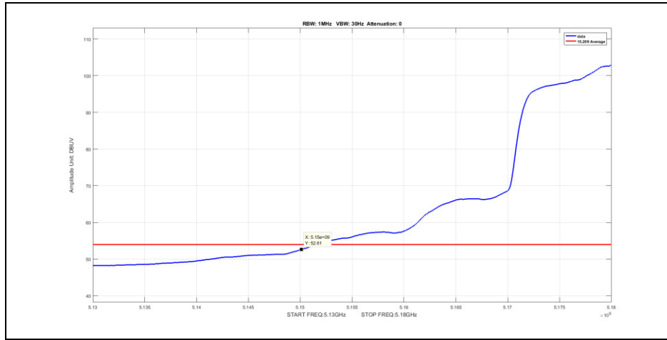
Plot 380. Radiated Band Edge, 802.11a, Channel 5180 MHz, 6x8, Average, P20-17
