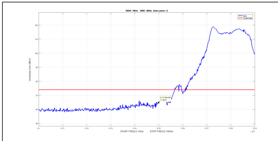
Plot 358. Radiated Band Edge, 802.11a, Channel 5180 MHz, 4x8, Peak, 6M, P21-17
