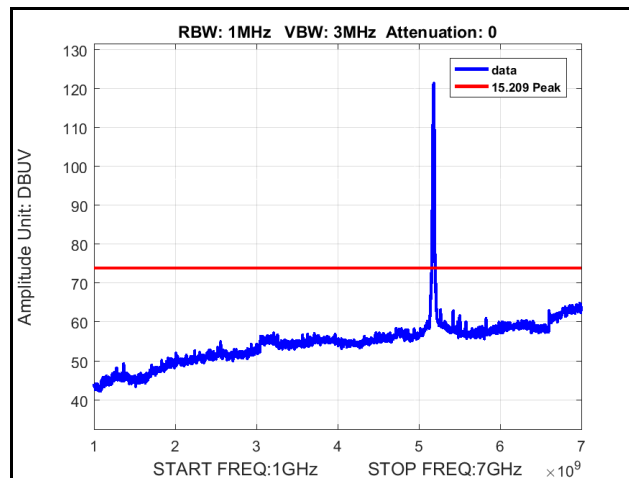
Plot 334. Radiated Spurious Emissions, 802.11a, 5180 MHz, 6x8, MCS0 NSS1, 1 GHz – 7 GHz, Peak
