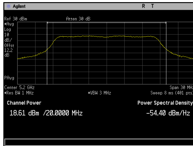
Plot 86. Output Power, 802.11a, Channel 5200 MHz, 6x8 MCS0 CH2
