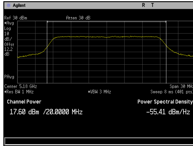
Plot 151. Output Power, 802.11n 20 MHz, Channel 5180 MHz, 6x8 MCS0 CH6
