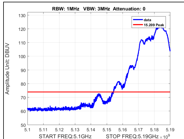
Plot 385. Radiated Band Edge, 802.11ac 20 MHz, Channel 5180 MHz, 6x8, Peak, P20-17
