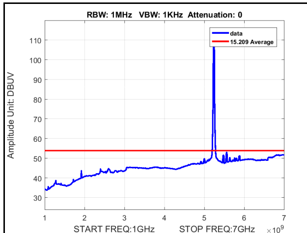
Plot 327. Radiated Spurious Emissions, 802.11n 20 MHz, 5240 MHz, 4x8, MCS0, 1 GHz – 7 GHz, Average
