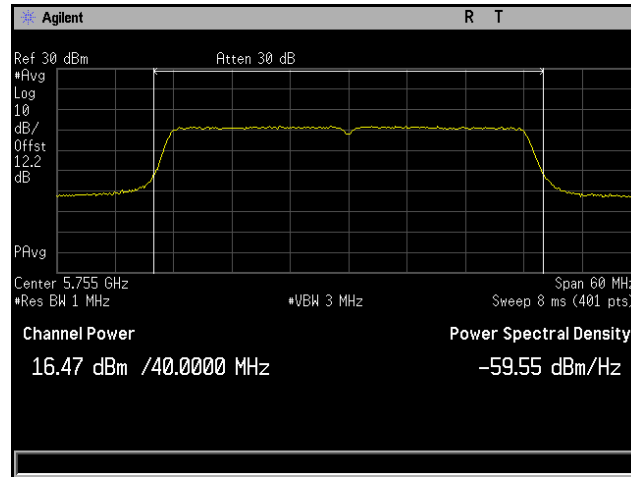
Plot 121. Conducted Output Power, 802.11ac 40 MHz, Channel 5755 MHz, 6x8, MCS0 NSS1, CH2
