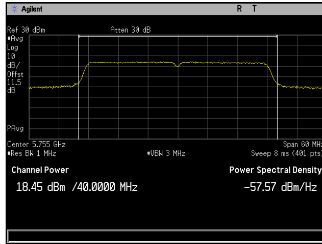
Plot 53. Conducted Output Power, 802.11ac 40 MHz, Channel 5755 MHz, 4x8, MCS0 NSS1, CH3
