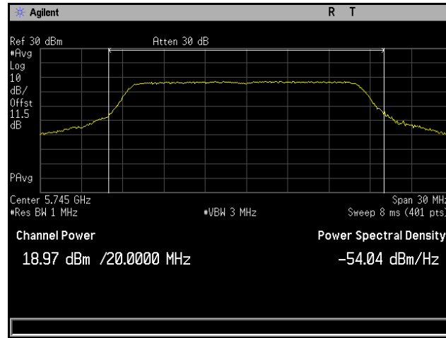
Plot 91. Conducted Output Power, 802.11a 20 MHz, Channel 5745 MHz, 6x8, 6M, CH4
