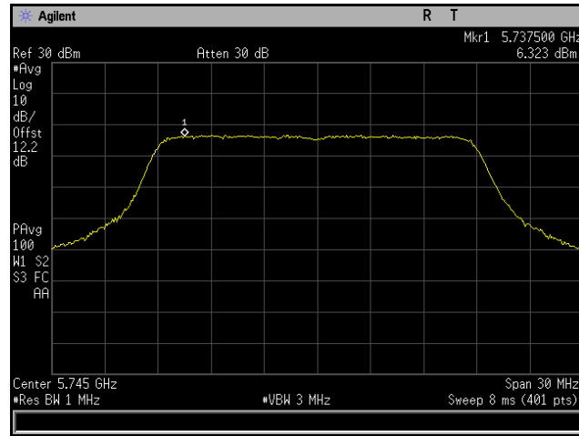
Plot 249. Power Spectral Density, 802.11ac 20 MHz, Channel 5745 MHz, 6x8, MCS0 NSS1, CH4
