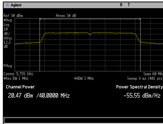
Plot 163. Conducted Output Power, 802.11n 40 MHz, Channel 5755 MHz, 6x8, MCS0 NSS1, CH5
