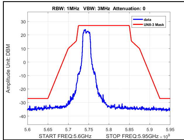
Plot 318. Radiated Spurious Emissions, Mask, 802.11n 20 MHz, Channel 5745 MHz, 4x8, MCS0
