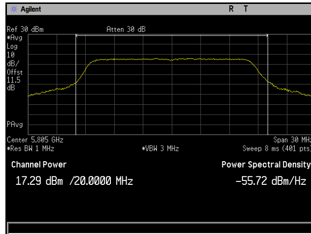
Plot 92. Conducted Output Power, 802.11a 20 MHz, Channel 5805 MHz, 6x8, 6M, CH4
