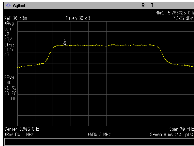
Plot 191. Power Spectral Density, 802.11ac 20 MHz, Channel 5805 MHz, 4x8, MCS0 NSS1, CH6
