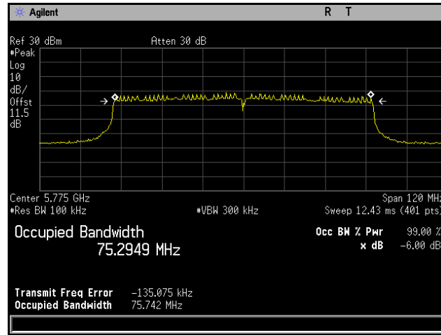
Plot 379. 6 dB Occupied Bandwidth, 802.11ac 80 MHz, Channel 5775 MHz, 6x8, NSS1 MCS0
