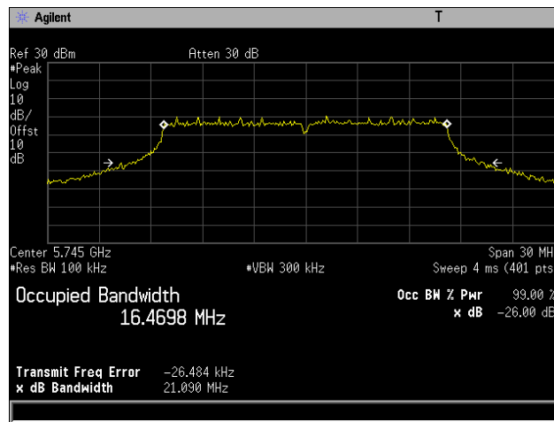
Plot 15. 26 dB Occupied Bandwidth, 802.11a 20 MHz, Channel 5745 MHz, 6x8, 6M
