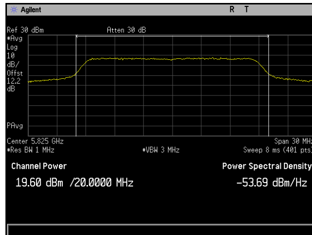
Plot 114. Conducted Output Power, 802.11ac 20 MHz, Channel 5825 MHz, 6x8, MCS0 NSS1, CH5
