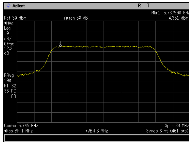
Plot 252. Power Spectral Density, 802.11ac 20 MHz, Channel 5745 MHz, 6x8, MCS0 NSS1, CH5
