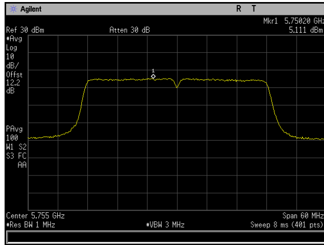
Plot 263. Power Spectral Density, 802.11ac 40 MHz, Channel 5755 MHz, 6x8, MCS0 NSS1, CH3
