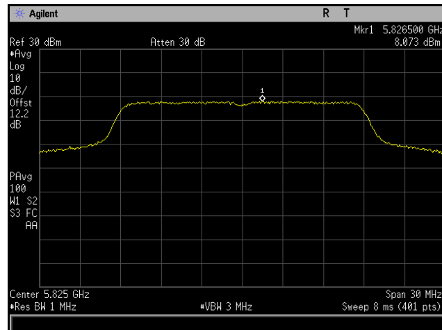
Plot 260. Power Spectral Density, 802.11ac 20 MHz, Channel 5825 MHz, 6x8, MCS0 NSS1, CH7
