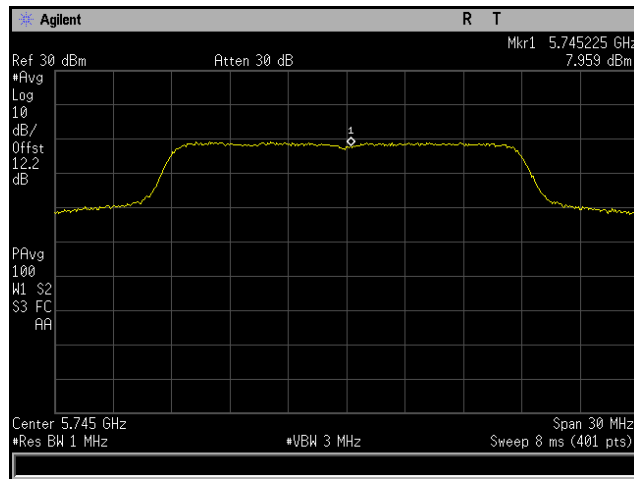
Plot 291. Power Spectral Density, 802.11n 20 MHz, Channel 5745 MHz, 6x8, MCS0 NSS1, CH6
