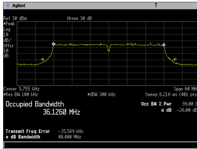
Plot 21. 26 dB Occupied Bandwidth, 802.11ac 40 MHz, Channel 5755 MHz, 6x8, NSS1 MCS0
