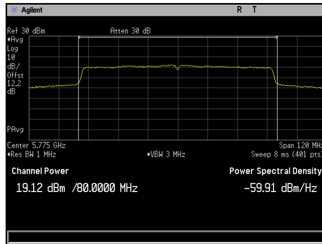
Plot 137. Conducted Output Power, 802.11ac 80 MHz, Channel 5775 MHz, 6x8, MCS0 NSS1, CH6
