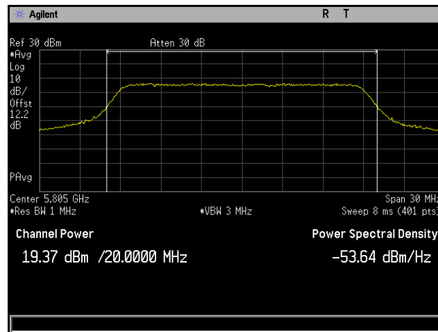
Plot 107. Conducted Output Power, 802.11ac 20 MHz, Channel 5805 MHz, 6x8, MCS0 NSS1, CH3
