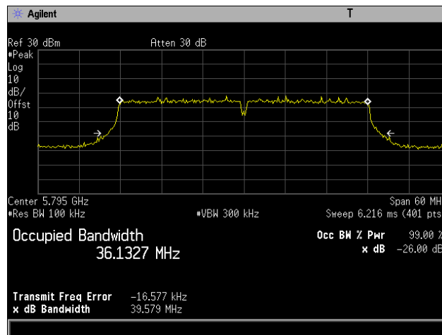
Plot 28. 26 dB Occupied Bandwidth, 802.11n 40 MHz, Channel 5795 MHz, 6x8, MCS0
