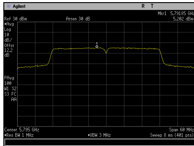
Plot 308. Power Spectral Density, 802.11n 40 MHz, Channel 5795 MHz, 6x8, MCS0 NSS1, CH7
