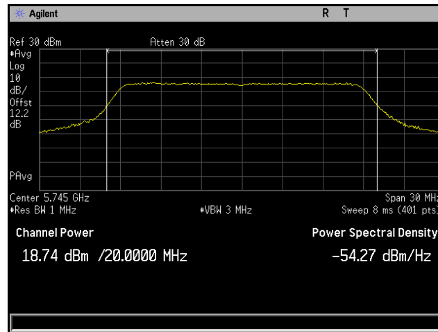
Plot 106. Conducted Output Power, 802.11ac 20 MHz, Channel 5745 MHz, 6x8, MCS0 NSS1, CH3
