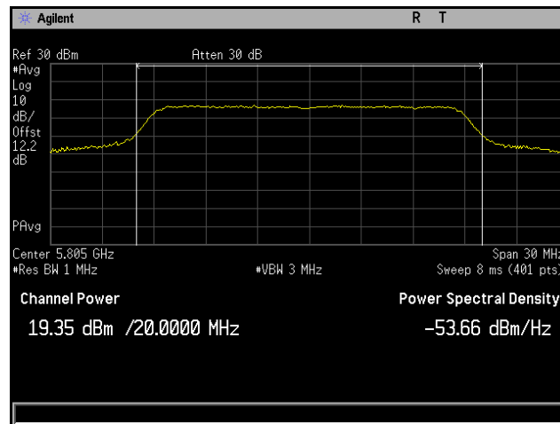
Plot 113. Conducted Output Power, 802.11ac 20 MHz, Channel 5805 MHz, 6x8, MCS0 NSS1, CH5
