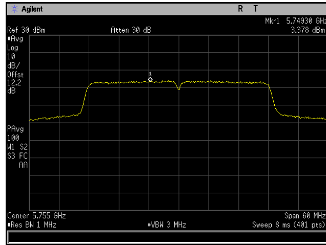
Plot 307. Power Spectral Density, 802.11n 40 MHz, Channel 5755 MHz, 6x8, MCS0 NSS1, CH7
