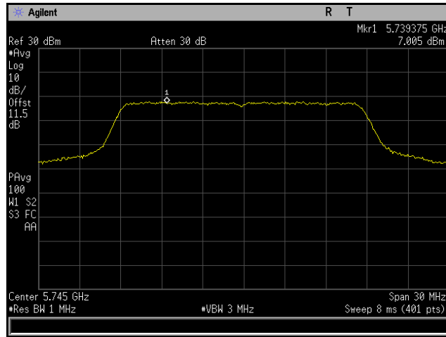
Plot 211. Power Spectral Density, 802.11n 20 MHz, Channel 5745 MHz, 4x8, MCS0 NSS1, CH5
