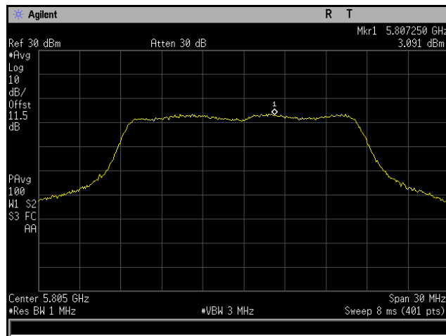
Plot 226. Power Spectral Density, 802.11a 20 MHz, Channel 5805 MHz, 6x8, 6M, CH2
