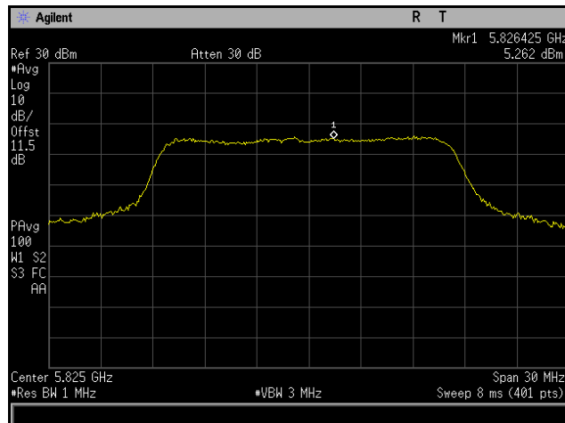
Plot 239. Power Spectral Density, 802.11a 20 MHz, Channel 5825 MHz, 6x8, 6M, CH6
