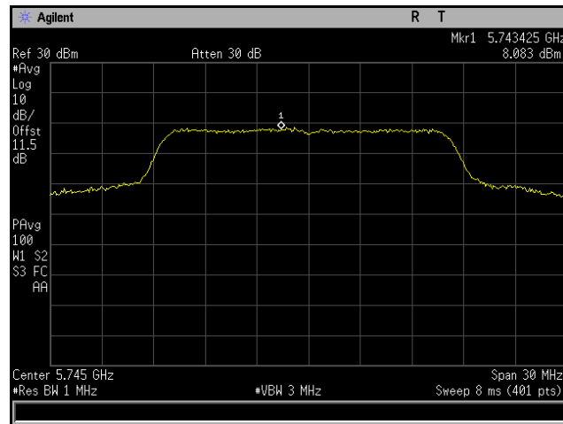
Plot 175. Power Spectral Density, 802.11a 20 MHz, Channel 5745 MHz, 4x8, 6M, CH5
