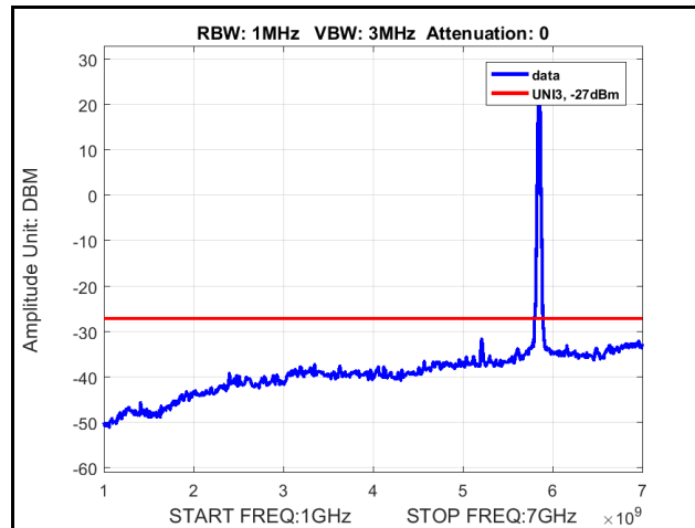
Plot 341. Radiated Spurious Emissions, 802.11n 20 MHz, Channel 5825 MHz, 4x8, MCS0, 1 GHz – 7 GHz
