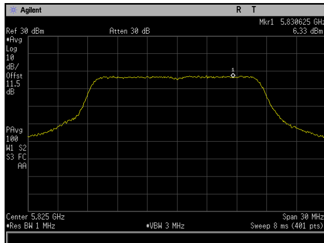
Plot 174. Power Spectral Density, 802.11a 20 MHz, Channel 5825 MHz, 4x8, 6M, CH4
