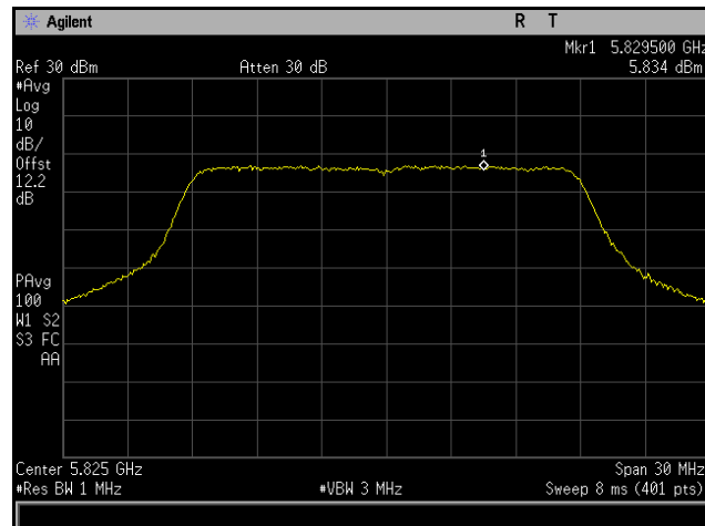
Plot 287. Power Spectral Density, 802.11n 20 MHz, Channel 5825 MHz, 6x8, MCS0 NSS1, CH4
