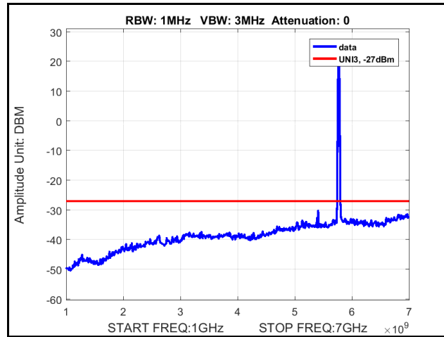
Plot 346. Radiated Spurious Emissions, 802.11ac 20 MHz, Channel 5745 MHz, 6x8, NSS1 MCS0, 1 GHz – 7 GHz
