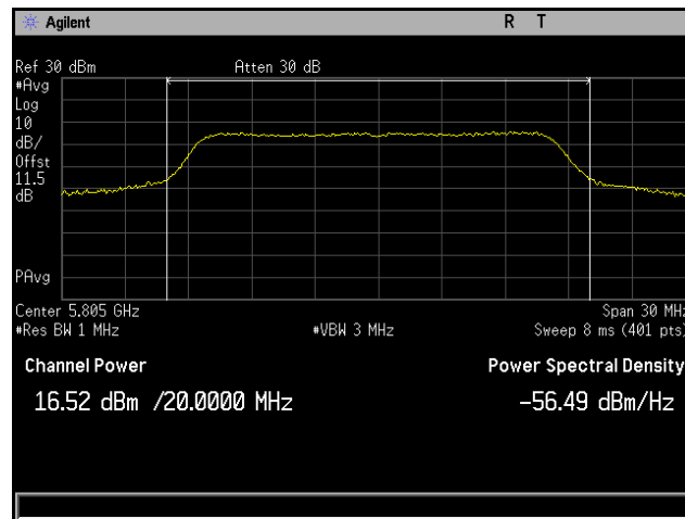
Plot 98. Conducted Output Power, 802.11a 20 MHz, Channel 5805 MHz, 6x8, 6M, CH6
