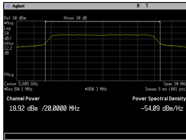
Plot 155. Conducted Output Power, 802.11n 20 MHz, Channel 5805 MHz, 6x8, MCS0 NSS1, CH7
