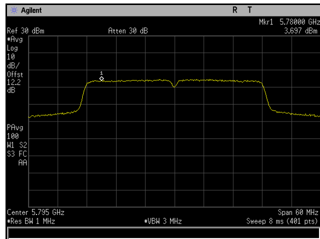
Plot 272. Power Spectral Density, 802.11ac 40 MHz, Channel 5795 MHz, 6x8, MCS0 NSS1, CH7
