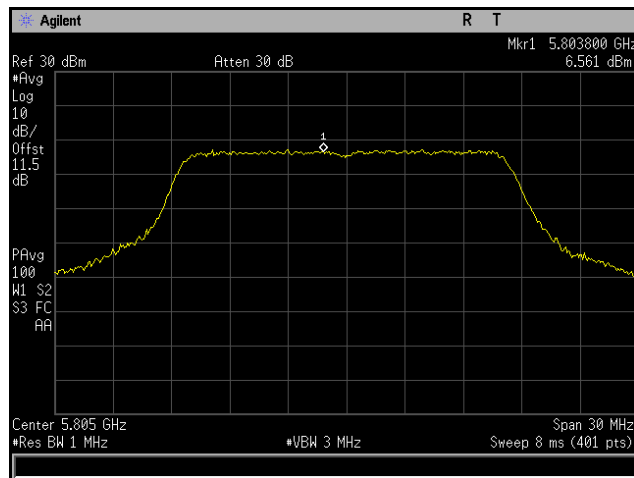
Plot 173. Power Spectral Density, 802.11a 20 MHz, Channel 5805 MHz, 4x8, 6M, CH4
