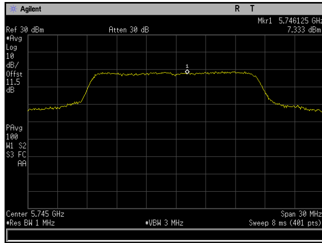
Plot 237. Power Spectral Density, 802.11a 20 MHz, Channel 5745 MHz, 6x8, 6M, CH6
