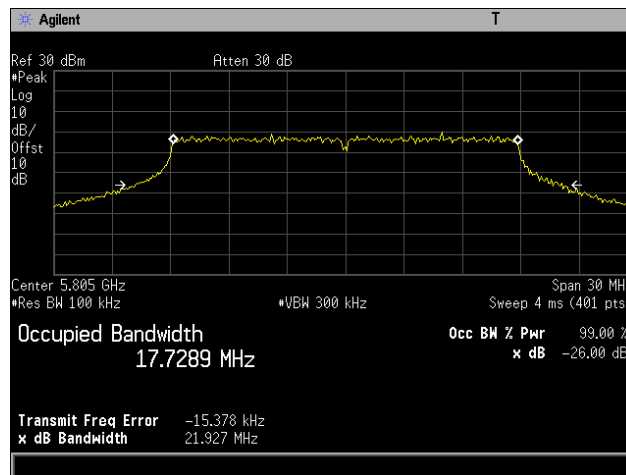
Plot 19. 26 dB Occupied Bandwidth, 802.11ac 20 MHz, Channel 5805 MHz, 6x8, NSS1 MCS0
