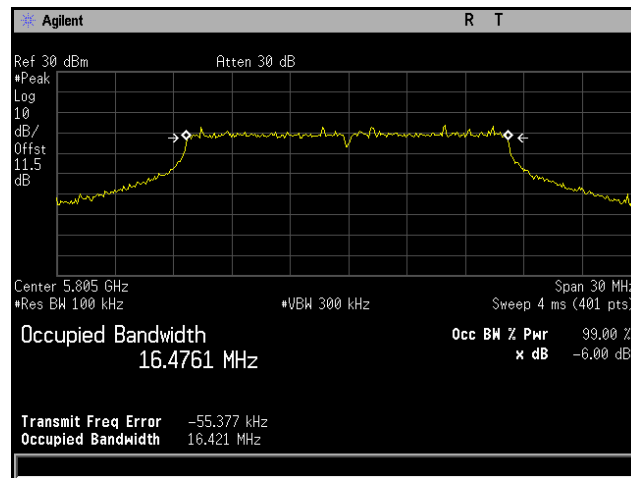
Plot 372. 6 dB Occupied Bandwidth, 802.11a 20 MHz, Channel 5805 MHz, 6x8, 6M
