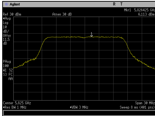
Plot 233. Power Spectral Density, 802.11a 20 MHz, Channel 5825 MHz, 6x8, 6M, CH4
