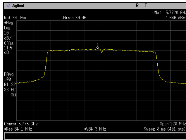
Plot 201. Power Spectral Density, 802.11ac 80 MHz, Channel 5775 MHz, 4x8, MCS0 NSS1, CH3
