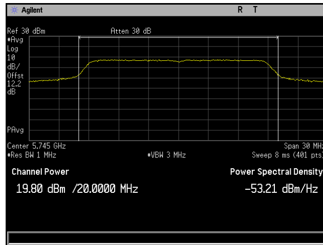
Plot 151. Conducted Output Power, 802.11n 20 MHz, Channel 5745 MHz, 6x8, MCS0 NSS1, CH6
