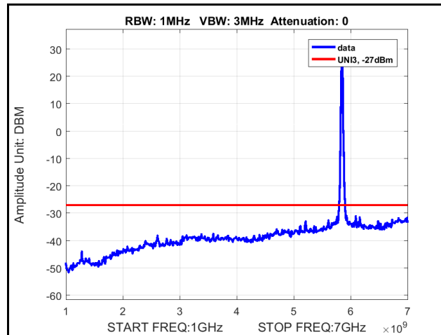
Plot 352. Radiated Spurious Emissions, 802.11n 20 MHz, Channel 5825 MHz, 6x8, MCS0, 1 GHz – 7 GHz
