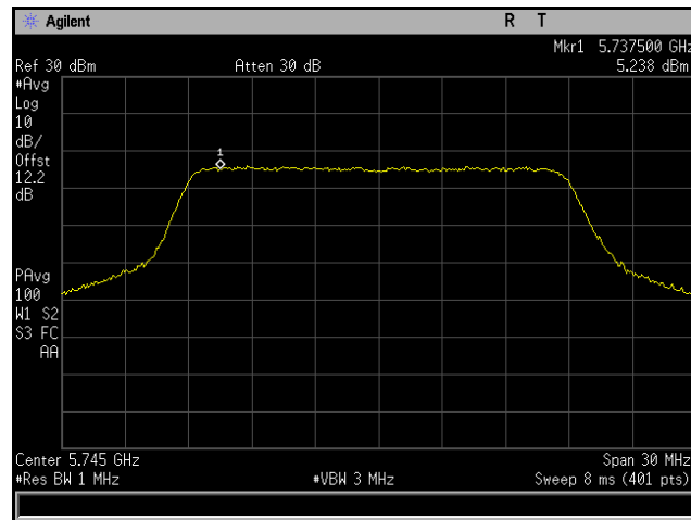
Plot 246. Power Spectral Density, 802.11ac 20 MHz, Channel 5745 MHz, 6x8, MCS0 NSS1, CH3
