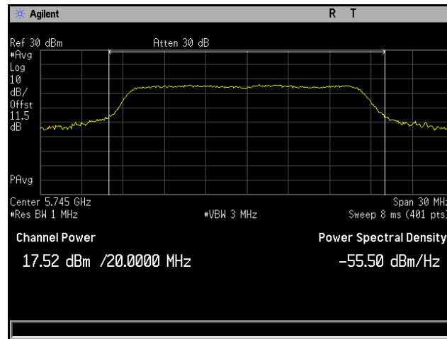
Plot 85. Conducted Output Power, 802.11a 20 MHz, Channel 5745 MHz, 6x8, 6M, CH2
