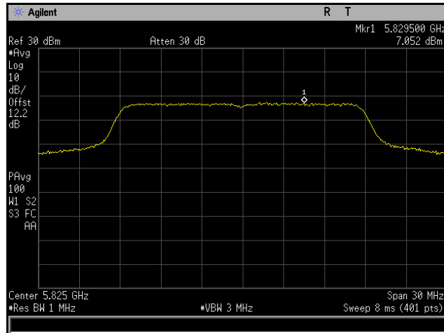
Plot 296. Power Spectral Density, 802.11n 20 MHz, Channel 5825 MHz, 6x8, MCS0 NSS1, CH7
