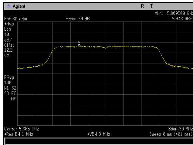
Plot 259. Power Spectral Density, 802.11ac 20 MHz, Channel 5805 MHz, 6x8, MCS0 NSS1, CH7
