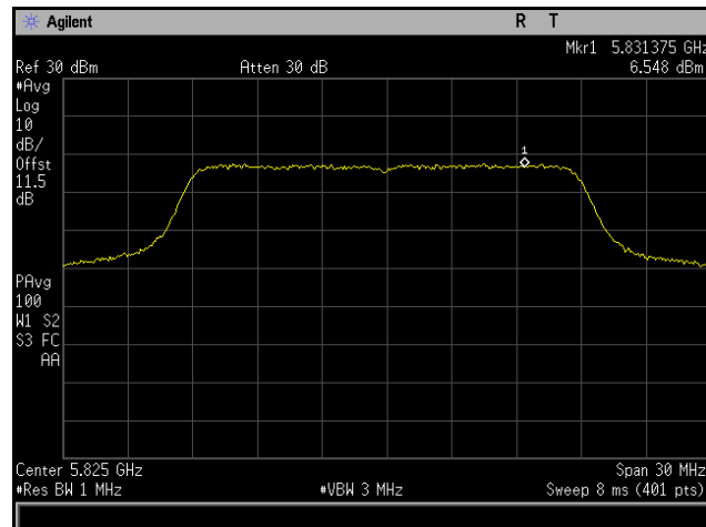
Plot 183. Power Spectral Density, 802.11ac 20 MHz, Channel 5825 MHz, 4x8, MCS0 NSS1, CH3
