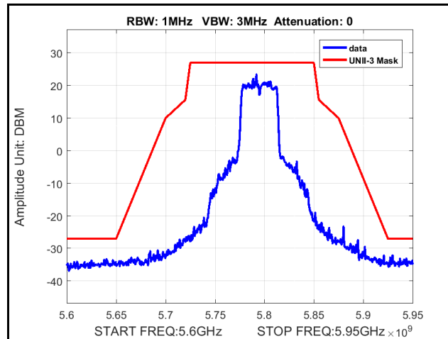
Plot 321. Radiated Spurious Emissions, Mask, 802.11n 40 MHz, Channel 5795 MHz, 4x8, MCS0
