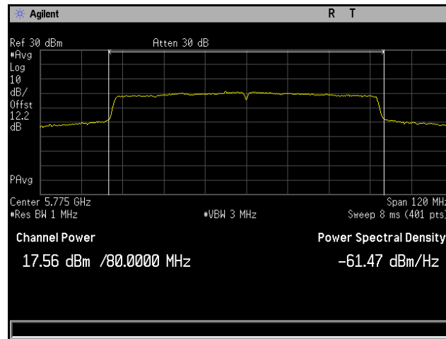
Plot 138. Conducted Output Power, 802.11ac 80 MHz, Channel 5775 MHz, 6x8, MCS0 NSS1, CH7
