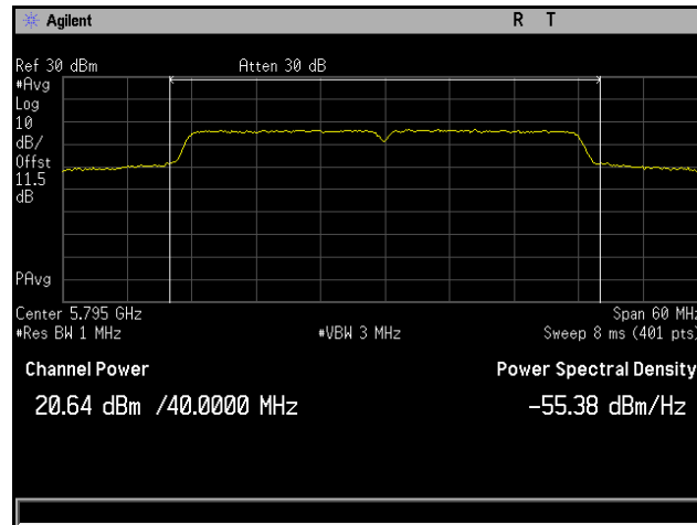
Plot 84. Conducted Output Power, 802.11n 40 MHz, Channel 5795 MHz, 4x8, MCS0 NSS1, CH6
