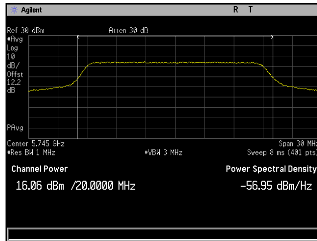
Plot 103. Conducted Output Power, 802.11ac 20 MHz, Channel 5745 MHz, 6x8, MCS0 NSS1, CH2
