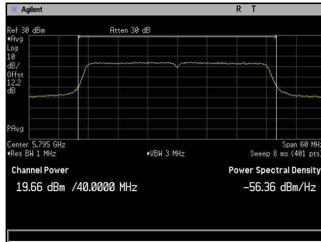
Plot 124. Conducted Output Power, 802.11ac 40 MHz, Channel 5795 MHz, 6x8, MCS0 NSS1, CH3
