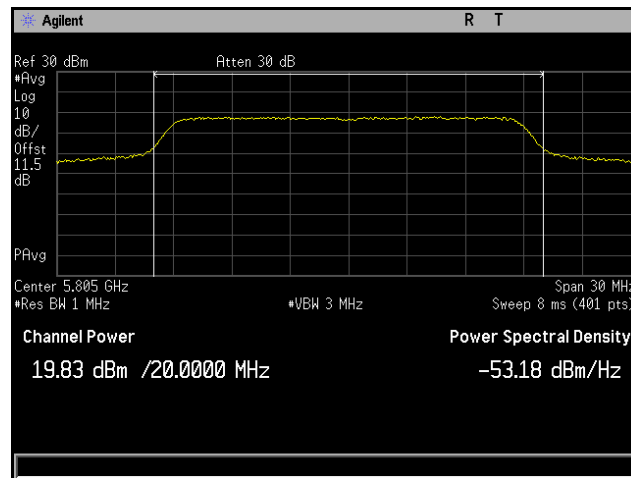
Plot 51. Conducted Output Power, 802.11ac 20 MHz, Channel 5805 MHz, 4x8, MCS0 NSS1, CH6
