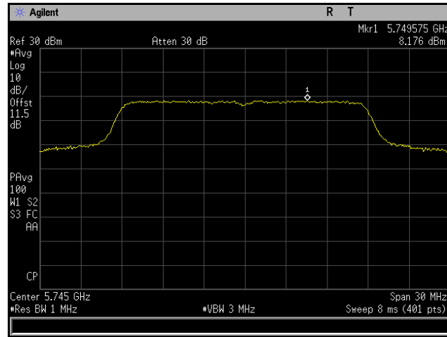
Plot 190. Power Spectral Density, 802.11ac 20 MHz, Channel 5745 MHz, 4x8, MCS0 NSS1, CH6
