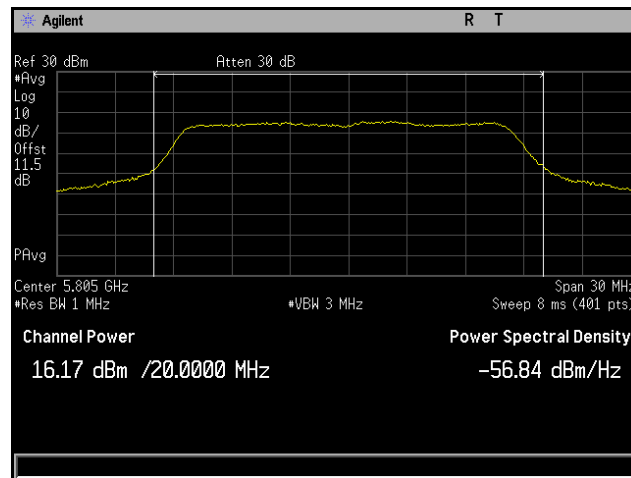
Plot 86. Conducted Output Power, 802.11a 20 MHz, Channel 5805 MHz, 6x8, 6M, CH2
