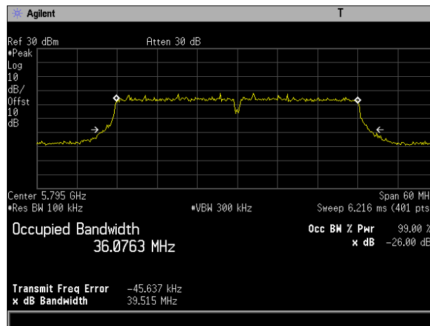
Plot 8. 26 dB Occupied Bandwidth, 802.11ac 40 MHz, Channel 5795 MHz, 4x8, NSS1 MCS0
