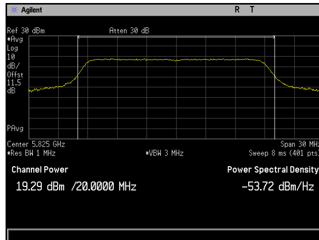
Plot 43. Conducted Output Power, 802.11ac 20 MHz, Channel 5825 MHz, 4x8, MCS0 NSS1, CH3
