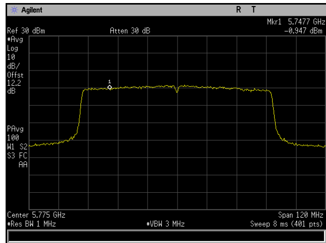
Plot 275. Power Spectral Density, 802.11ac 80 MHz, Channel 5775 MHz, 6x8, MCS0 NSS1, CH4
