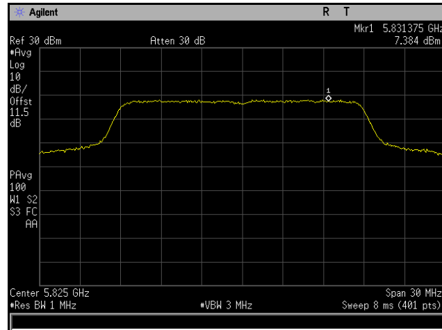
Plot 192. Power Spectral Density, 802.11ac 20 MHz, Channel 5825 MHz, 4x8, MCS0 NSS1, CH6
