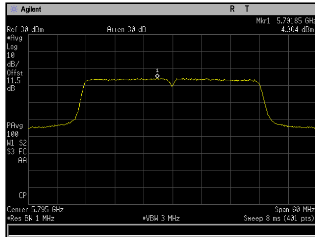
Plot 196. Power Spectral Density, 802.11ac 40 MHz, Channel 5795 MHz, 4x8, MCS0 NSS1, CH4
