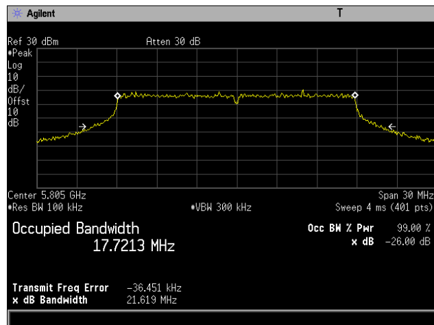
Plot 11. 26 dB Occupied Bandwidth, 802.11n 20 MHz, Channel 5805 MHz, 4x8, MCS0
