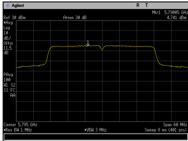
Plot 222. Power Spectral Density, 802.11n 40 MHz, Channel 5795 MHz, 4x8, MCS0 NSS1, CH5
