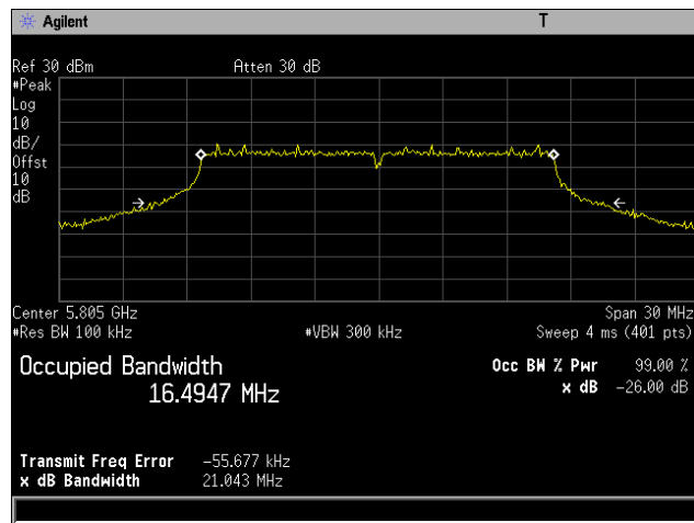
Plot 2. 26 dB Occupied Bandwidth, 802.11a 20 MHz, Channel 5805 MHz, 4x8, 6M
