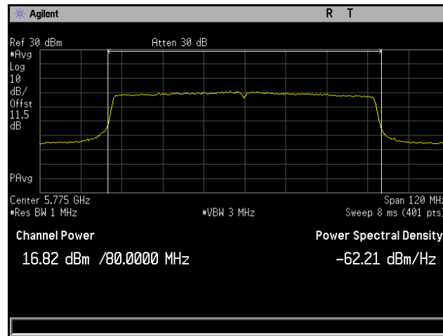
Plot 62. Conducted Output Power, 802.11ac 80 MHz, Channel 5775 MHz, 4x8, MCS0 NSS1, CH4
