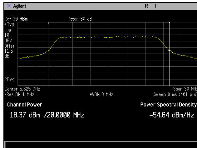
Plot 34. Conducted Output Power, 802.11a 20 MHz, Channel 5825 MHz, 4x8, 6M, CH4
