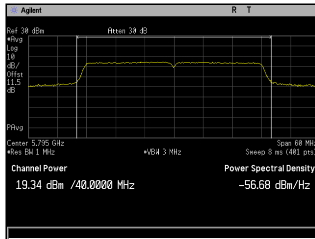
Plot 58. Conducted Output Power, 802.11ac 40 MHz, Channel 5795 MHz, 4x8, MCS0 NSS1, CH5
