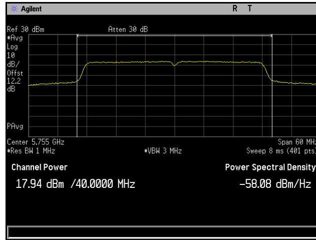
Plot 131. Conducted Output Power, 802.11ac 40 MHz, Channel 5755 MHz, 6x8, MCS0 NSS1, CH7
