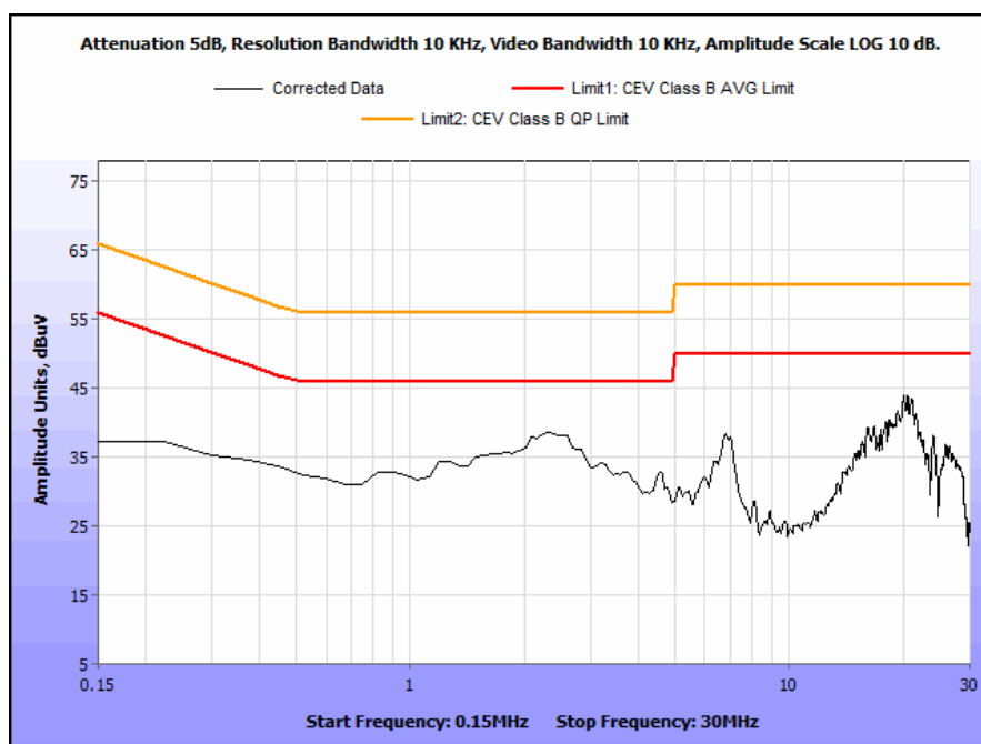
Plot 355. Conducted Emissions, 15.207(a), Phase Line
