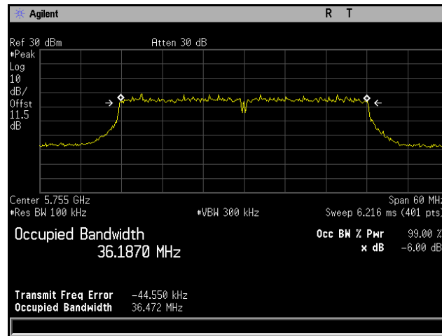
Plot 377. 6 dB Occupied Bandwidth, 802.11ac 40 MHz, Channel 5755 MHz, 6x8, NSS1 MCS0
