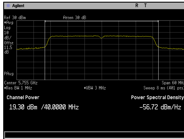
Plot 57. Conducted Output Power, 802.11ac 40 MHz, Channel 5755 MHz, 4x8, MCS0 NSS1, CH5
