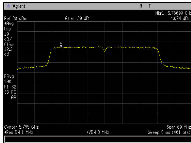
Plot 268. Power Spectral Density, 802.11ac 40 MHz, Channel 5795 MHz, 6x8, MCS0 NSS1, CH5
