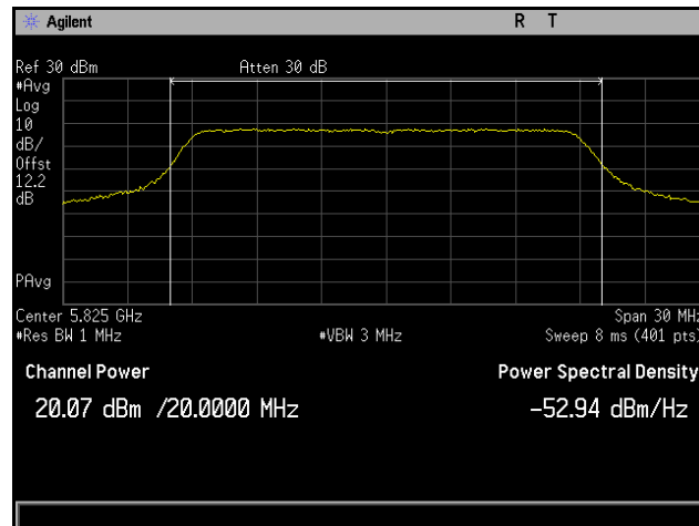
Plot 108. Conducted Output Power, 802.11ac 20 MHz, Channel 5825 MHz, 6x8, MCS0 NSS1, CH3
