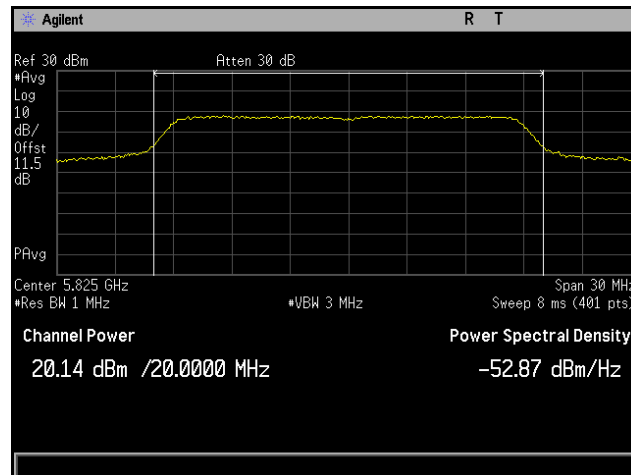
Plot 52. Conducted Output Power, 802.11ac 20 MHz, Channel 5825 MHz, 4x8, MCS0 NSS1, CH6
