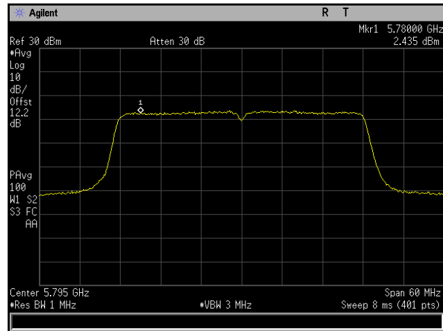
Plot 262. Power Spectral Density, 802.11ac 40 MHz, Channel 5795 MHz, 6x8, MCS0 NSS1, CH2
