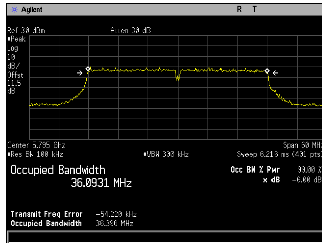
Plot 370. 6 dB Occupied Bandwidth, 802.11n 40 MHz, Channel 5795 MHz, 4x8, MCS0
