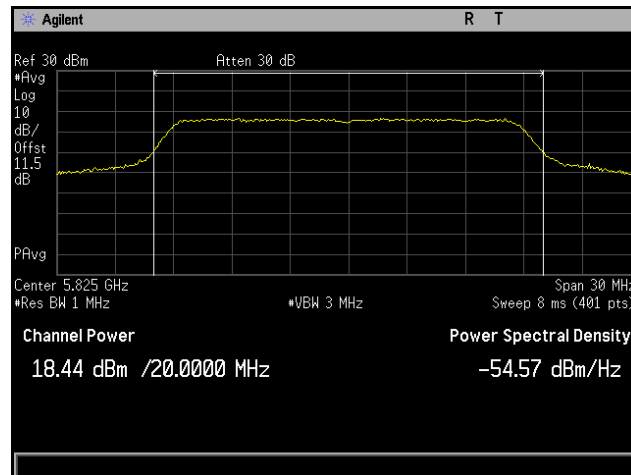
Plot 73. Conducted Output Power, 802.11n 20 MHz, Channel 5825 MHz, 4x8, MCS0 NSS1, CH5
