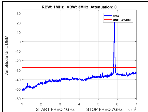
Plot 334. Radiated Spurious Emissions, 802.11a 20 MHz, Channel 5825 MHz, 4x8, 6M, 1 GHz – 7 GHz
