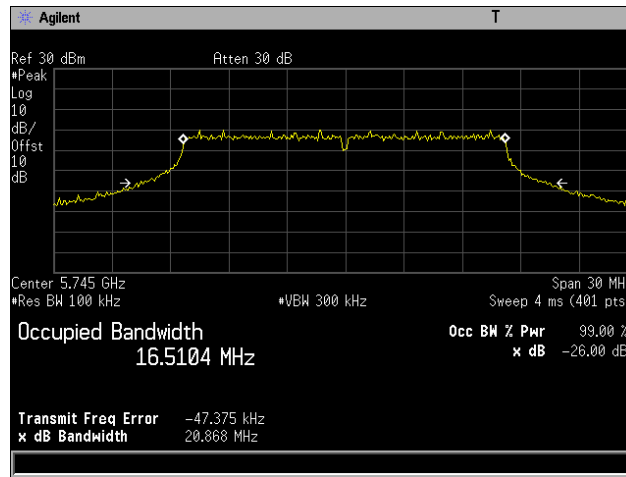
Plot 1. 26 dB Occupied Bandwidth, 802.11a 20 MHz, Channel 5745 MHz, 4x8, 6M
