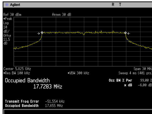
Plot 368. 6 dB Occupied Bandwidth, 802.11n 20 MHz, Channel 5825 MHz, 4x8, MCS0
