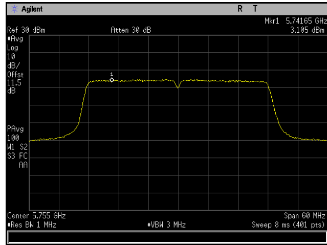
Plot 219. Power Spectral Density, 802.11n 40 MHz, Channel 5755 MHz, 4x8, MCS0 NSS1, CH4
