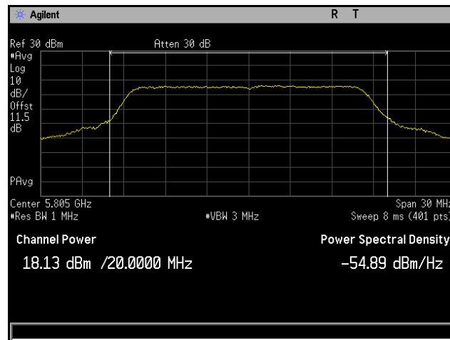
Plot 89. Conducted Output Power, 802.11a 20 MHz, Channel 5805 MHz, 6x8, 6M, CH3
