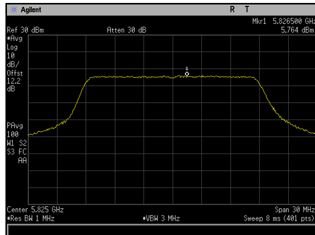
Plot 245. Power Spectral Density, 802.11ac 20 MHz, Channel 5825 MHz, 6x8, MCS0 NSS1, CH2
