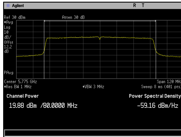
Plot 134. Conducted Output Power, 802.11ac 80 MHz, Channel 5775 MHz, 6x8, MCS0 NSS1, CH3
