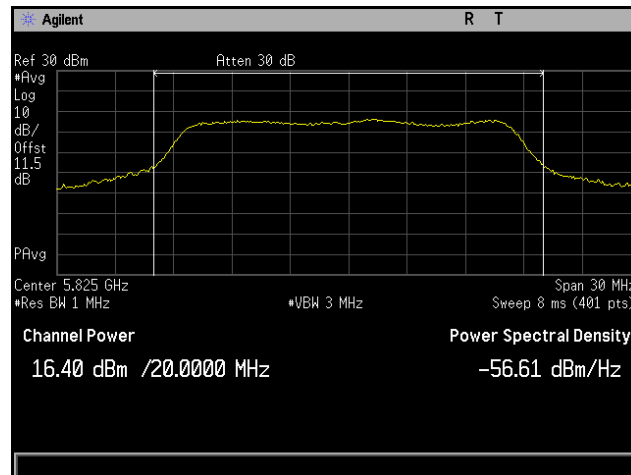
Plot 96. Conducted Output Power, 802.11a 20 MHz, Channel 5825 MHz, 6x8, 6M, CH5
