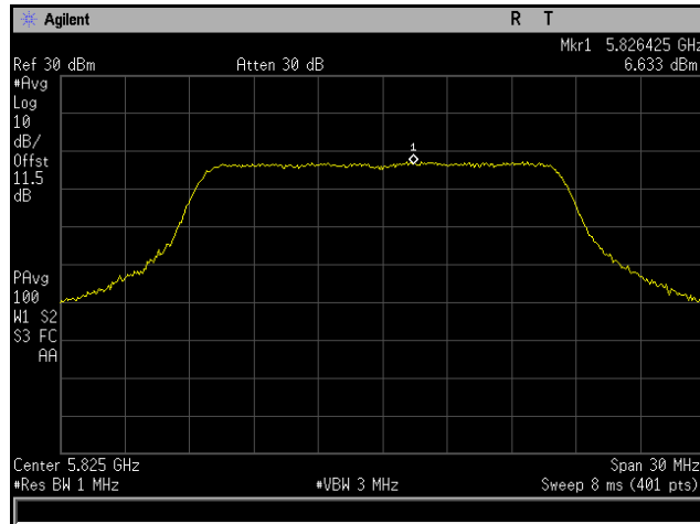
Plot 230. Power Spectral Density, 802.11a 20 MHz, Channel 5825 MHz, 6x8, 6M, CH3
