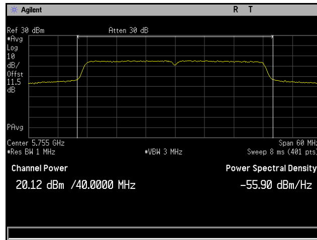
Plot 81. Conducted Output Power, 802.11n 40 MHz, Channel 5755 MHz, 4x8, MCS0 NSS1, CH5
