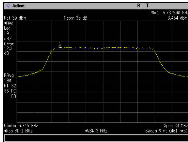
Plot 243. Power Spectral Density, 802.11ac 20 MHz, Channel 5745 MHz, 6x8, MCS0 NSS1, CH2
