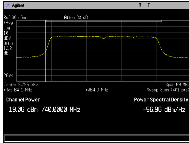
Plot 161. Conducted Output Power, 802.11n 40 MHz, Channel 5755 MHz, 6x8, MCS0 NSS1, CH4
