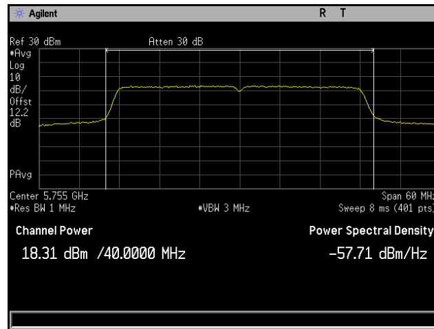
Plot 125. Conducted Output Power, 802.11ac 40 MHz, Channel 5755 MHz, 6x8, MCS0 NSS1, CH4
