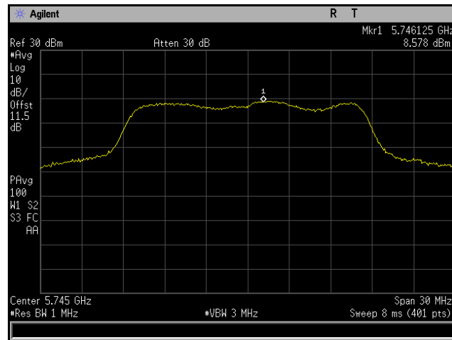
Plot 234. Power Spectral Density, 802.11a 20 MHz, Channel 5745 MHz, 6x8, 6M, CH5
