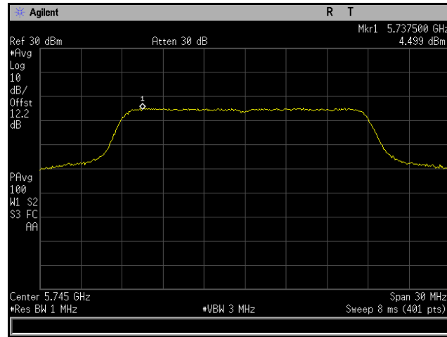
Plot 258. Power Spectral Density, 802.11ac 20 MHz, Channel 5745 MHz, 6x8, MCS0 NSS1, CH7
