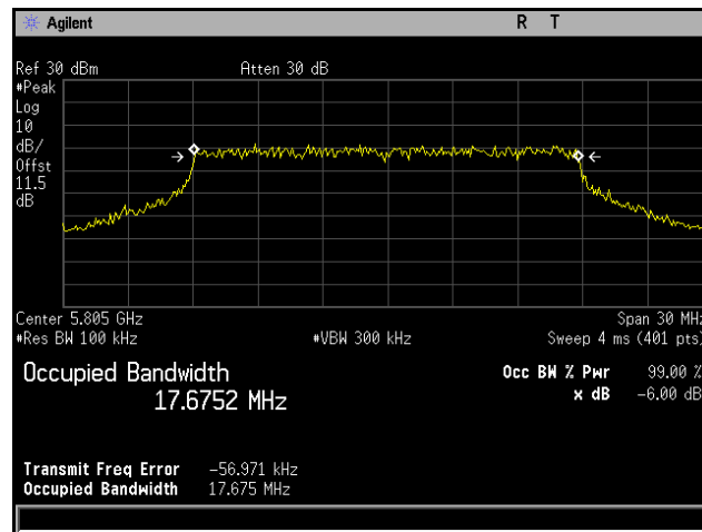
Plot 375. 6 dB Occupied Bandwidth, 802.11ac 20 MHz, Channel 5805 MHz, 6x8, NSS1 MCS0
