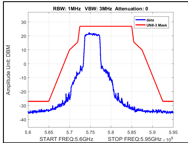
Plot 320. Radiated Spurious Emissions, Mask, 802.11n 40 MHz, Channel 5755 MHz, 4x8, MCS0
