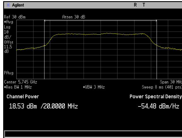
Plot 94. Conducted Output Power, 802.11a 20 MHz, Channel 5745 MHz, 6x8, 6M, CH5
