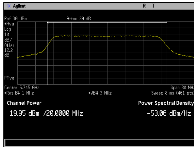
Plot 142. Conducted Output Power, 802.11n 20 MHz, Channel 5745 MHz, 6x8, MCS0 NSS1, CH3
