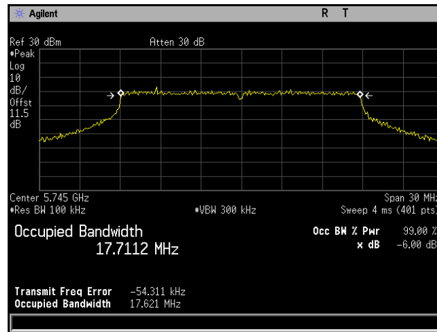
Plot 380. 6 dB Occupied Bandwidth, 802.11n 20 MHz, Channel 5745 MHz, 6x8, MCS0
