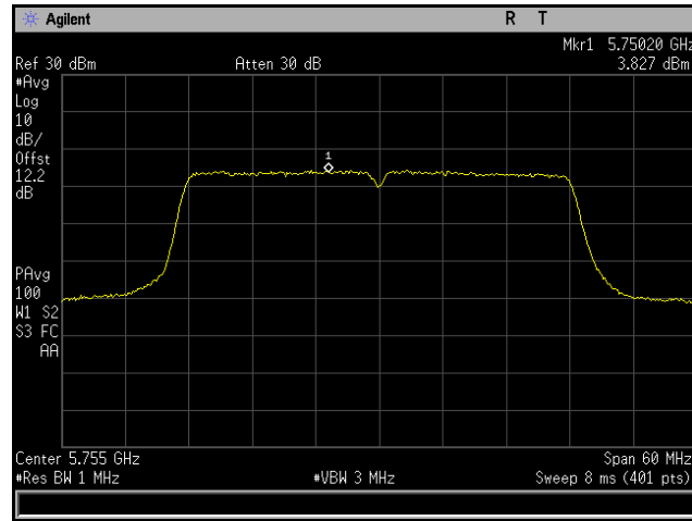
Plot 265. Power Spectral Density, 802.11ac 40 MHz, Channel 5755 MHz, 6x8, MCS0 NSS1, CH4
