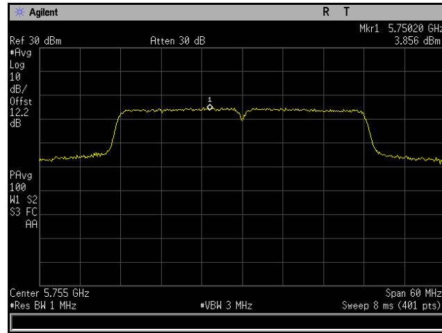
Plot 267. Power Spectral Density, 802.11ac 40 MHz, Channel 5755 MHz, 6x8, MCS0 NSS1, CH5
