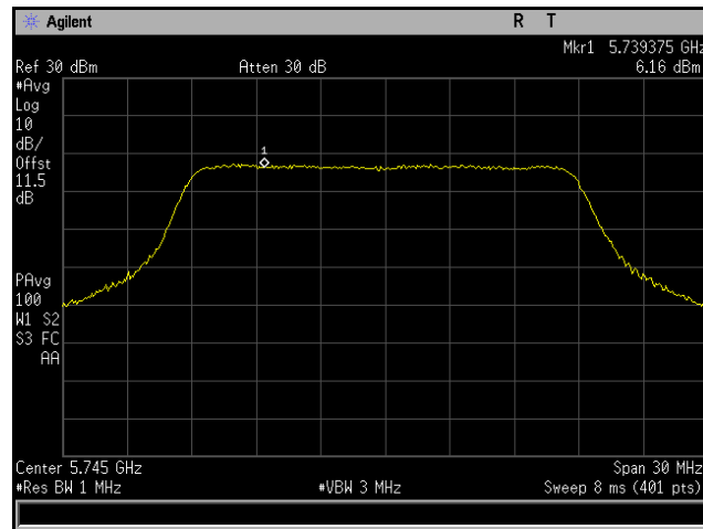
Plot 208. Power Spectral Density, 802.11n 20 MHz, Channel 5745 MHz, 4x8, MCS0 NSS1, CH4
