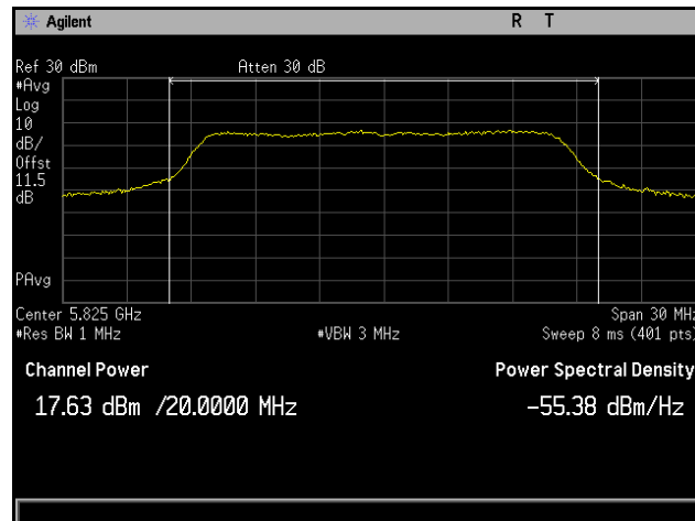
Plot 99. Conducted Output Power, 802.11a 20 MHz, Channel 5825 MHz, 6x8, 6M, CH6
