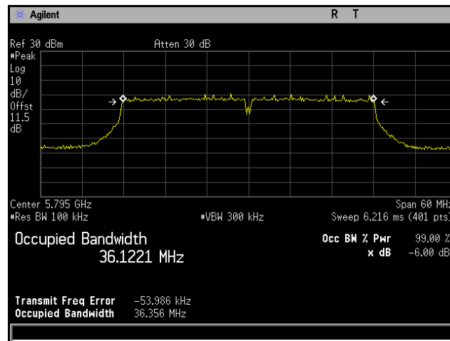
Plot 364. 6 dB Occupied Bandwidth, 802.11ac 40 MHz, Channel 5795 MHz, 4x8, NSS1 MCS0
