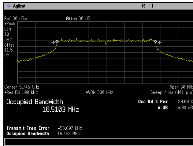
Plot 371. 6 dB Occupied Bandwidth, 802.11a 20 MHz, Channel 5745 MHz, 6x8, 6M
