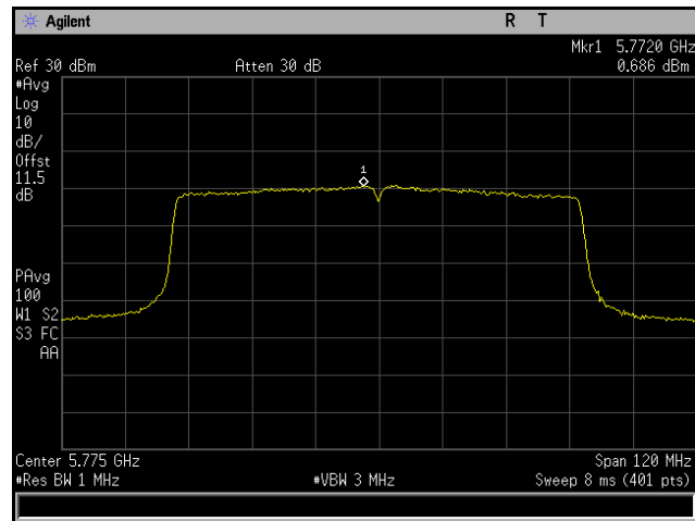
Plot 202. Power Spectral Density, 802.11ac 80 MHz, Channel 5775 MHz, 4x8, MCS0 NSS1, CH4
