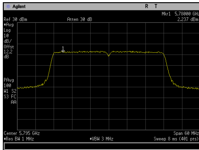
Plot 264. Power Spectral Density, 802.11ac 40 MHz, Channel 5795 MHz, 6x8, MCS0 NSS1, CH3
