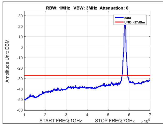
Plot 350. Radiated Spurious Emissions, 802.11ac 80 MHz, Channel 5775 MHz, 6x8, NSS1 MCS0, 1 GHz – 7 GHz
