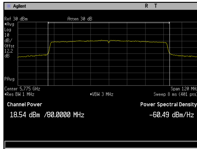
Plot 136. Conducted Output Power, 802.11ac 80 MHz, Channel 5775 MHz, 6x8, MCS0 NSS1, CH5
