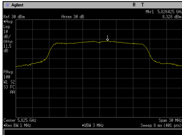
Plot 242. Power Spectral Density, 802.11a 20 MHz, Channel 5825 MHz, 6x8, 6M, CH7
