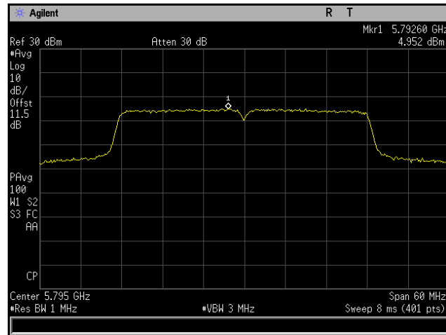
Plot 198. Power Spectral Density, 802.11ac 40 MHz, Channel 5795 MHz, 4x8, MCS0 NSS1, CH5
