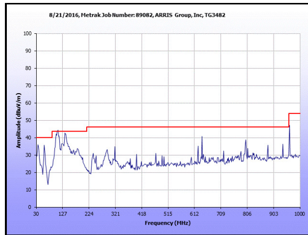
Plot 309. Radiated Spurious Emissions, 30 MHz – 1 GHz, Radio Off
