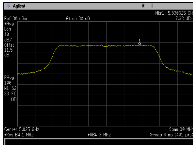
Plot 171. Power Spectral Density, 802.11a 20 MHz, Channel 5825 MHz, 4x8, 6M, CH3
