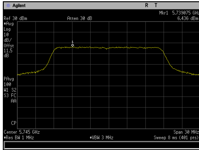
Plot 187. Power Spectral Density, 802.11ac 20 MHz, Channel 5745 MHz, 4x8, MCS0 NSS1, CH5
