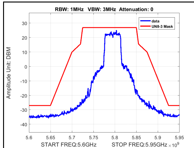
Plot 327. Radiated Spurious Emissions, Mask, 802.11ac 40 MHz, Channel 5795 MHz, 6x8, NSS1 MCS0
