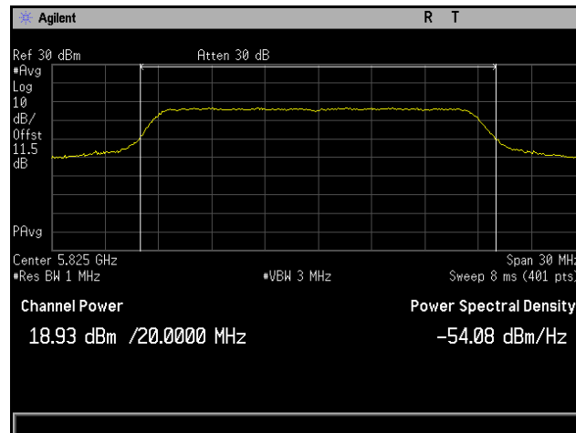
Plot 49. Conducted Output Power, 802.11ac 20 MHz, Channel 5825 MHz, 4x8, MCS0 NSS1, CH5
