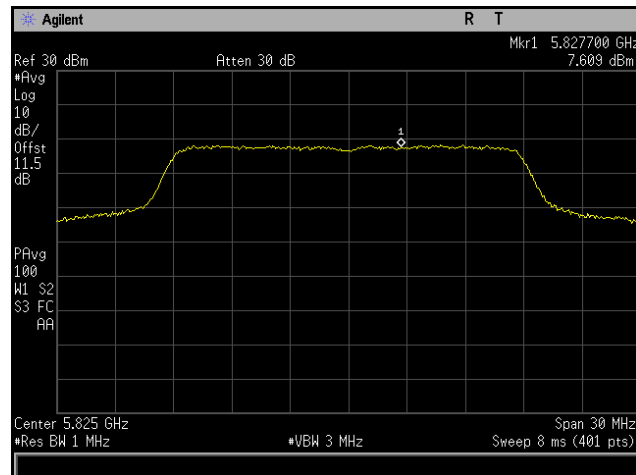
Plot 216. Power Spectral Density, 802.11n 20 MHz, Channel 5825 MHz, 4x8, MCS0 NSS1, CH6
