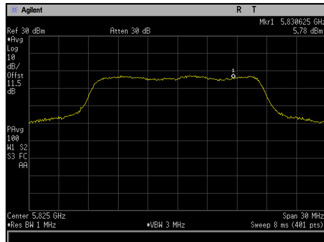
Plot 177. Power Spectral Density, 802.11a 20 MHz, Channel 5825 MHz, 4x8, 6M, CH5
