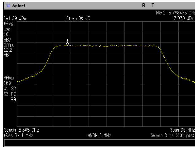
Plot 283. Power Spectral Density, 802.11n 20 MHz, Channel 5805 MHz, 6x8, MCS0 NSS1, CH3
