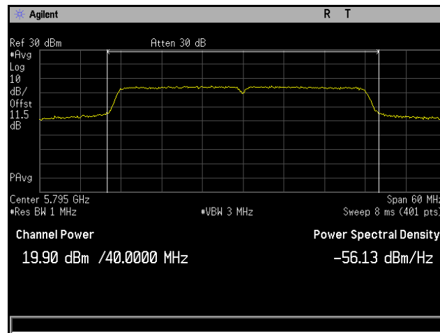
Plot 82. Conducted Output Power, 802.11n 40 MHz, Channel 5795 MHz, 4x8, MCS0 NSS1, CH5
