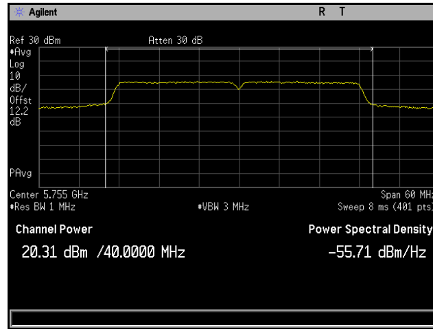
Plot 165. Conducted Output Power, 802.11n 40 MHz, Channel 5755 MHz, 6x8, MCS0 NSS1, CH6
