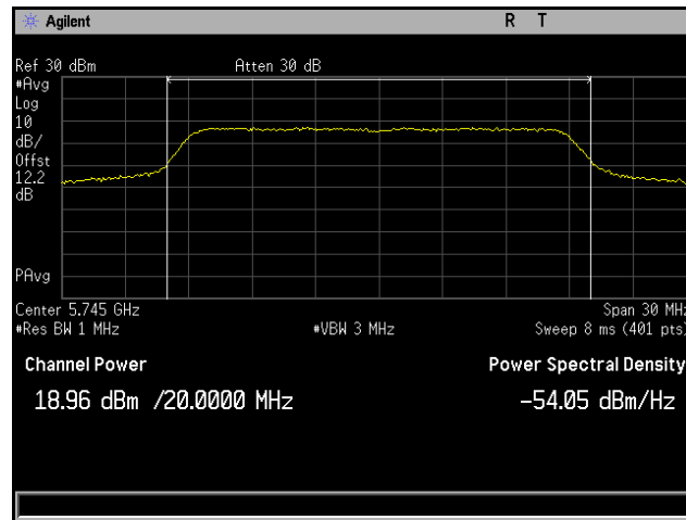
Plot 115. Conducted Output Power, 802.11ac 20 MHz, Channel 5745 MHz, 6x8, MCS0 NSS1, CH6
