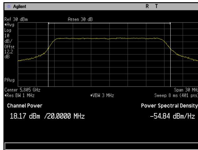
Plot 140. Conducted Output Power, 802.11n 20 MHz, Channel 5805 MHz, 6x8, MCS0 NSS1, CH2
