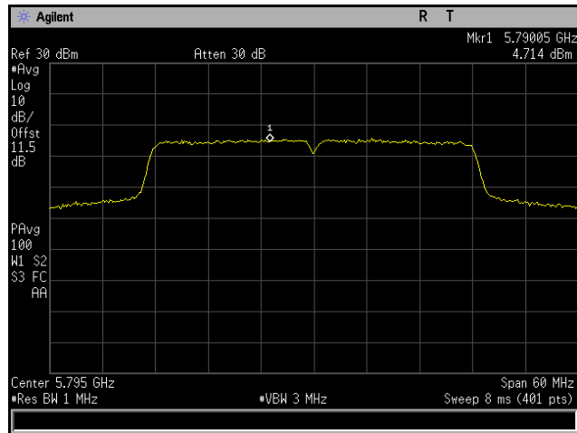
Plot 218. Power Spectral Density, 802.11n 40 MHz, Channel 5795 MHz, 4x8, MCS0 NSS1, CH3
