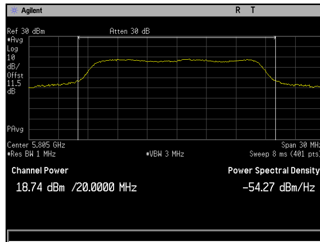
Plot 36. Conducted Output Power, 802.11a 20 MHz, Channel 5805 MHz, 4x8, 6M, CH5
