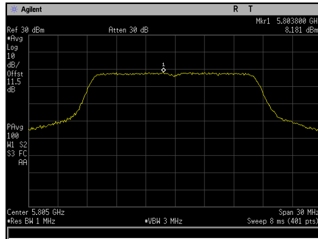
Plot 170. Power Spectral Density, 802.11a 20 MHz, Channel 5805 MHz, 4x8, 6M, CH3
