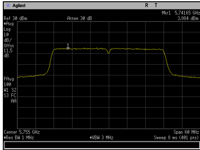
Plot 217. Power Spectral Density, 802.11n 40 MHz, Channel 5755 MHz, 4x8, MCS0 NSS1, CH3
