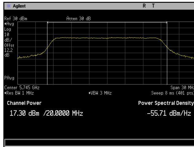
Plot 139. Conducted Output Power, 802.11n 20 MHz, Channel 5745 MHz, 6x8, MCS0 NSS1, CH2
