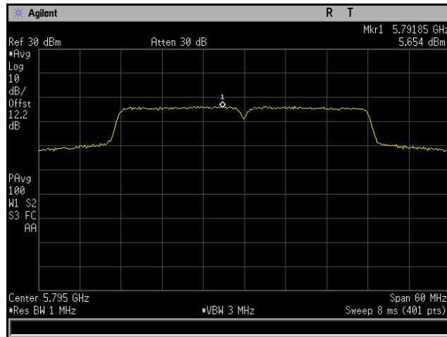
Plot 306. Power Spectral Density, 802.11n 40 MHz, Channel 5795 MHz, 6x8, MCS0 NSS1, CH6
