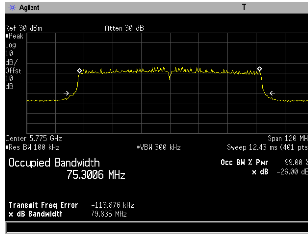
Plot 9. 26 dB Occupied Bandwidth, 802.11ac 80 MHz, Channel 5775 MHz, 4x8, NSS1 MCS0
