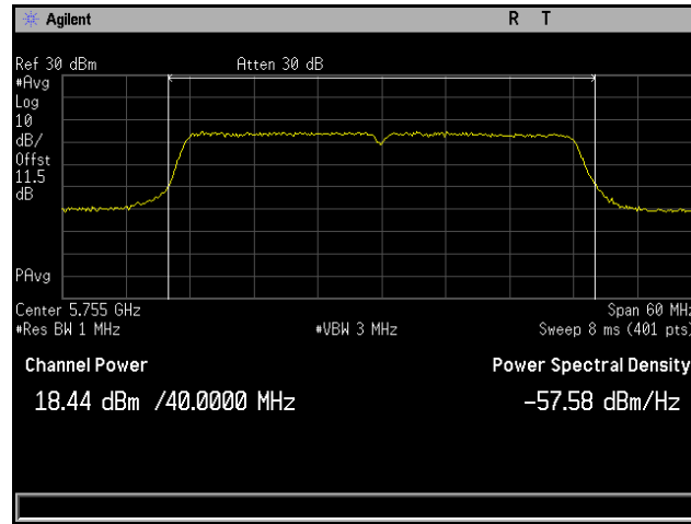
Plot 77. Conducted Output Power, 802.11n 40 MHz, Channel 5755 MHz, 4x8, MCS0 NSS1, CH3
