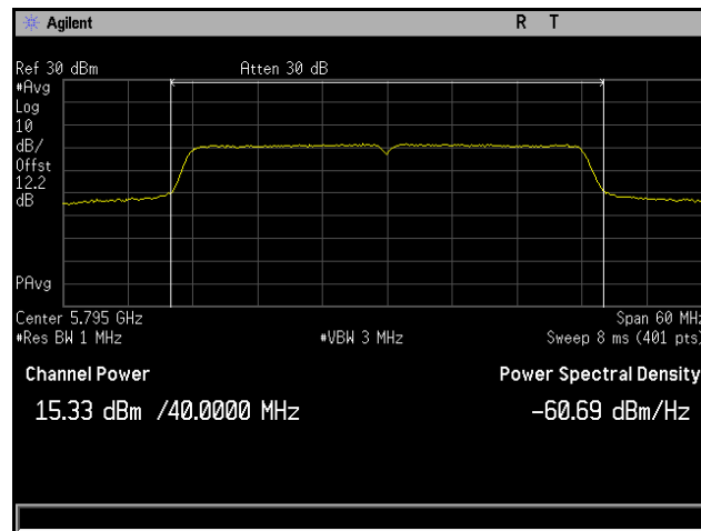
Plot 122. Conducted Output Power, 802.11ac 40 MHz, Channel 5795 MHz, 6x8, MCS0 NSS1, CH2
