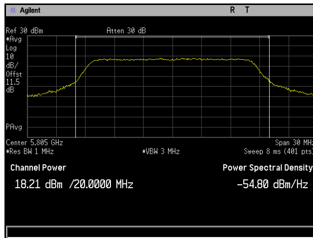
Plot 30. Conducted Output Power, 802.11a 20 MHz, Channel 5805 MHz, 4x8, 6M, CH3
