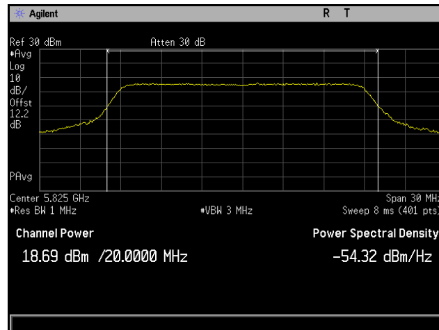
Plot 147. Conducted Output Power, 802.11n 20 MHz, Channel 5825 MHz, 6x8, MCS0 NSS1, CH4
