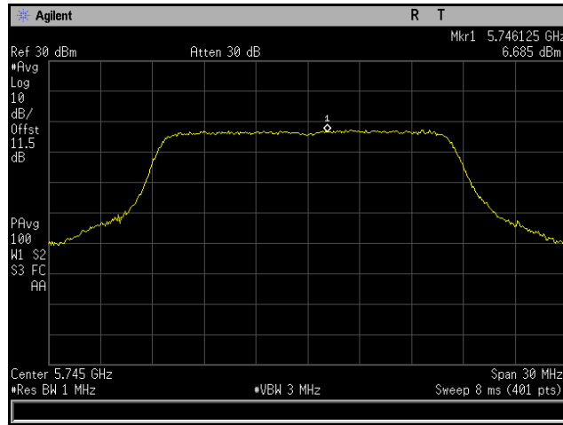
Plot 231. Power Spectral Density, 802.11a 20 MHz, Channel 5745 MHz, 6x8, 6M, CH4
