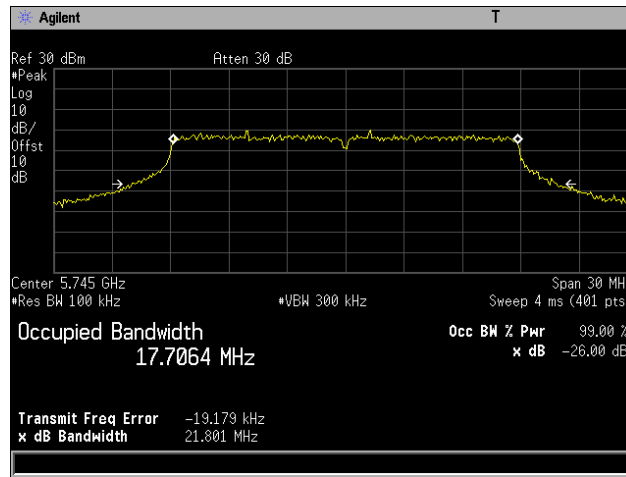
Plot 24. 26 dB Occupied Bandwidth, 802.11n 20 MHz, Channel 5745 MHz, 6x8, MCS0
