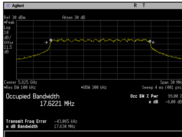
Plot 376. 6 dB Occupied Bandwidth, 802.11ac 20 MHz, Channel 5825 MHz, 6x8, NSS1 MCS0
