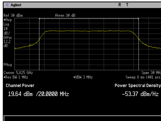
Plot 144. Conducted Output Power, 802.11n 20 MHz, Channel 5825 MHz, 6x8, MCS0 NSS1, CH3
