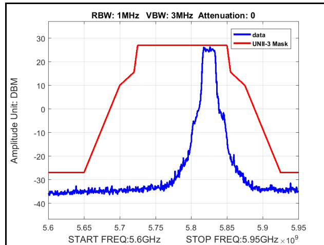
Plot 330. Radiated Spurious Emissions, Mask, 802.11n 20 MHz, Channel 5825 MHz, 6x8, MCS0
