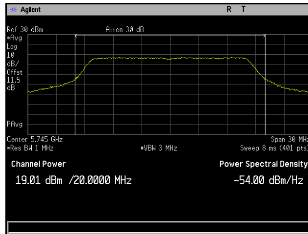
Plot 88. Conducted Output Power, 802.11a 20 MHz, Channel 5745 MHz, 6x8, 6M, CH3
