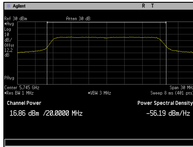
Plot 118. Conducted Output Power, 802.11ac 20 MHz, Channel 5745 MHz, 6x8, MCS0 NSS1, CH7
