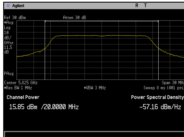
Plot 93. Conducted Output Power, 802.11a 20 MHz, Channel 5825 MHz, 6x8, 6M, CH4
