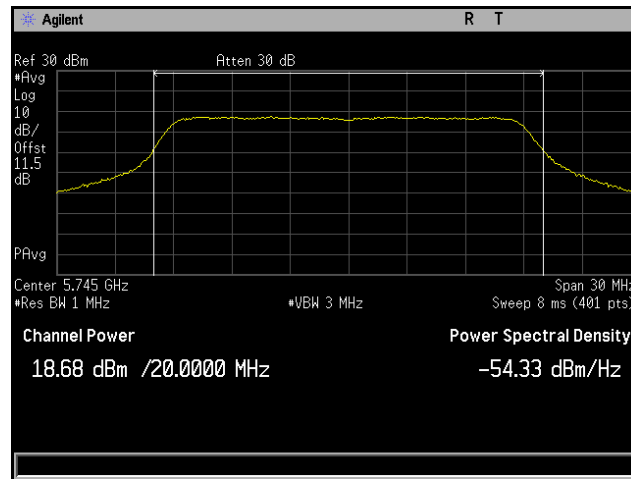
Plot 68. Conducted Output Power, 802.11n 20 MHz, Channel 5745 MHz, 4x8, MCS0 NSS1, CH4
