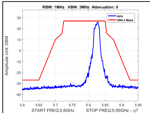
Plot 312. Radiated Spurious Emissions, Mask, 802.11a 20 MHz, Channel 5825 MHz, 4x8, 6M
