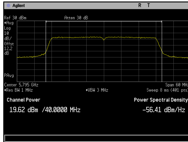
Plot 160. Conducted Output Power, 802.11n 40 MHz, Channel 5795 MHz, 6x8, MCS0 NSS1, CH3
