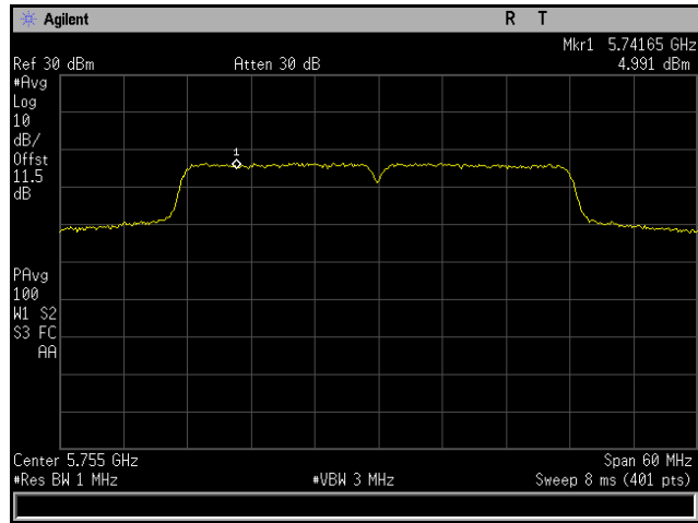
Plot 223. Power Spectral Density, 802.11n 40 MHz, Channel 5755 MHz, 4x8, MCS0 NSS1, CH6
