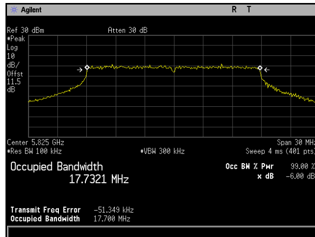
Plot 362. 6 dB Occupied Bandwidth, 802.11ac 20 MHz, Channel 5825 MHz, 4x8, NSS1 MCS0
