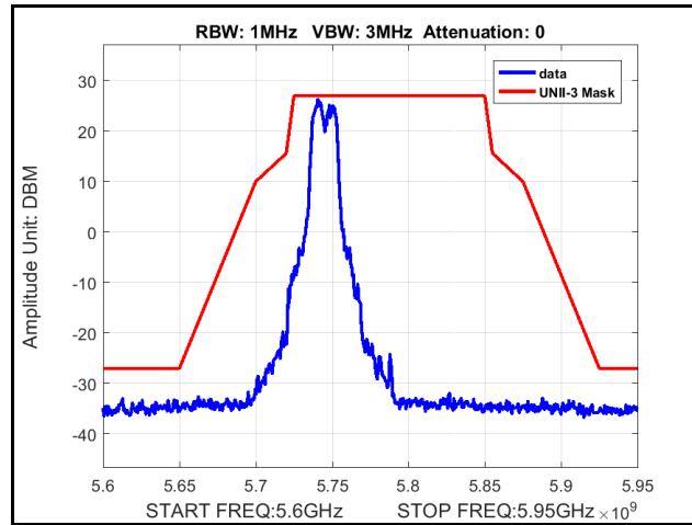
Plot 311. Radiated Spurious Emissions, Mask, 802.11a 20 MHz, Channel 5745 MHz, 4x8, 6M
