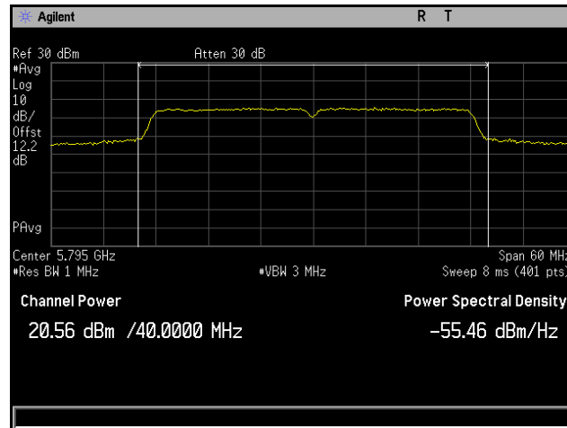
Plot 166. Conducted Output Power, 802.11n 40 MHz, Channel 5795 MHz, 6x8, MCS0 NSS1, CH6
