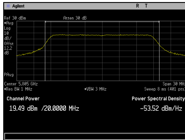
Plot 143. Conducted Output Power, 802.11n 20 MHz, Channel 5805 MHz, 6x8, MCS0 NSS1, CH3
