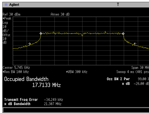
Plot 10. 26 dB Occupied Bandwidth, 802.11n 20 MHz, Channel 5745 MHz, 4x8, MCS0
