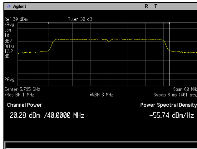
Plot 128. Conducted Output Power, 802.11ac 40 MHz, Channel 5795 MHz, 6x8, MCS0 NSS1, CH5
