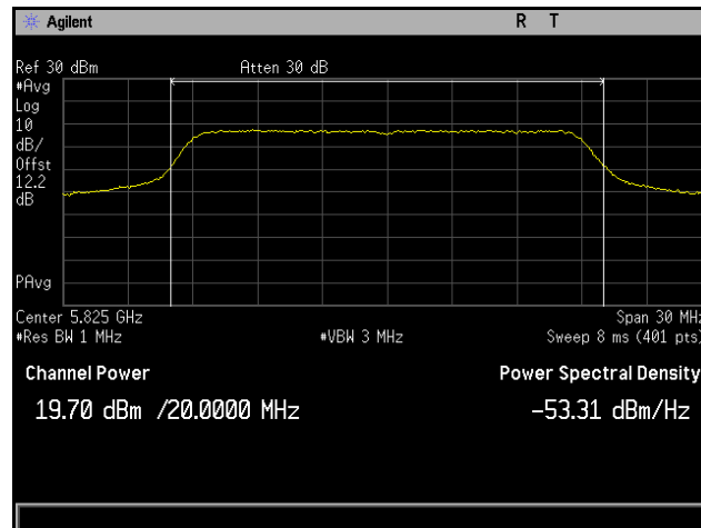
Plot 111. Conducted Output Power, 802.11ac 20 MHz, Channel 5825 MHz, 6x8, MCS0 NSS1, CH4
