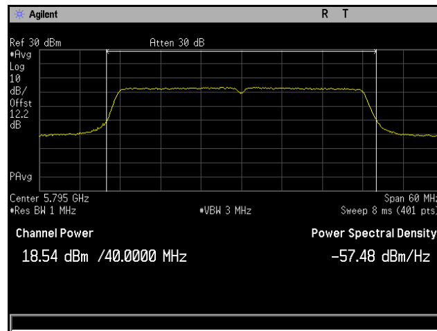
Plot 126. Conducted Output Power, 802.11ac 40 MHz, Channel 5795 MHz, 6x8, MCS0 NSS1, CH4
