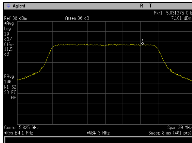
Plot 186. Power Spectral Density, 802.11ac 20 MHz, Channel 5825 MHz, 4x8, MCS0 NSS1, CH4
