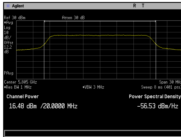
Plot 104. Conducted Output Power, 802.11ac 20 MHz, Channel 5805 MHz, 6x8, MCS0 NSS1, CH2
