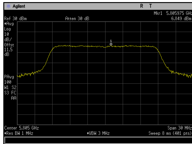
Plot 206. Power Spectral Density, 802.11n 20 MHz, Channel 5805 MHz, 4x8, MCS0 NSS1, CH3
