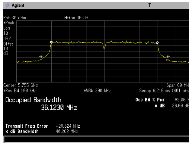
Plot 27. 26 dB Occupied Bandwidth, 802.11n 40 MHz, Channel 5755 MHz, 6x8, MCS0
