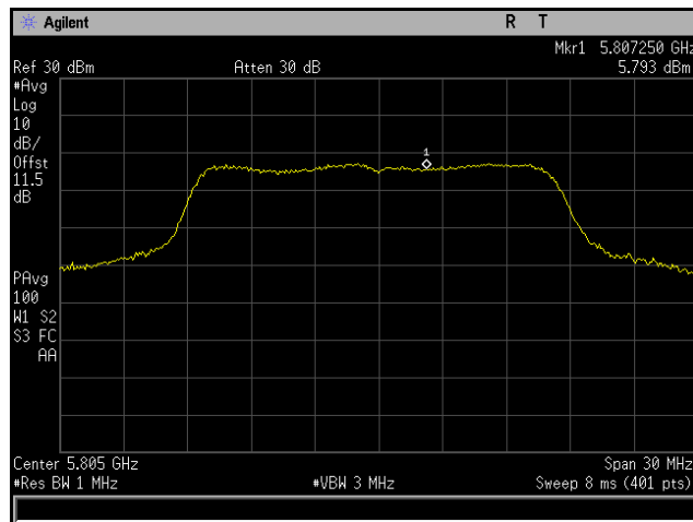
Plot 238. Power Spectral Density, 802.11a 20 MHz, Channel 5805 MHz, 6x8, 6M, CH6
