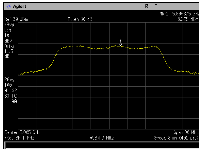
Plot 176. Power Spectral Density, 802.11a 20 MHz, Channel 5805 MHz, 4x8, 6M, CH5
