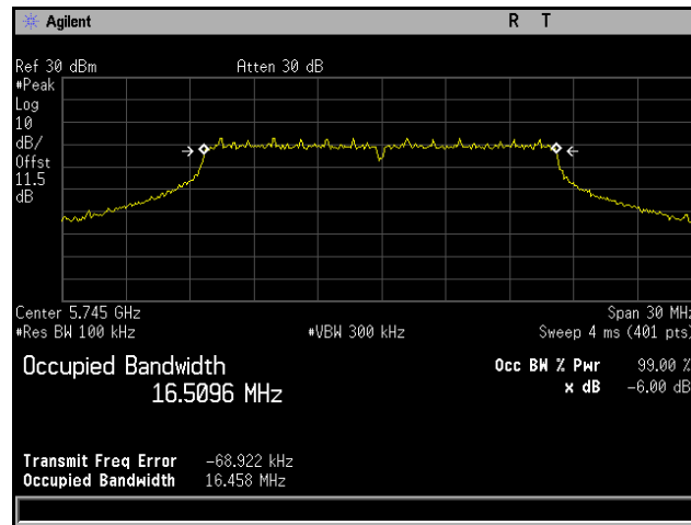
Plot 357. 6 dB Occupied Bandwidth, 802.11a 20 MHz, Channel 5745 MHz, 4x8, 6M
