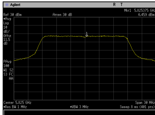
Plot 207. Power Spectral Density, 802.11n 20 MHz, Channel 5825 MHz, 4x8, MCS0 NSS1, CH3
