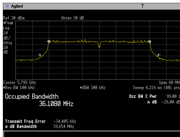
Plot 22. 26 dB Occupied Bandwidth, 802.11ac 40 MHz, Channel 5795 MHz, 6x8, NSS1 MCS0
