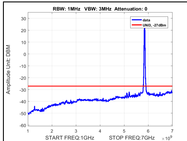
Plot 345. Radiated Spurious Emissions, 802.11a 20 MHz, Channel 5825 MHz, 6x8, 6M, 1 GHz – 7 GHz
