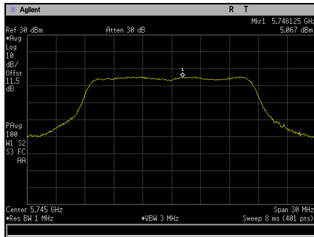
Plot 225. Power Spectral Density, 802.11a 20 MHz, Channel 5745 MHz, 6x8, 6M, CH2
