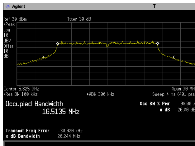
Plot 17. 26 dB Occupied Bandwidth, 802.11a 20 MHz, Channel 5825 MHz, 6x8, 6M
