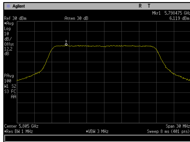
Plot 286. Power Spectral Density, 802.11n 20 MHz, Channel 5805 MHz, 6x8, MCS0 NSS1, CH4
