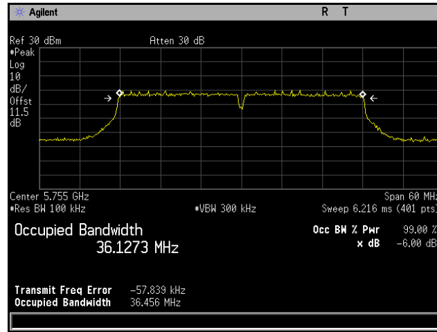
Plot 369. 6 dB Occupied Bandwidth, 802.11n 40 MHz, Channel 5755 MHz, 4x8, MCS0
