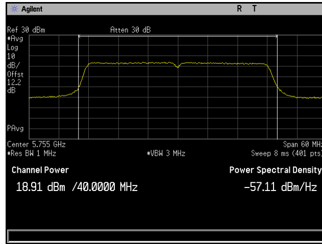
Plot 123. Conducted Output Power, 802.11ac 40 MHz, Channel 5755 MHz, 6x8, MCS0 NSS1, CH3
