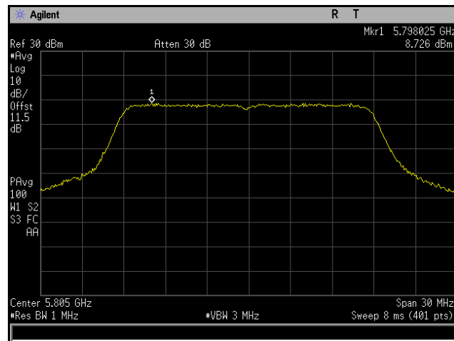
Plot 182. Power Spectral Density, 802.11ac 20 MHz, Channel 5805 MHz, 4x8, MCS0 NSS1, CH3
