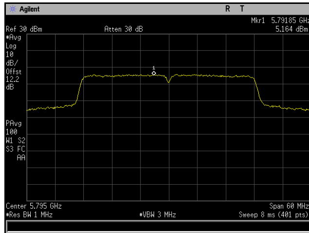
Plot 304. Power Spectral Density, 802.11n 40 MHz, Channel 5795 MHz, 6x8, MCS0 NSS1, CH5
