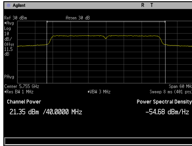
Plot 83. Conducted Output Power, 802.11n 40 MHz, Channel 5755 MHz, 4x8, MCS0 NSS1, CH6
