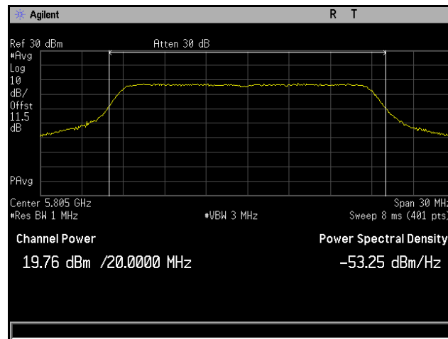
Plot 42. Conducted Output Power, 802.11ac 20 MHz, Channel 5805 MHz, 4x8, MCS0 NSS1, CH3
