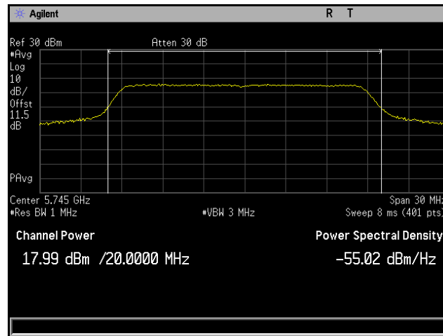
Plot 47. Conducted Output Power, 802.11ac 20 MHz, Channel 5745 MHz, 4x8, MCS0 NSS1, CH5
