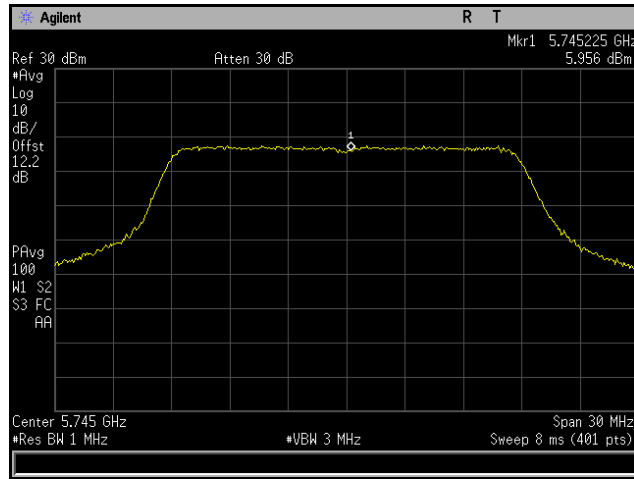
Plot 282. Power Spectral Density, 802.11n 20 MHz, Channel 5745 MHz, 6x8, MCS0 NSS1, CH3
