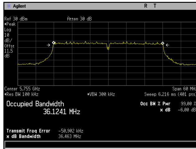
Plot 363. 6 dB Occupied Bandwidth, 802.11ac 40 MHz, Channel 5755 MHz, 4x8, NSS1 MCS0
