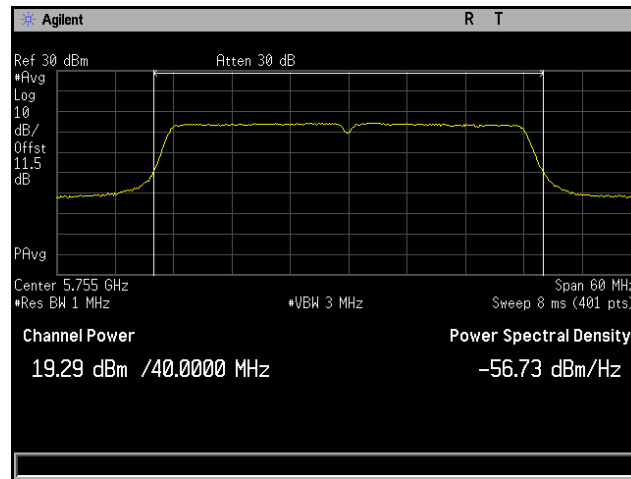
Plot 79. Conducted Output Power, 802.11n 40 MHz, Channel 5755 MHz, 4x8, MCS0 NSS1, CH4
