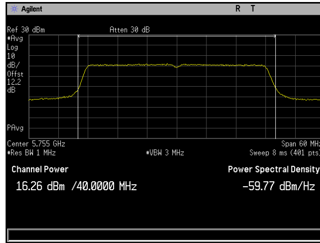
Plot 157. Conducted Output Power, 802.11n 40 MHz, Channel 5755 MHz, 6x8, MCS0 NSS1, CH2
