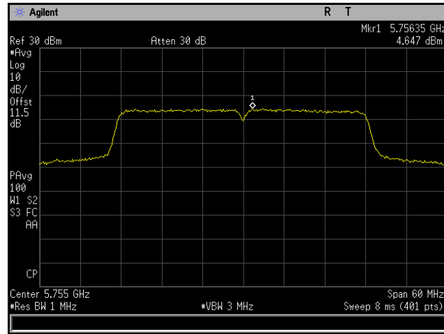
Plot 197. Power Spectral Density, 802.11ac 40 MHz, Channel 5755 MHz, 4x8, MCS0 NSS1, CH5
