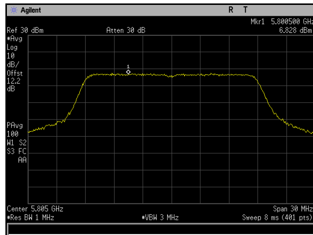
Plot 247. Power Spectral Density, 802.11ac 20 MHz, Channel 5805 MHz, 6x8, MCS0 NSS1, CH3
