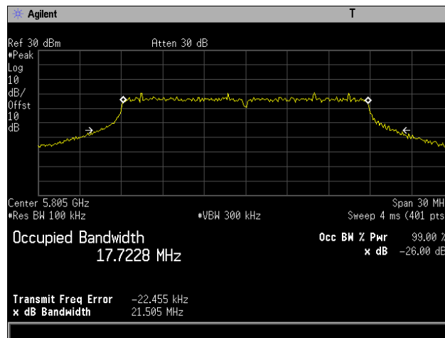
Plot 5. 26 dB Occupied Bandwidth, 802.11ac 20 MHz, Channel 5805 MHz, 4x8, NSS1 MCS0
