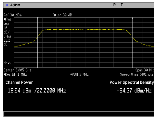
Plot 110. Conducted Output Power, 802.11ac 20 MHz, Channel 5805 MHz, 6x8, MCS0 NSS1, CH4
