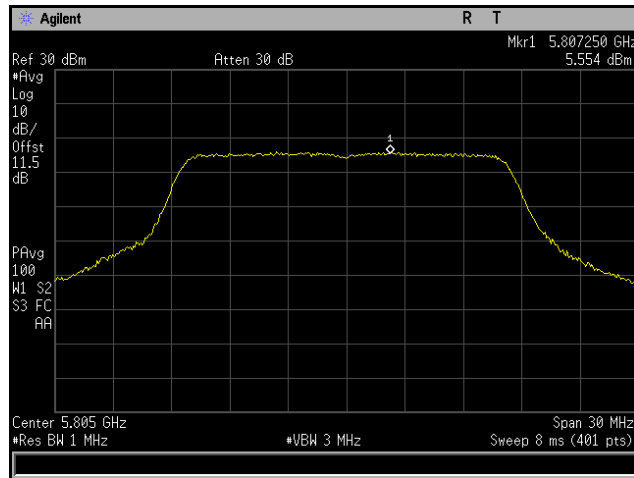
Plot 232. Power Spectral Density, 802.11a 20 MHz, Channel 5805 MHz, 6x8, 6M, CH4
