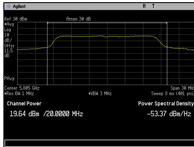
Plot 39. Conducted Output Power, 802.11a 20 MHz, Channel 5805 MHz, 4x8, 6M, CH6
