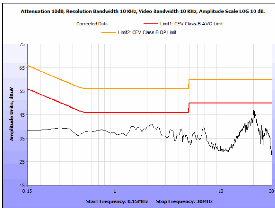
Plot 356. Conducted Emissions, 15.207(a), Neutral Line
