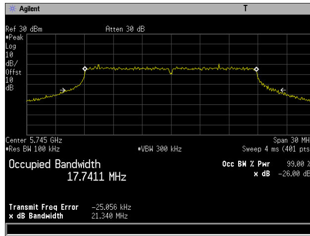
Plot 4. 26 dB Occupied Bandwidth, 802.11ac 20 MHz, Channel 5745 MHz, 4x8, NSS1 MCS0
