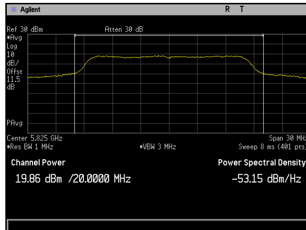
Plot 40. Conducted Output Power, 802.11a 20 MHz, Channel 5825 MHz, 4x8, 6M, CH6
