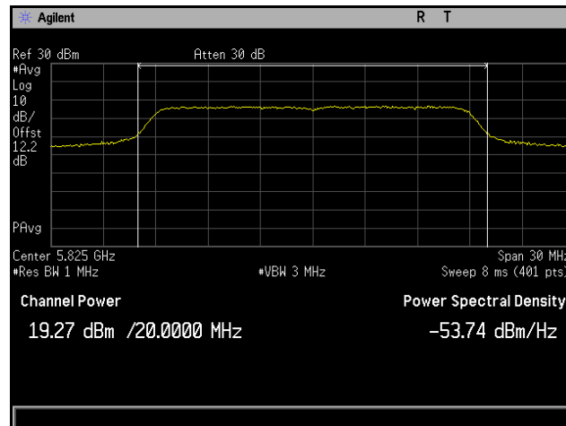
Plot 156. Conducted Output Power, 802.11n 20 MHz, Channel 5825 MHz, 6x8, MCS0 NSS1, CH7
