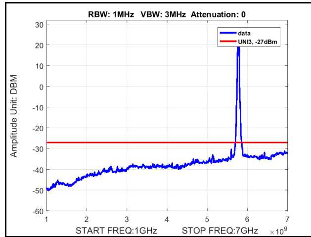
Plot 342. Radiated Spurious Emissions, 802.11n 40 MHz, Channel 5755 MHz, 4x8, MCS0, 1 GHz – 7 GHz
