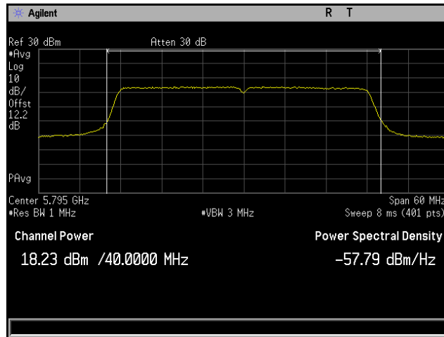
Plot 162. Conducted Output Power, 802.11n 40 MHz, Channel 5795 MHz, 6x8, MCS0 NSS1, CH4
