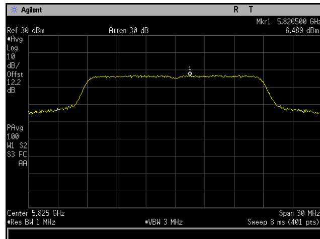
Plot 257. Power Spectral Density, 802.11ac 20 MHz, Channel 5825 MHz, 6x8, MCS0 NSS1, CH6
