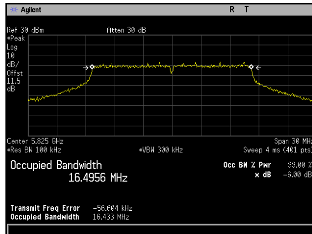
Plot 373. 6 dB Occupied Bandwidth, 802.11a 20 MHz, Channel 5825 MHz, 6x8, 6M
