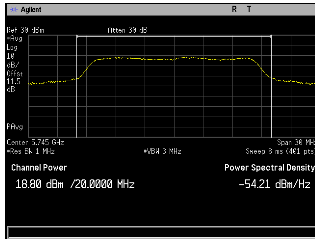
Plot 35. Conducted Output Power, 802.11a 20 MHz, Channel 5745 MHz, 4x8, 6M, CH5
