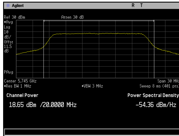
Plot 32. Conducted Output Power, 802.11a 20 MHz, Channel 5745 MHz, 4x8, 6M, CH4
