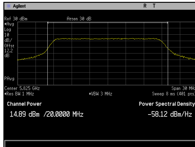
Plot 141. Conducted Output Power, 802.11n 20 MHz, Channel 5825 MHz, 6x8, MCS0 NSS1, CH2
