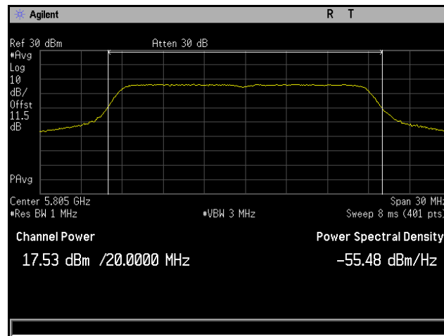
Plot 69. Conducted Output Power, 802.11n 20 MHz, Channel 5805 MHz, 4x8, MCS0 NSS1, CH4
