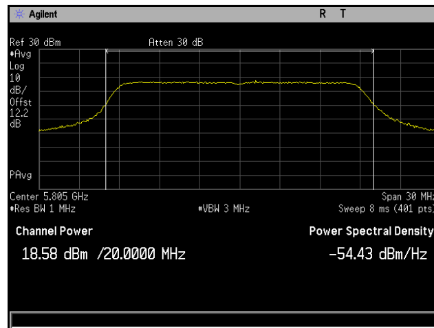
Plot 146. Conducted Output Power, 802.11n 20 MHz, Channel 5805 MHz, 6x8, MCS0 NSS1, CH4
