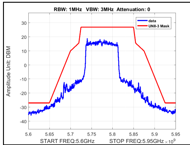
Plot 317. Radiated Spurious Emissions, Mask, 802.11ac 80 MHz, Channel 5775 MHz, 4x8, NSS1 MCS0
