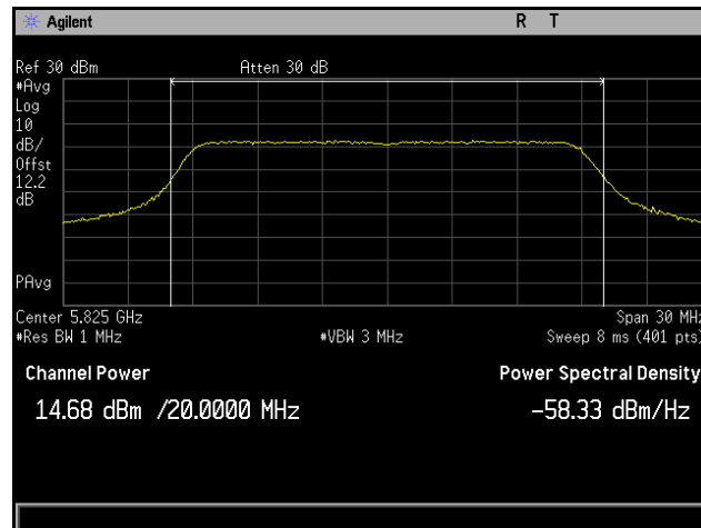
Plot 117. Conducted Output Power, 802.11ac 20 MHz, Channel 5825 MHz, 6x8, MCS0 NSS1, CH6
