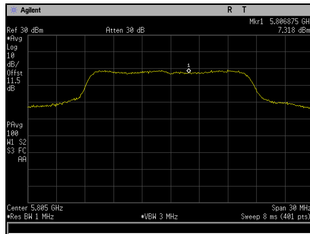
Plot 179. Power Spectral Density, 802.11a 20 MHz, Channel 5805 MHz, 4x8, 6M, CH6
