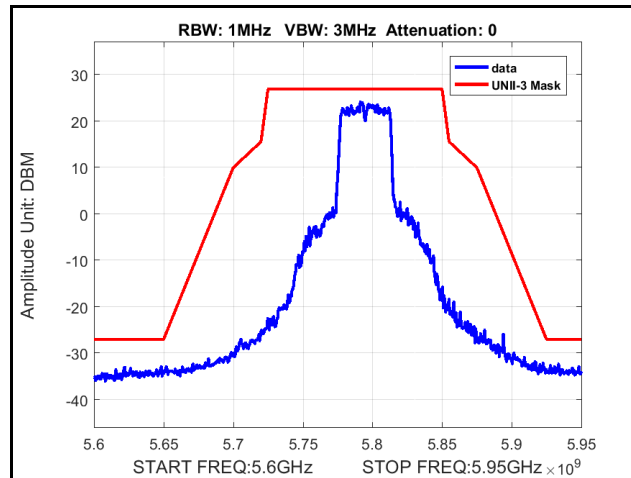
Plot 332. Radiated Spurious Emissions, Mask, 802.11n 40 MHz, Channel 5795 MHz, 6x8, MCS0
