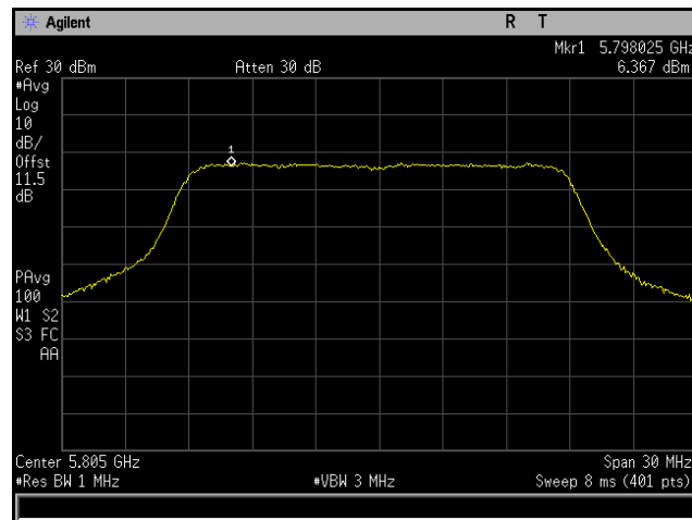
Plot 185. Power Spectral Density, 802.11ac 20 MHz, Channel 5805 MHz, 4x8, MCS0 NSS1, CH4
