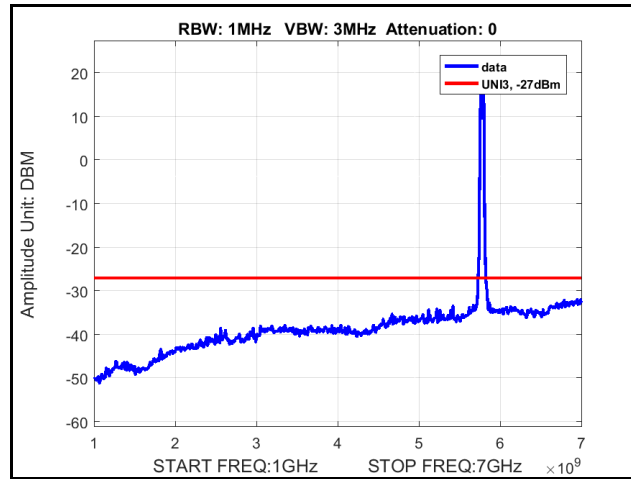
Plot 353. Radiated Spurious Emissions, 802.11n 40 MHz, Channel 5755 MHz, 6x8, MCS0, 1 GHz – 7 GHz
