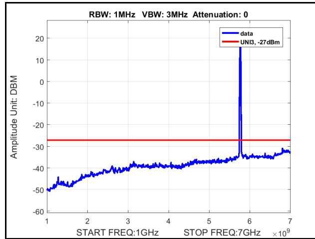
Plot 335. Radiated Spurious Emissions, 802.11ac 20 MHz, Channel 5745 MHz, 4x8, NSS1 MCS0, 1 GHz – 7 GHz
