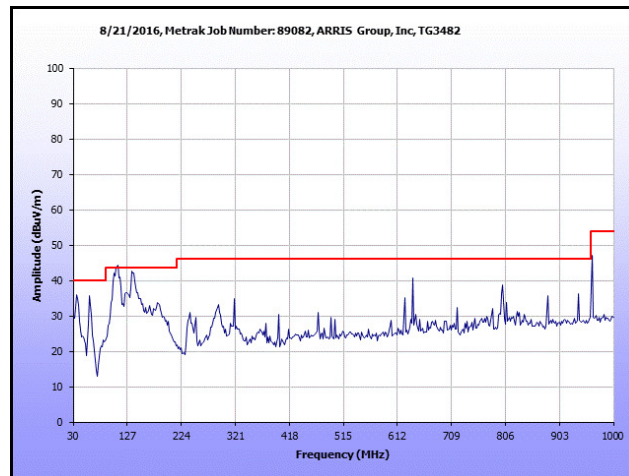
Plot 310. Radiated Spurious Emissions, 30 MHz – 1 GHz, Radio On
