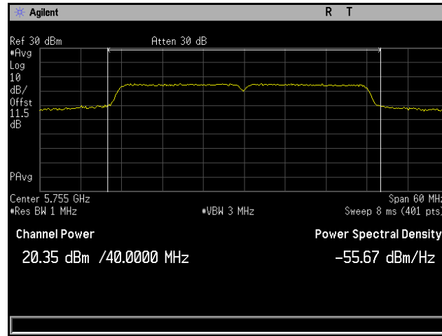
Plot 59. Conducted Output Power, 802.11ac 40 MHz, Channel 5755 MHz, 4x8, MCS0 NSS1, CH6
