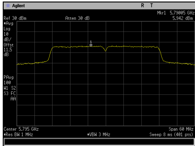
Plot 224. Power Spectral Density, 802.11n 40 MHz, Channel 5795 MHz, 4x8, MCS0 NSS1, CH6
