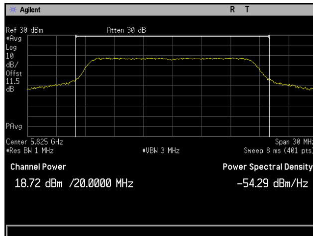
Plot 31. Conducted Output Power, 802.11a 20 MHz, Channel 5825 MHz, 4x8, 6M, CH3
