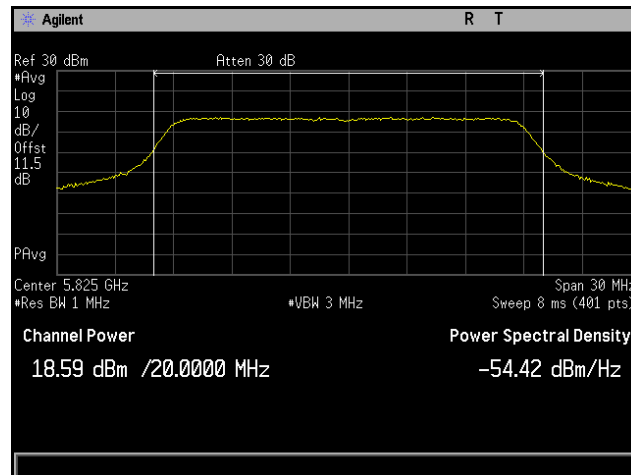
Plot 46. Conducted Output Power, 802.11ac 20 MHz, Channel 5825 MHz, 4x8, MCS0 NSS1, CH4
