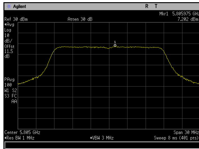
Plot 209. Power Spectral Density, 802.11n 20 MHz, Channel 5805 MHz, 4x8, MCS0 NSS1, CH4
