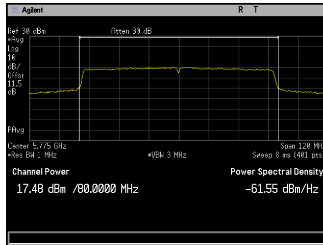
Plot 64. Conducted Output Power, 802.11ac 80 MHz, Channel 5775 MHz, 4x8, MCS0 NSS1, CH6
