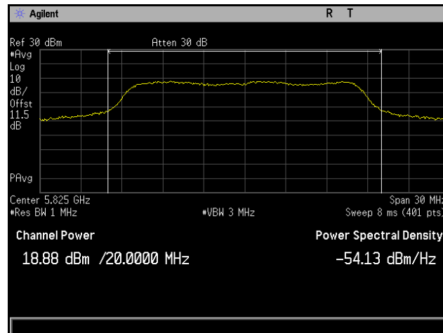
Plot 37. Conducted Output Power, 802.11a 20 MHz, Channel 5825 MHz, 4x8, 6M, CH5
