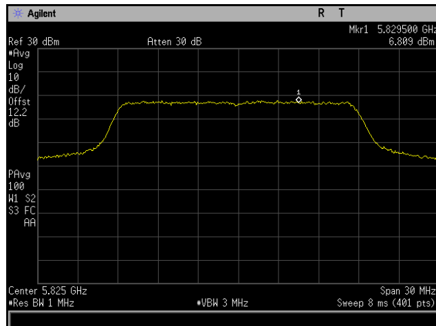
Plot 290. Power Spectral Density, 802.11n 20 MHz, Channel 5825 MHz, 6x8, MCS0 NSS1, CH5
