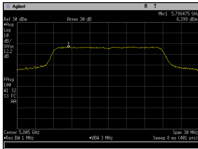
Plot 292. Power Spectral Density, 802.11n 20 MHz, Channel 5805 MHz, 6x8, MCS0 NSS1, CH6
