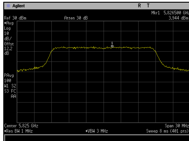
Plot 254. Power Spectral Density, 802.11ac 20 MHz, Channel 5825 MHz, 6x8, MCS0 NSS1, CH5
