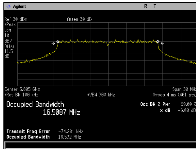
Plot 358. 6 dB Occupied Bandwidth, 802.11a 20 MHz, Channel 5805 MHz, 4x8, 6M
