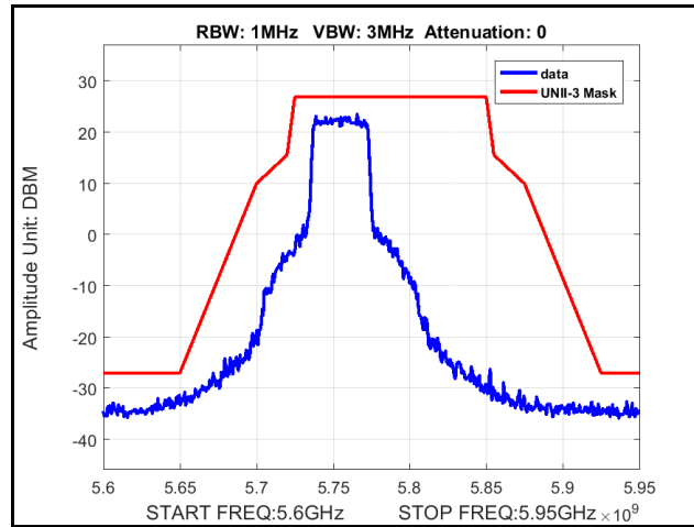
Plot 331. Radiated Spurious Emissions, Mask, 802.11n 40 MHz, Channel 5755 MHz, 6x8, MCS0
