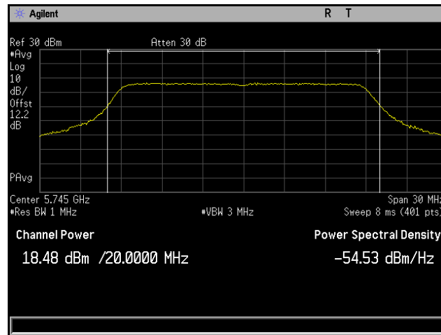
Plot 109. Conducted Output Power, 802.11ac 20 MHz, Channel 5745 MHz, 6x8, MCS0 NSS1, CH4
