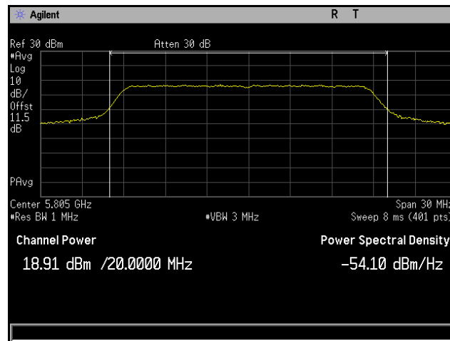
Plot 72. Conducted Output Power, 802.11n 20 MHz, Channel 5805 MHz, 4x8, MCS0 NSS1, CH5
