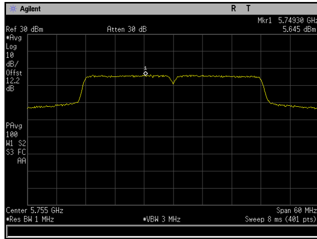
Plot 305. Power Spectral Density, 802.11n 40 MHz, Channel 5755 MHz, 6x8, MCS0 NSS1, CH6
