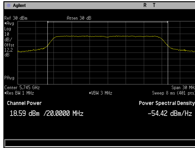
Plot 148. Conducted Output Power, 802.11n 20 MHz, Channel 5745 MHz, 6x8, MCS0 NSS1, CH5
