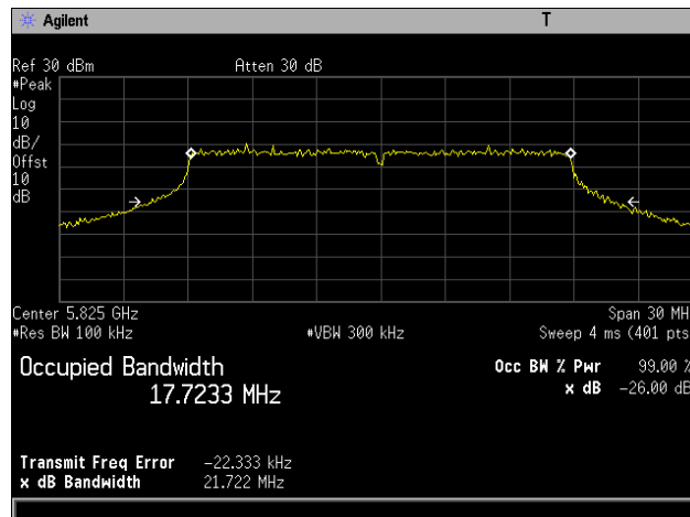
Plot 6. 26 dB Occupied Bandwidth, 802.11ac 20 MHz, Channel 5825 MHz, 4x8, NSS1 MCS0
