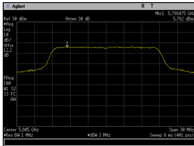
Plot 289. Power Spectral Density, 802.11n 20 MHz, Channel 5805 MHz, 6x8, MCS0 NSS1, CH5
