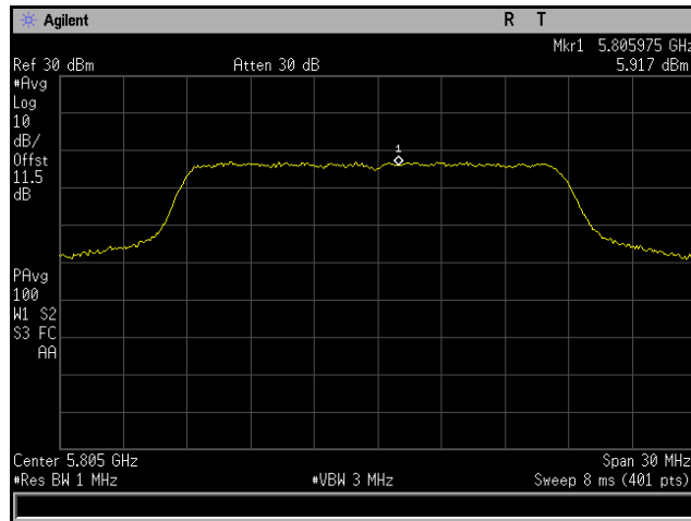
Plot 212. Power Spectral Density, 802.11n 20 MHz, Channel 5805 MHz, 4x8, MCS0 NSS1, CH5
