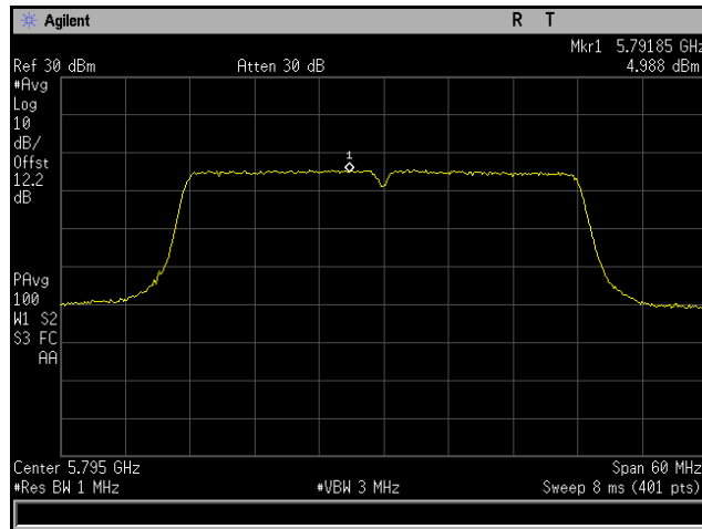
Plot 300. Power Spectral Density, 802.11n 40 MHz, Channel 5795 MHz, 6x8, MCS0 NSS1, CH3
