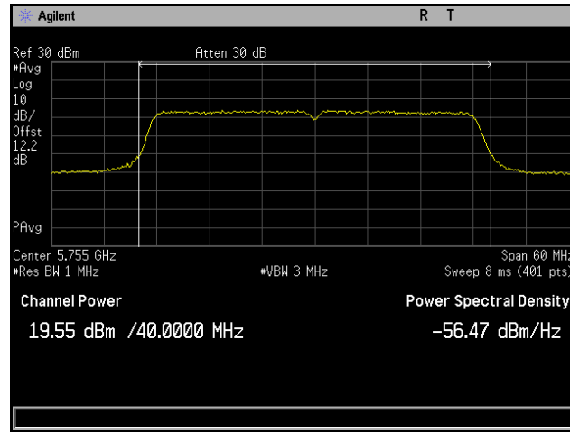
Plot 159. Conducted Output Power, 802.11n 40 MHz, Channel 5755 MHz, 6x8, MCS0 NSS1, CH3
