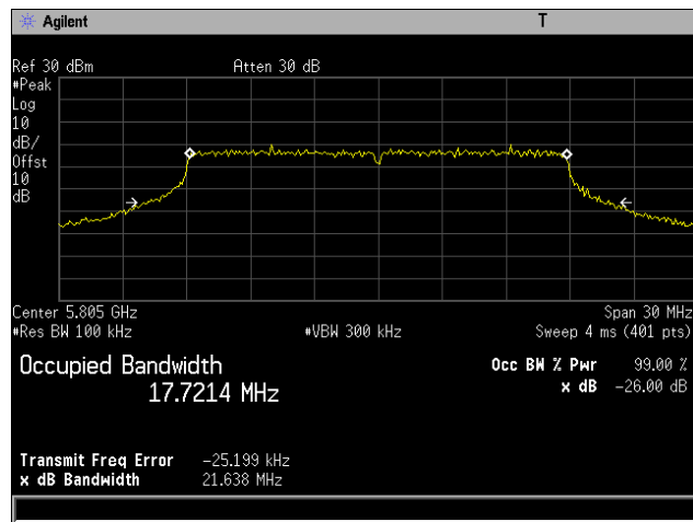
Plot 25. 26 dB Occupied Bandwidth, 802.11n 20 MHz, Channel 5805 MHz, 6x8, MCS0
