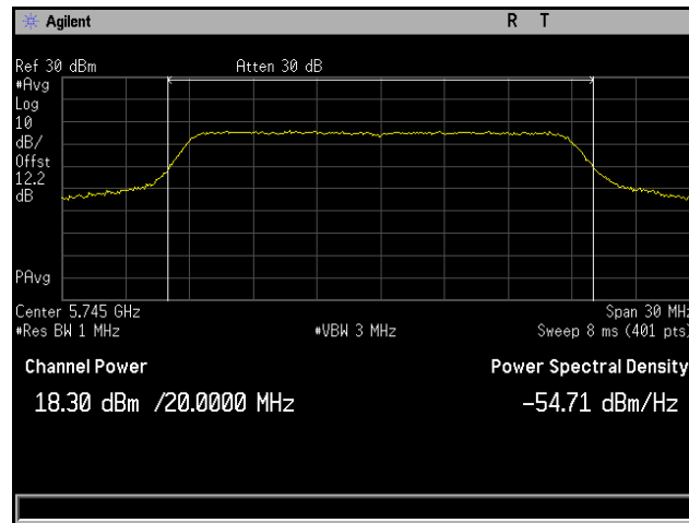
Plot 112. Conducted Output Power, 802.11ac 20 MHz, Channel 5745 MHz, 6x8, MCS0 NSS1, CH5
