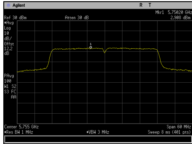
Plot 271. Power Spectral Density, 802.11ac 40 MHz, Channel 5755 MHz, 6x8, MCS0 NSS1, CH7
