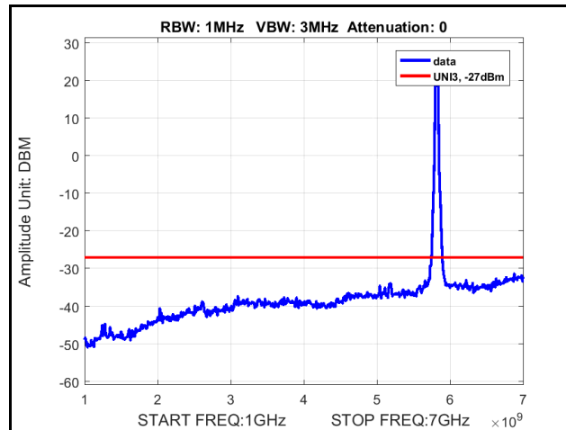
Plot 343. Radiated Spurious Emissions, 802.11n 40 MHz, Channel 5795 MHz, 4x8, MCS0, 1 GHz – 7 GHz
