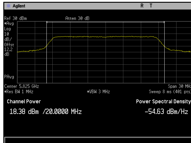
Plot 150. Conducted Output Power, 802.11n 20 MHz, Channel 5825 MHz, 6x8, MCS0 NSS1, CH5
