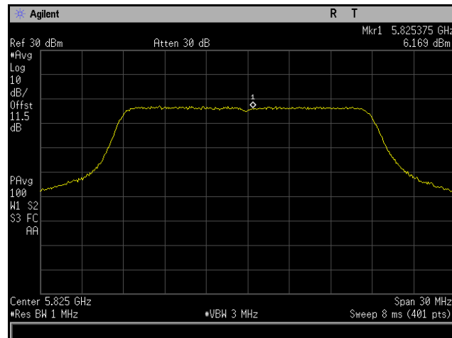
Plot 210. Power Spectral Density, 802.11n 20 MHz, Channel 5825 MHz, 4x8, MCS0 NSS1, CH4
