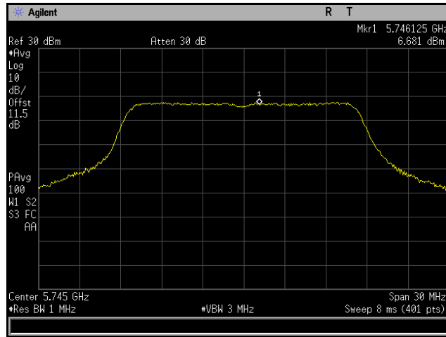
Plot 228. Power Spectral Density, 802.11a 20 MHz, Channel 5745 MHz, 6x8, 6M, CH3
