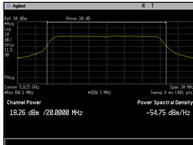
Plot 70. Conducted Output Power, 802.11n 20 MHz, Channel 5825 MHz, 4x8, MCS0 NSS1, CH4
