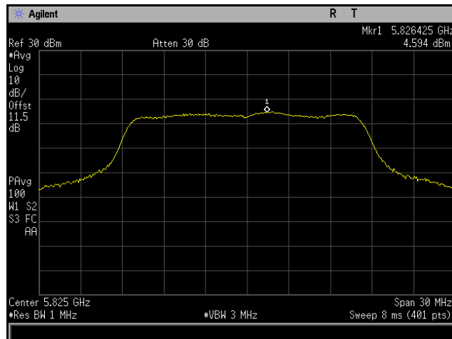
Plot 227. Power Spectral Density, 802.11a 20 MHz, Channel 5825 MHz, 6x8, 6M, CH2
