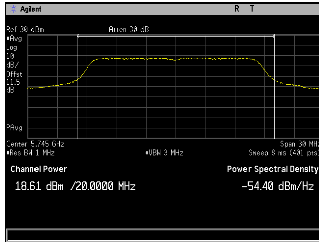
Plot 29. Conducted Output Power, 802.11a 20 MHz, Channel 5745 MHz, 4x8, 6M, CH3
