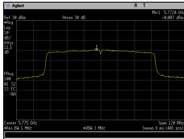
Plot 203. Power Spectral Density, 802.11ac 80 MHz, Channel 5775 MHz, 4x8, MCS0 NSS1, CH5
