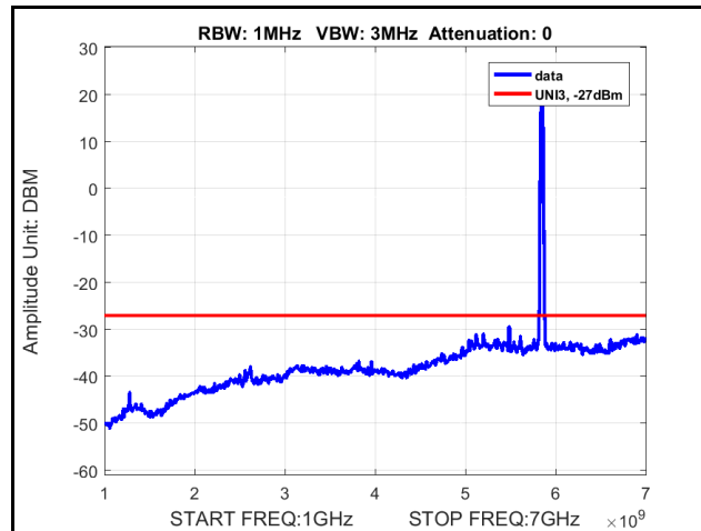
Plot 347. Radiated Spurious Emissions, 802.11ac 20 MHz, Channel 5825 MHz, 6x8, NSS1 MCS0, 1 GHz – 7 GHz
