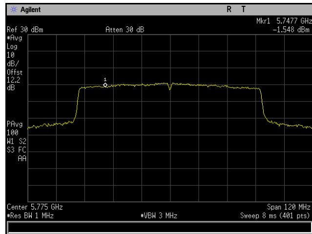
Plot 276. Power Spectral Density, 802.11ac 80 MHz, Channel 5775 MHz, 6x8, MCS0 NSS1, CH5
