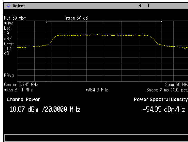
Plot 38. Conducted Output Power, 802.11a 20 MHz, Channel 5745 MHz, 4x8, 6M, CH6
