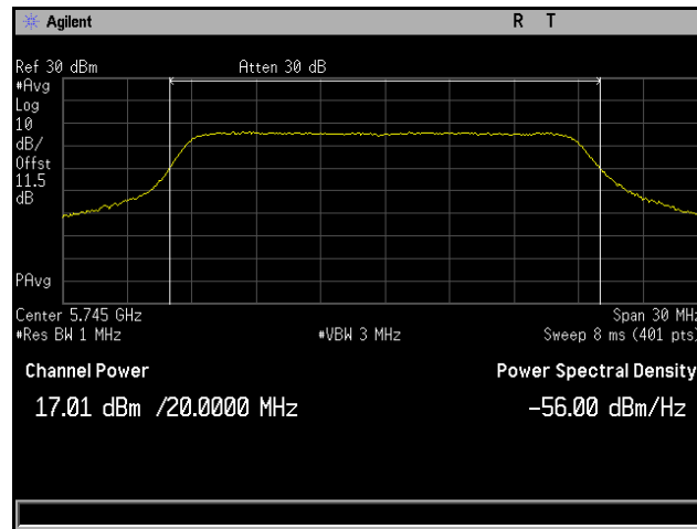
Plot 44. Conducted Output Power, 802.11ac 20 MHz, Channel 5745 MHz, 4x8, MCS0 NSS1, CH4
