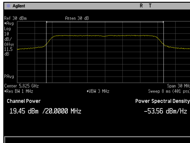
Plot 76. Conducted Output Power, 802.11n 20 MHz, Channel 5825 MHz, 4x8, MCS0 NSS1, CH6
