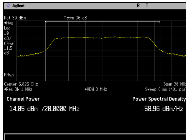
Plot 87. Conducted Output Power, 802.11a 20 MHz, Channel 5825 MHz, 6x8, 6M, CH2
