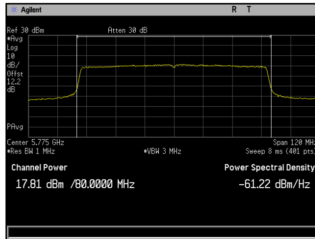
Plot 133. Conducted Output Power, 802.11ac 80 MHz, Channel 5775 MHz, 6x8, MCS0 NSS1, CH2
