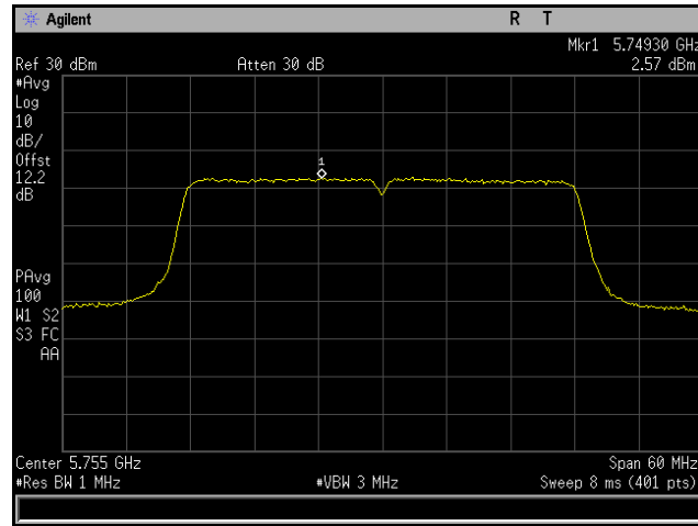
Plot 297. Power Spectral Density, 802.11n 40 MHz, Channel 5755 MHz, 6x8, MCS0 NSS1, CH2
