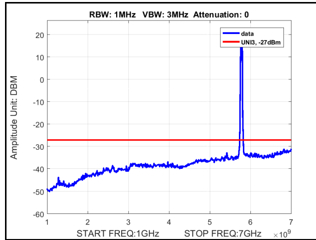
Plot 337. Radiated Spurious Emissions, 802.11ac 40 MHz, Channel 5755 MHz, 4x8, NSS1 MCS0, 1 GHz – 7 GHz
