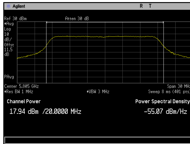
Plot 45. Conducted Output Power, 802.11ac 20 MHz, Channel 5805 MHz, 4x8, MCS0 NSS1, CH4
