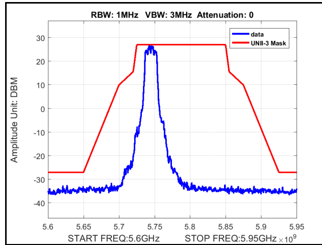
Plot 322. Radiated Spurious Emissions, Mask, 802.11a 20 MHz, Channel 5745 MHz, 6x8, 6M
