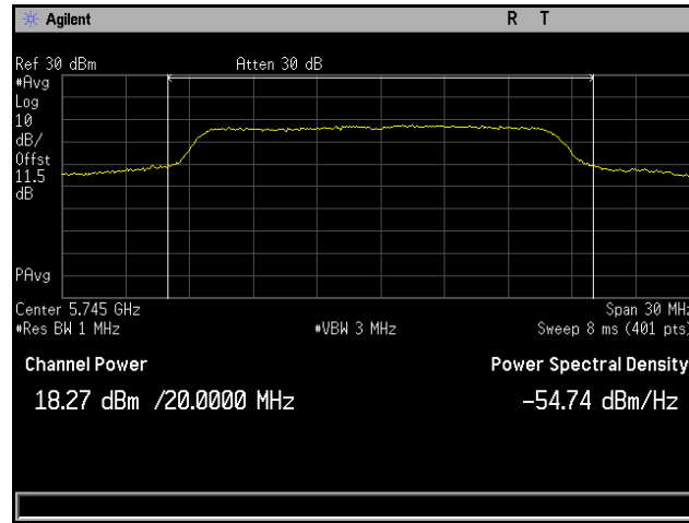
Plot 100. Conducted Output Power, 802.11a 20 MHz, Channel 5745 MHz, 6x8, 6M, CH7
