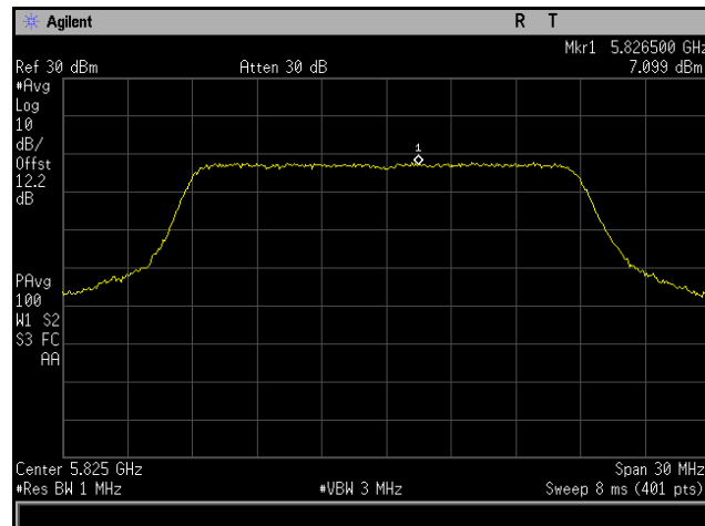
Plot 248. Power Spectral Density, 802.11ac 20 MHz, Channel 5825 MHz, 6x8, MCS0 NSS1, CH3
