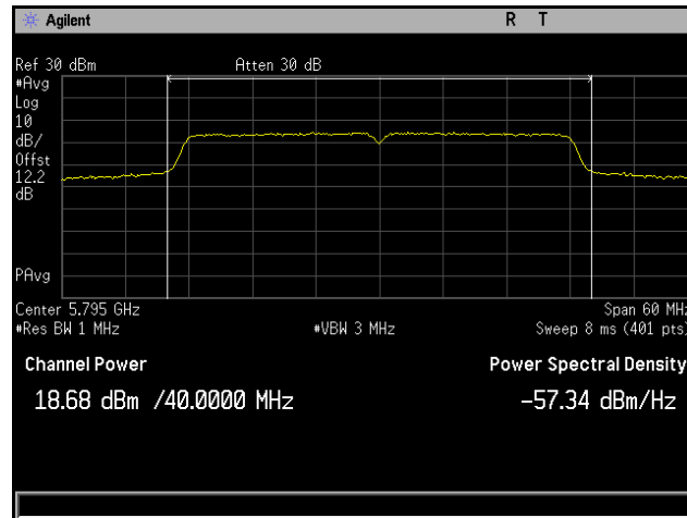
Plot 168. Conducted Output Power, 802.11n 40 MHz, Channel 5795 MHz, 6x8, MCS0 NSS1, CH7
