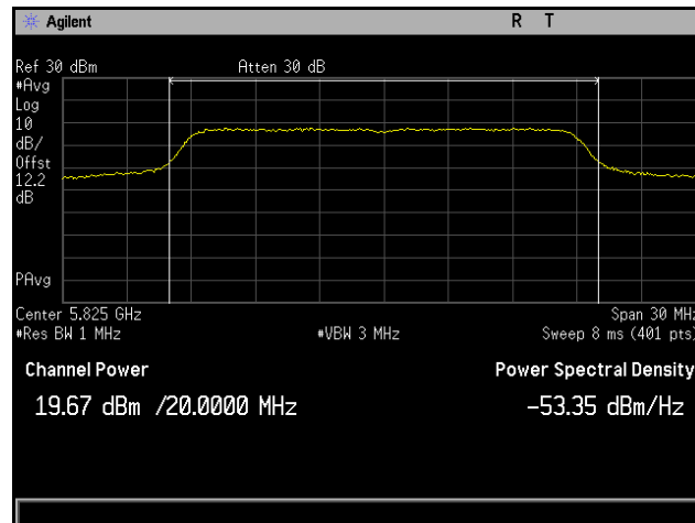
Plot 153. Conducted Output Power, 802.11n 20 MHz, Channel 5825 MHz, 6x8, MCS0 NSS1, CH6
