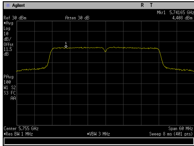
Plot 221. Power Spectral Density, 802.11n 40 MHz, Channel 5755 MHz, 4x8, MCS0 NSS1, CH5
