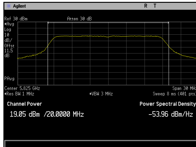
Plot 67. Conducted Output Power, 802.11n 20 MHz, Channel 5825 MHz, 4x8, MCS0 NSS1, CH3
