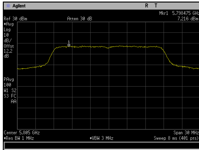
Plot 295. Power Spectral Density, 802.11n 20 MHz, Channel 5805 MHz, 6x8, MCS0 NSS1, CH7
