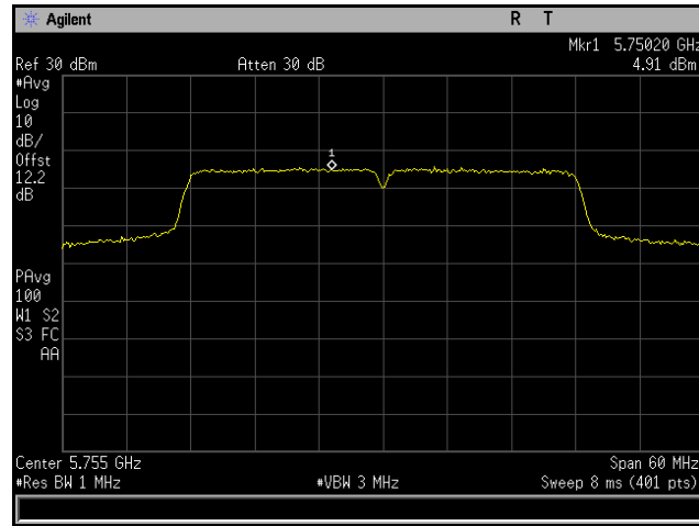
Plot 269. Power Spectral Density, 802.11ac 40 MHz, Channel 5755 MHz, 6x8, MCS0 NSS1, CH6
