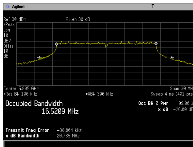
Plot 16. 26 dB Occupied Bandwidth, 802.11a 20 MHz, Channel 5805 MHz, 6x8, 6M
