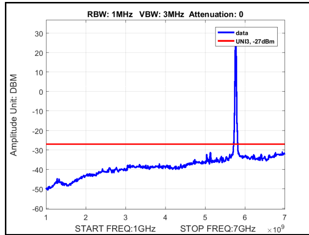
Plot 344. Radiated Spurious Emissions, 802.11a 20 MHz, Channel 5745 MHz, 6x8, 6M, 1 GHz – 7 GHz
