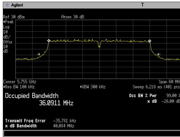
Plot 7. 26 dB Occupied Bandwidth, 802.11ac 40 MHz, Channel 5755 MHz, 4x8, NSS1 MCS0
