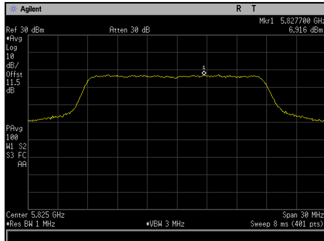
Plot 213. Power Spectral Density, 802.11n 20 MHz, Channel 5825 MHz, 4x8, MCS0 NSS1, CH5
