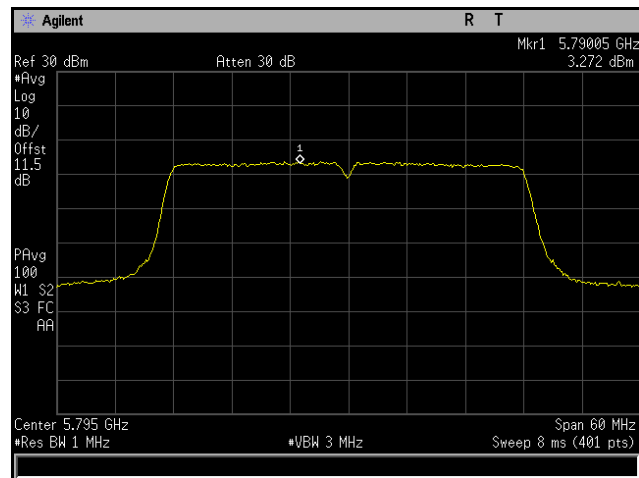
Plot 220. Power Spectral Density, 802.11n 40 MHz, Channel 5795 MHz, 4x8, MCS0 NSS1, CH4
