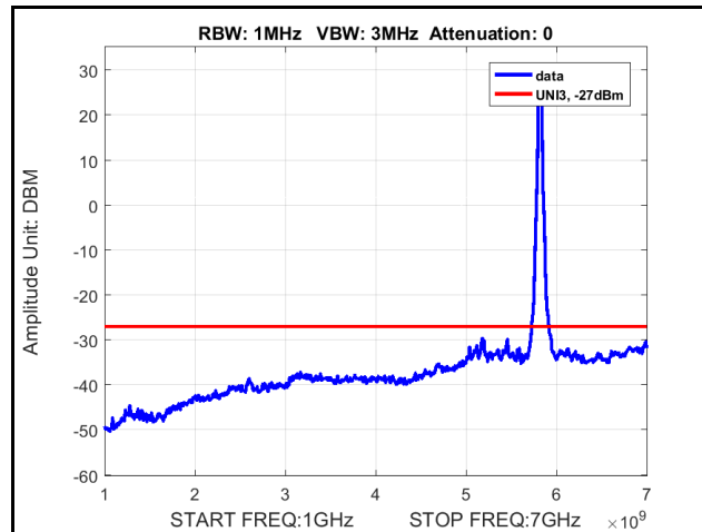
Plot 354. Radiated Spurious Emissions, 802.11n 40 MHz, Channel 5795 MHz, 6x8, MCS0, 1 GHz – 7 GHz
