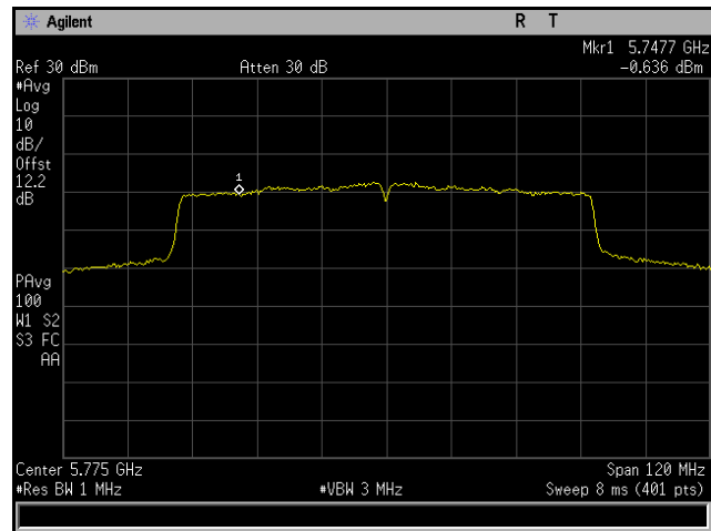
Plot 278. Power Spectral Density, 802.11ac 80 MHz, Channel 5775 MHz, 6x8, MCS0 NSS1, CH7
