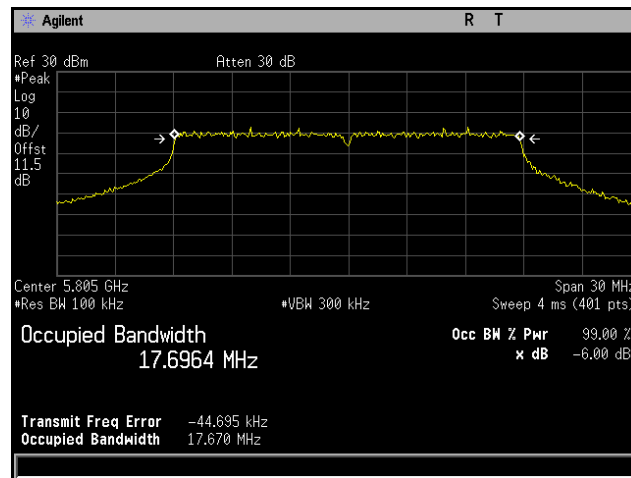
Plot 381. 6 dB Occupied Bandwidth, 802.11n 20 MHz, Channel 5805 MHz, 6x8, MCS0
