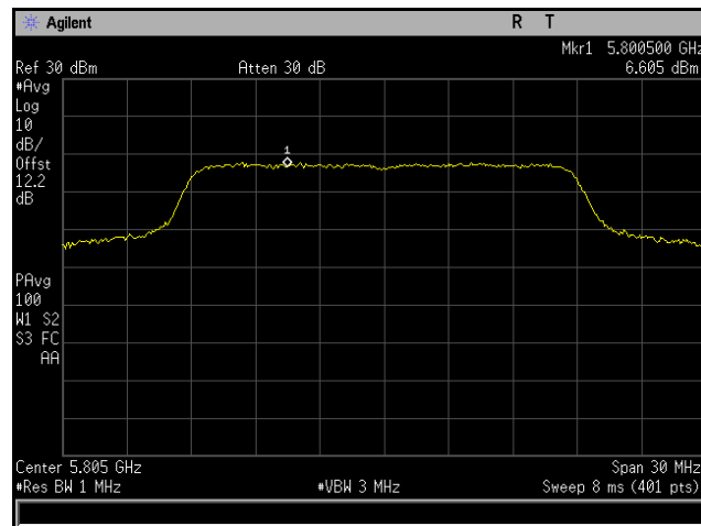
Plot 256. Power Spectral Density, 802.11ac 20 MHz, Channel 5805 MHz, 6x8, MCS0 NSS1, CH6
