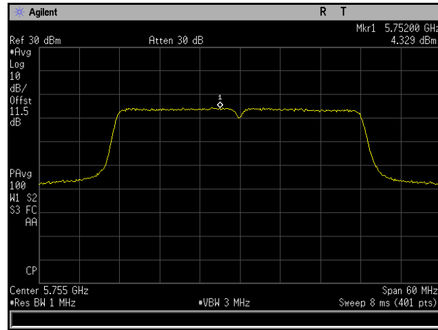
Plot 195. Power Spectral Density, 802.11ac 40 MHz, Channel 5755 MHz, 4x8, MCS0 NSS1, CH4
