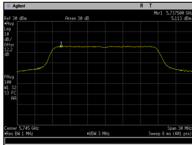
Plot 255. Power Spectral Density, 802.11ac 20 MHz, Channel 5745 MHz, 6x8, MCS0 NSS1, CH6
