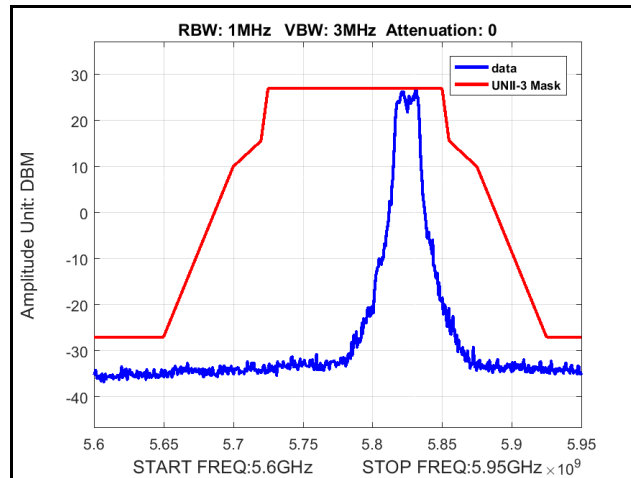
Plot 323. Radiated Spurious Emissions, Mask, 802.11a 20 MHz, Channel 5825 MHz, 6x8, 6M
