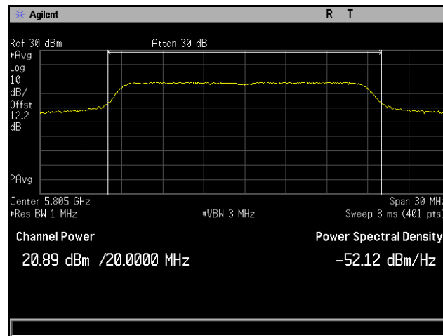
Plot 116. Conducted Output Power, 802.11ac 20 MHz, Channel 5805 MHz, 6x8, MCS0 NSS1, CH6
