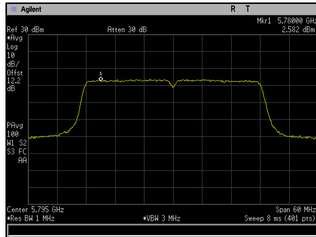
Plot 266. Power Spectral Density, 802.11ac 40 MHz, Channel 5795 MHz, 6x8, MCS0 NSS1, CH4
