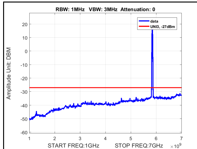
Plot 336. Radiated Spurious Emissions, 802.11ac 20 MHz, Channel 5825 MHz, 4x8, NSS1 MCS0, 1 GHz – 7 GHz
