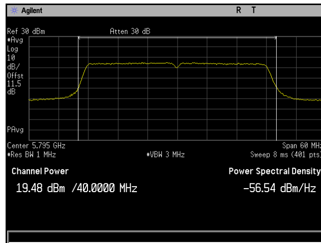
Plot 56. Conducted Output Power, 802.11ac 40 MHz, Channel 5795 MHz, 4x8, MCS0 NSS1, CH4
