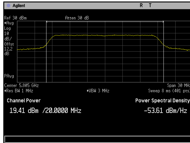
Plot 149. Conducted Output Power, 802.11n 20 MHz, Channel 5805 MHz, 6x8, MCS0 NSS1, CH5
