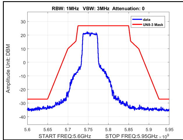
Plot 315. Radiated Spurious Emissions, Mask, 802.11ac 40 MHz, Channel 5755 MHz, 4x8, NSS1 MCS0
