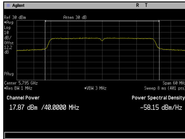
Plot 132. Conducted Output Power, 802.11ac 40 MHz, Channel 5795 MHz, 6x8, MCS0 NSS1, CH7
