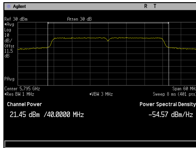
Plot 60. Conducted Output Power, 802.11ac 40 MHz, Channel 5795 MHz, 4x8, MCS0 NSS1, CH6
