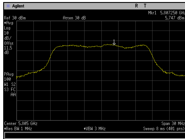
Plot 235. Power Spectral Density, 802.11a 20 MHz, Channel 5805 MHz, 6x8, 6M, CH5
