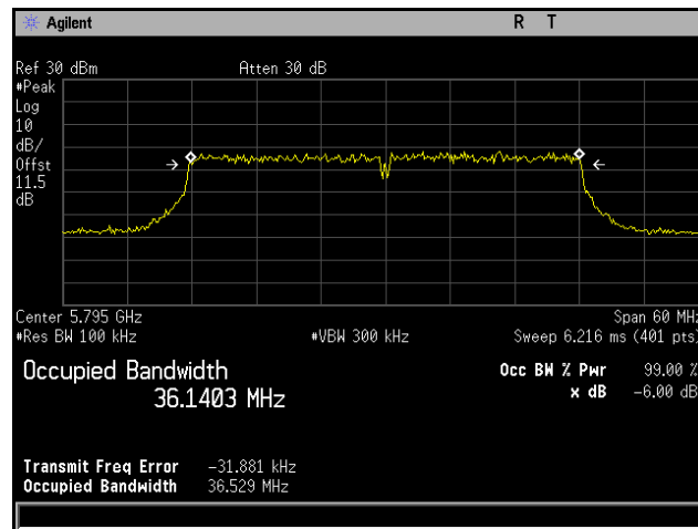
Plot 378. 6 dB Occupied Bandwidth, 802.11ac 40 MHz, Channel 5795 MHz, 6x8, NSS1 MCS0
