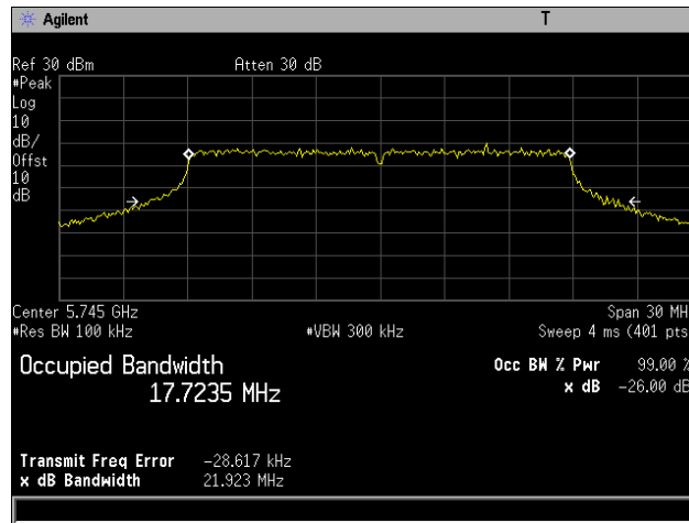
Plot 18. 26 dB Occupied Bandwidth, 802.11ac 20 MHz, Channel 5745 MHz, 6x8, NSS1 MCS0
