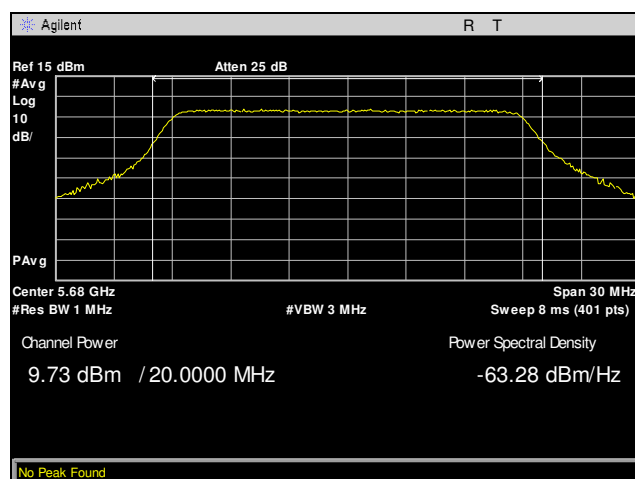
Plot 472. Conducted Output Power, 802.11n 20 MHz, 5680 MHz, Port 6, Radio 0, 8x8
