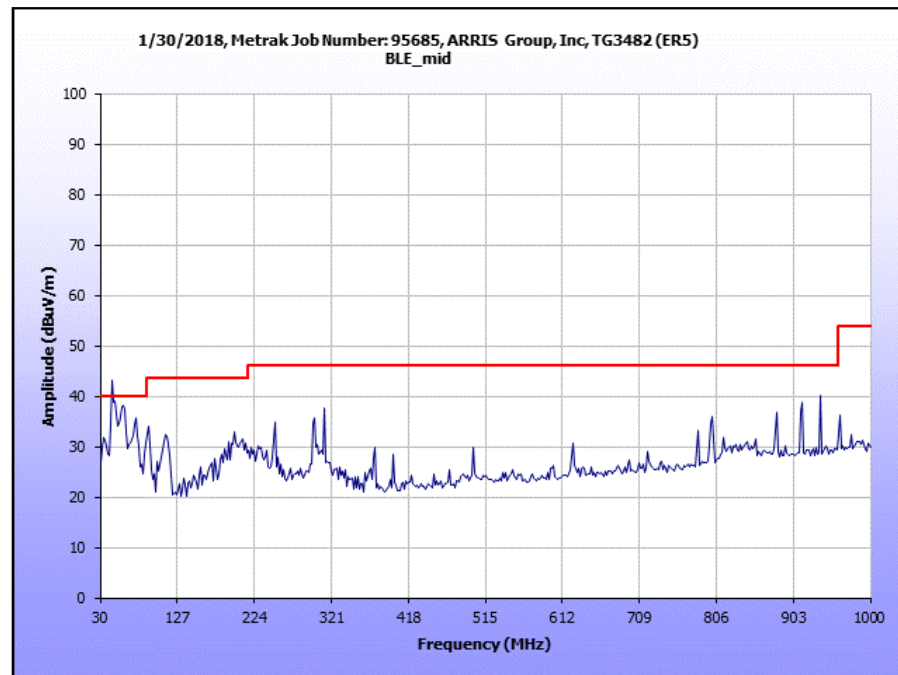
Plot 10. Radiated Emissions, BLE, mid
