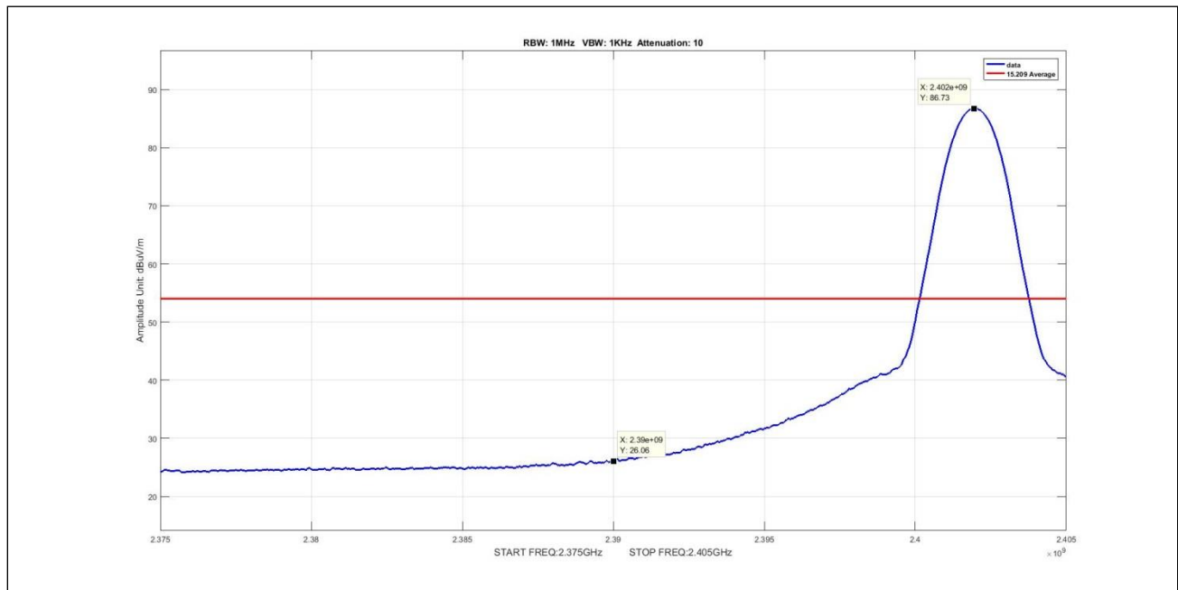
Plot 18. Radiated Emissions, average, BLE, radiated band edge, low
