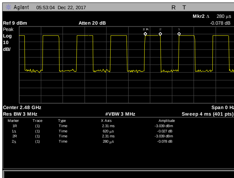
Plot 9. Peak Power Output, Duty cycle
