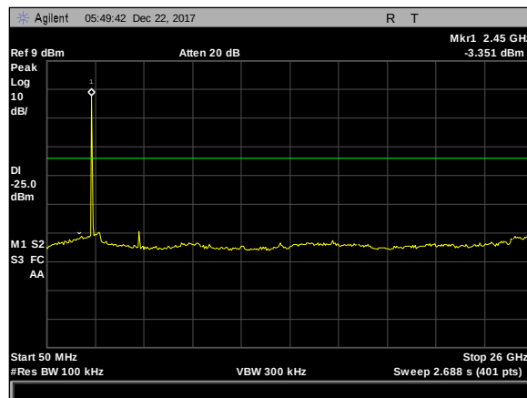
Plot 23. Spurious RF Conducted Emissions, 50M-26G, high
