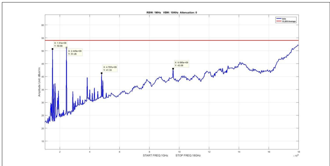
Plot 12. Radiated Emissions, average, BLE, radiated spurious 1G-18G, mid
