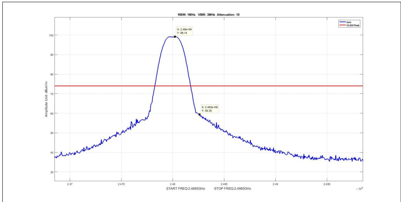
Plot 19. Radiated Emissions, peak, BLE, radiated band edge, high
