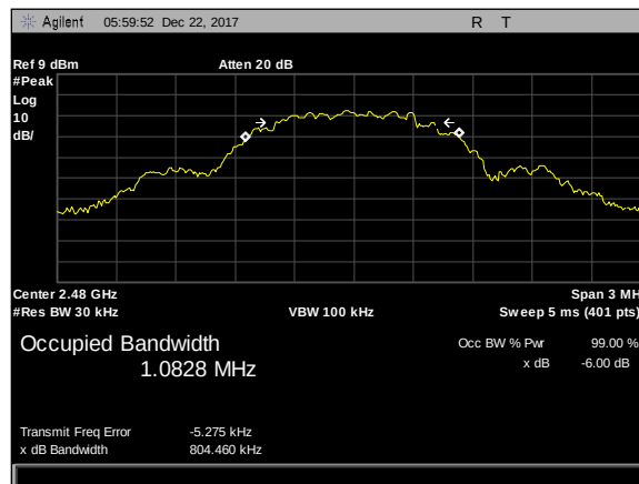
Plot 5. 6 dB Occupied Bandwidth, high
