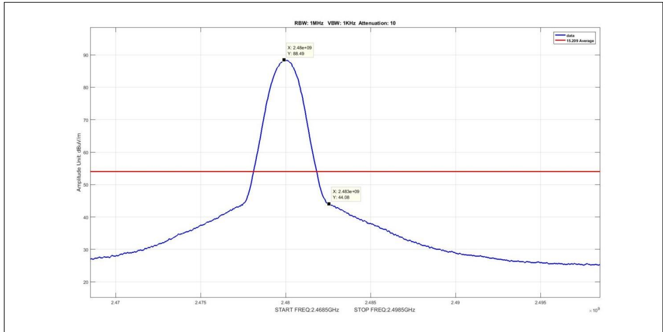
Plot 17. Radiated Emissions, average, BLE, radiated band edge, high
