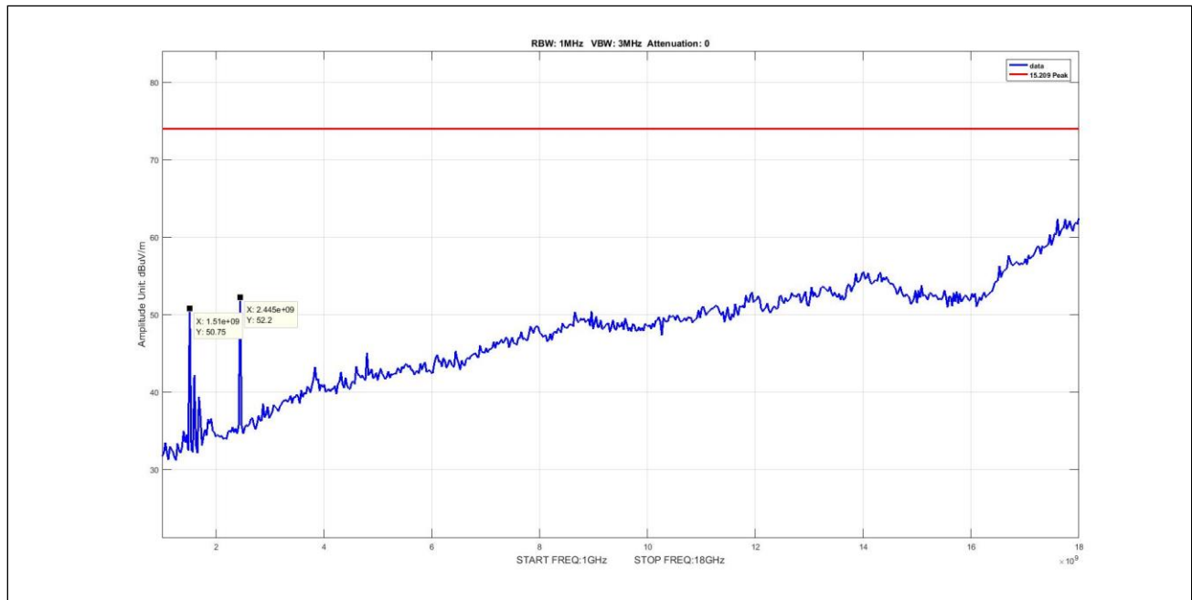
Plot 15. Radiated Emissions, peak, BLE, radiated spurious 1G-18G, mid
