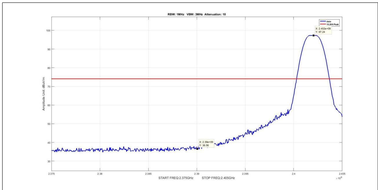
Plot 20. Radiated Emissions, peak, BLE, radiated band edge, low
