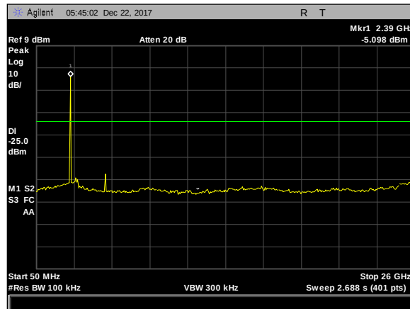
Plot 21. Spurious RF Conducted Emissions, 50M-26G, low
