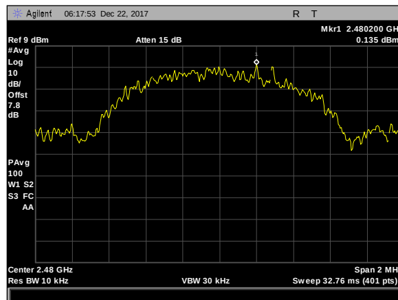
Plot 28. Power Spectral Density, high
