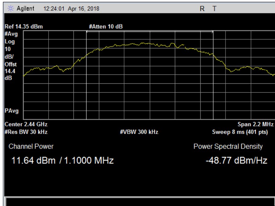
Plot 7. Peak Power Output, mid
