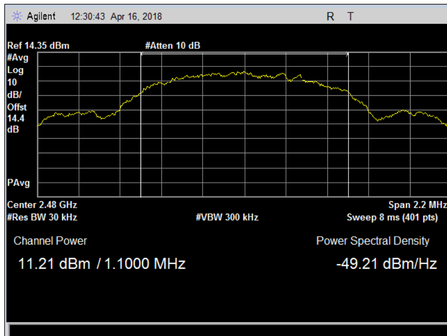
Plot 8. Peak Power Output, high
