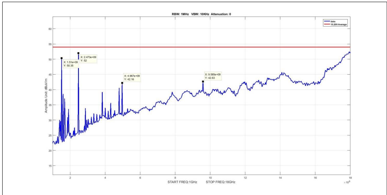
Plot 13. Radiated Emissions, average, BLE, radiated spurious 1G-18G, high
