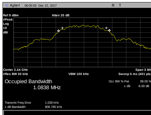
Plot 4. 6 dB Occupied Bandwidth, mid
