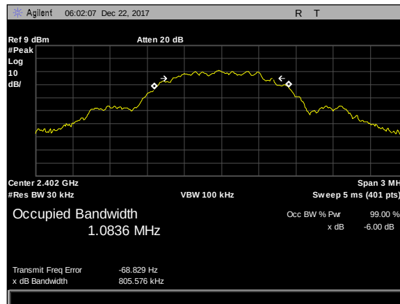
Plot 3. 6 dB Occupied Bandwidth, low
