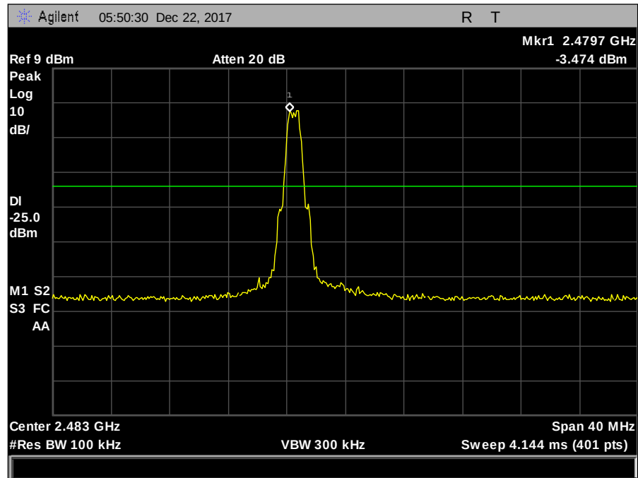
Plot 24. Spurious RF Conducted Emissions, conducted band edge, high
