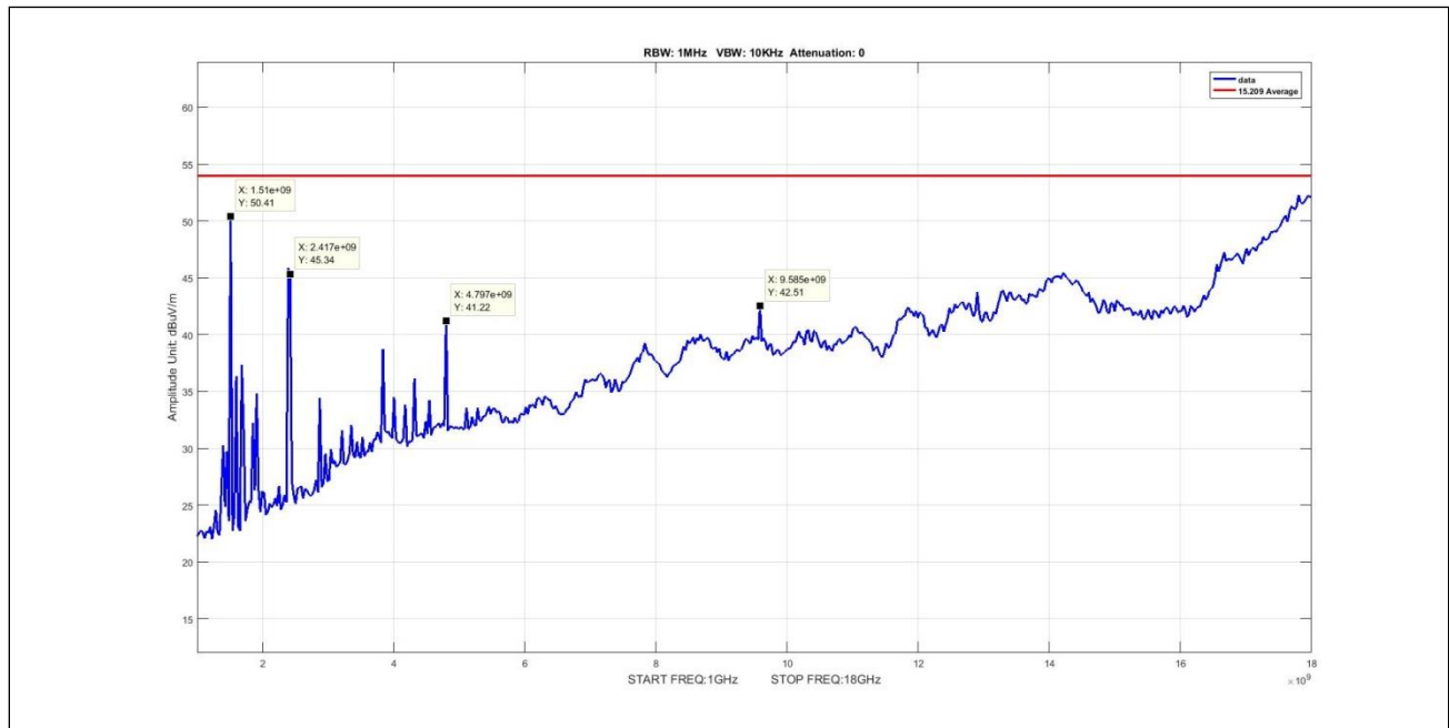
Plot 11. Radiated Emissions, average, BLE, radiated spurious 1G-18G, low
