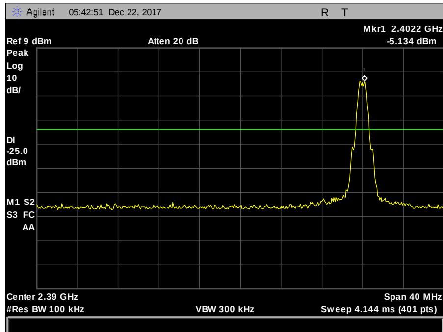
Plot 25. Spurious RF Conducted Emissions, conducted band edge, low
