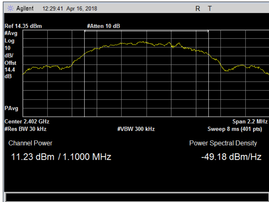
Plot 6. Peak Power Output, low
