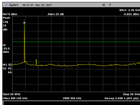
Plot 22. Spurious RF Conducted Emissions, 50M-26G, mid
