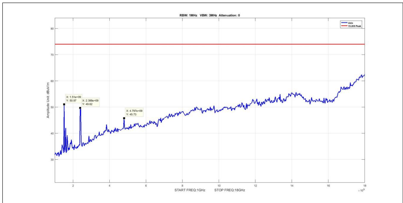
Plot 14. Radiated Emissions, peak, BLE, radiated spurious 1G-18G, low
