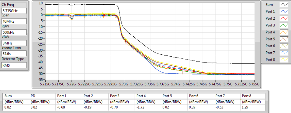
802.11ac VHT40-BF_Nss1,(MCS0)_8TX
