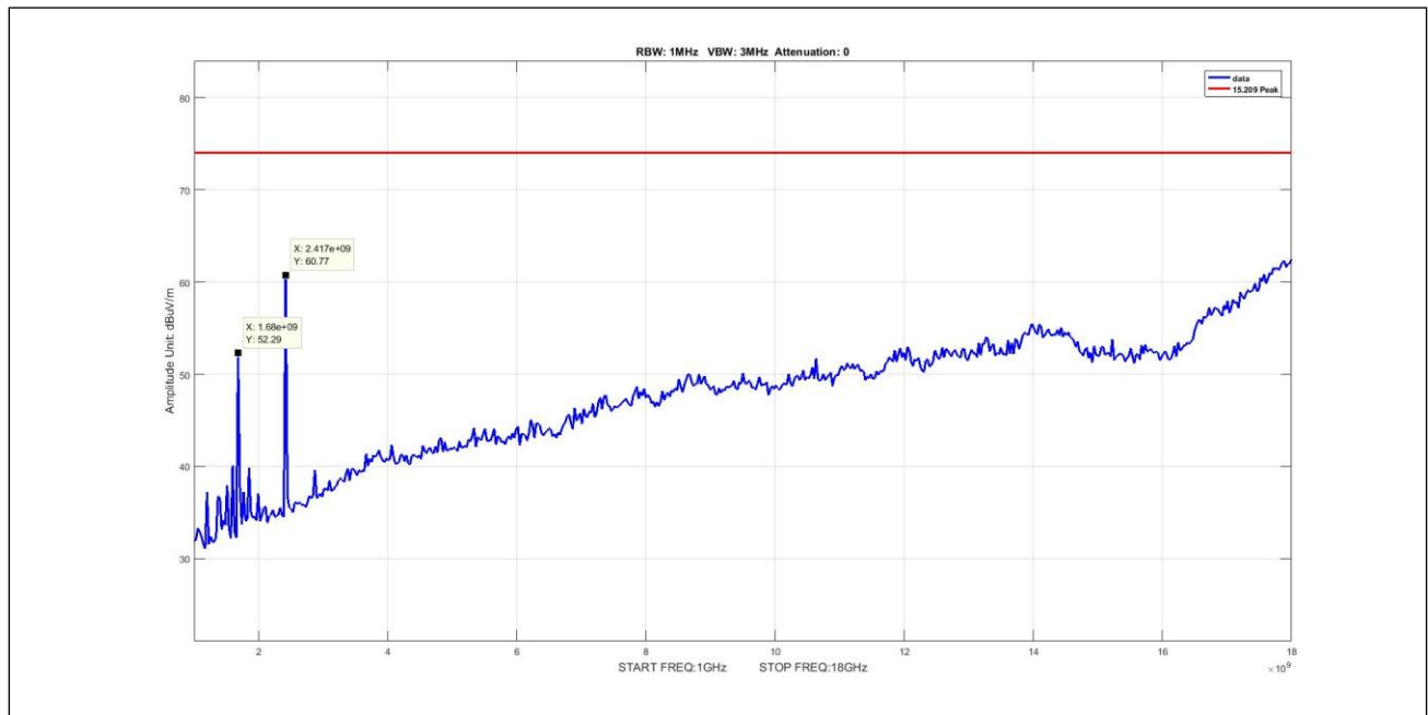
Plot 14. Radiated Emissions, peak, Thread, radiated spurious 1G-18G, low
