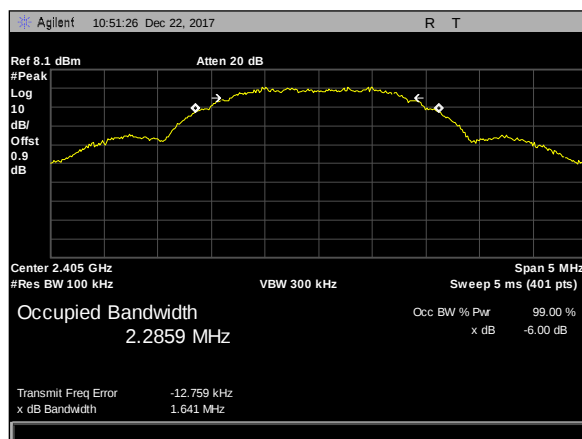
Plot 3. 6 dB Occupied Bandwidth, Thread, OBW, low
