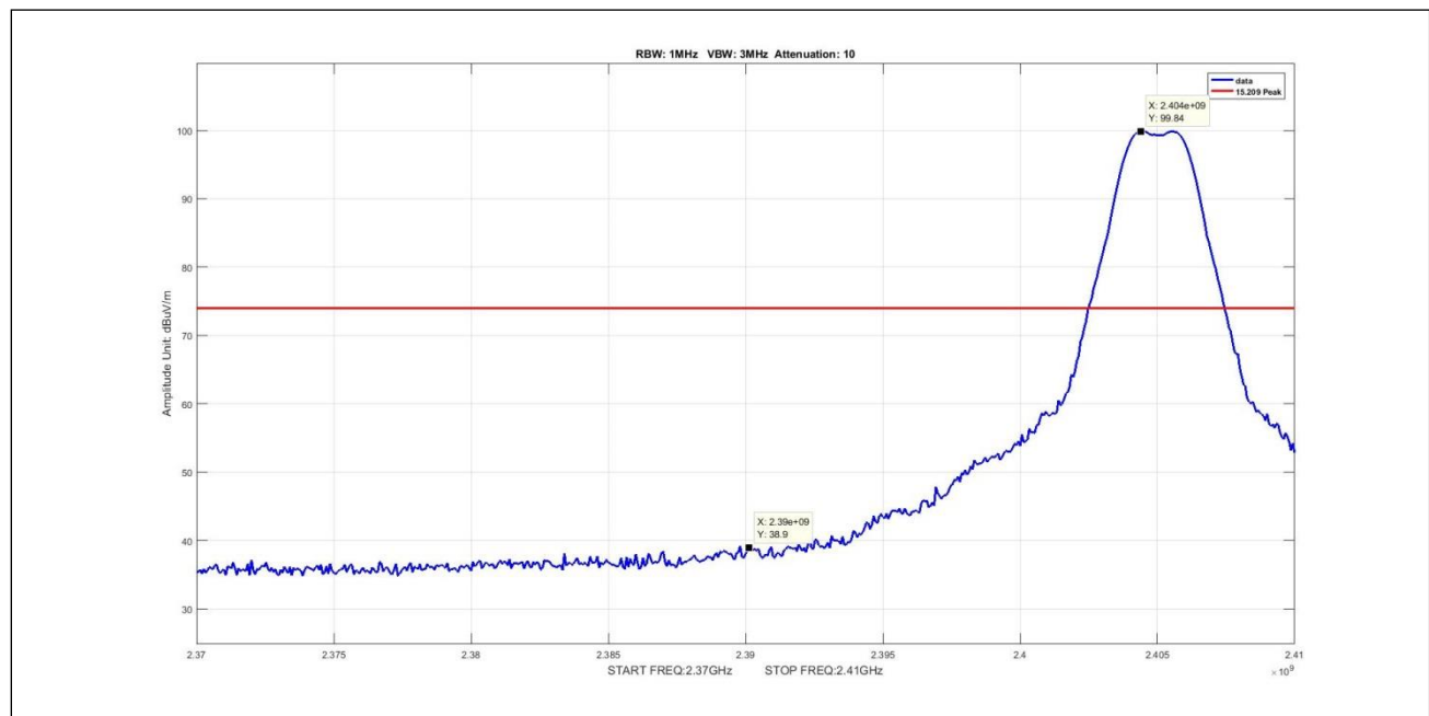
Plot 20. Radiated Emissions, peak, Thread, radiated band edge, low
