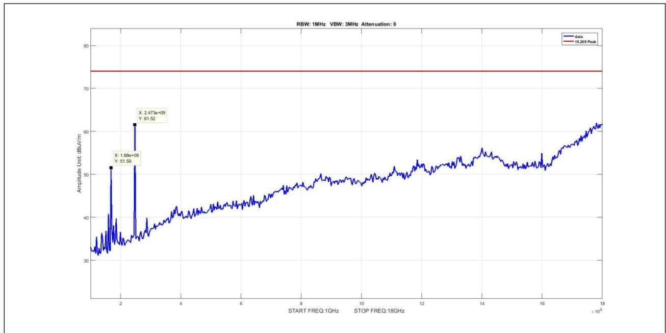
Plot 16. Radiated Emissions, peak, Thread, radiated spurious 1G-18G, high
