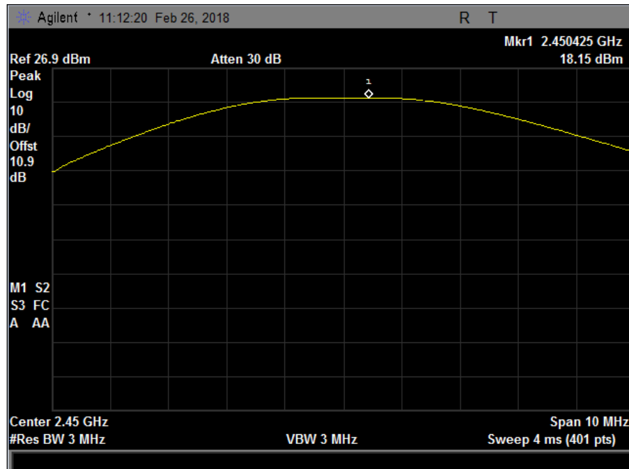
Plot 7. Peak Output Power, Thread, mid
