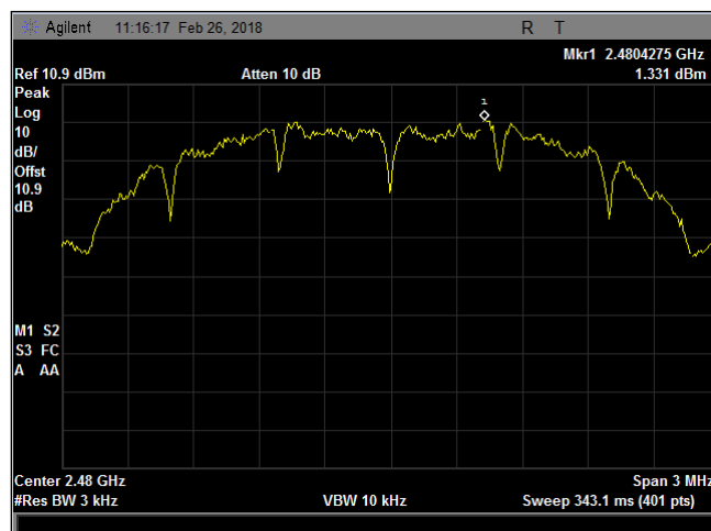
Plot 28. Power Spectral Density, Thread, high
