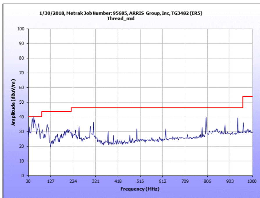
Plot 10. Radiated Emissions, Thread, mid
