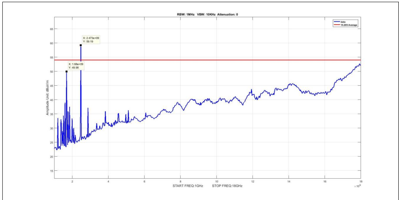
Plot 13. Radiated Emissions, average, Thread, radiated spurious 1G-18G, high
