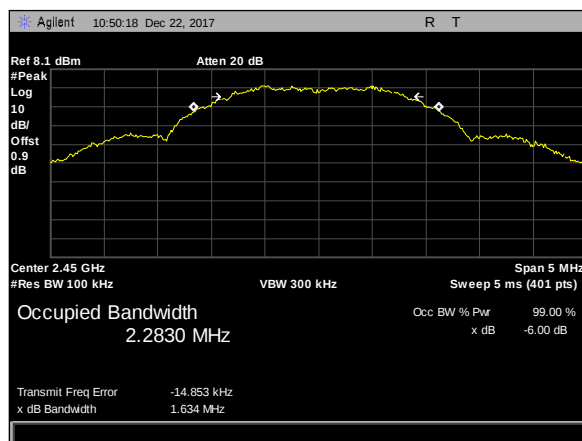
Plot 4. 6 dB Occupied Bandwidth, Thread, OBW, mid
