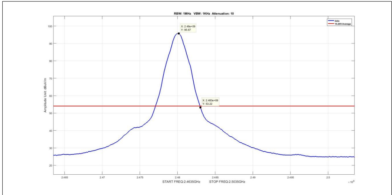
Plot 17. Radiated Emissions, average, Thread, radiated band edge, high
