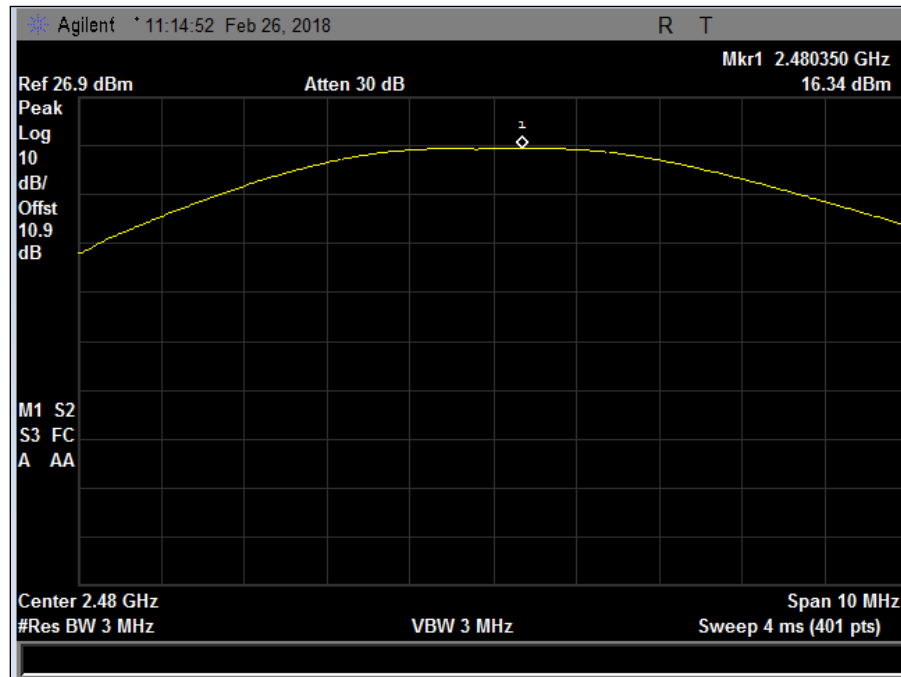
Plot 8. Peak Output Power, Thread, high
