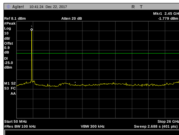
Plot 23. Spurious RF Conducted Emissions, Thread, conducted spurious, 50M-26G, high
