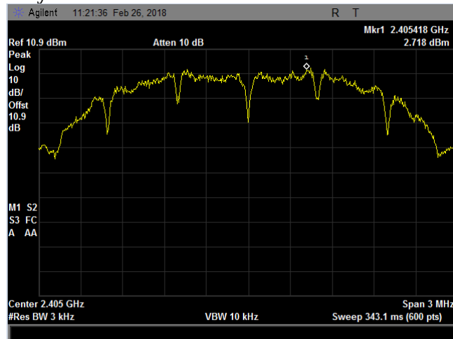
Plot 26. Power Spectral Density, Thread, low
