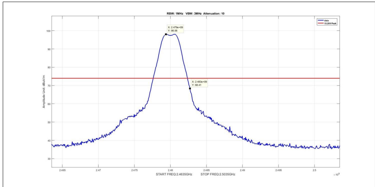
Plot 19. Radiated Emissions, peak, Thread, radiated band edge, high
