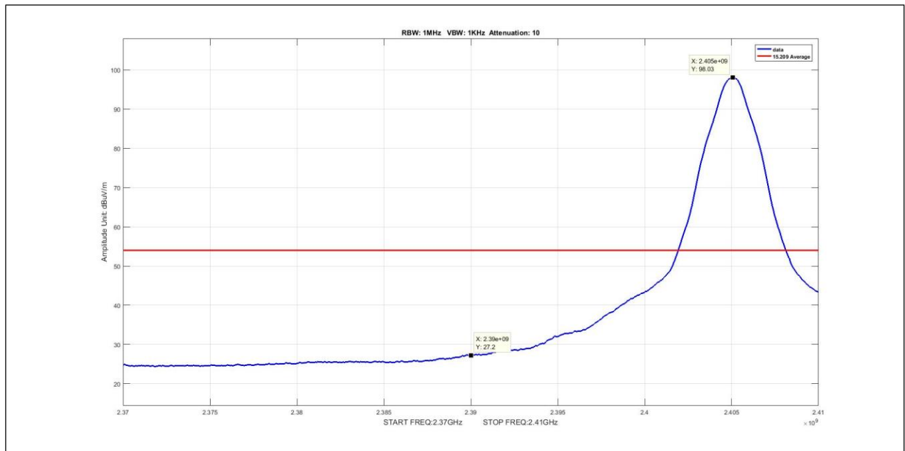
Plot 18. Radiated Emissions, average, Thread, radiated band edge, low
