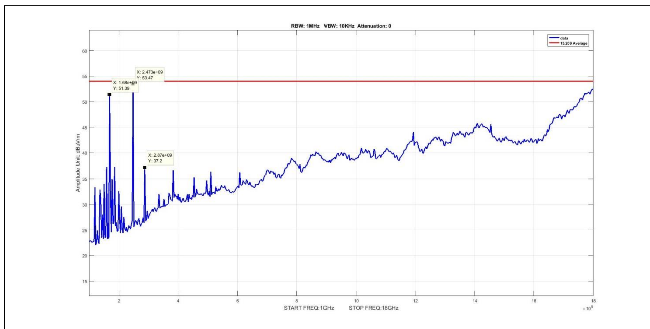
Plot 12. Radiated Emissions, average, Thread, radiated spurious 1G-18G, mid
