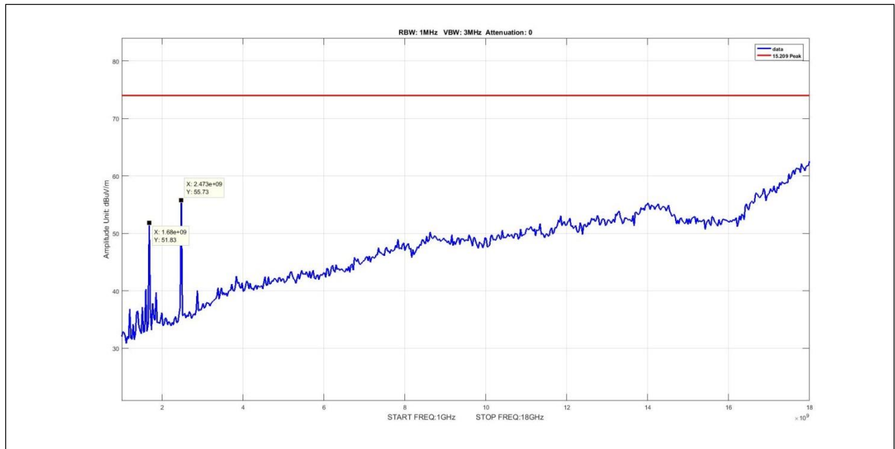
Plot 15. Radiated Emissions, peak, Thread, radiated spurious 1G-18G, mid
