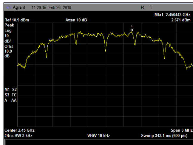
Plot 27. Power Spectral Density, Thread, mid
