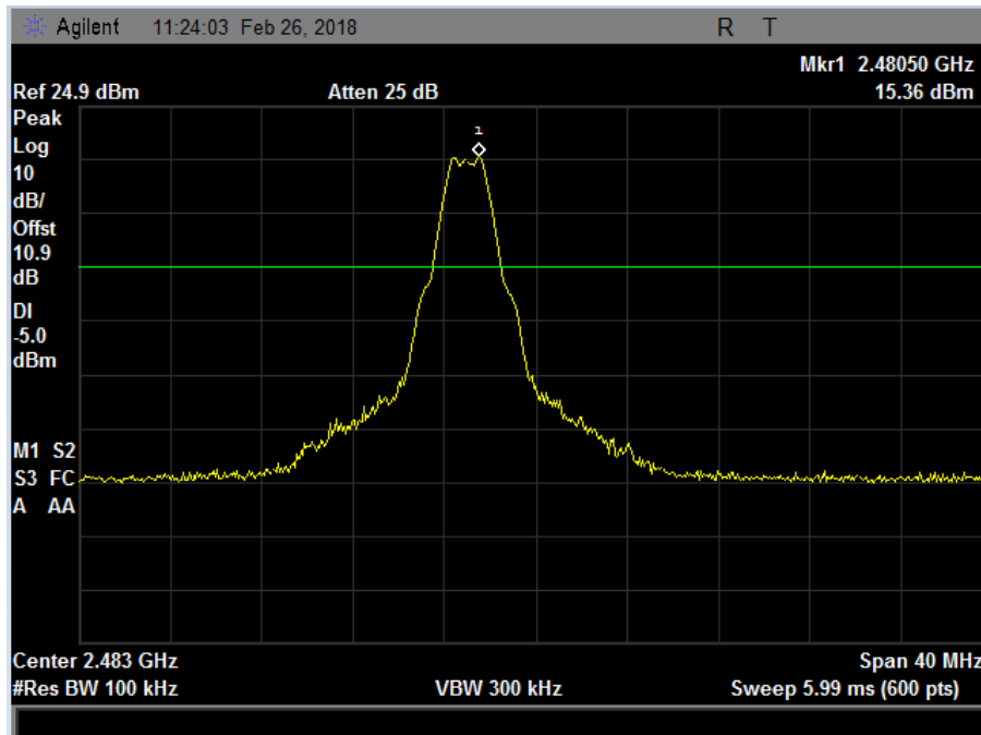
Plot 25. Spurious RF Conducted Emissions, Thread, conducted band edge, high
