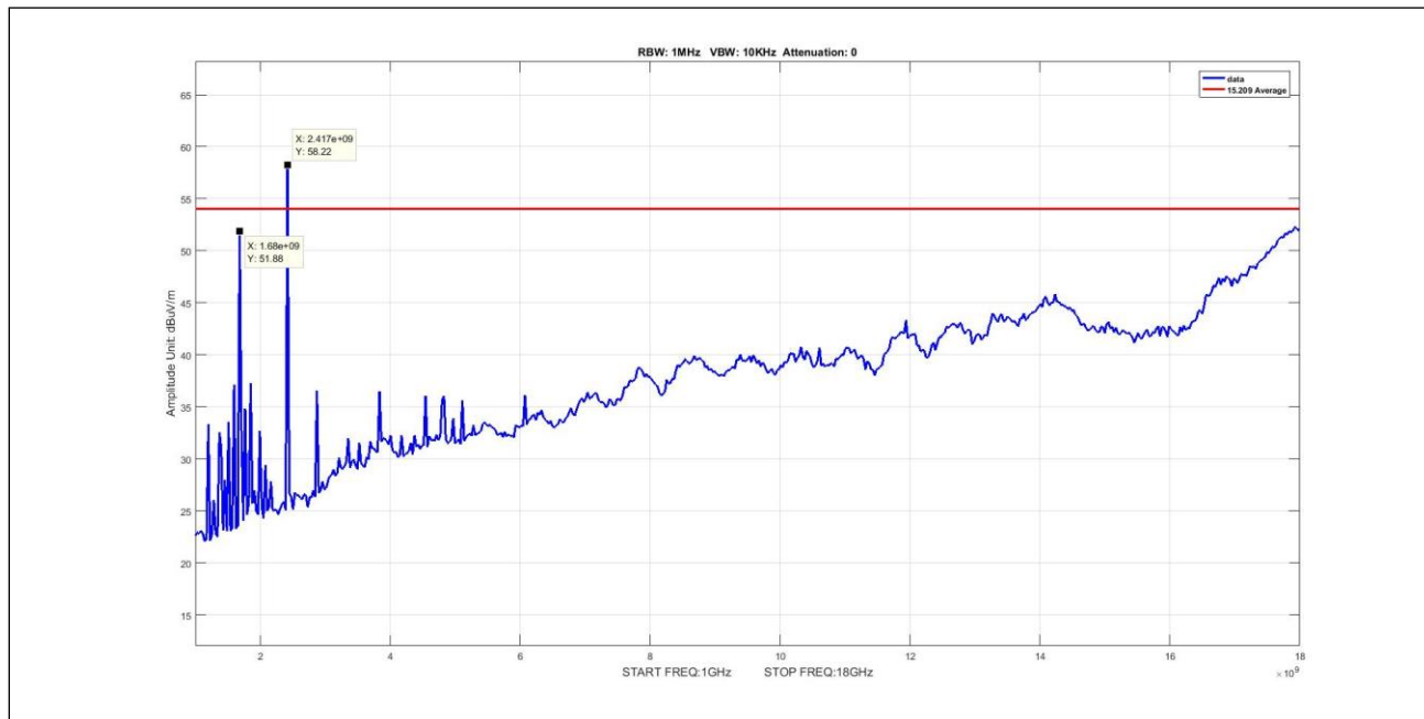
Plot 11. Radiated Emissions, average, Thread, radiated spurious 1G-18G, low
