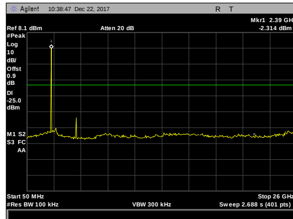
Plot 21. Spurious RF Conducted Emissions, Thread, conducted spurious, 50M-26G, low
