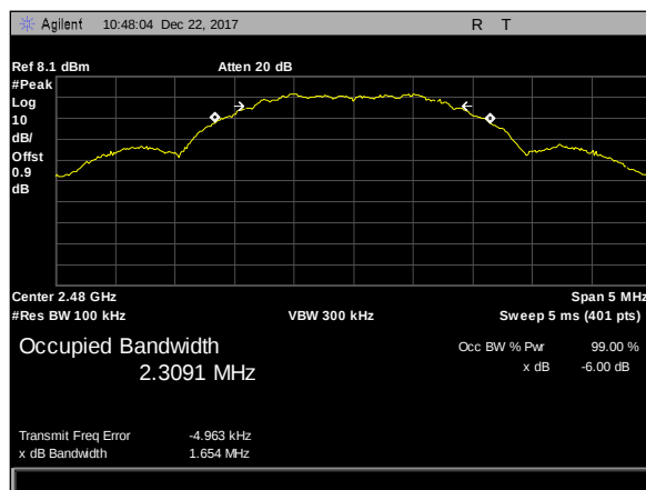
Plot 5. 6 dB Occupied Bandwidth, Thread, OBW, high
