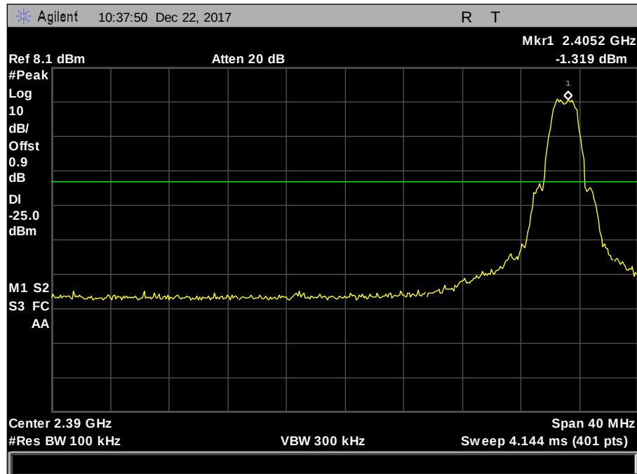
Plot 24. Spurious RF Conducted Emissions, Thread, conducted band edge, low
