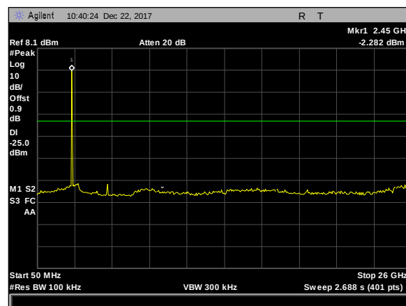
Plot 22. Spurious RF Conducted Emissions, Thread, conducted spurious, 50M-26G, mid
