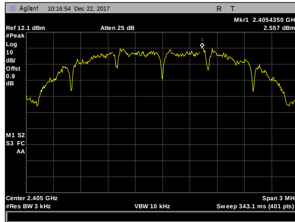
Plot 26. Power Spectral Density, Zigbee, PSD, low
