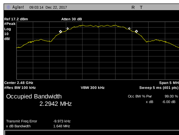
Plot 5. 6 dB Occupied Bandwidth, Zigbee, high
