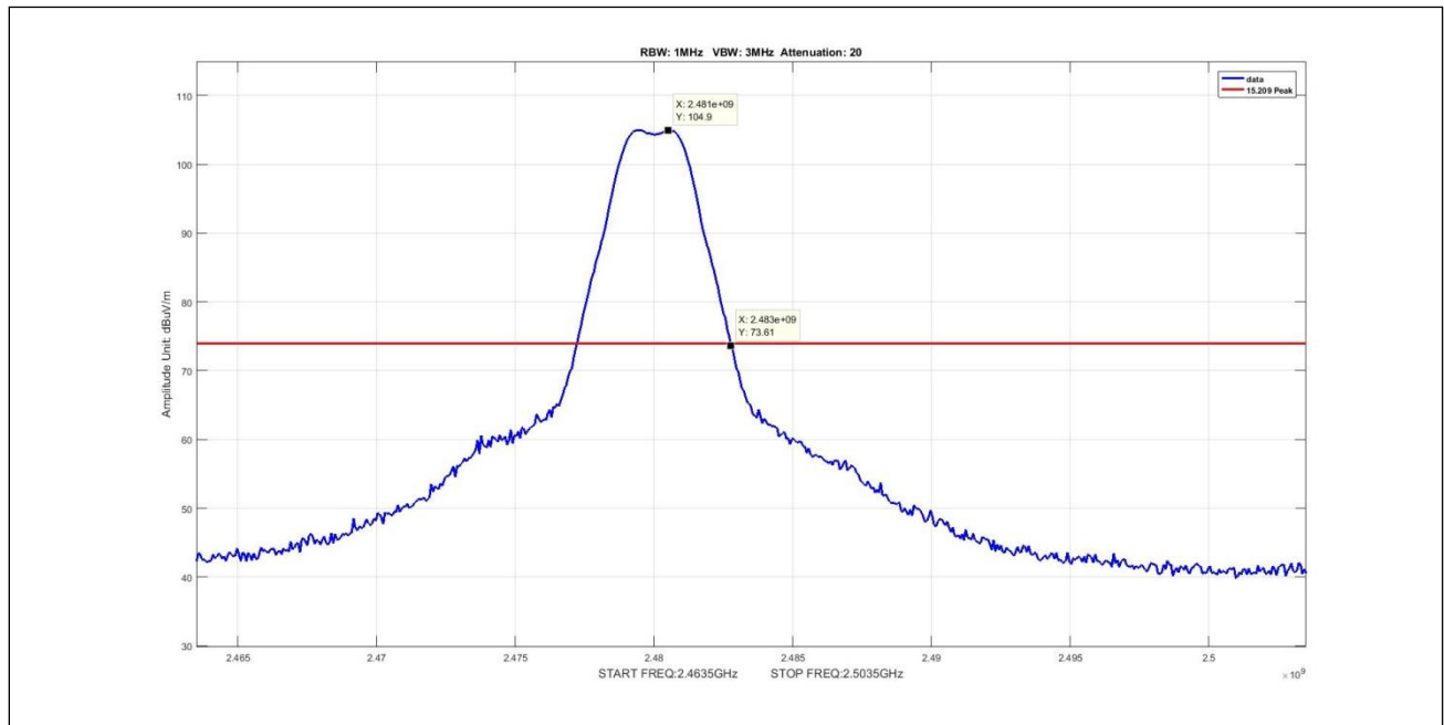
Plot 19. Radiated Emissions, peak, Zigbee, radiated band edge, high
