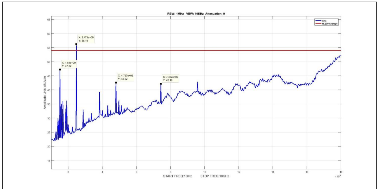
Plot 13. Radiated Emissions, average, Zigbee, radiated spurious 1G-18G, high
