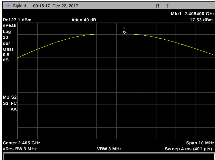
Plot 6. Peak Power Output, Zigbee, low
