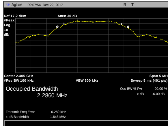
Plot 3. 6 dB Occupied Bandwidth, Zigbee, low
