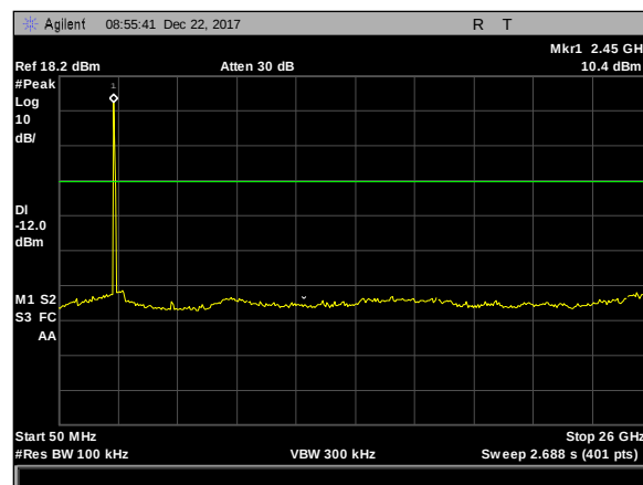
Plot 23. Spurious RF Conducted Emissions, Zigbee, conducted spurious, 50M-26G, high
