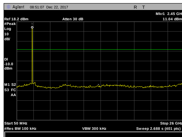
Plot 22. Spurious RF Conducted Emissions, Zigbee, conducted spurious, 50M-26G, mid
