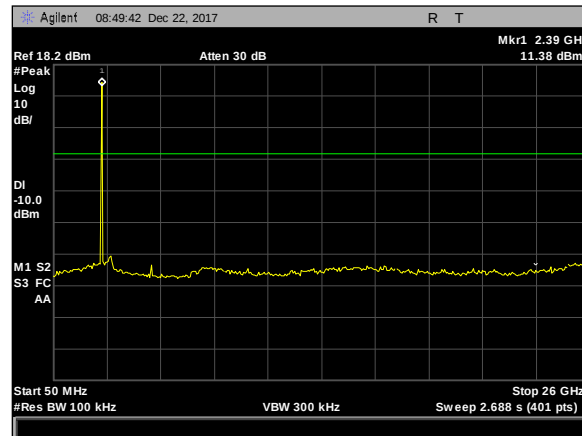
Plot 21. Spurious RF Conducted Emissions, Zigbee, conducted spurious, 50M-26G, low
