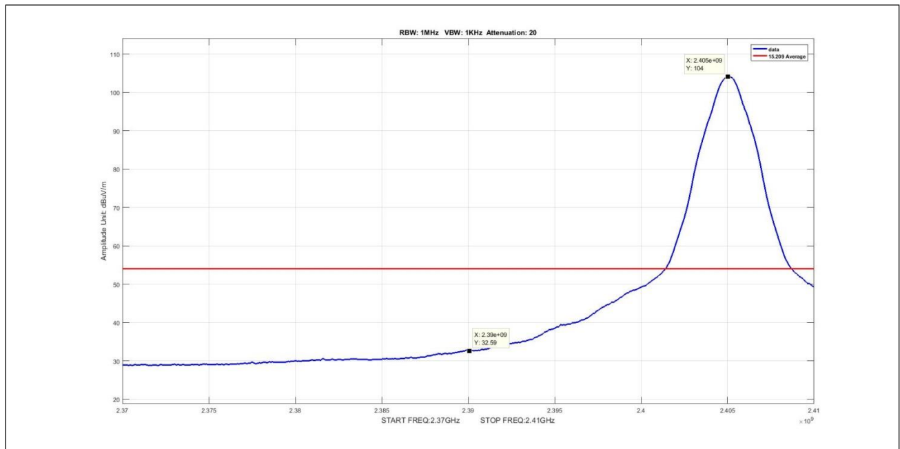
Plot 18. Radiated Emissions, average, Zigbee, radiated band edge, low
