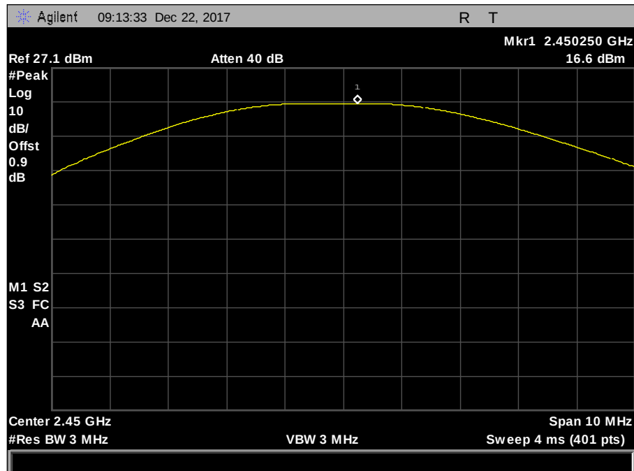
Plot 7. Peak Power Output, Zigbee, mid
