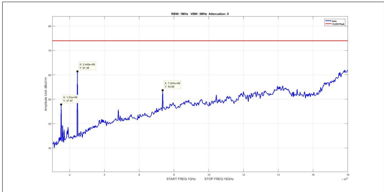
Plot 15. Radiated Emissions, peak, Zigbee, radiated spurious 1G-18G, mid
