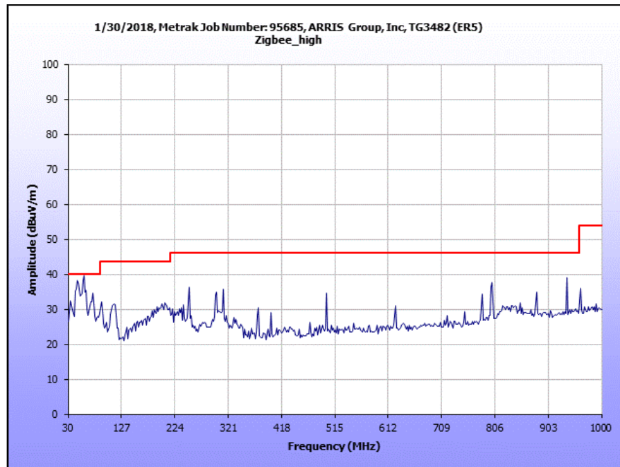
Plot 10. Radiated Emissions, Zigbee, high
