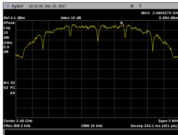
Plot 28. Power Spectral Density, Zigbee, PSD, high
