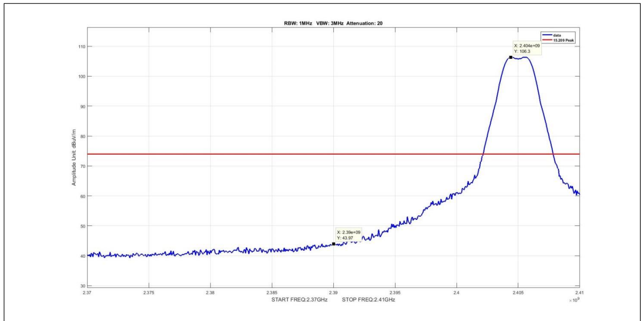
Plot 20. Radiated Emissions, peak, Zigbee, radiated band edge, low
