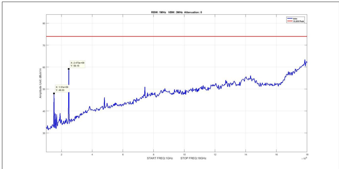
Plot 16. Radiated Emissions, peak, Zigbee, radiated spurious 1G-18G, high
