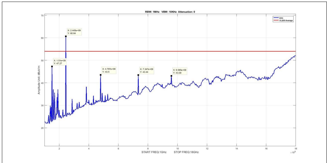
Plot 12. Radiated Emissions, average, Zigbee, radiated spurious 1G-18G, mid
