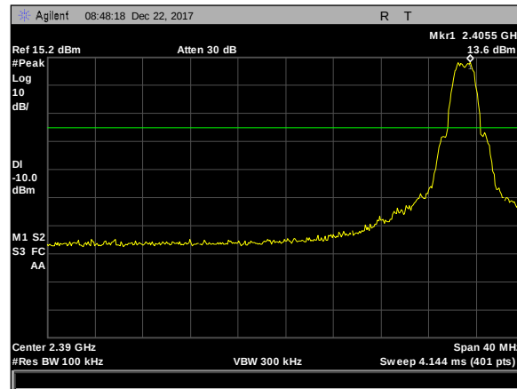
Plot 24. Spurious RF Conducted Emissions, Zigbee, conducted band edge, low
