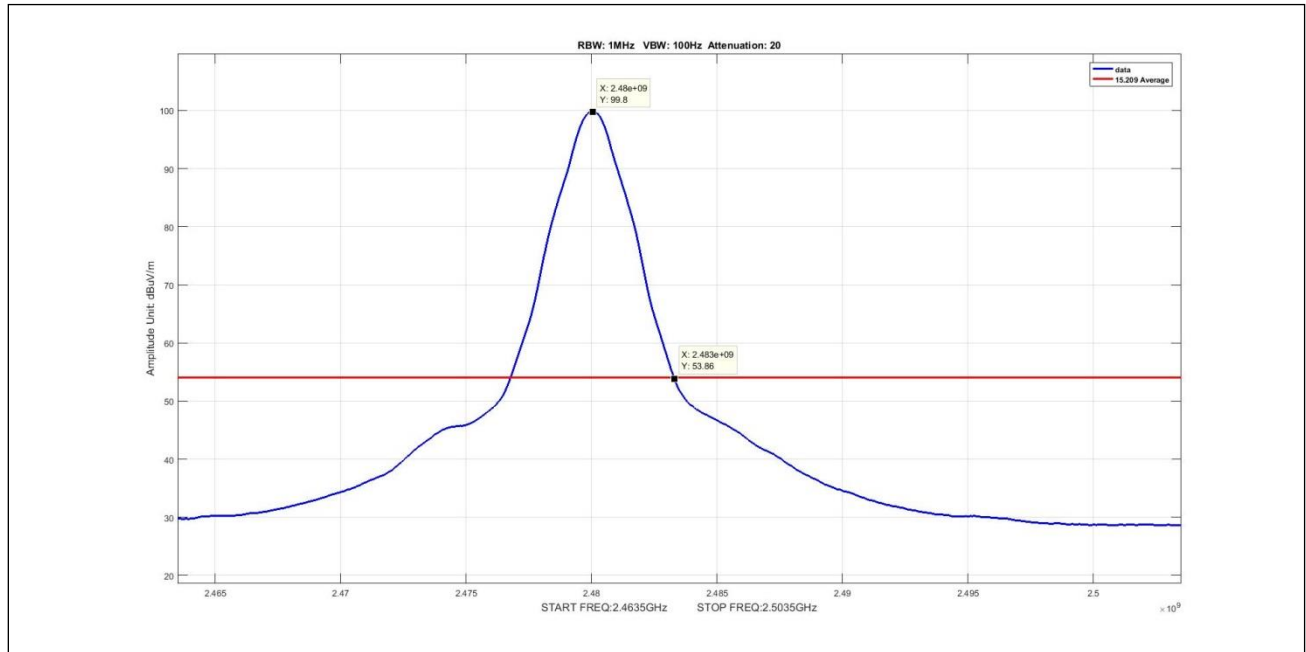
Plot 17. Radiated Emissions, average, Zigbee, radiated band edge, high
