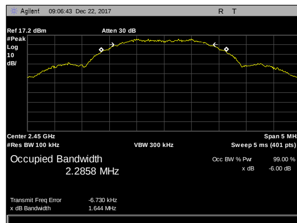
Plot 4. 6 dB Occupied Bandwidth, Zigbee, mid
