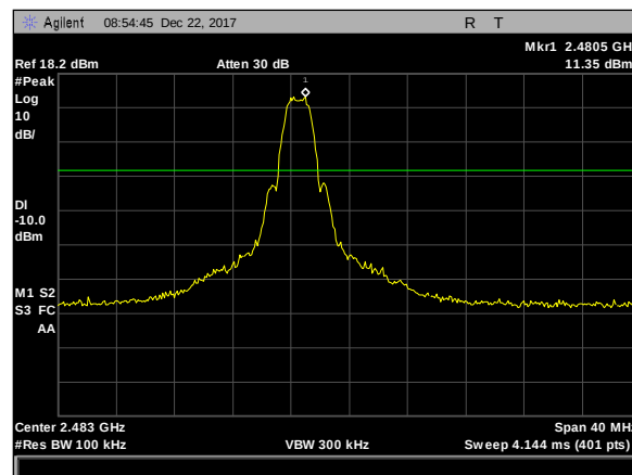
Plot 25. Spurious RF Conducted Emissions, Zigbee, conducted band edge, high
