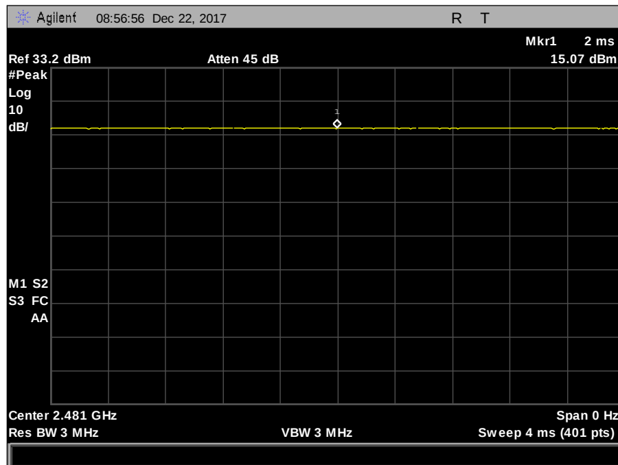
Plot 9. Peak Power Output, Zigbee, Duty Cycle
