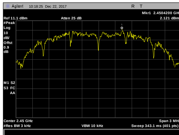
Plot 27. Power Spectral Density, Zigbee, PSD, mid
