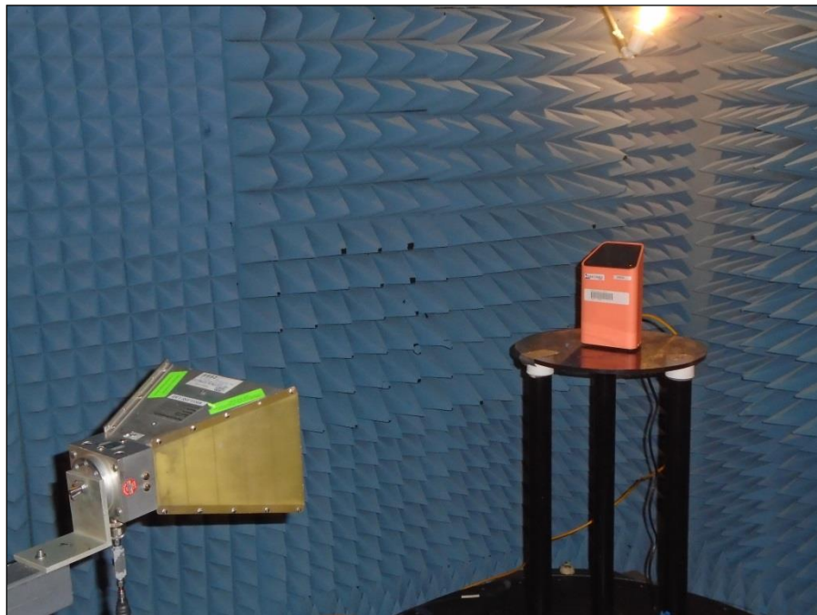
Photograph 3. Radiated Emissions, above 1 GHz
