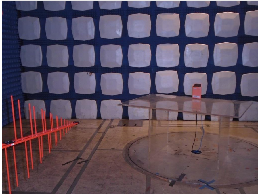
Photograph 2. Radiated Emissions, up to 1 GHz
