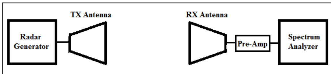
Figure 15: Radiated DFS Calibration Block Diagram
