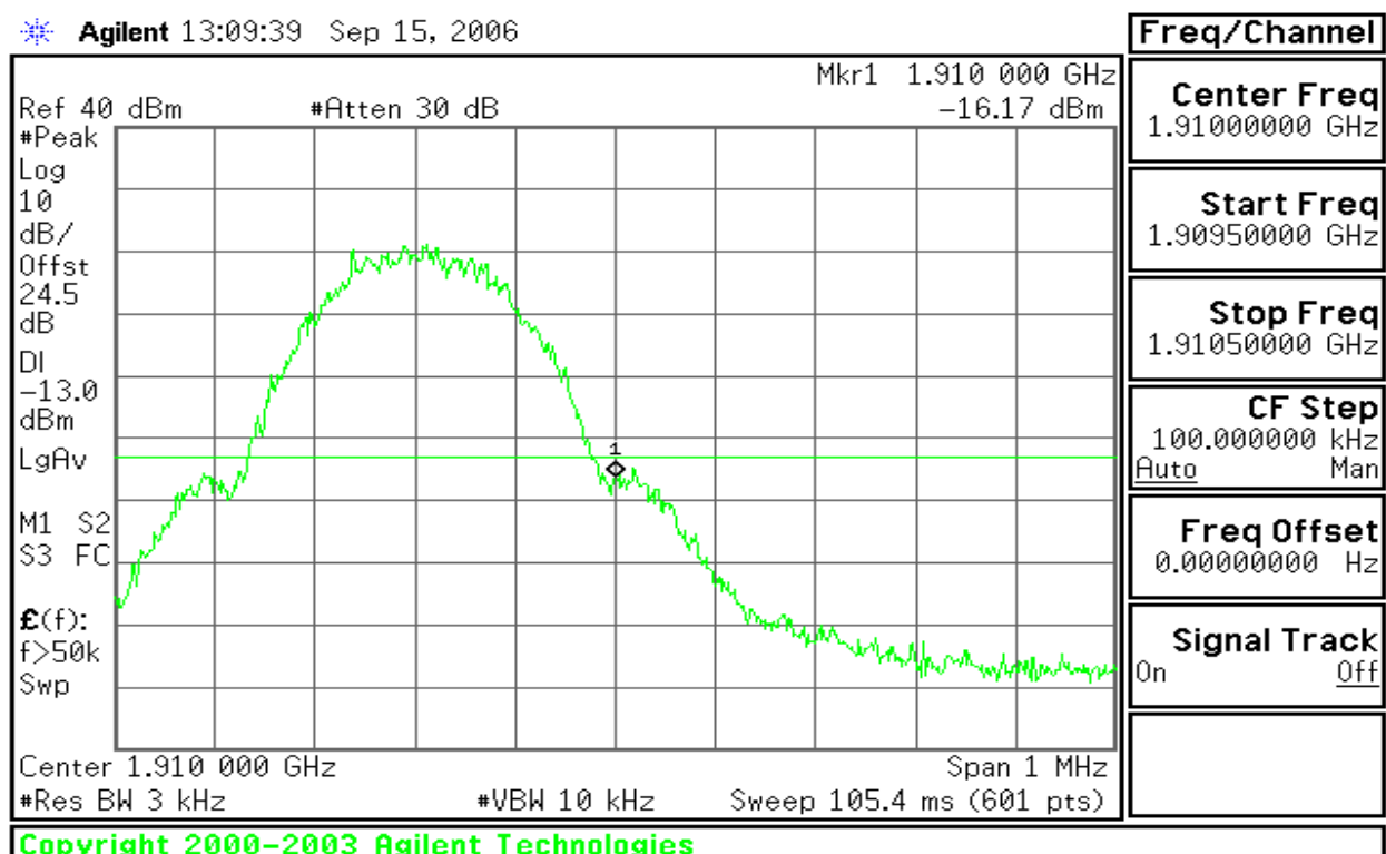
Figure 10-2: Band Edge emissions – GSM CH High
