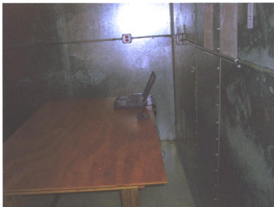
EUT 40cm from vertical ground plane
