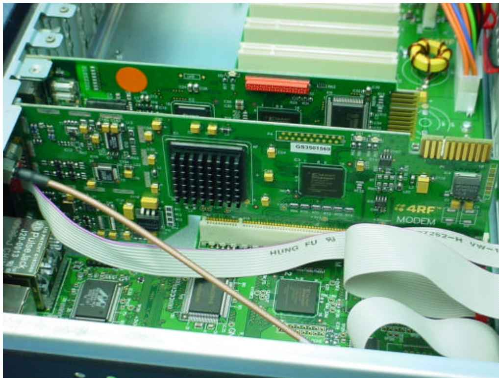
Modem board
