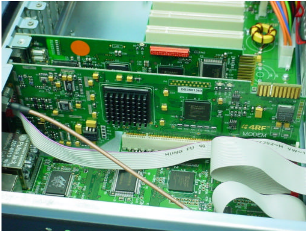
Modem board
