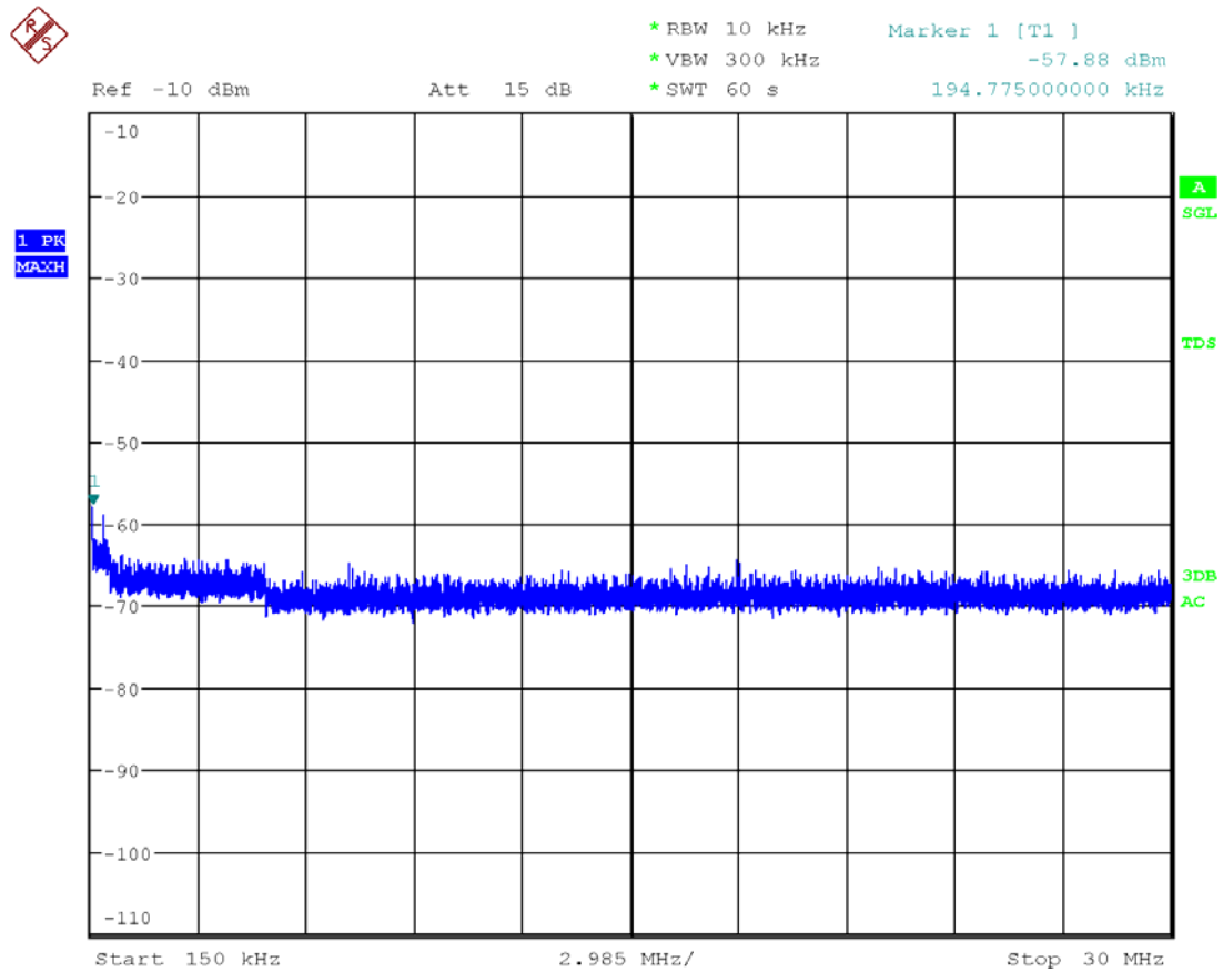
Graph 13: Conducted spurious emissions (non-restricted band), 150 kHz-30 MHz
