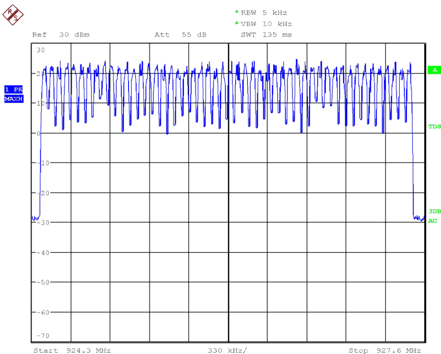
Graph 8: Number of hopping frequencies, middle range
