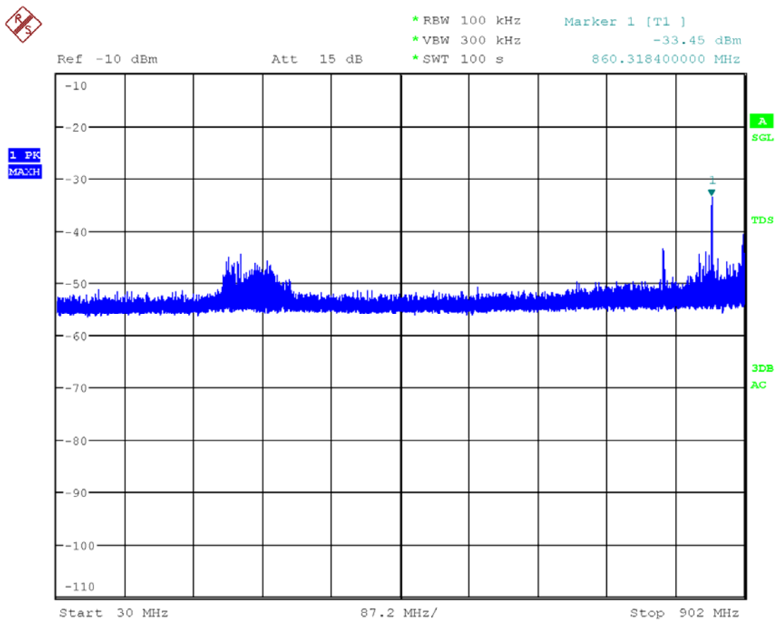
Graph 14: Conducted spurious emissions (non-restricted band), 30 MHz-902 MHz
