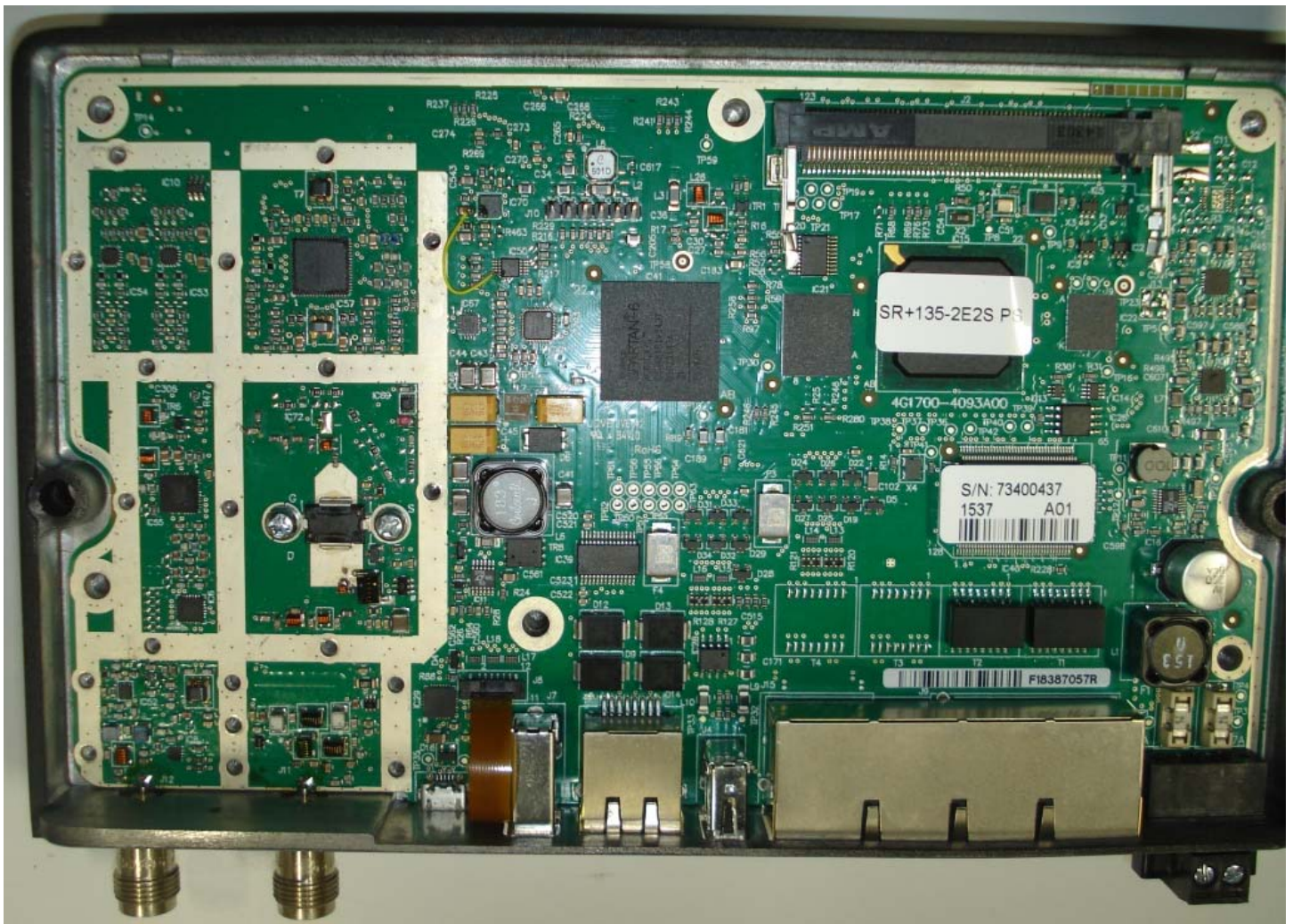
Internal Photo – Shielding Removed
