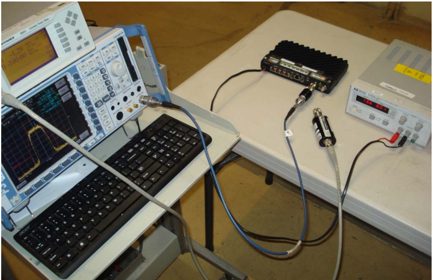
Conducted Power and OBW Set-Up
