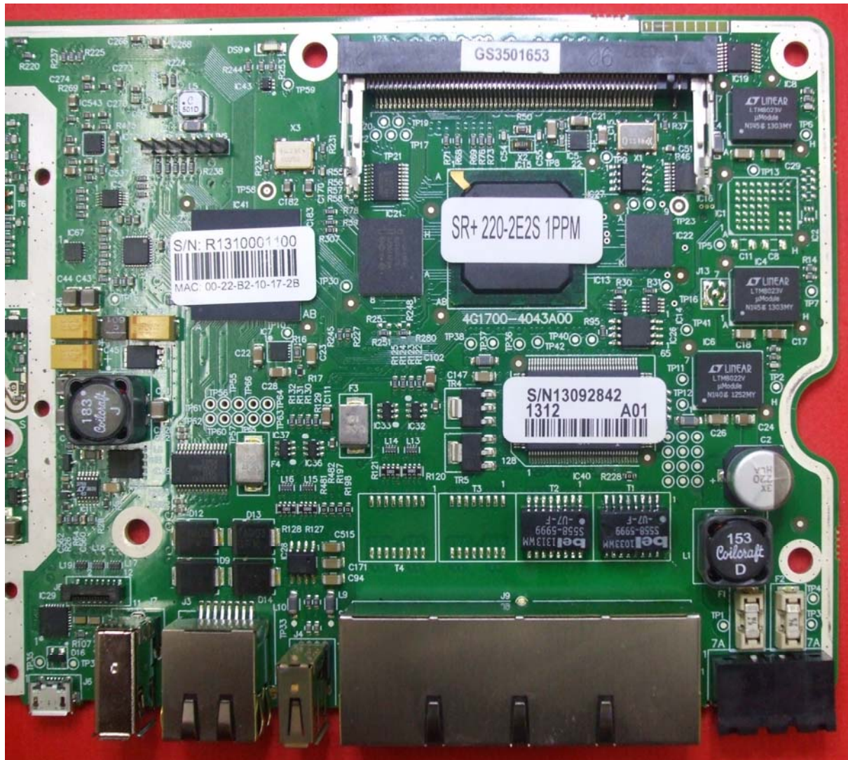
Top side of main board - Right hand side close up
