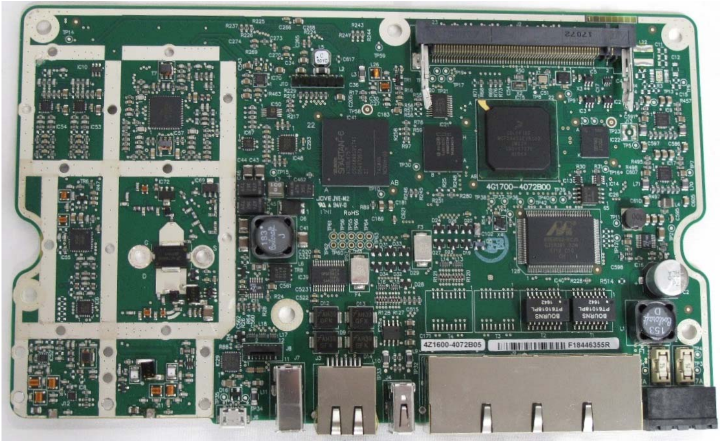
Figure E14.1 – Internal Photo - PCB Top Side
