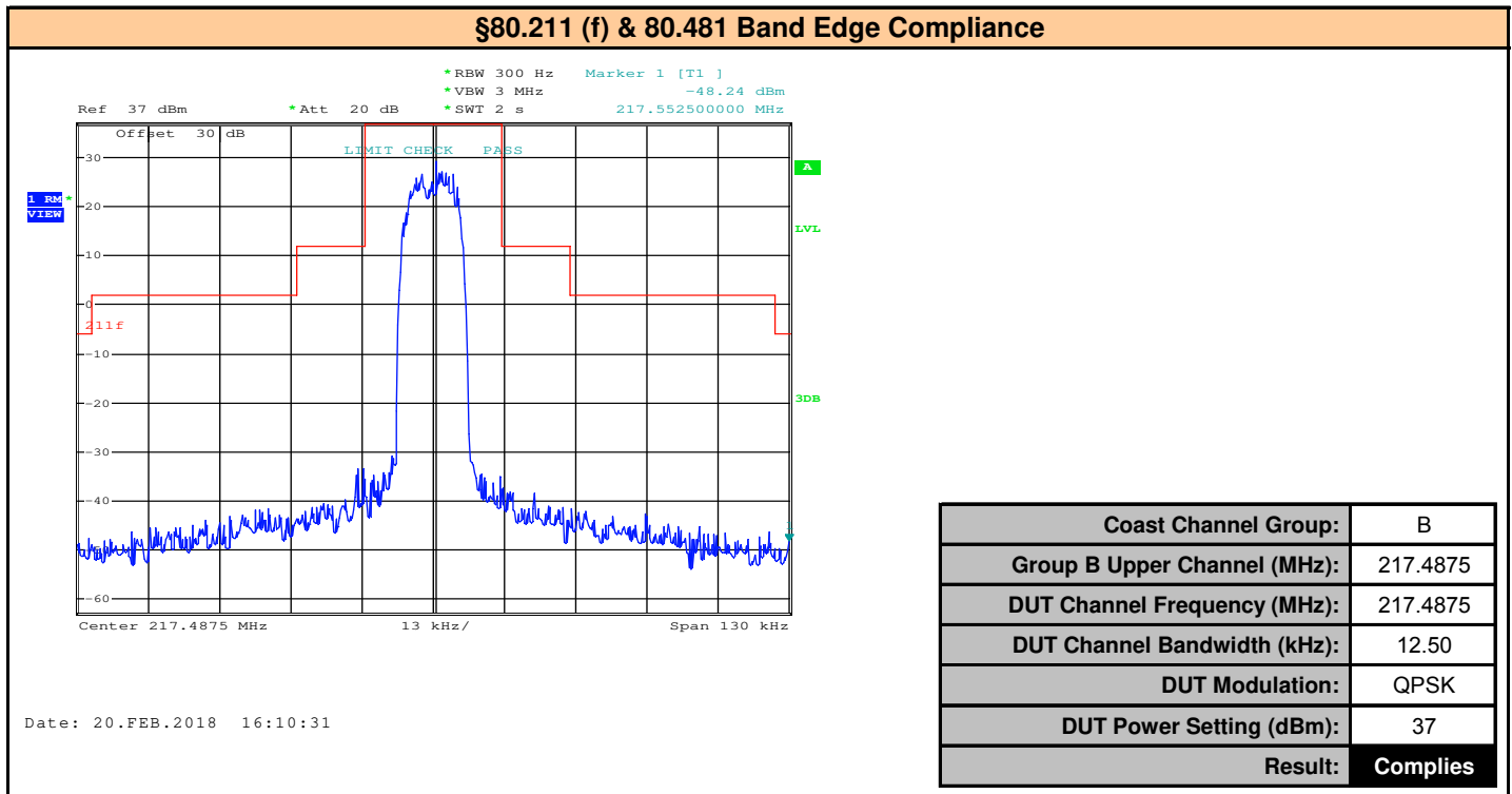
Plot 10.24 – Band Edge, Coast Channel Group B, Upper Channel, 217.4875MHz, 12.5kHz BW, QPSK
