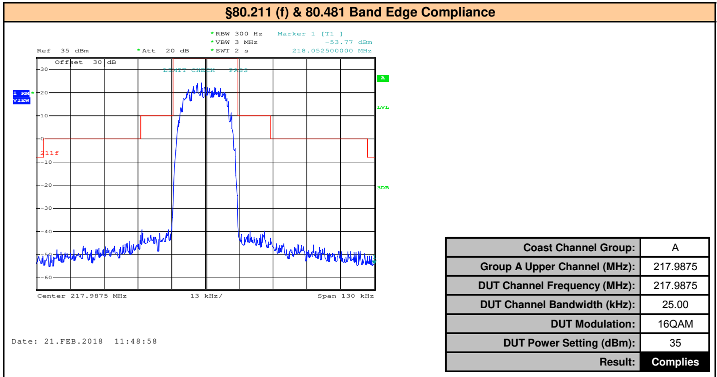
Plot 10.37 – Band Edge, Coast Channel Group A, Upper Channel, 217.9875MHz, 25kHz BW, 16QAM
