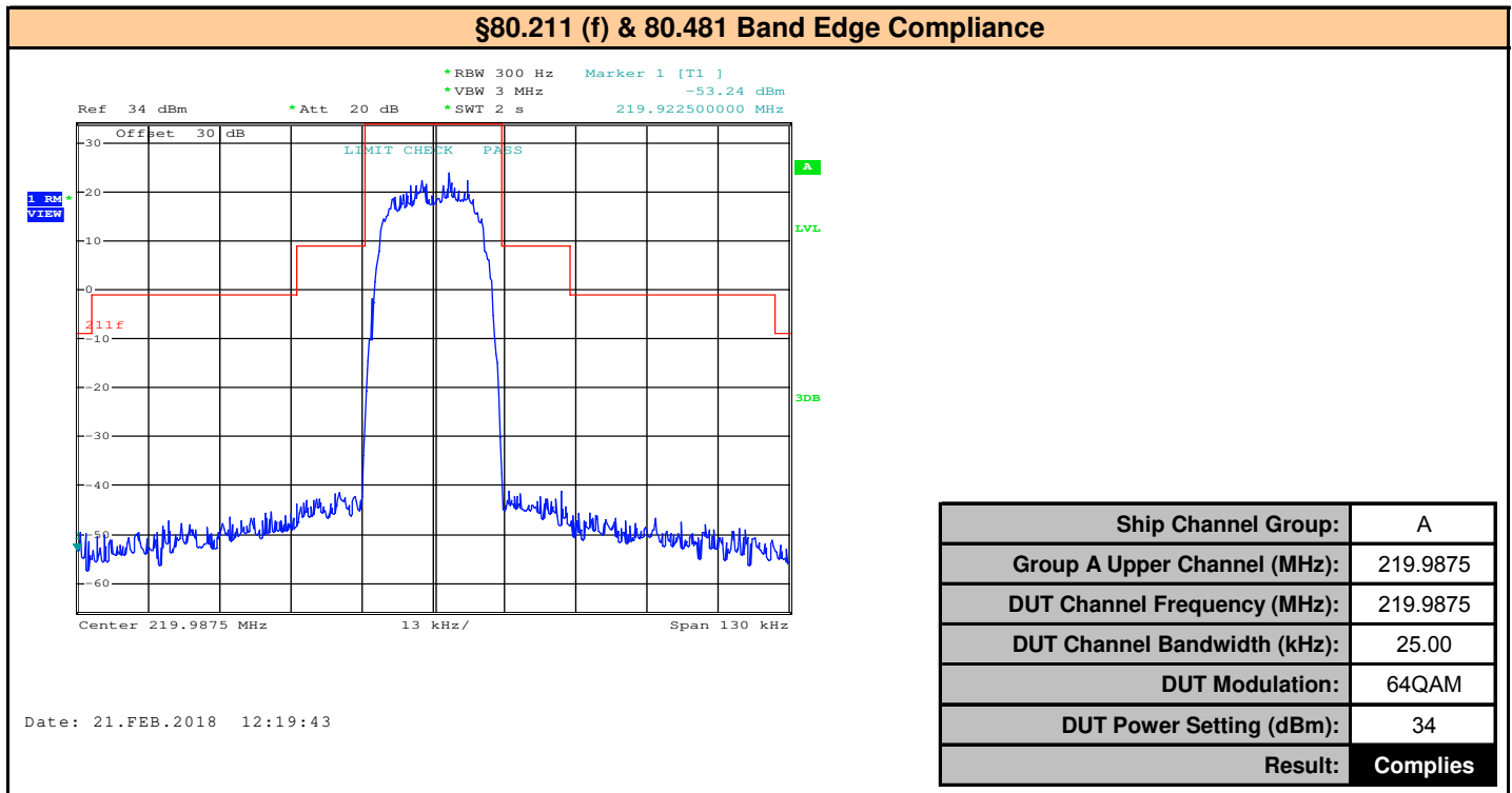
Plot 10.46 – Band Edge, Ship Channel Group A, Upper Channel, 219.9875MHz, 25kHz BW, 64QAM
