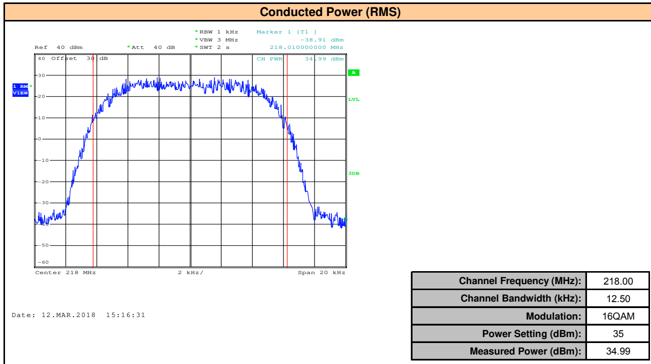
Plot 7.5 – Conducted Power 218MHz, 12.5kHz BW, 16QAM
