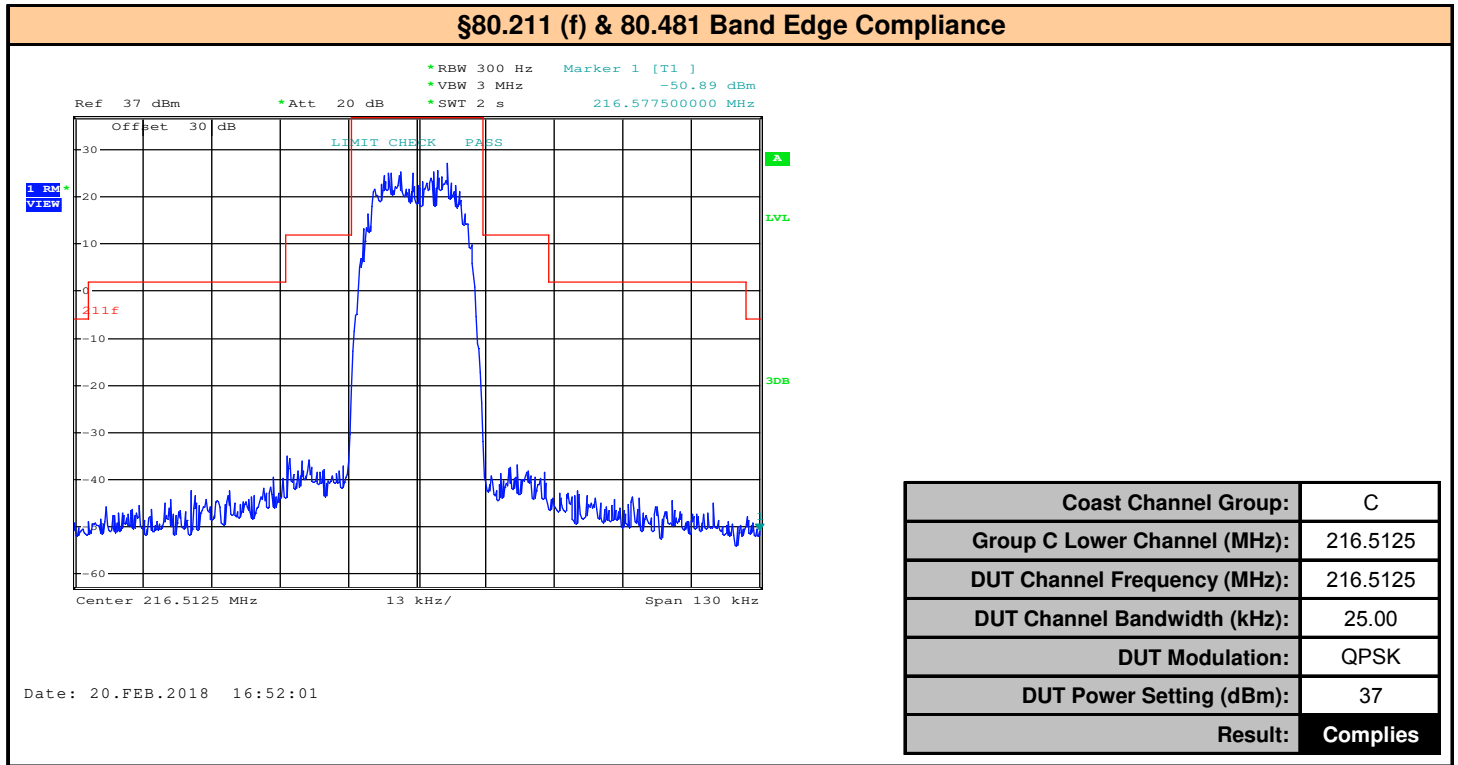
Plot 10.9 – Band Edge, Coast Channel Group C, Lower Channel, 216.5125MHz, 25kHz BW, QPSK
