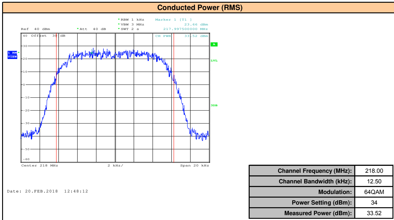
Plot 7.6 – Conducted Power 218MHz, 12.5kHz BW, 64QAM
