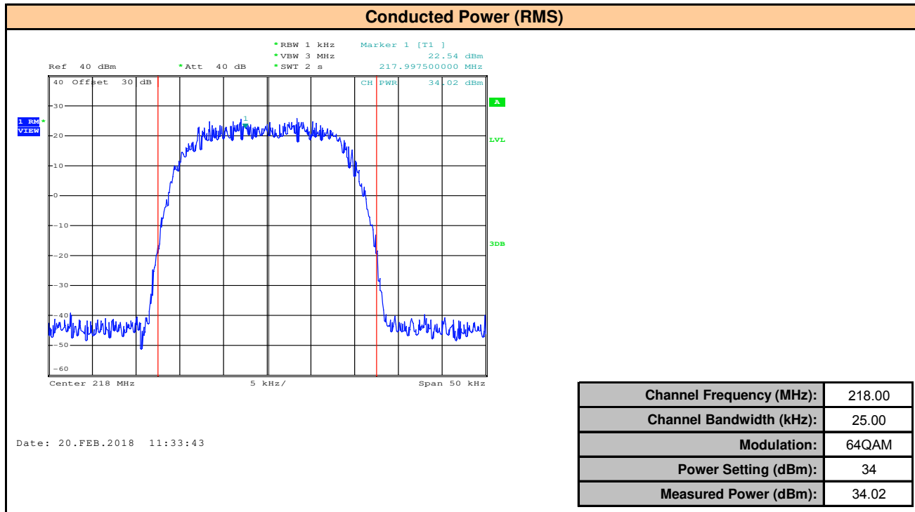
Plot 7.3 – Conducted Power 218MHz, 25kHz BW, 64QAM
