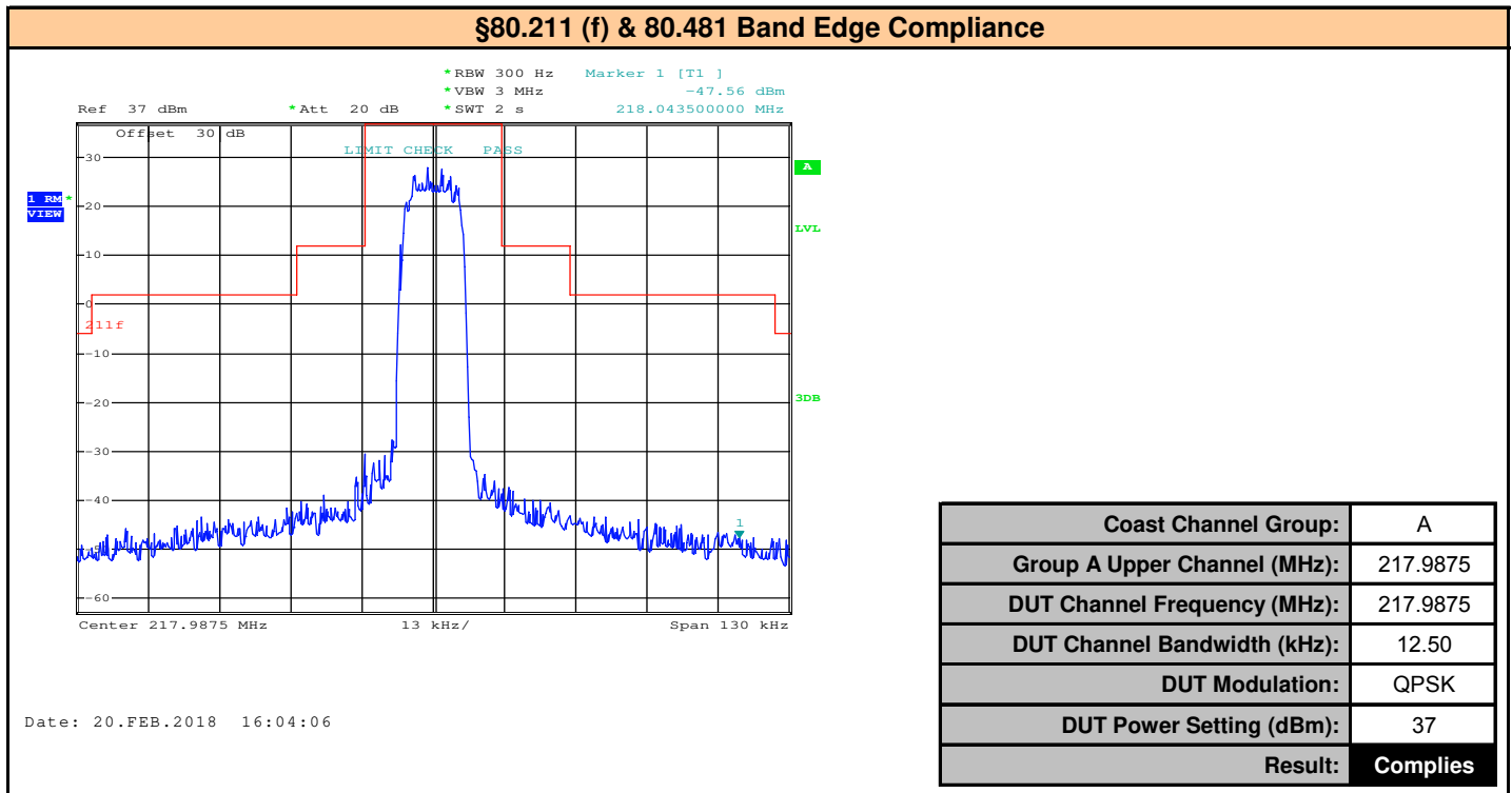
Plot 10.40 – Band Edge, Coast Channel Group A, Upper Channel, 217.9875MHz, 12.5kHz BW, QPSK
