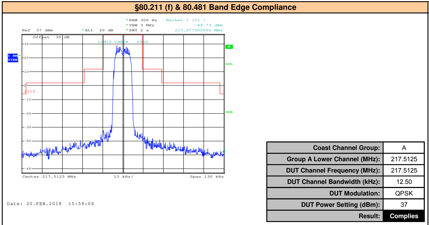
Plot 10.39 – Band Edge, Coast Channel Group A, Lower Channel, 217.5125MHz, 12.5kHz BW, QPSK
