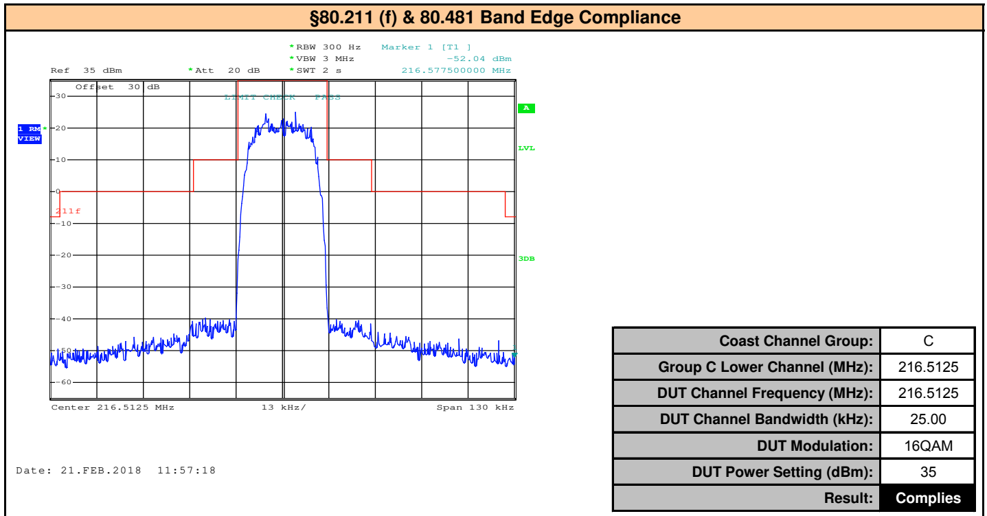
Plot 10.10 – Band Edge, Coast Channel Group C, Lower Channel, 216.5125MHz, 25kHz BW, 16QAM
