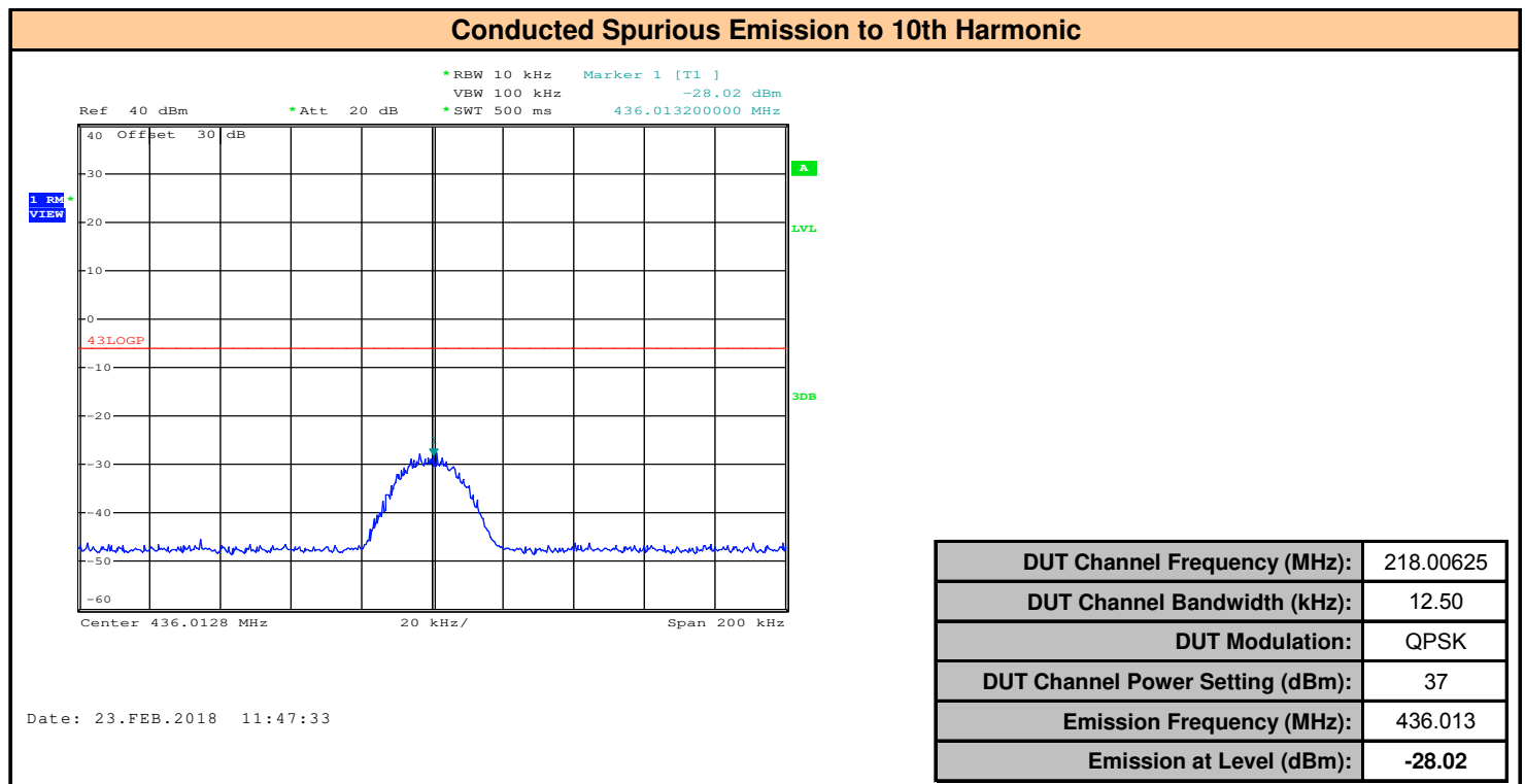
Plot 13.2 – Spurious Emissions 2 nd Harmonic
