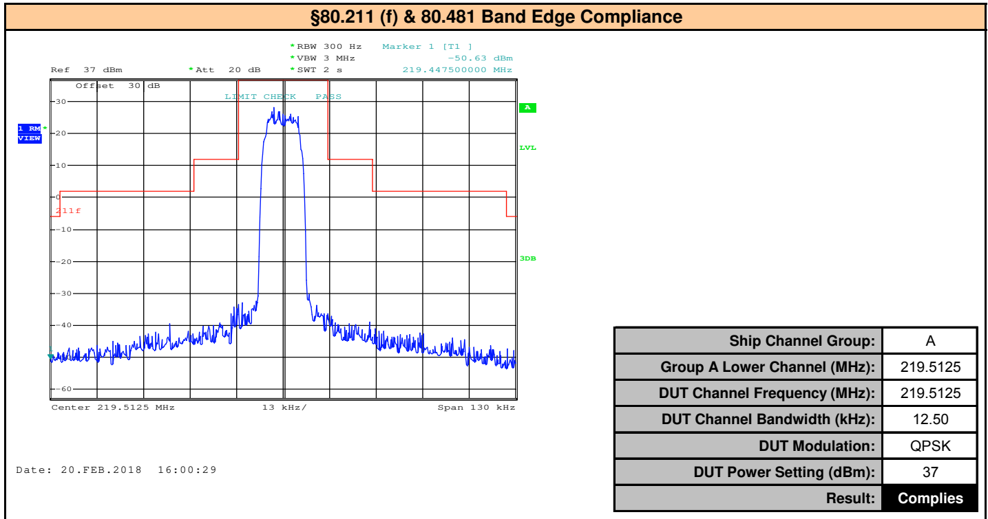
Plot 10.47 – Band Edge, Ship Channel Group A, Lower Channel, 219.5125MHz, 12.5kHz BW, QPSK
