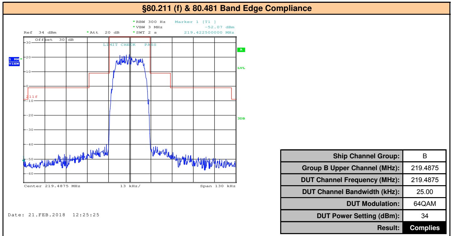
Plot 10.30 – Band Edge, Ship Channel Group B, Upper Channel, 219.4875MHz, 25kHz BW, 64QAM
