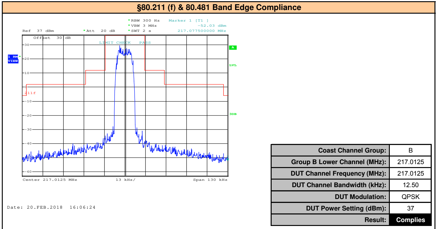
Plot 10.23 – Band Edge, Coast Channel Group B, Lower Channel, 217.0125MHz, 12.5kHz BW, QPSK
