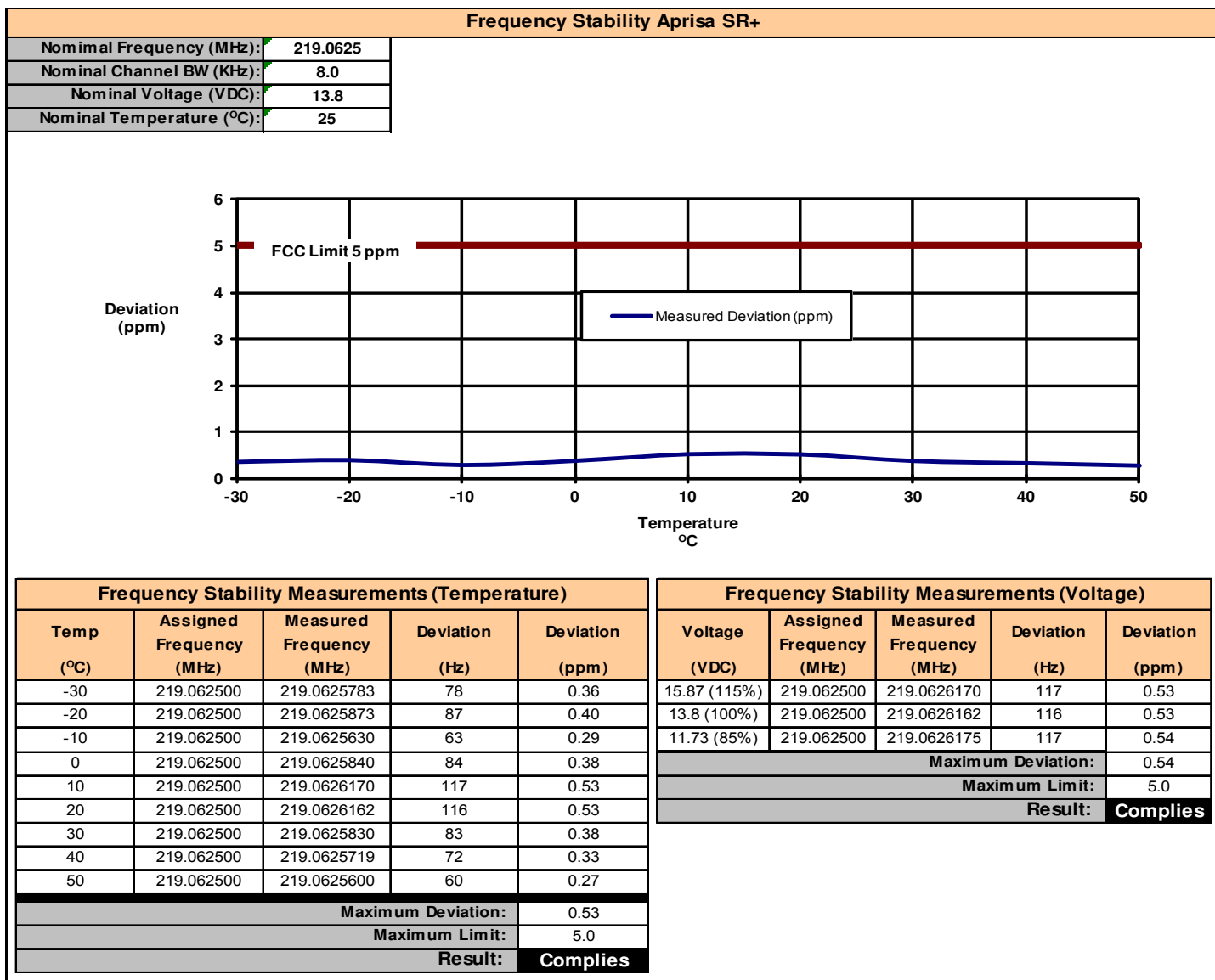
Plot 15.1 – Frequency Stability Aprisa SR+
