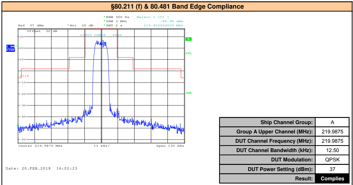
Plot 10.48 – Band Edge, Ship Channel Group A, Upper Channel, 219.9875MHz, 12.5kHz BW, QPSK
