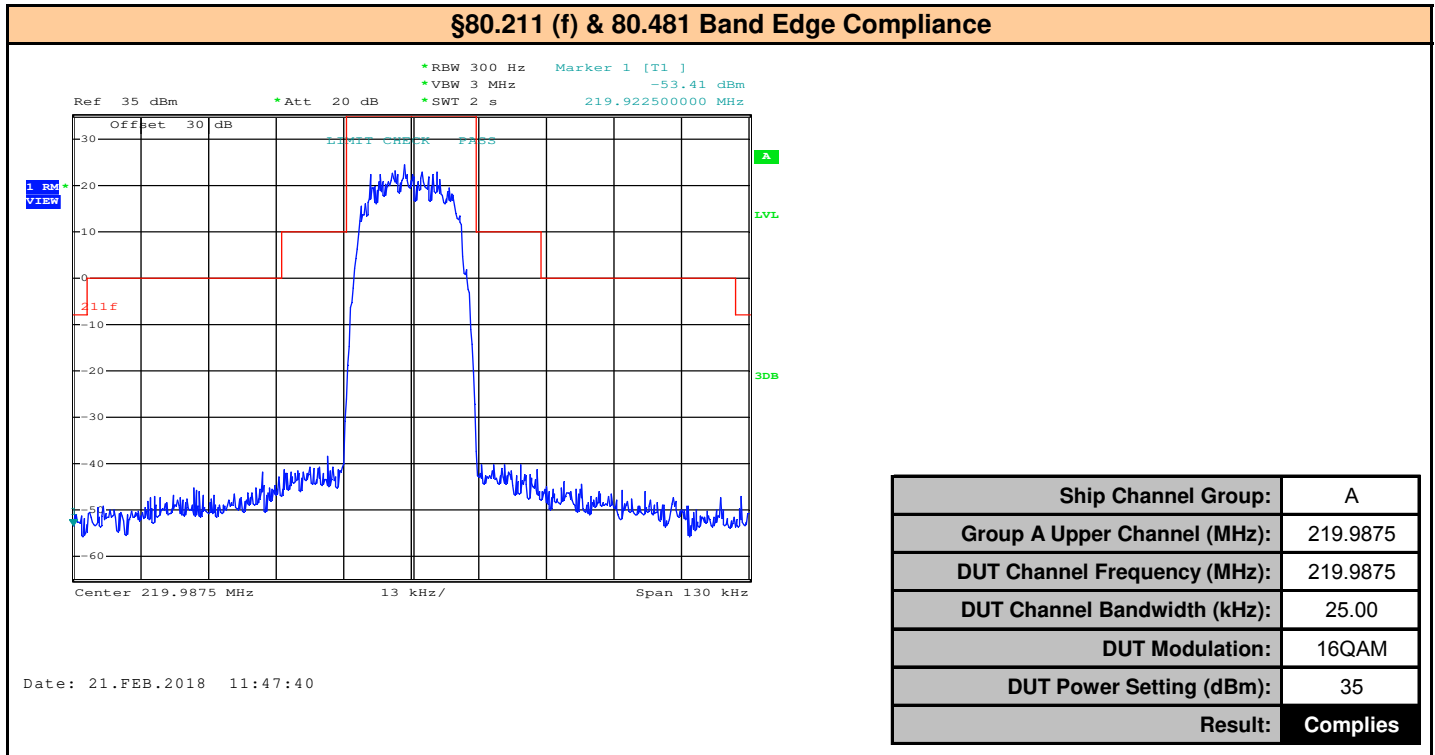
Plot 10.45 – Band Edge, Ship Channel Group A, Upper Channel, 219.9875MHz, 25kHz BW, 16QAM
