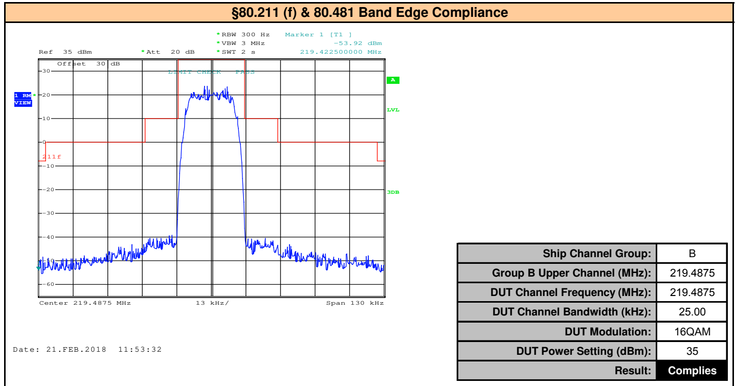
Plot 10.29 – Band Edge, Ship Channel Group B, Upper Channel, 219.4875MHz, 25kHz BW, 16QAM
