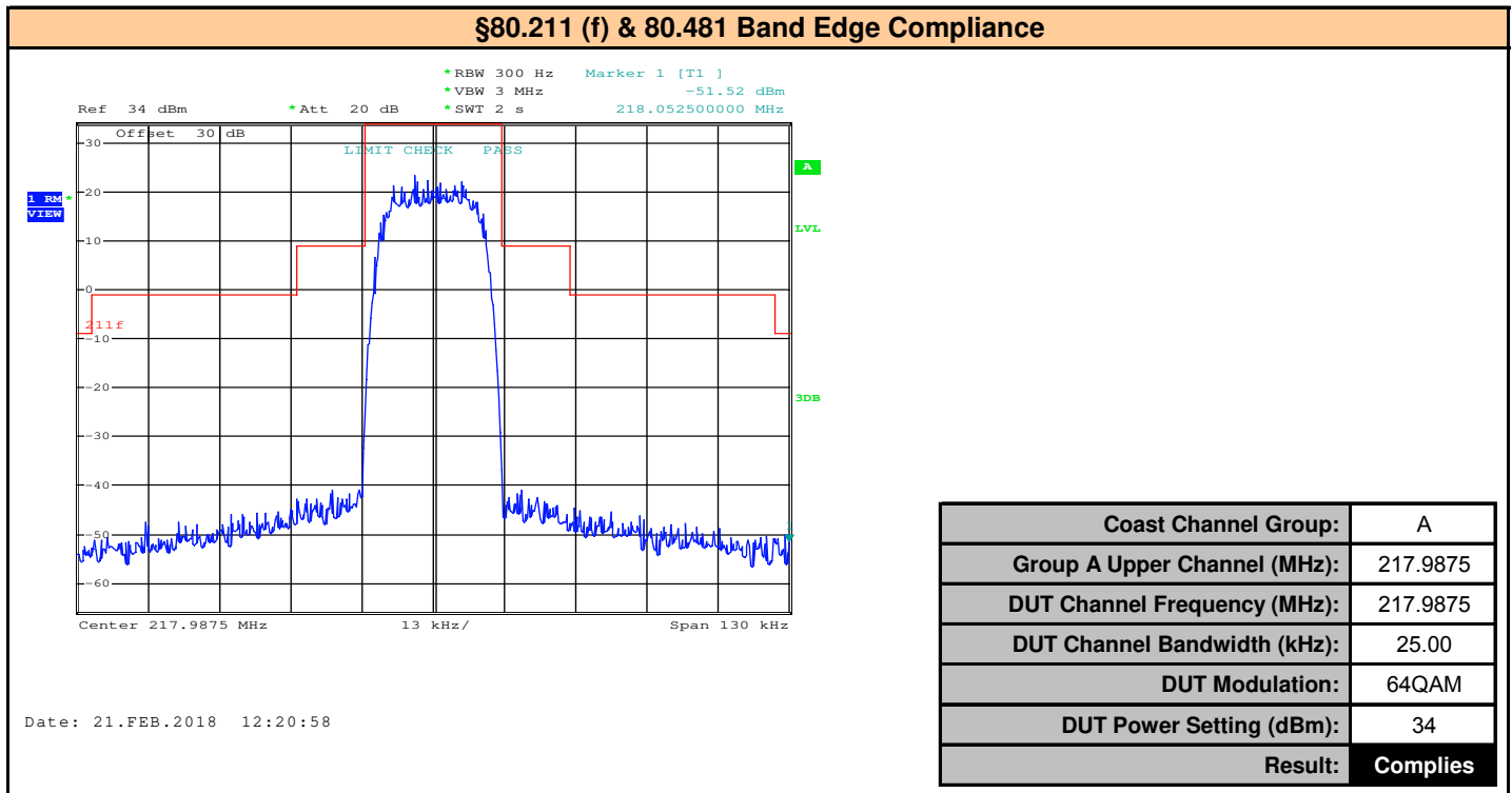
Plot 10.37 – Band Edge, Coast Channel Group A, Upper Channel, 217.9875MHz, 25kHz BW, 64QAM
