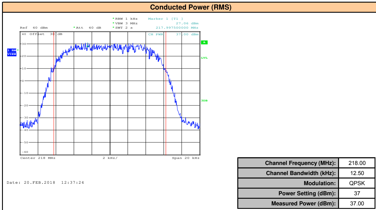
Plot 7.4 – Conducted Power 218MHz, 12.5kHz BW, QPSK
