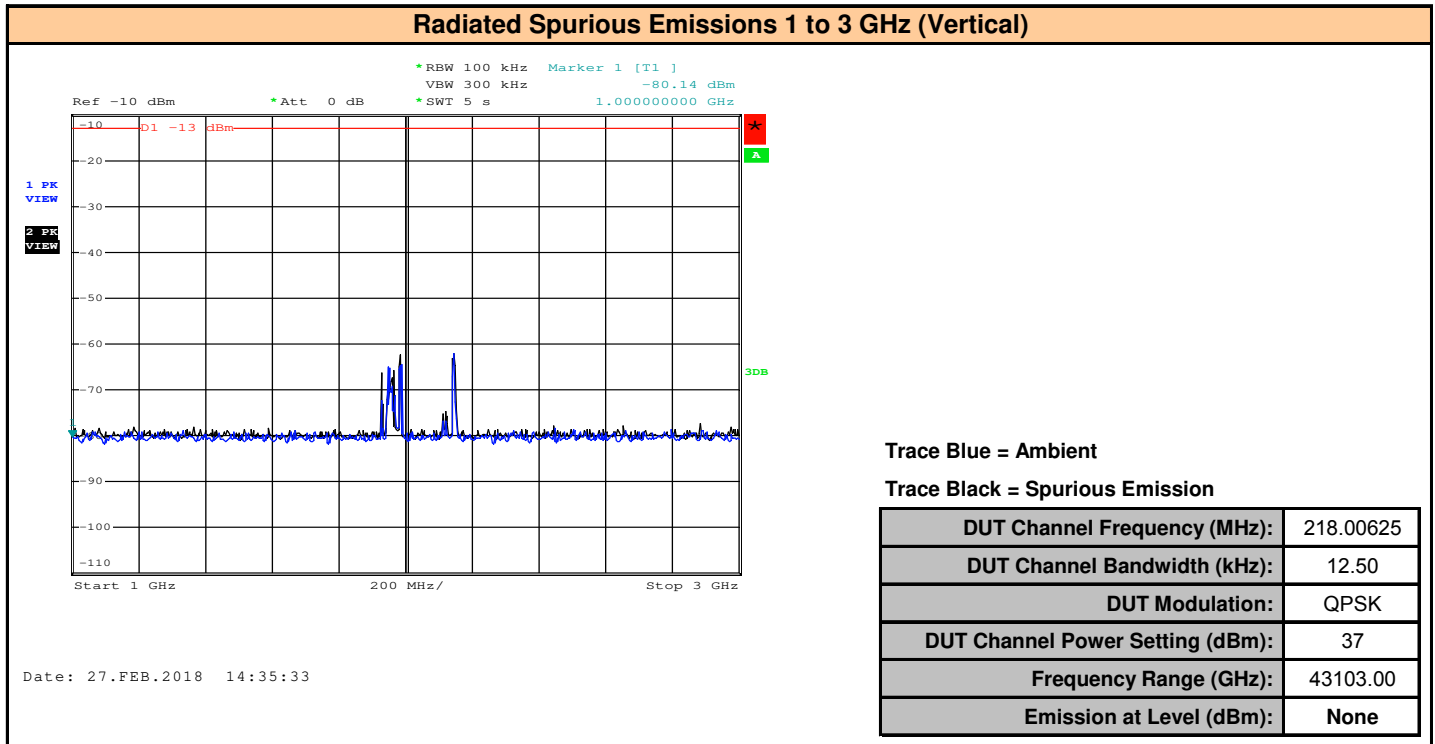
Plot 14.2 – Radiated Spurious Emissions 1 – 3GHz Vertical
