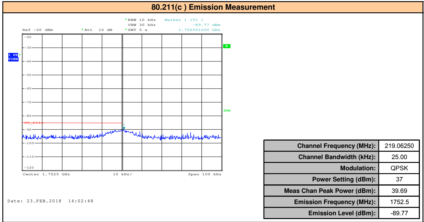
Plot 9.3 – §80.211(c) Emission Mask and Spurious Emissions, Worst Case
