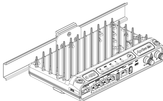
Horizontal Mount
