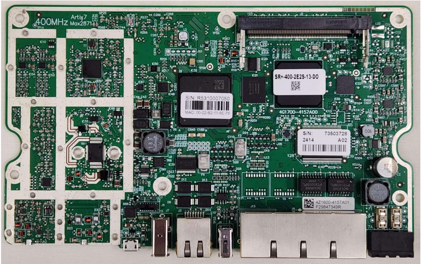
Figure E9.1 – Internal, PCB Top
