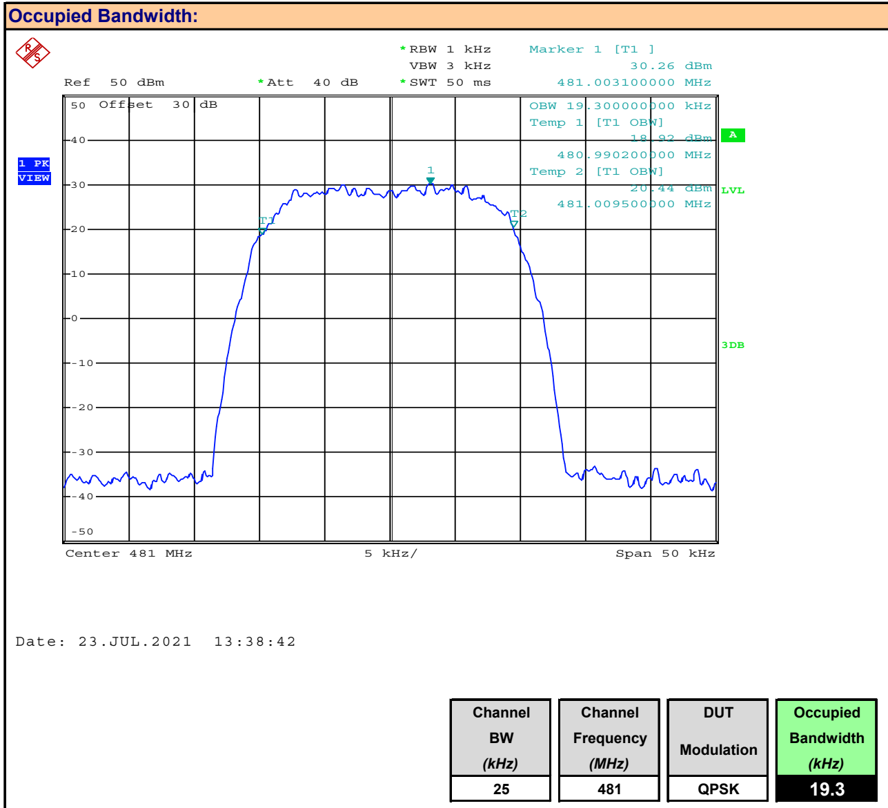
Plot 8.11 – Occupied Bandwidth, 25kHz BW, 481MHz, QPSK
