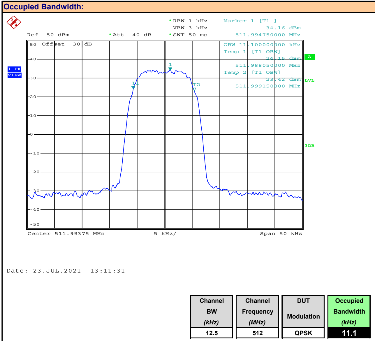
Plot 8.3 – Occupied Bandwidth, 12.5kHz BW, 512MHz, QPSK
