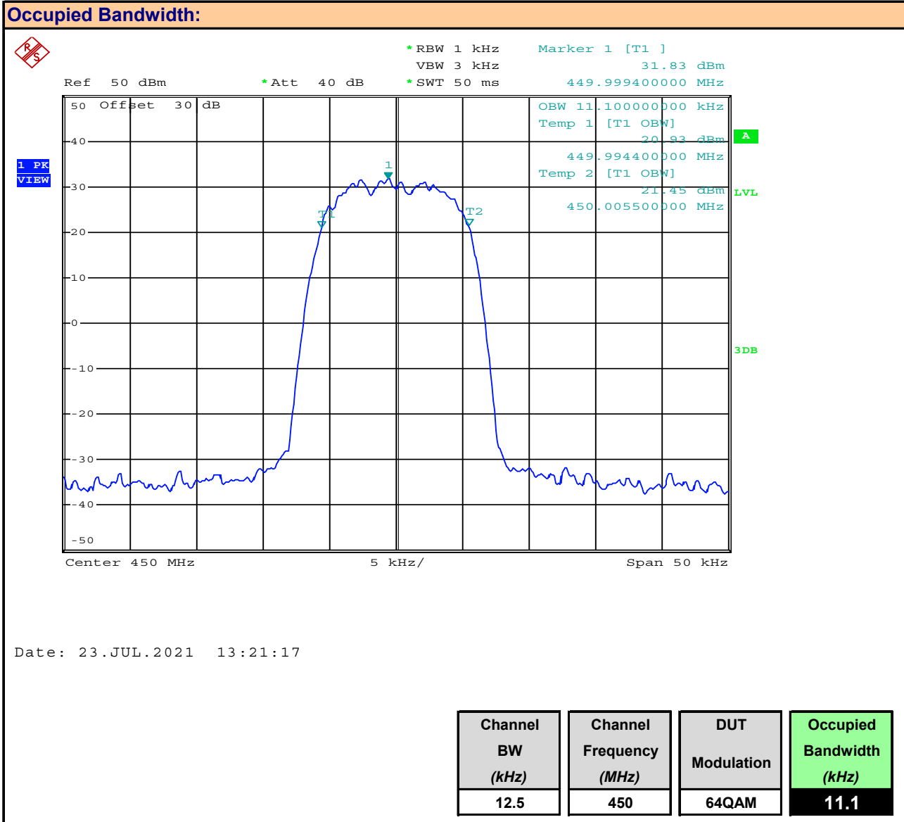
Plot 8.7 – Occupied Bandwidth, 12.5kHz BW, 450MHz, 64QAM
