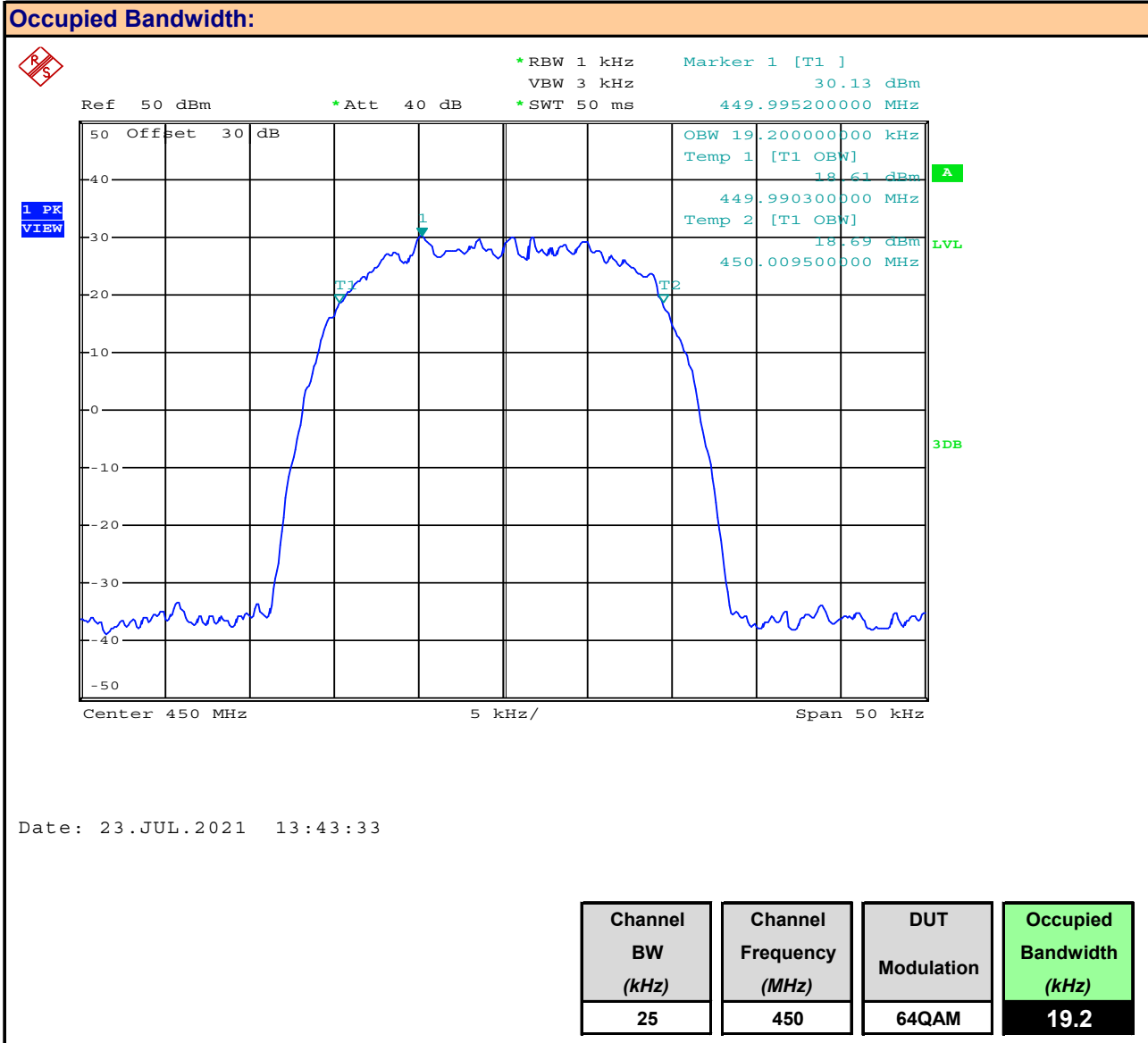
Plot 8.16 – Occupied Bandwidth, 25kHz BW, 450MHz, 64QAM
