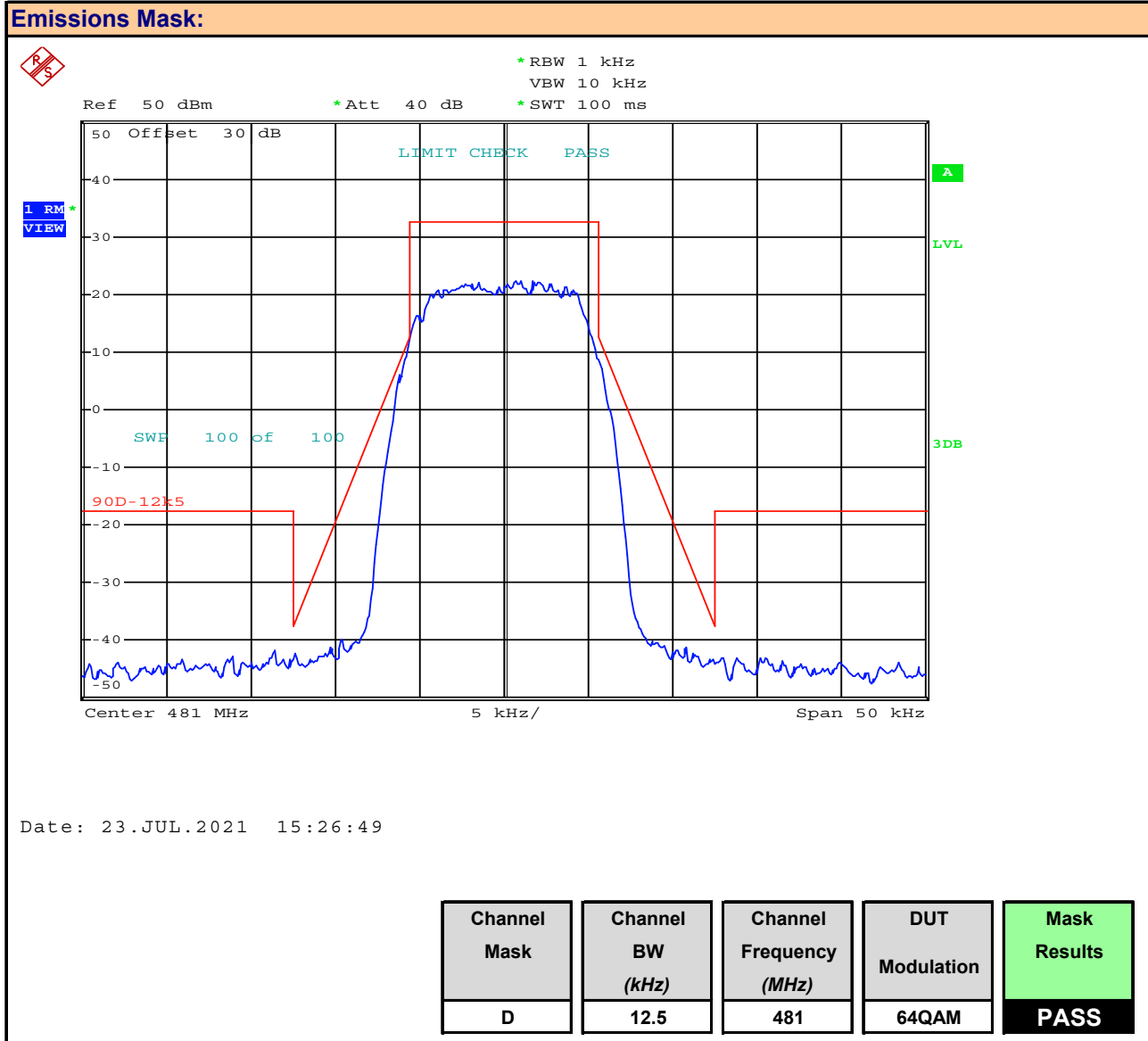
Plot 9.3 – Emissions Mask, 12.5kHz BW, Mask D, 64QAM
