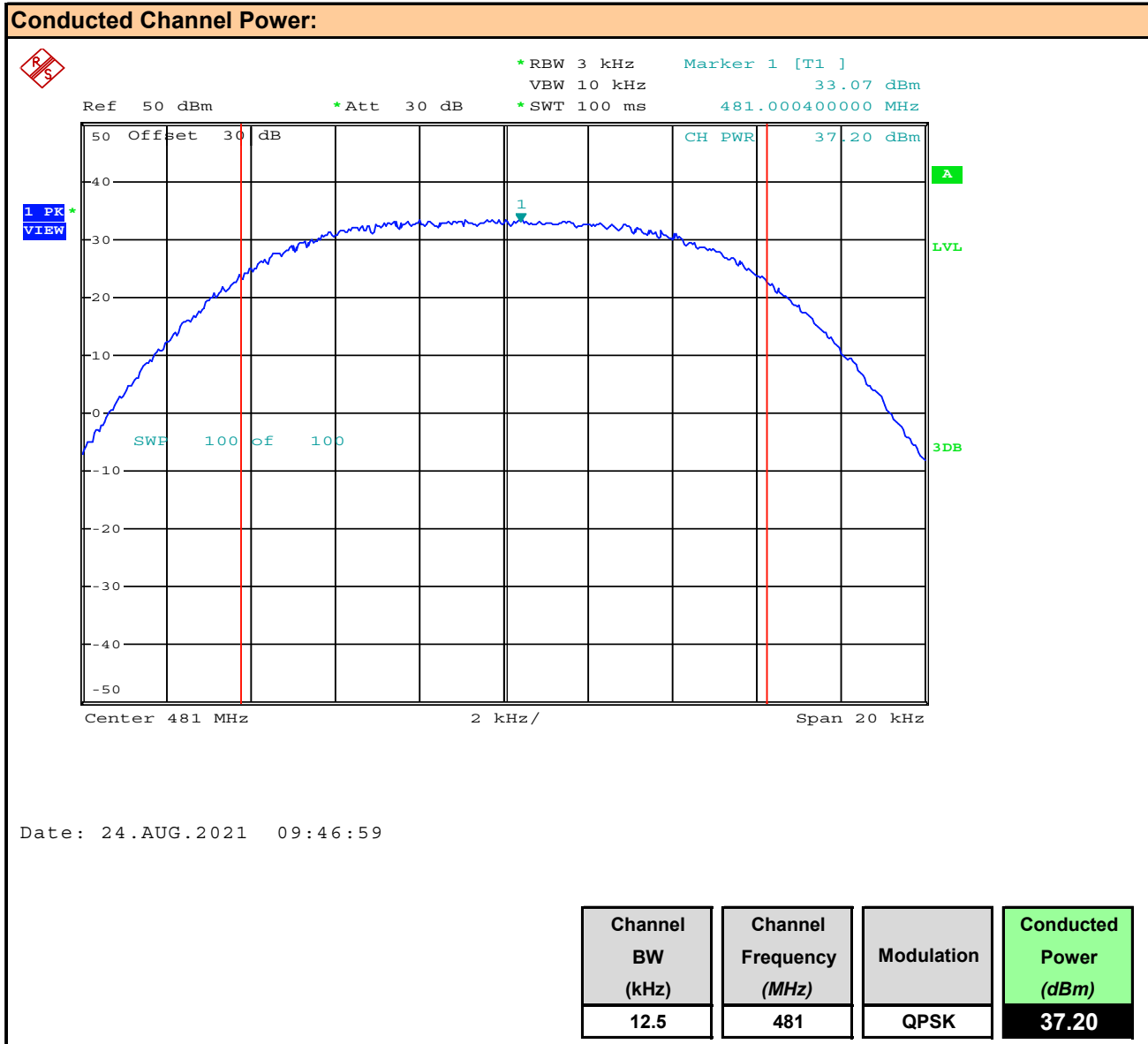
Plot 7.1 – Conducted Power, 12.5kHz BW, QPSK
