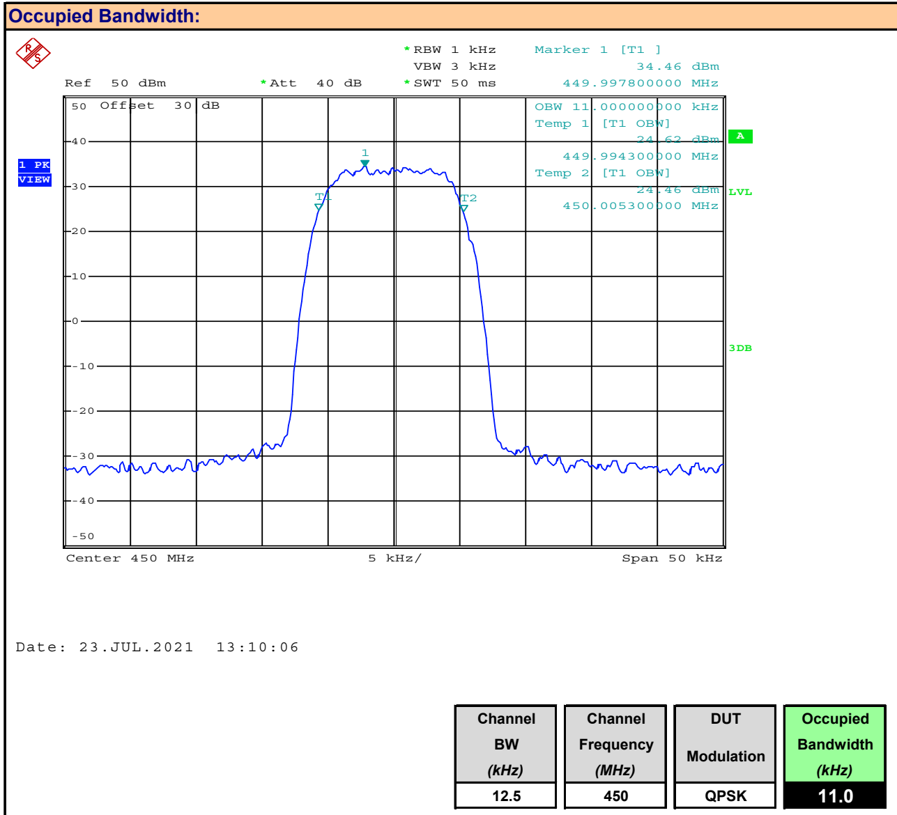
Plot 8.1 – Occupied Bandwidth, 12.5kHz BW, 450MHz, QPSK
