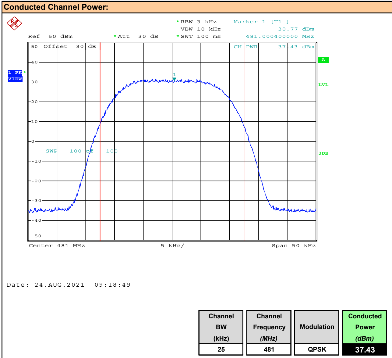
Plot 7.4 – Conducted Power, 25kHz BW, QPSK
