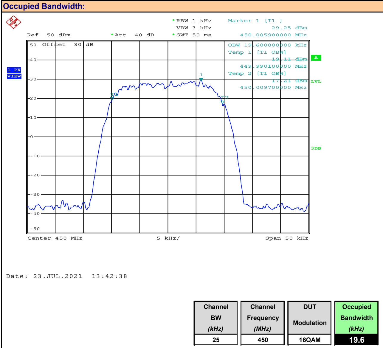
Plot 8.13 – Occupied Bandwidth, 25kHz BW, 450MHz, 16QAM
