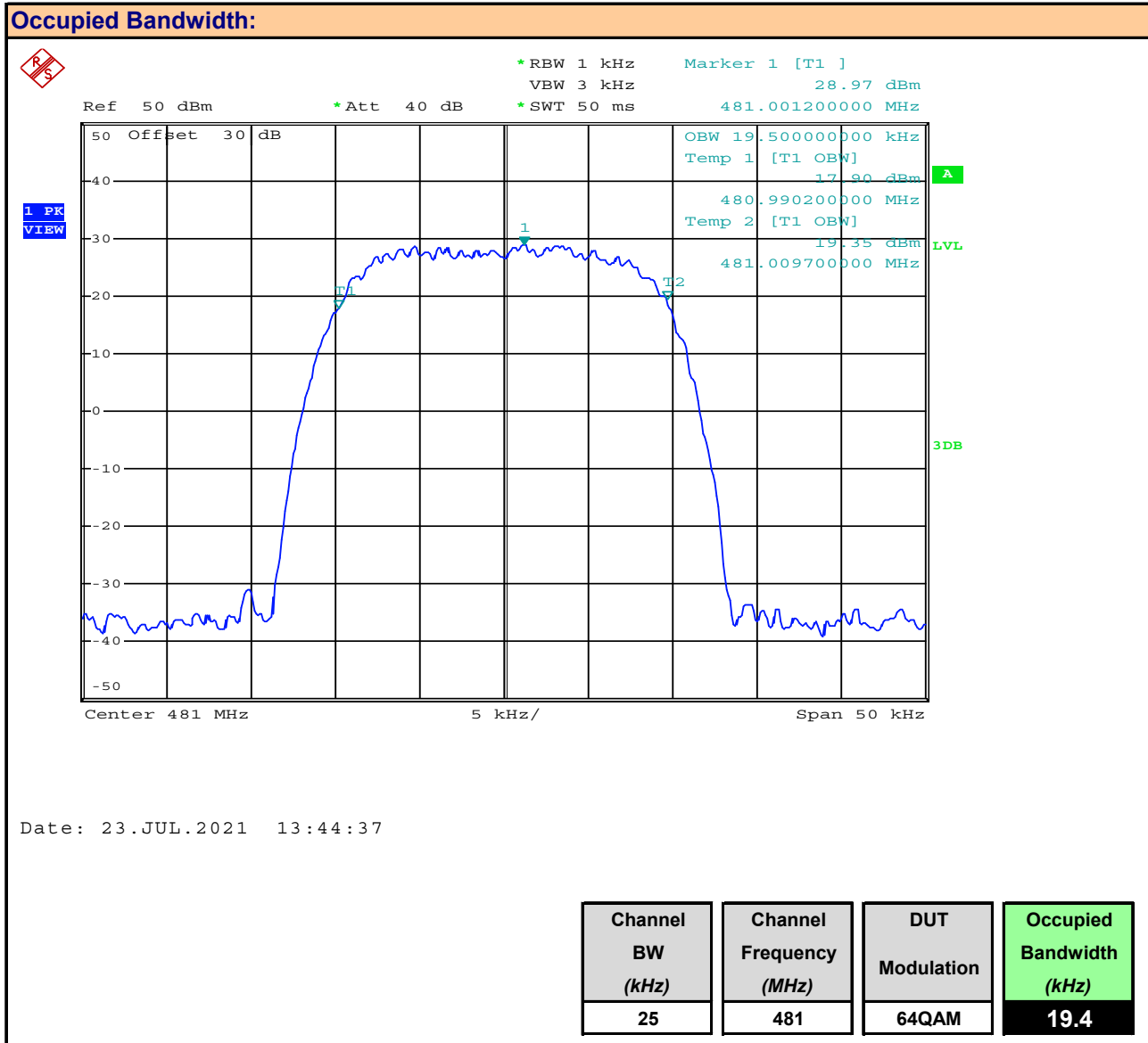
Plot 8.17 – Occupied Bandwidth, 25kHz BW, 481MHz, 64QAM
