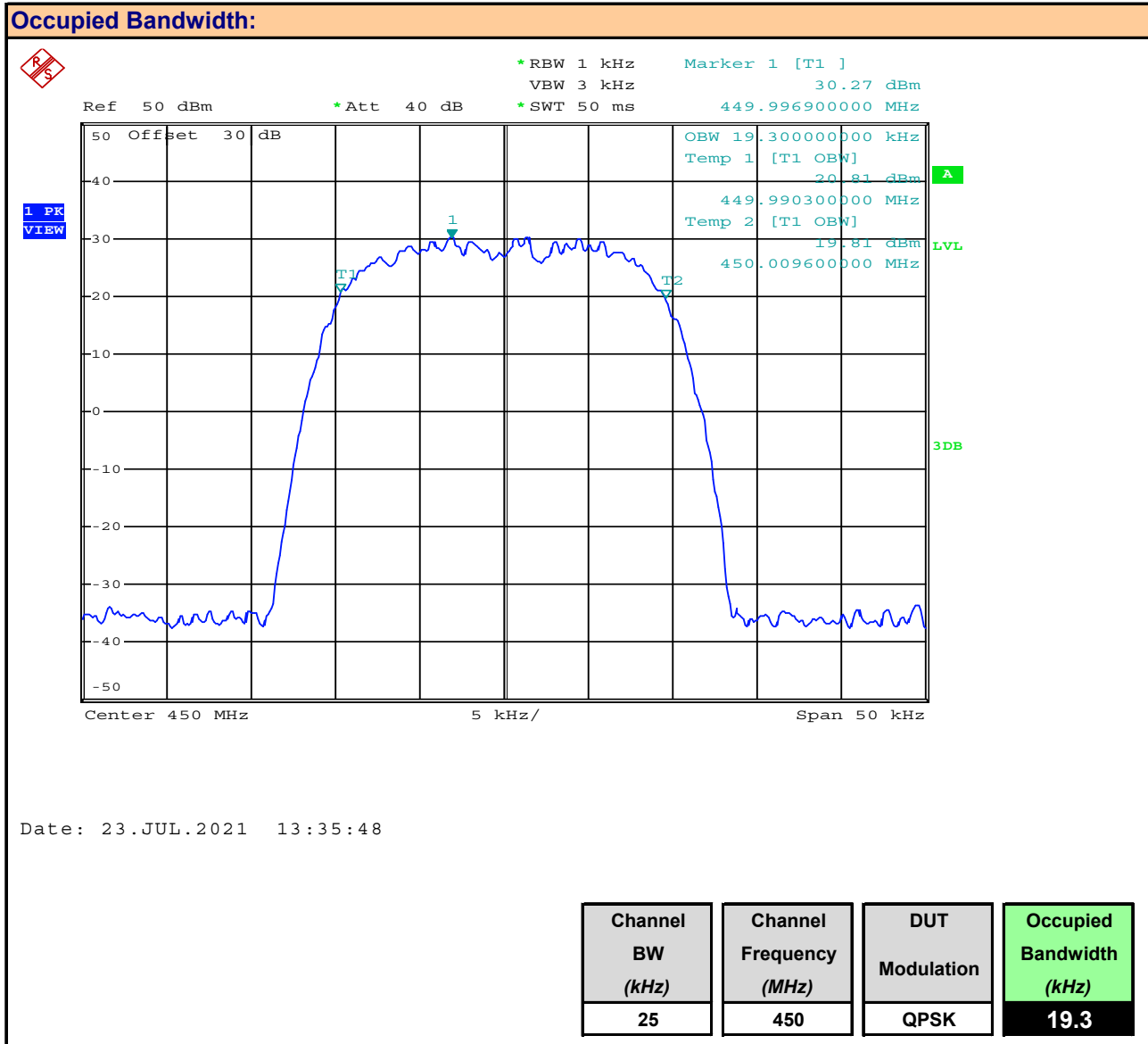
Plot 8.10 – Occupied Bandwidth, 25kHz BW, 450MHz, QPSK
