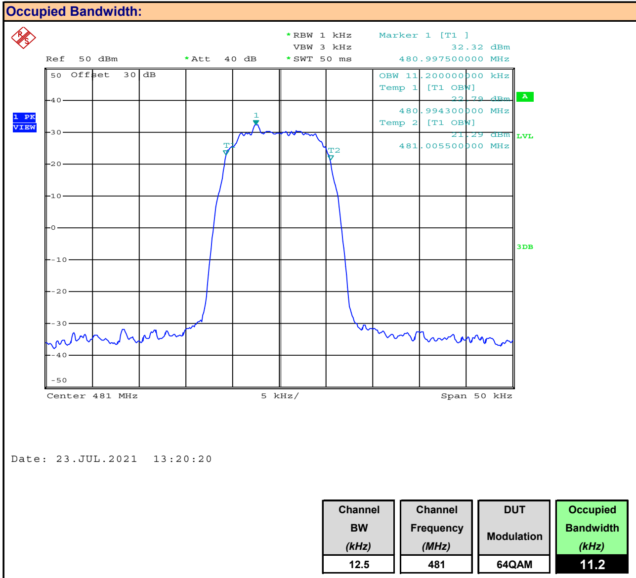
Plot 8.8 – Occupied Bandwidth, 12.5kHz BW, 481MHz, 64QAM
