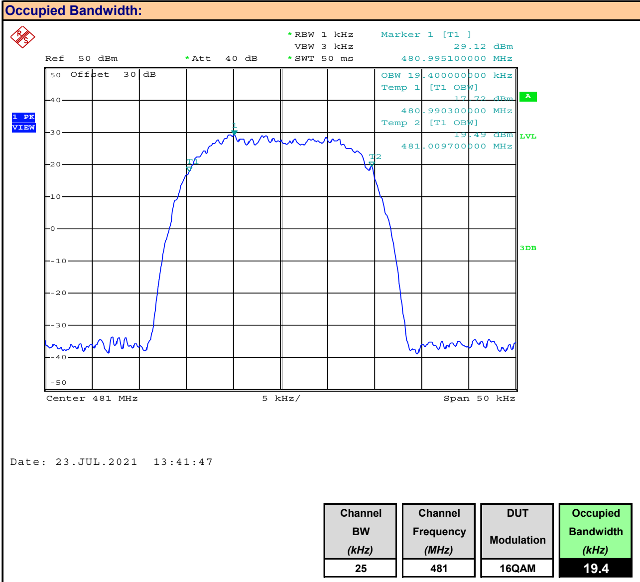
Plot 8.14 – Occupied Bandwidth, 25kHz BW, 481MHz, 16QAM
