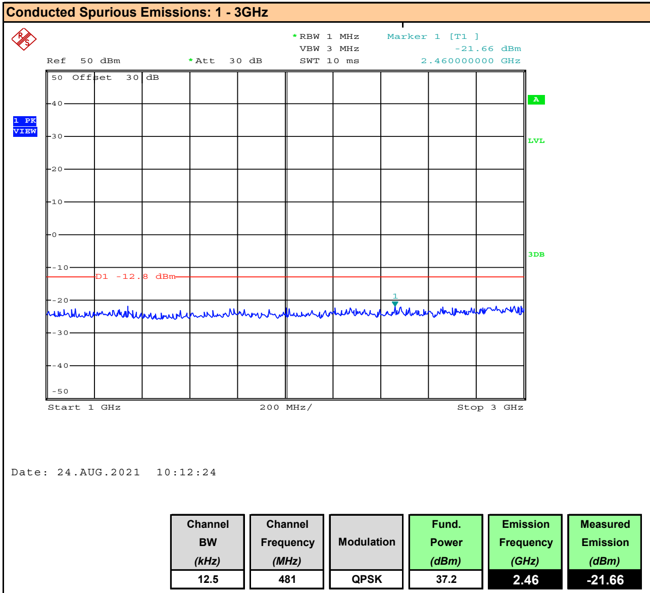
Plot 10.2 – Conducted Spurious Emissions, 1 to 3GHz, 12.5kHz BW
