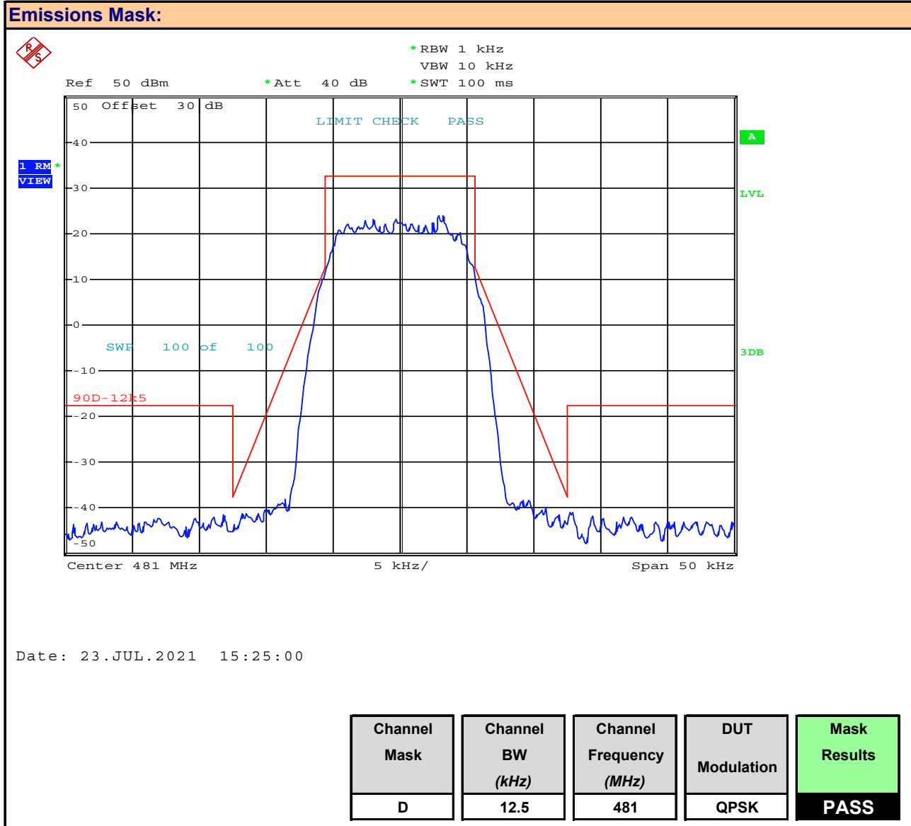
Plot 9.1 – Emissions Mask, 12.5kHz BW, Mask D, QPSK
