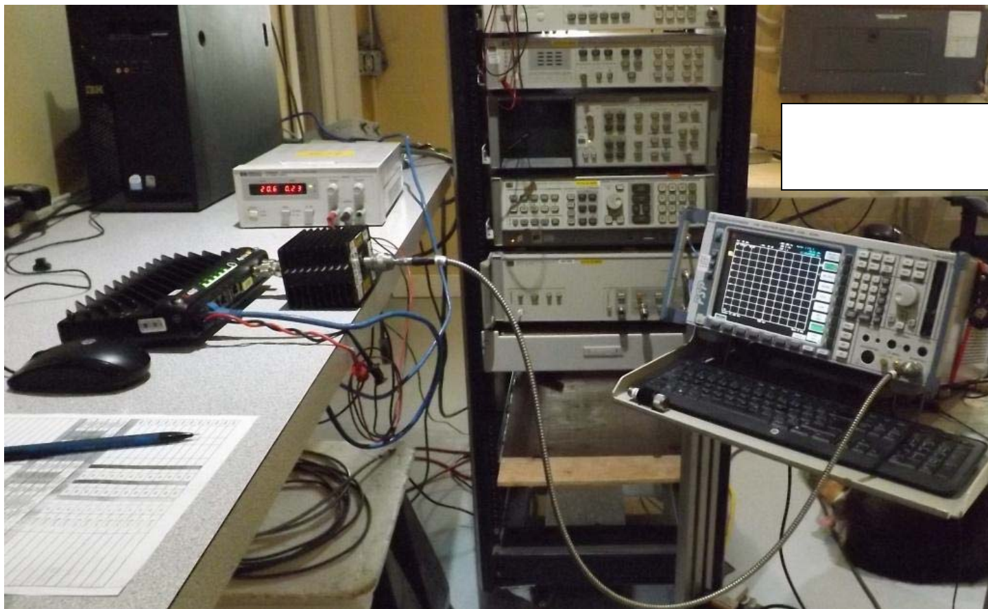
Figure E10.1 – Setup – Conducted Measurements
