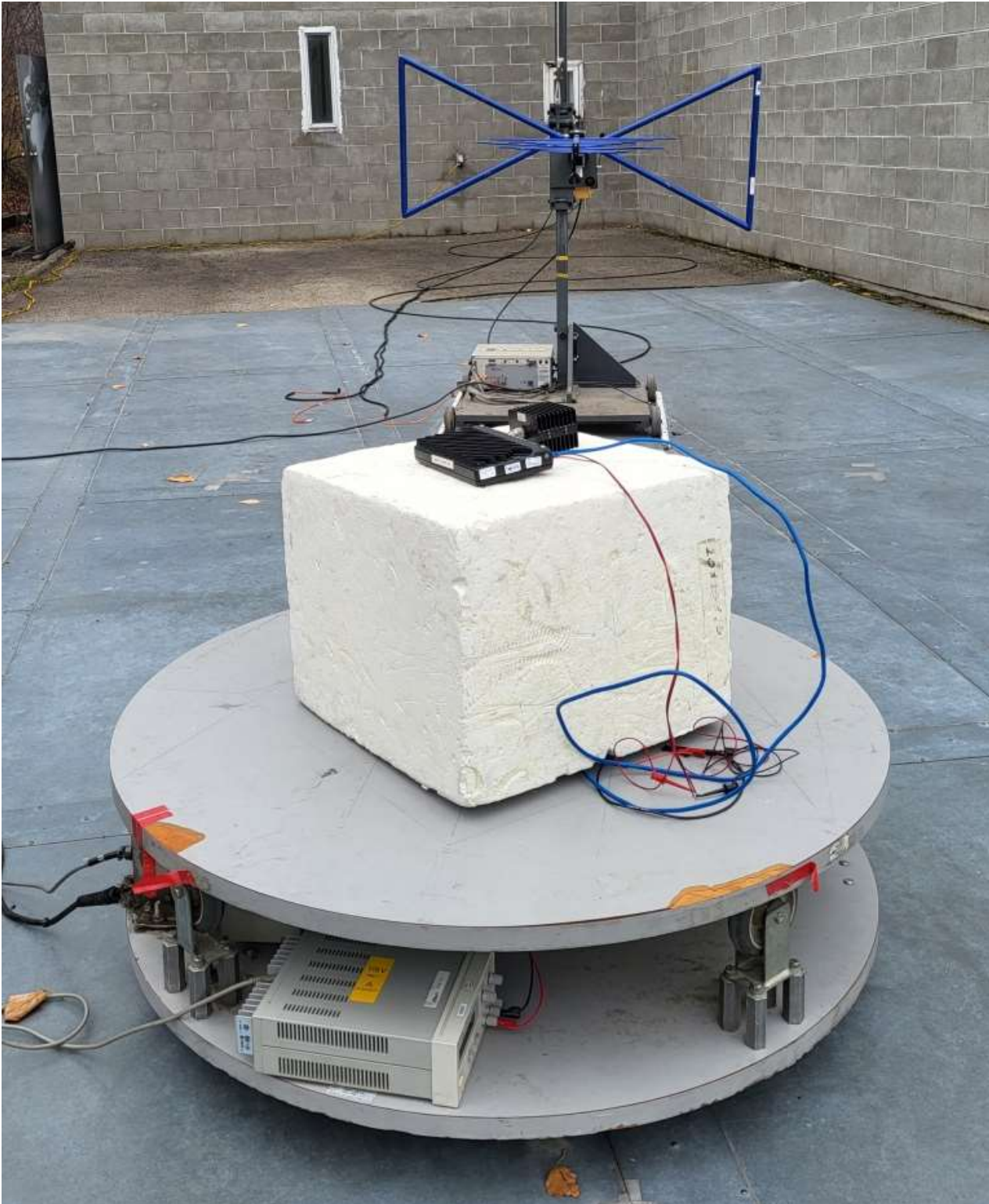
Figure E12.2 – Setup, Radiated Measurements Below 1GHz
