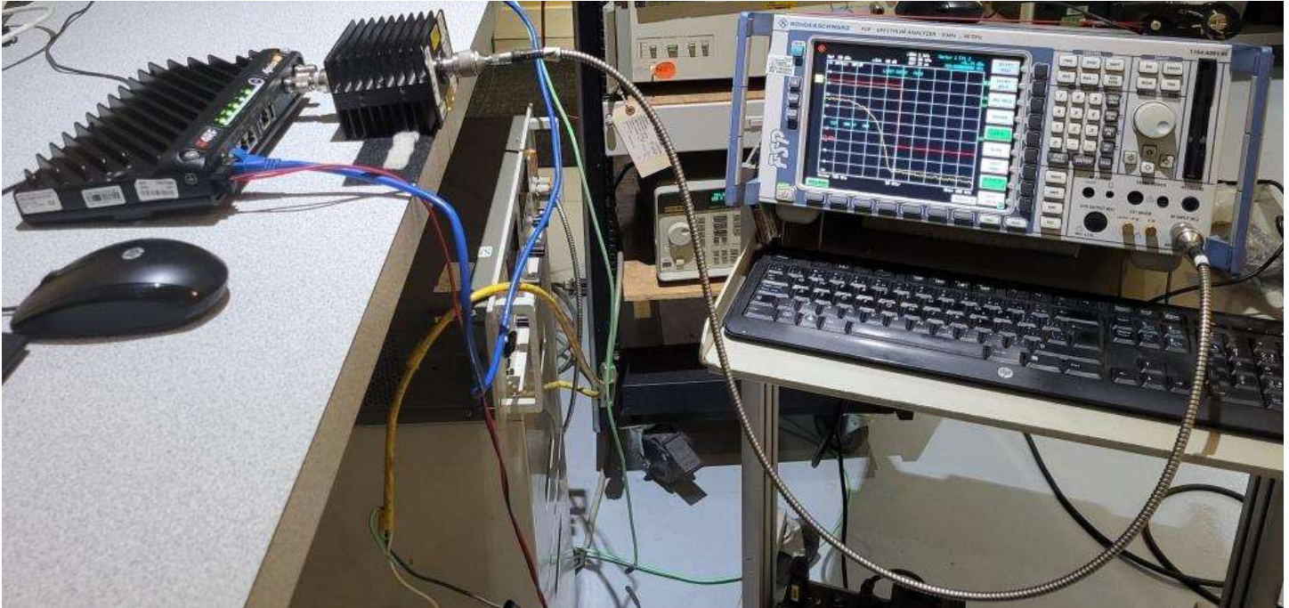
Figure E12.1 – Setup, Conducted Measurements
