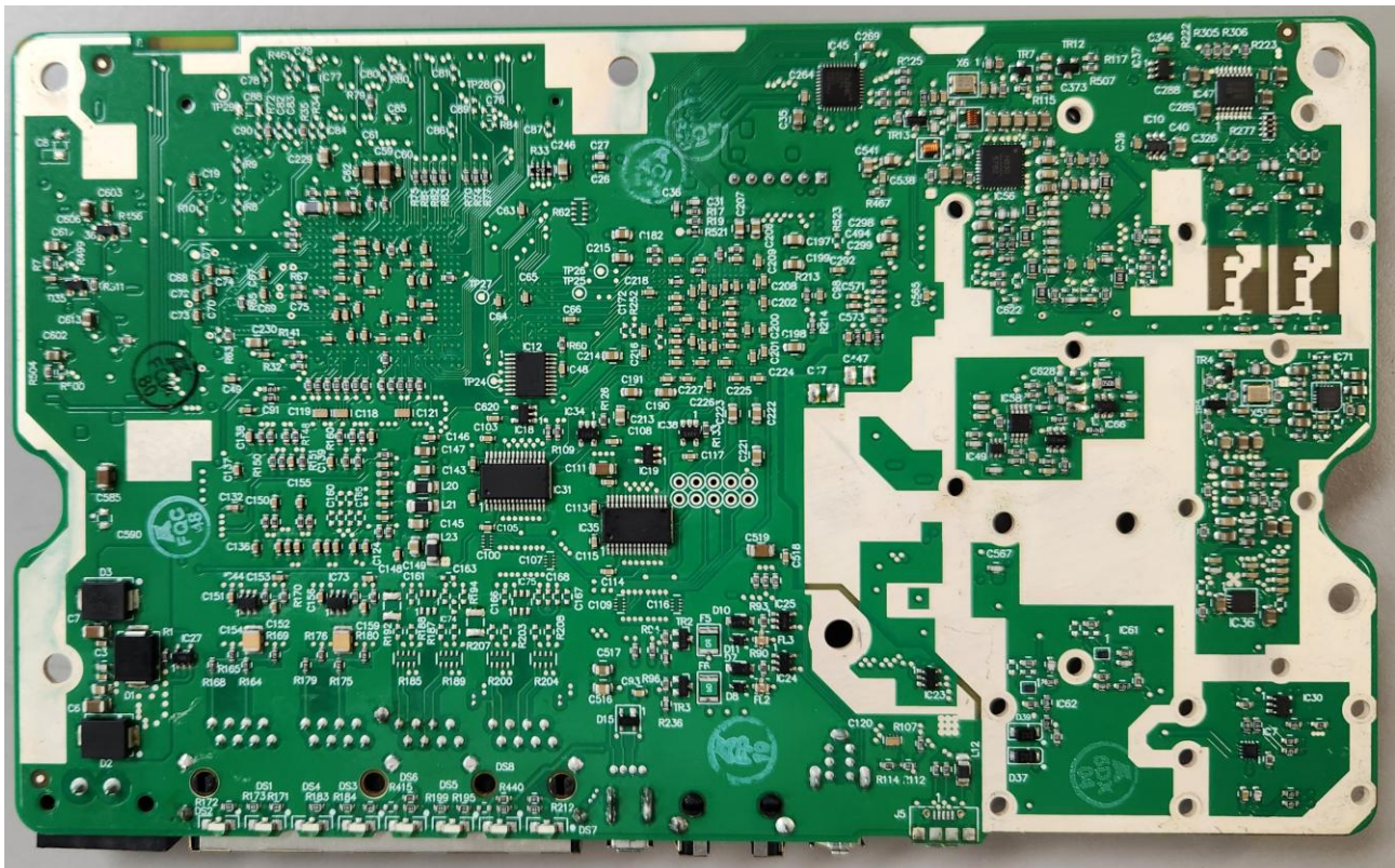
Figure 4: Old PCA Photo bottom view
