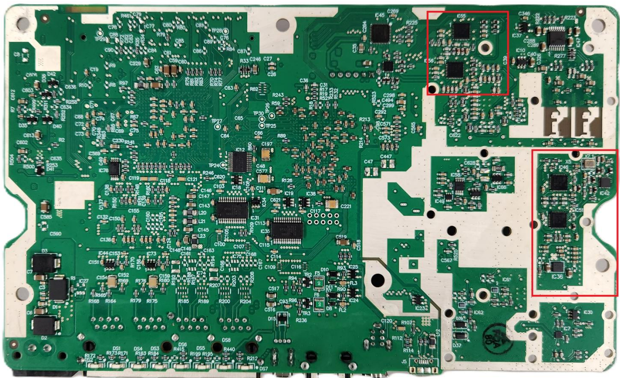
Figure 8: New PCA photo bottom view (changed areas highlighted)
