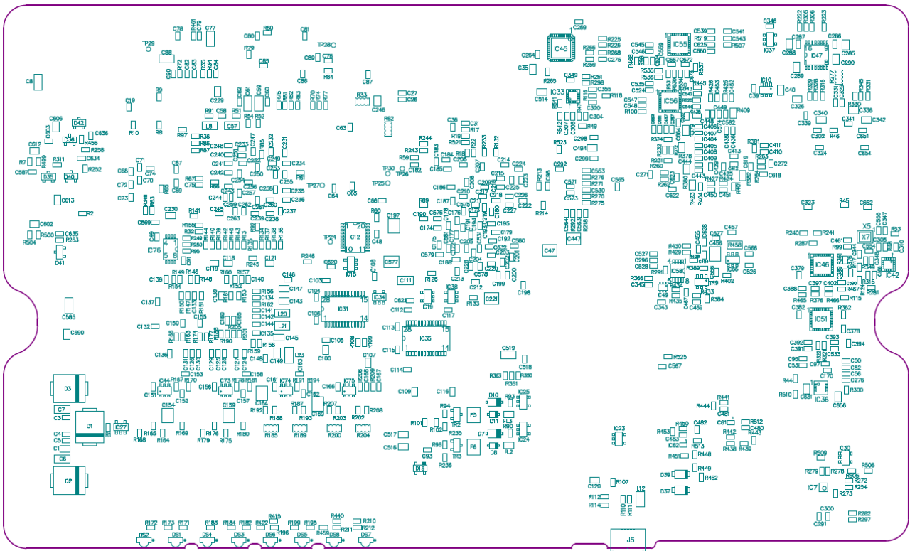
Figure 7: New PCA layout bottom view
