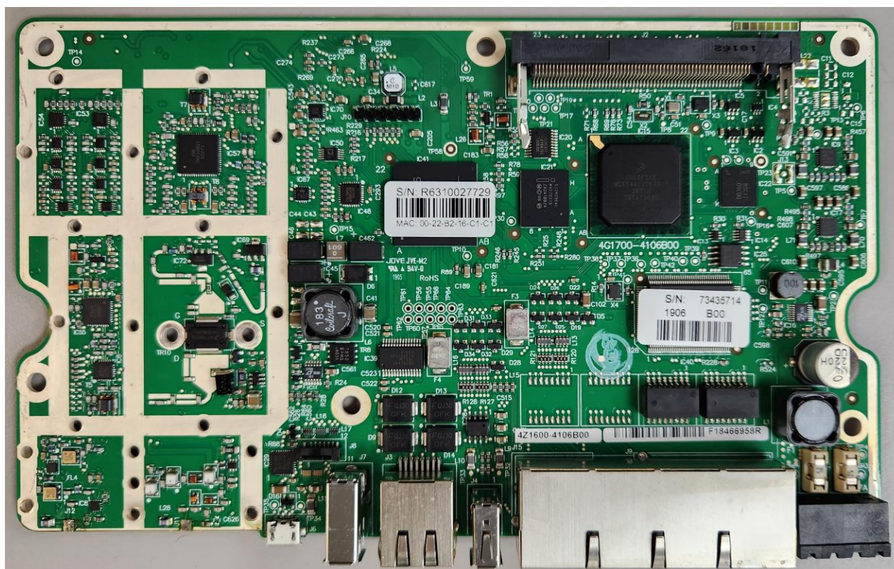
Figure 2: Old PCA photo top view
