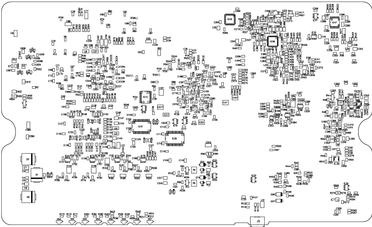
Figure 3: Old PCA layout bottom view
