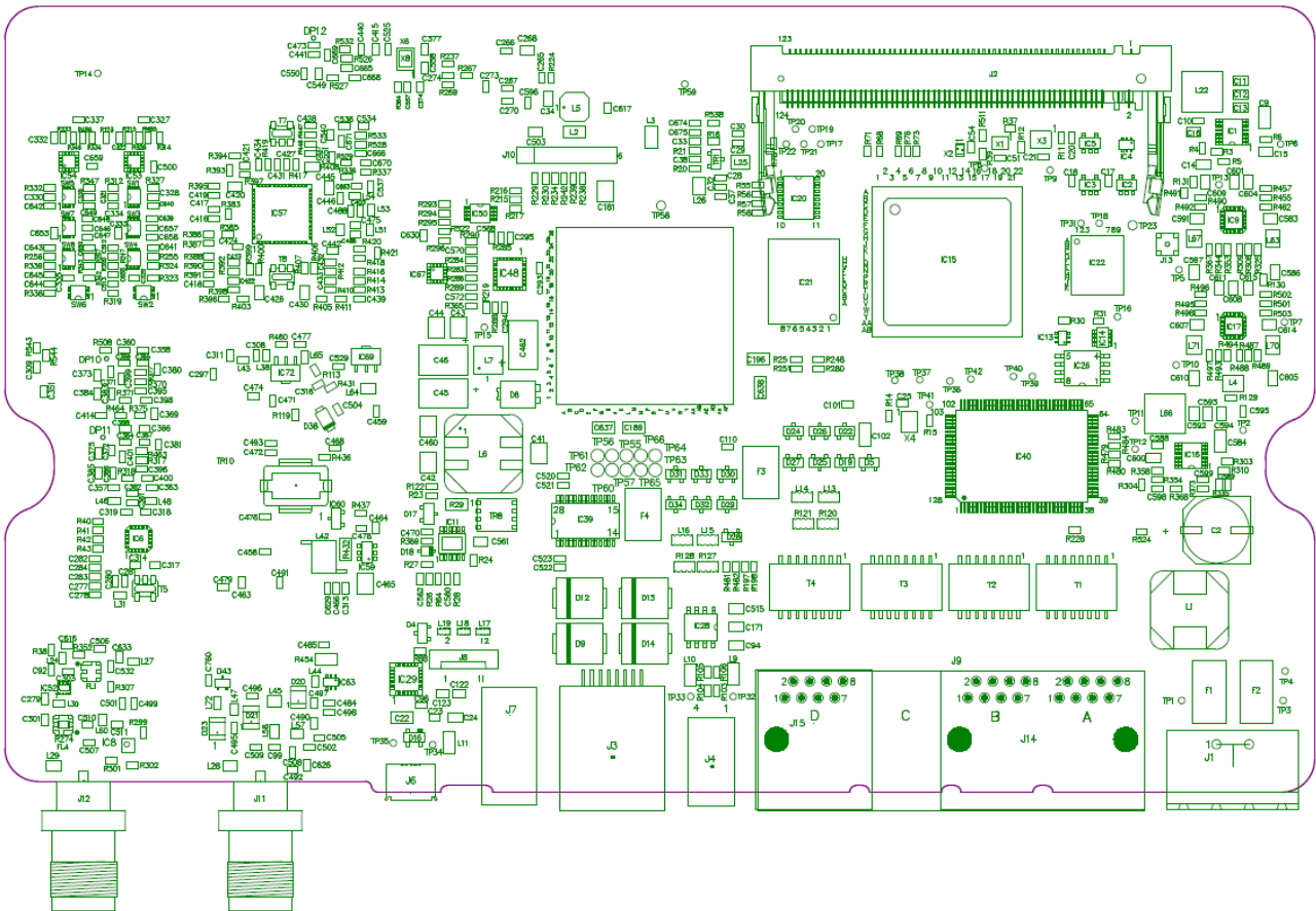
Figure 5: New PCA layout top view
