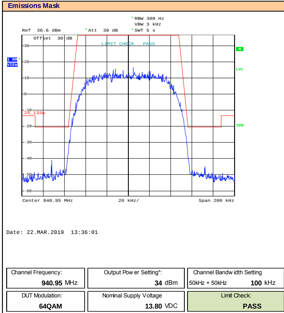
Plot 9.27 – Emissions Mask – 940.95, 100kHz BW, 64QAM
