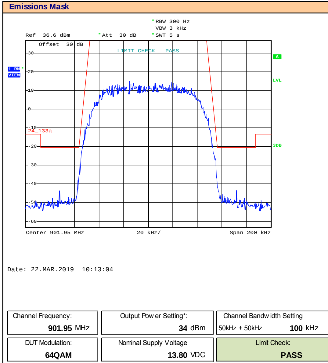
Plot 9.9 – Emissions Mask – 901.95, 100kHz BW, 64QAM
