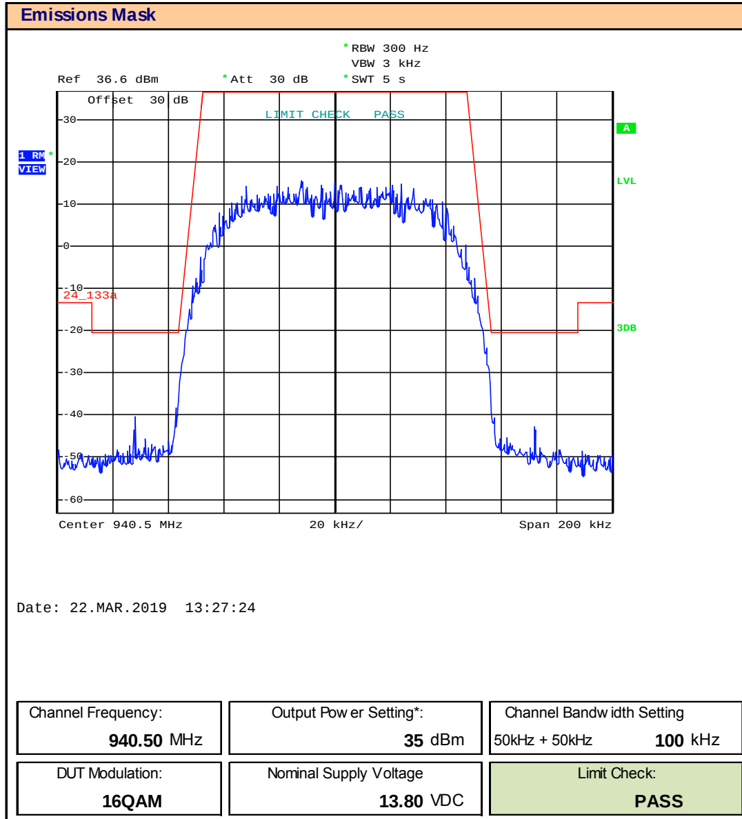
Plot 9.23 – Emissions Mask – 940.5, 100kHz BW, 16QAM
