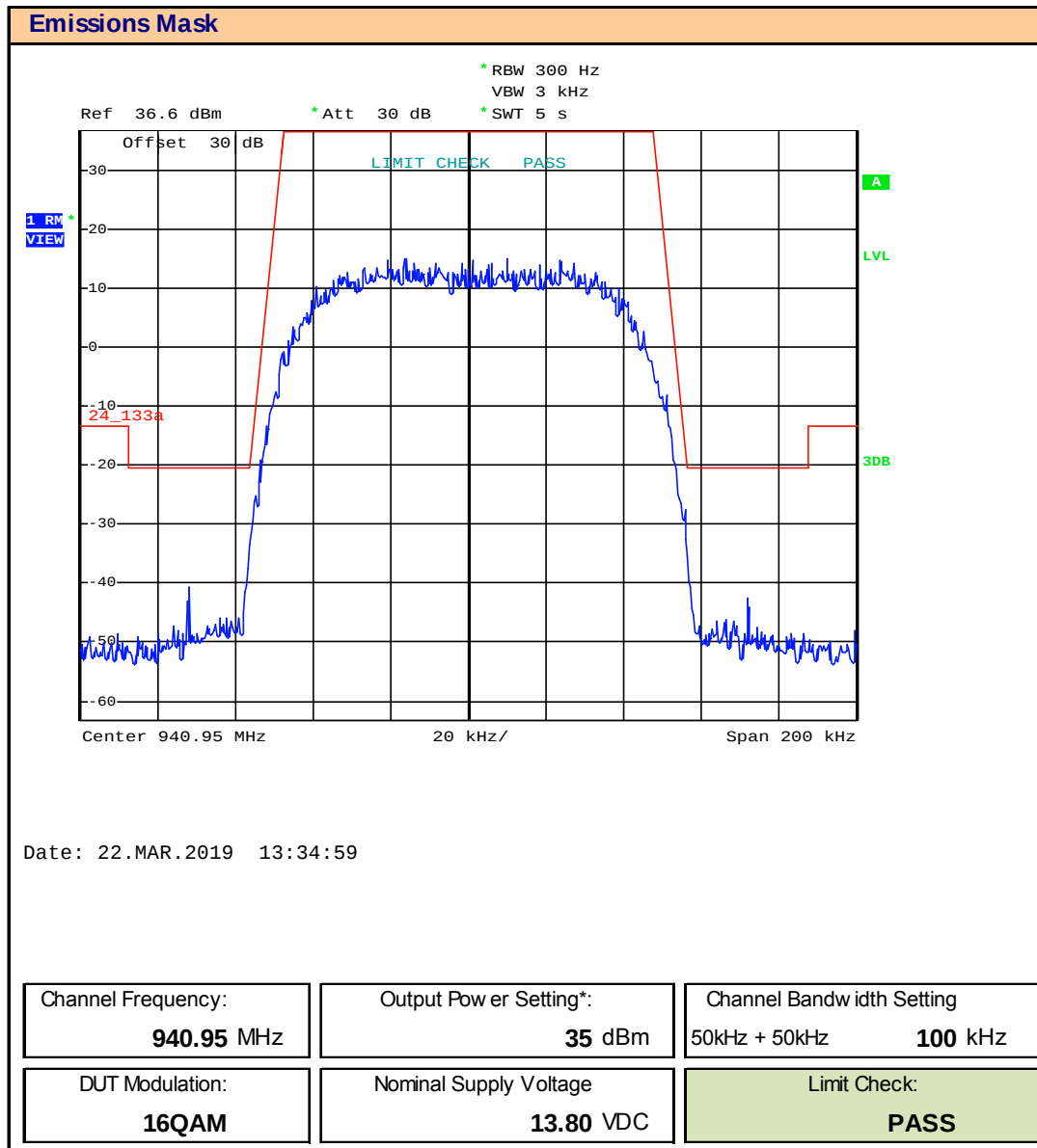
Plot 9.26 – Emissions Mask – 940.95, 100kHz BW, 16QAM
