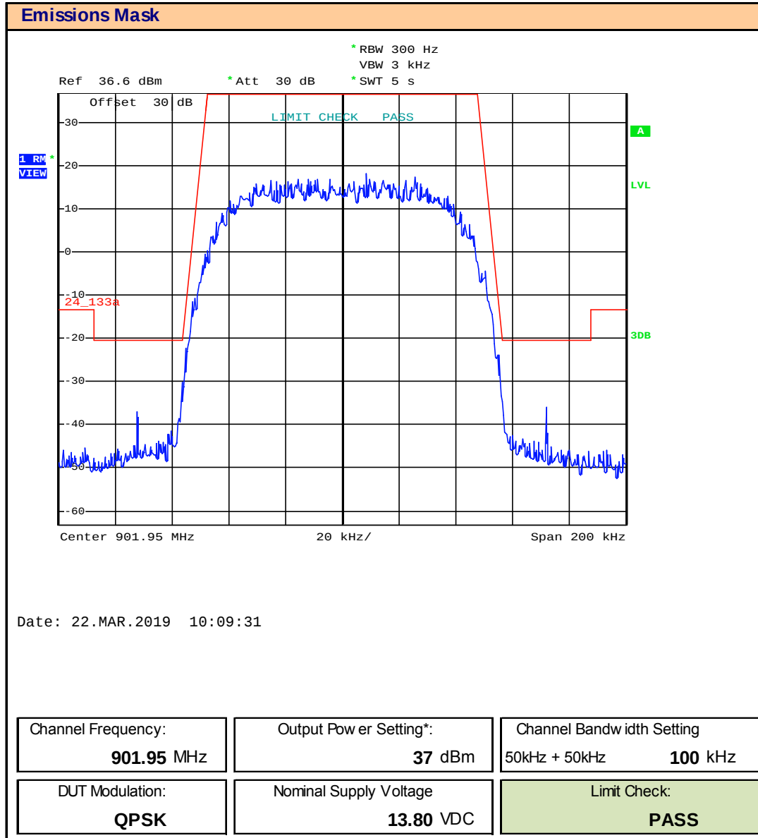
Plot 9.7 – Emissions Mask – 901.95, 100kHz BW, QPSK
