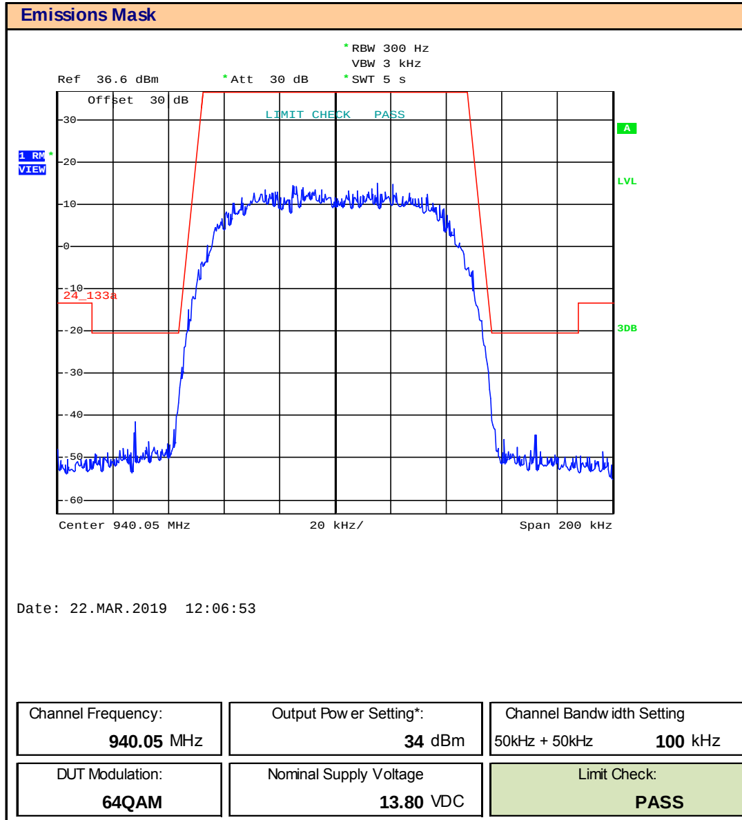
Plot 9.21 – Emissions Mask – 940.05, 100kHz BW, 64QAM
