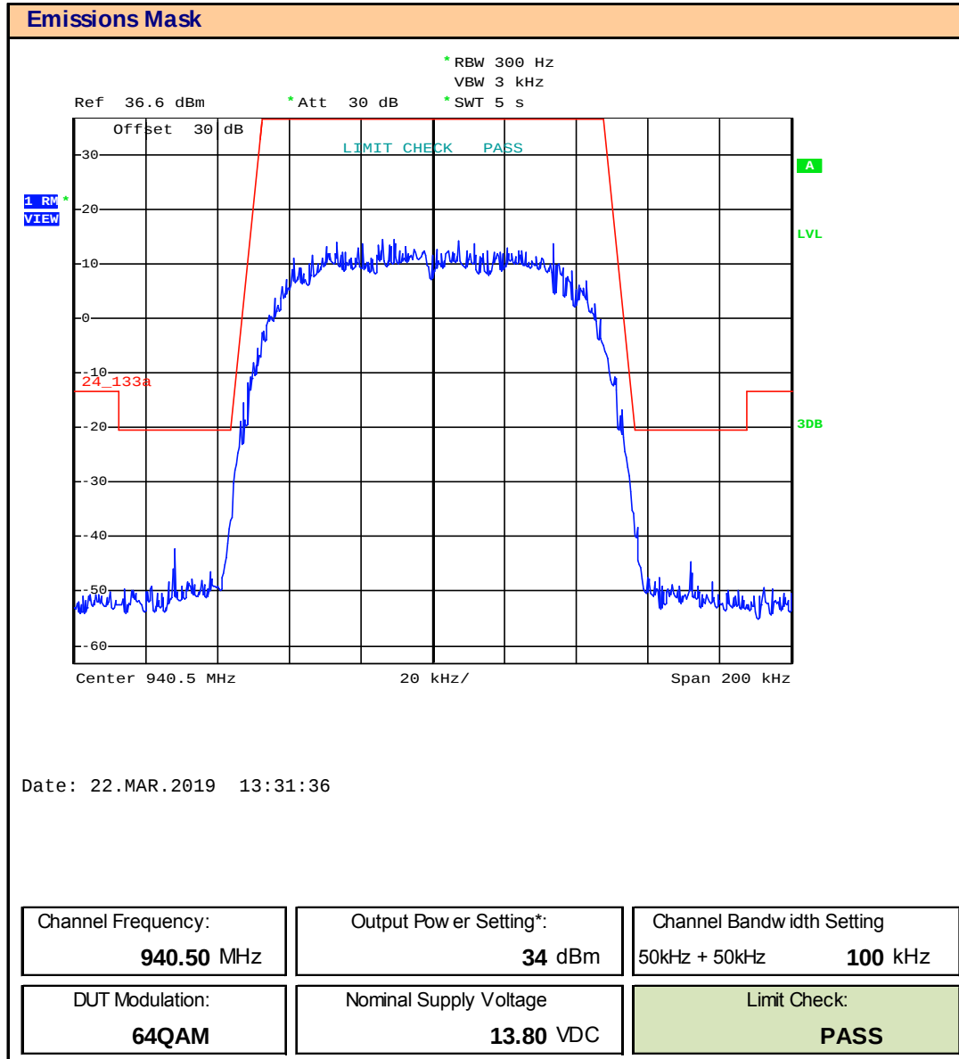
Plot 9.24 – Emissions Mask – 940.5, 100kHz BW, 64QAM
