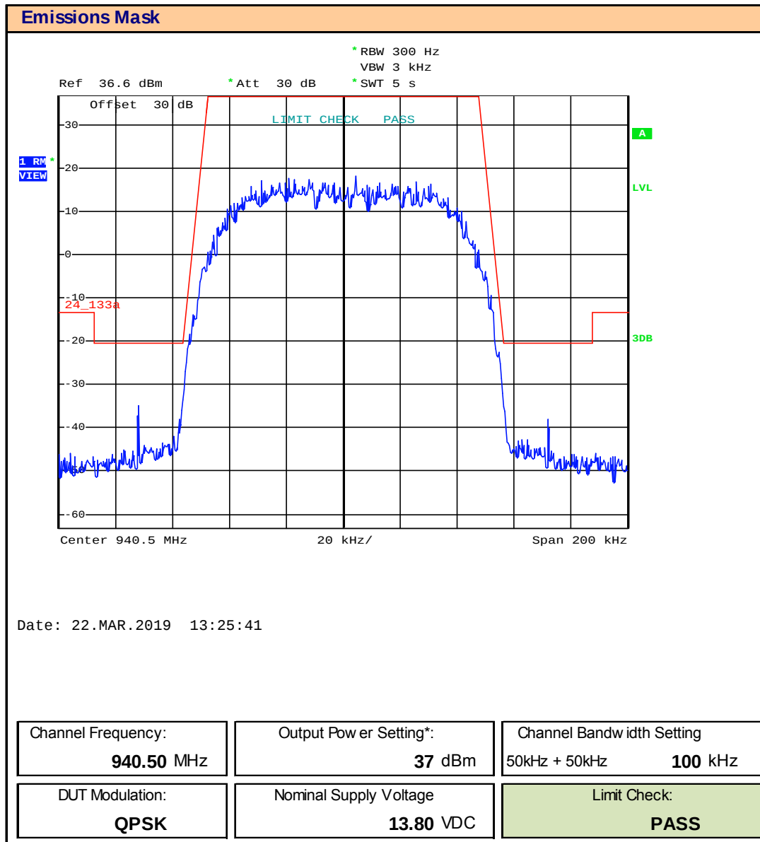
Plot 9.22 – Emissions Mask – 940.5, 100kHz BW, QPSK
