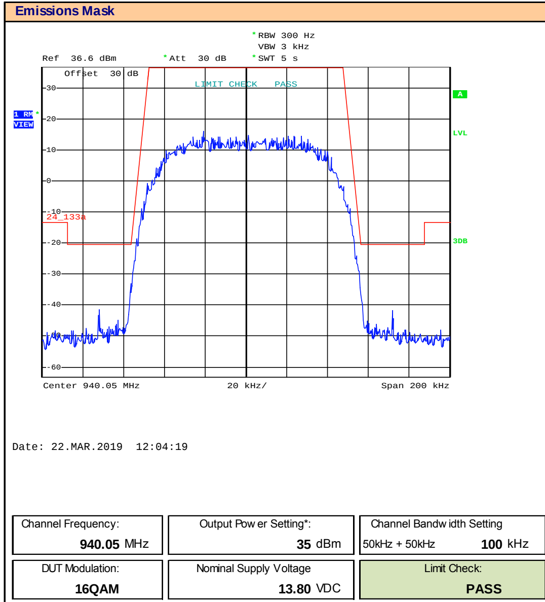
Plot 9.20 – Emissions Mask – 940.05, 100kHz BW, 16QAM
