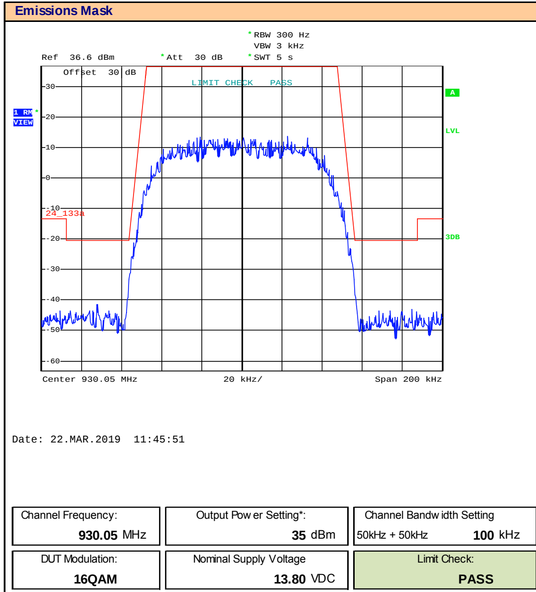
Plot 9.11 – Emissions Mask – 930.05, 100kHz BW, 16QAM
