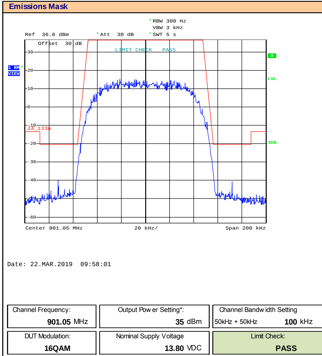
Plot 9.2 – Emissions Mask – 901.05, 100kHz BW, 16QAM
