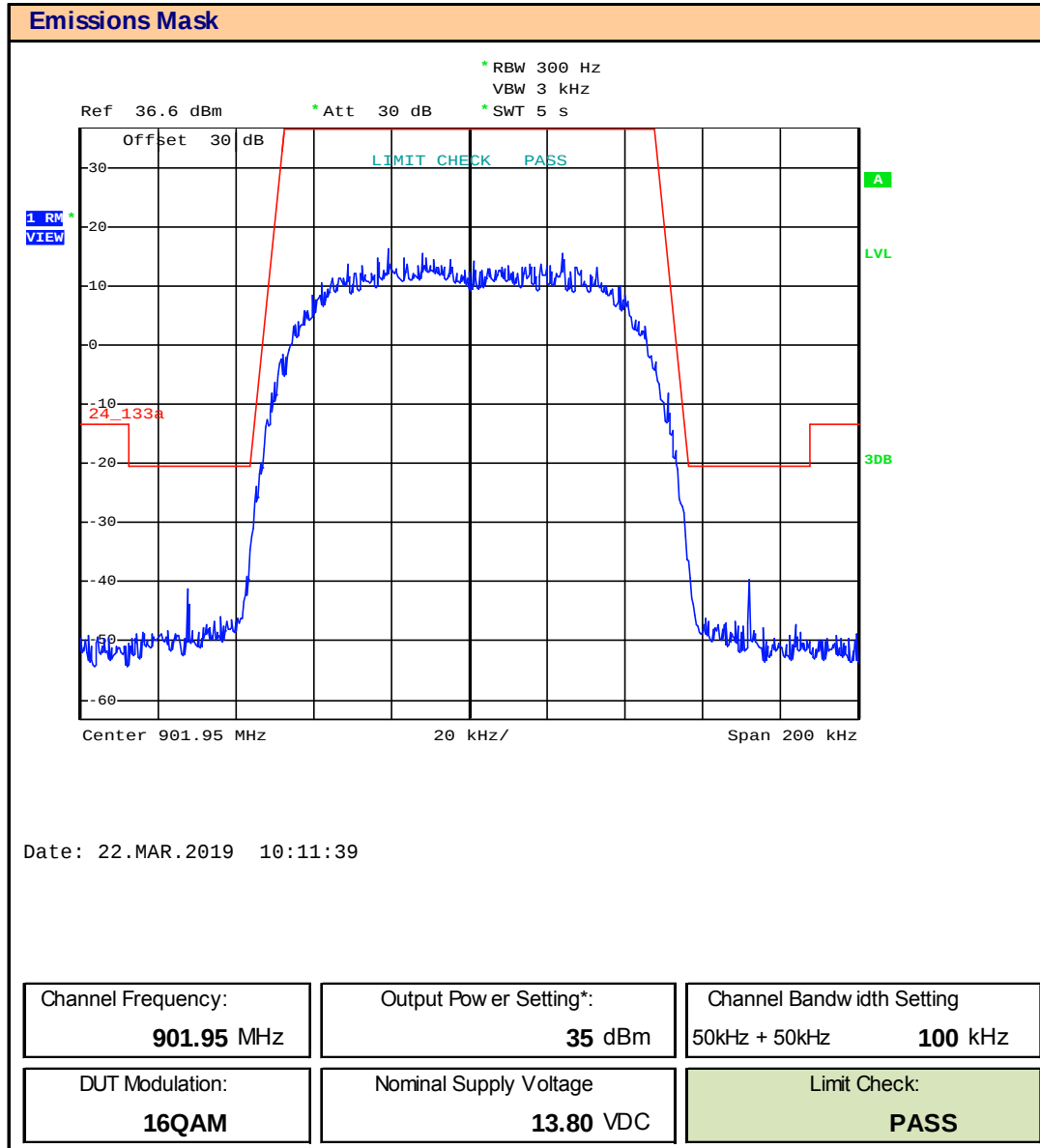
Plot 9.8 – Emissions Mask – 901.95, 100kHz BW, 16QAM
