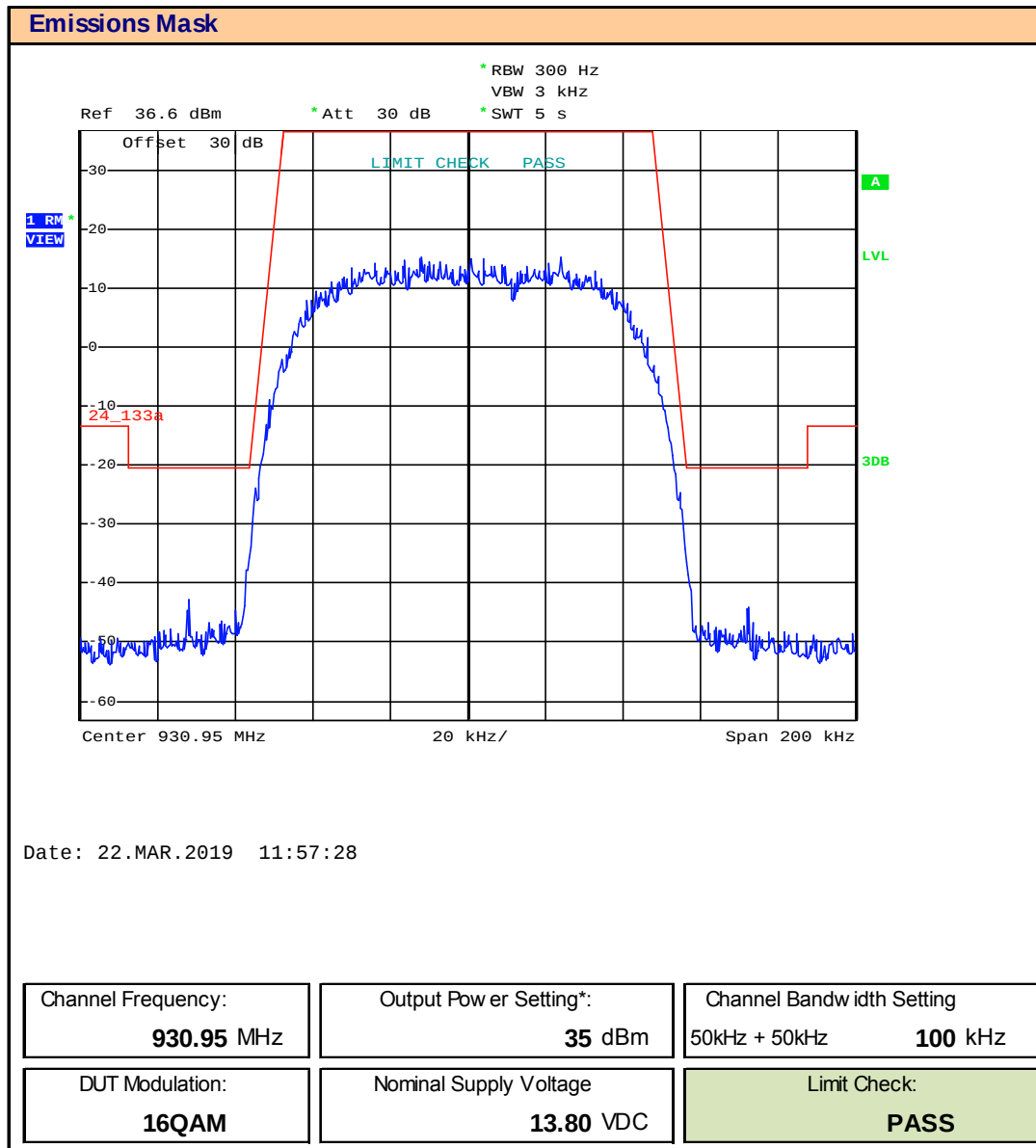
Plot 9.17 – Emissions Mask – 930.95, 100kHz BW, 16QAM
