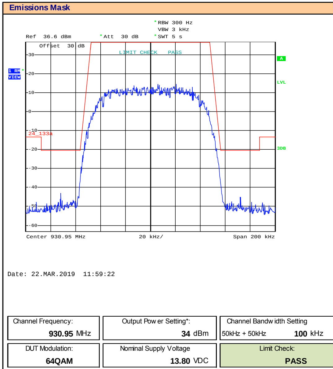
Plot 9.18 – Emissions Mask – 930.95, 100kHz BW, 64QAM
