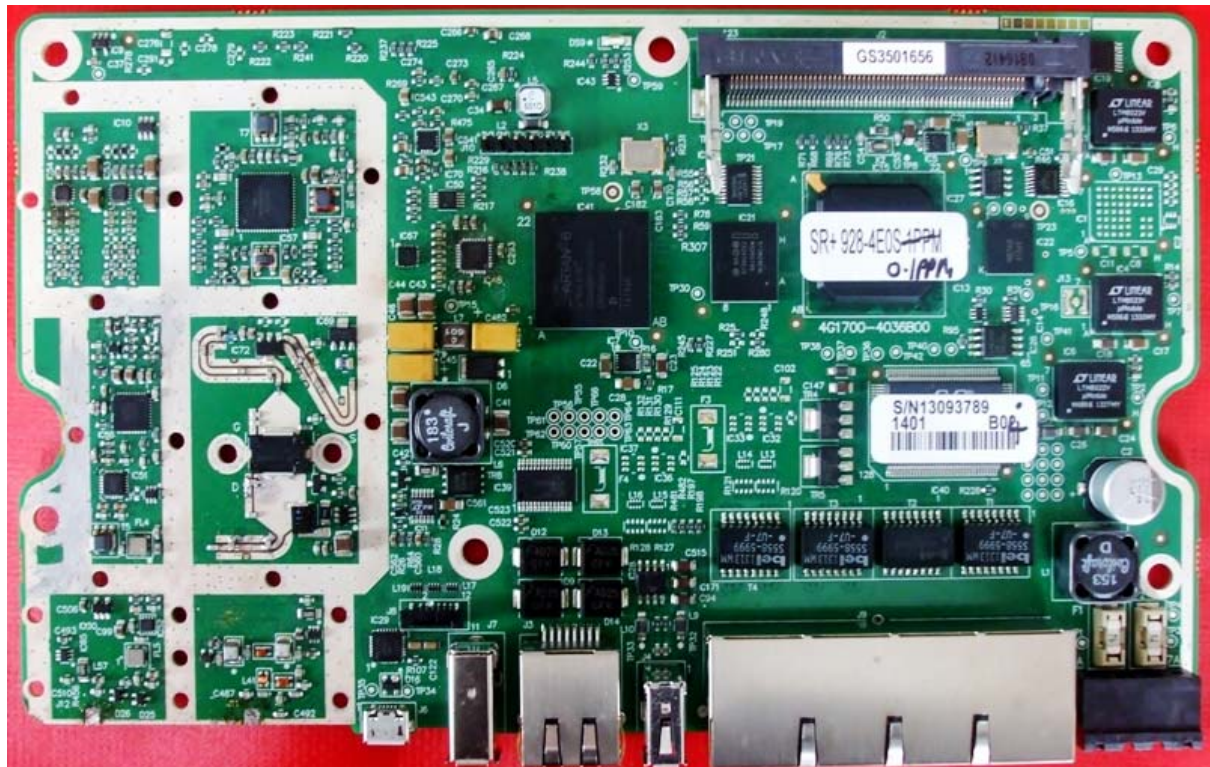
Top of board overall
