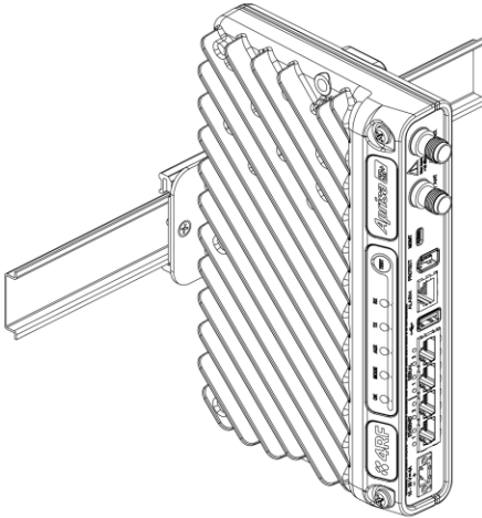
Vertical Mount
