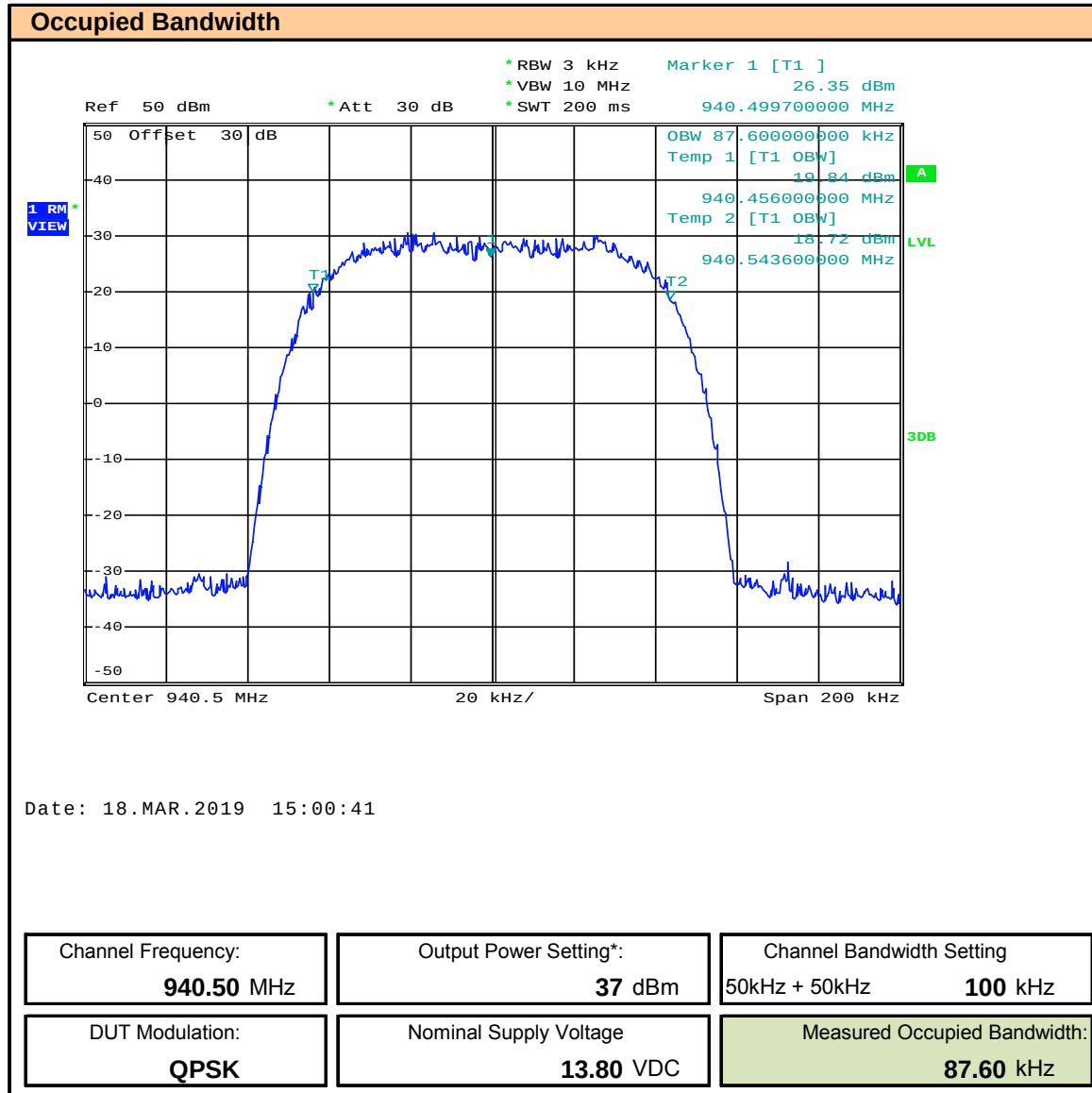
Plot 8.7 – Occupied Bandwidth – 940.5MHz, 100kHz BW, QPSK
