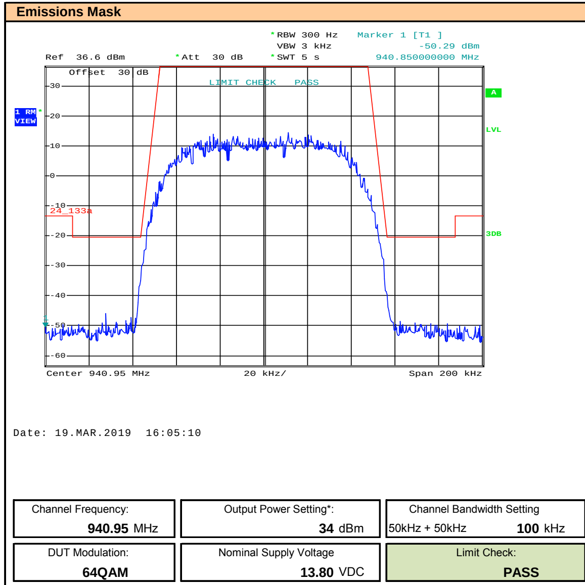
Plot 9.27 – Emissions Mask – 940.95, 100kHz BW, 64QAM
