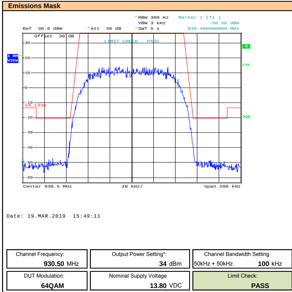
Plot 9.15 – Emissions Mask – 930.5, 100kHz BW, 64QAM
