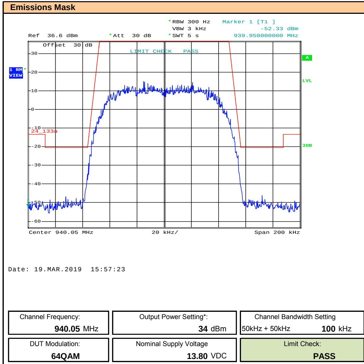
Plot 9.21 – Emissions Mask – 940.05, 100kHz BW, 64QAM
