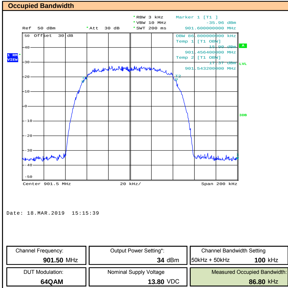
Plot 8.3 – Occupied Bandwidth – 901.5MHz, 100kHz BW, 64QAM
