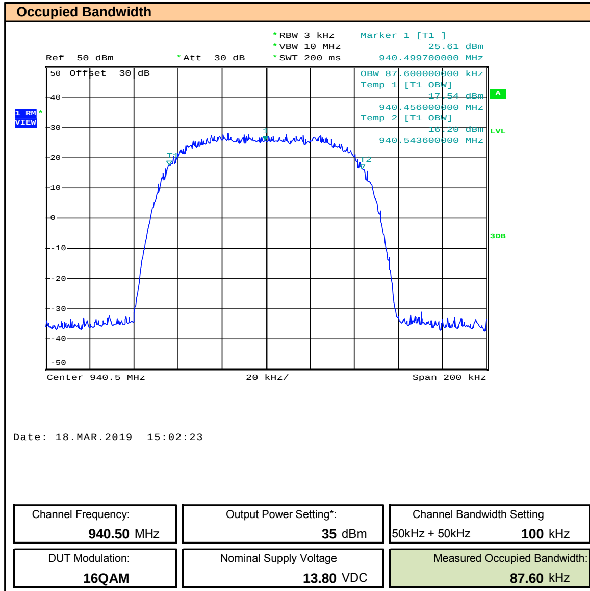
Plot 8.8 – Occupied Bandwidth – 940.5MHz, 100kHz BW, 16QAM
