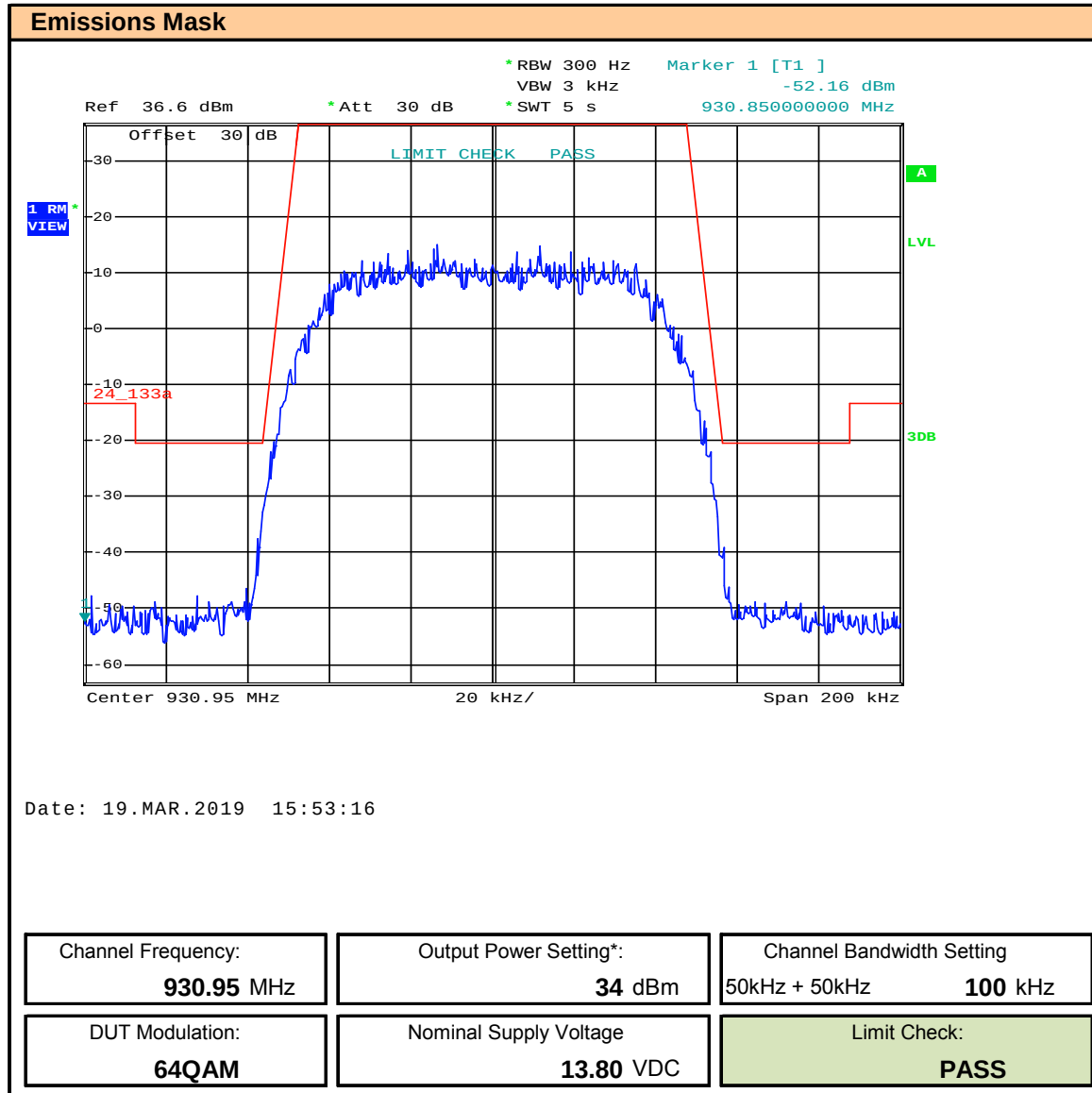
Plot 9.18 – Emissions Mask – 930.95, 100kHz BW, 64QAM
