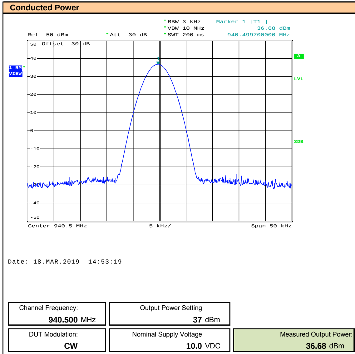
Plot 7.7 – Conducted Power – 940.5MHz, 10VDC
