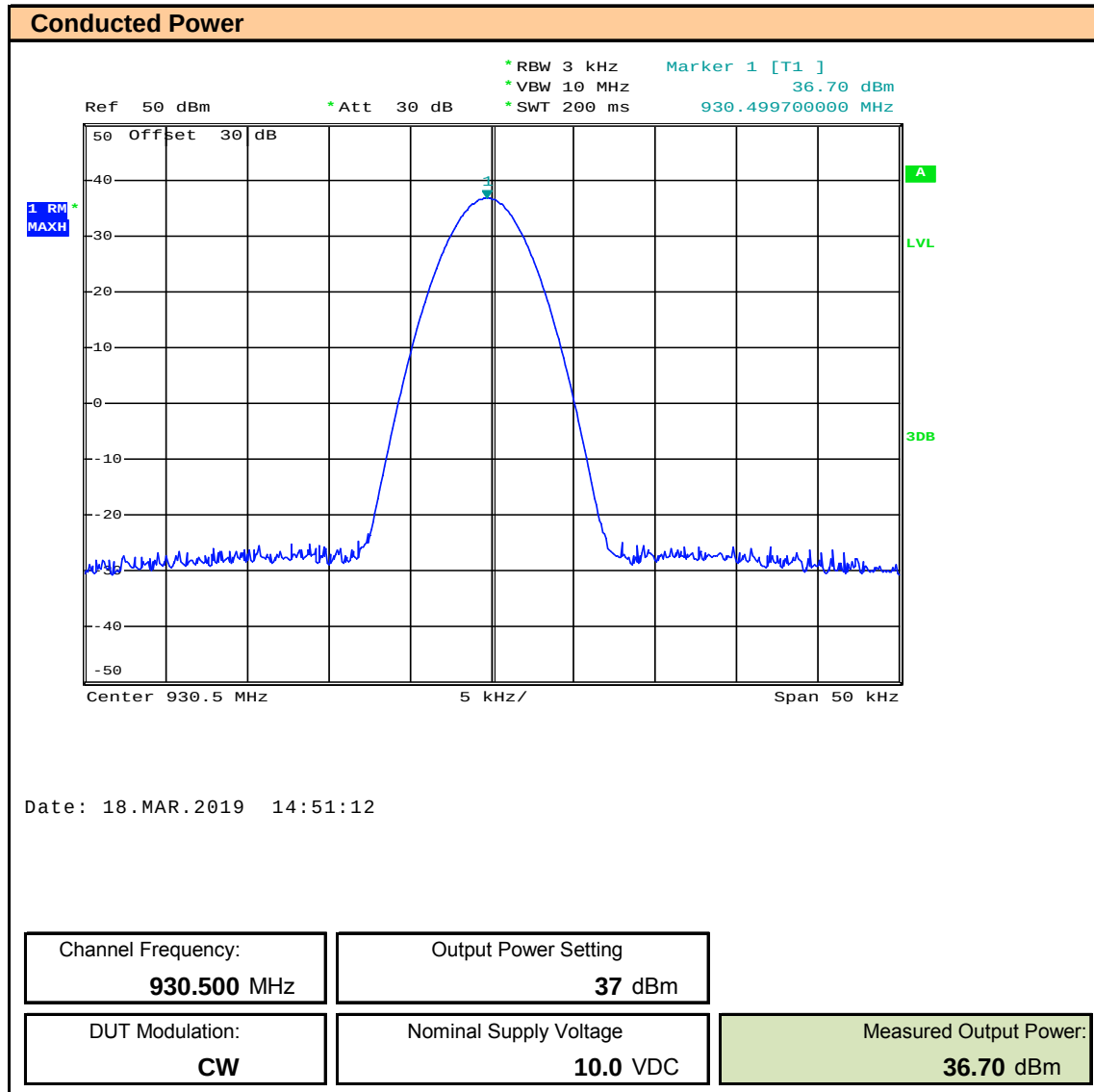
Plot 7.4 – Conducted Power – 930.5MHz, 10VDC
