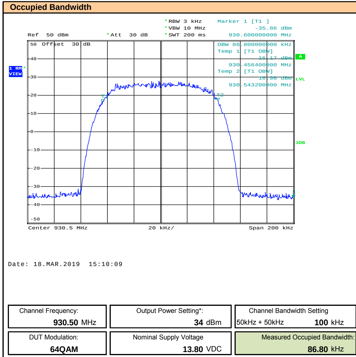
Plot 8.6 – Occupied Bandwidth – 930.5MHz, 100kHz BW, 64QAM
