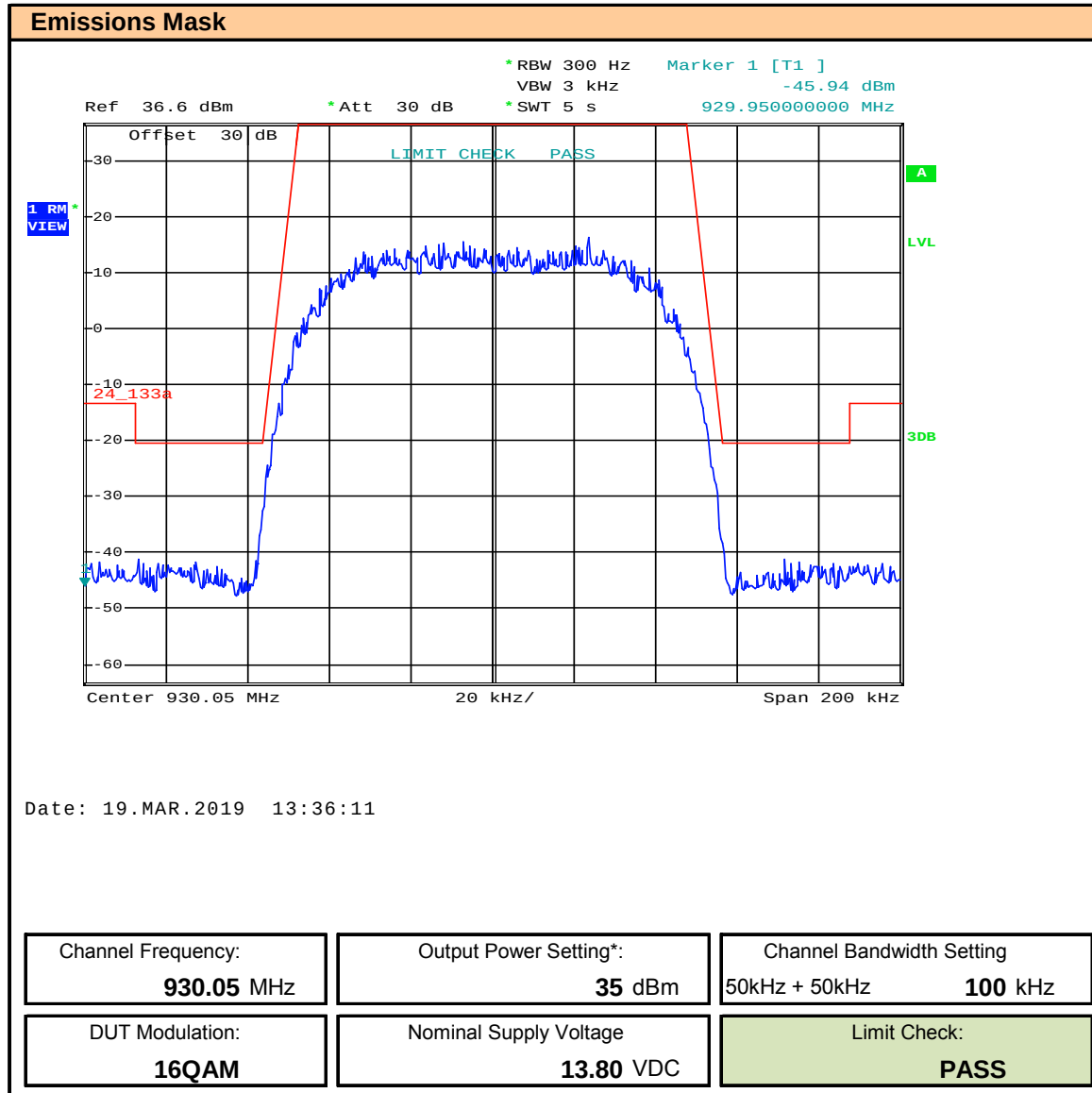
Plot 9.11 – Emissions Mask – 930.05, 100kHz BW, 16QAM
