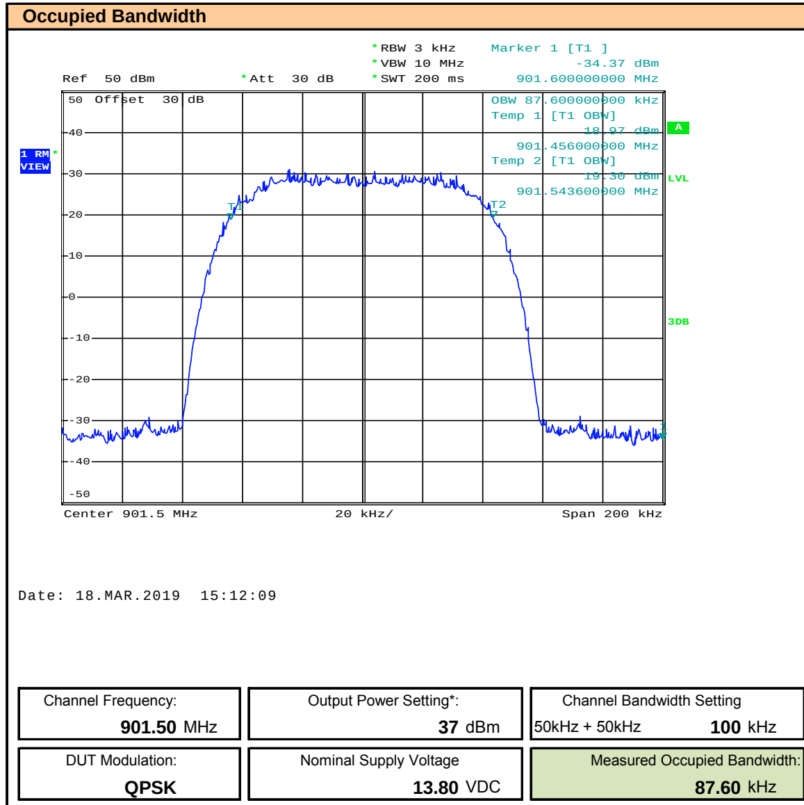
Plot 8.1 – Occupied Bandwidth – 901.5MHz, 100kHz BW, QPSK
