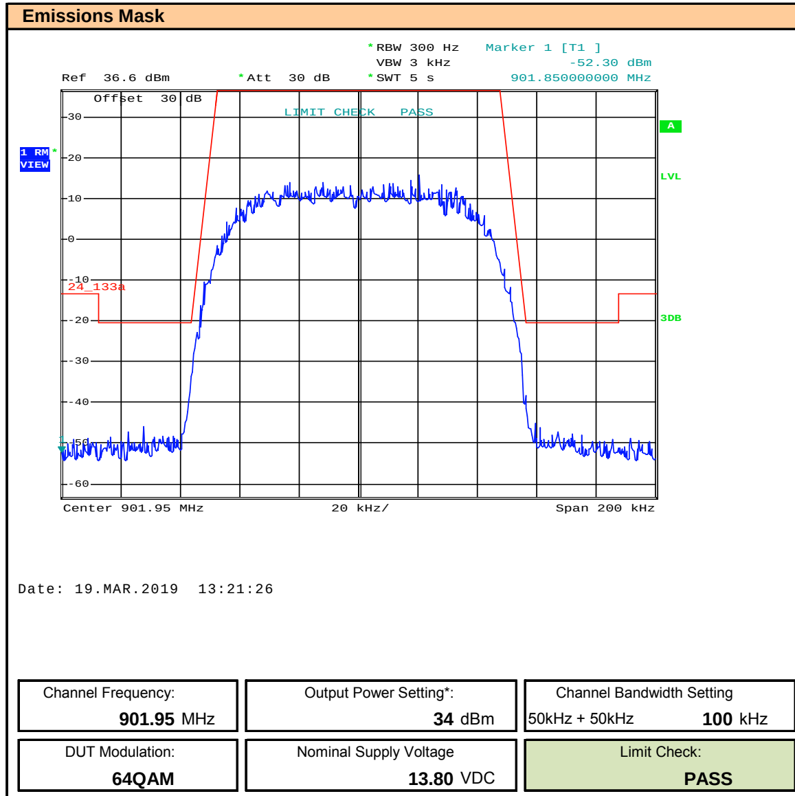
Plot 9.9 – Emissions Mask – 901.95, 100kHz BW, 64QAM
