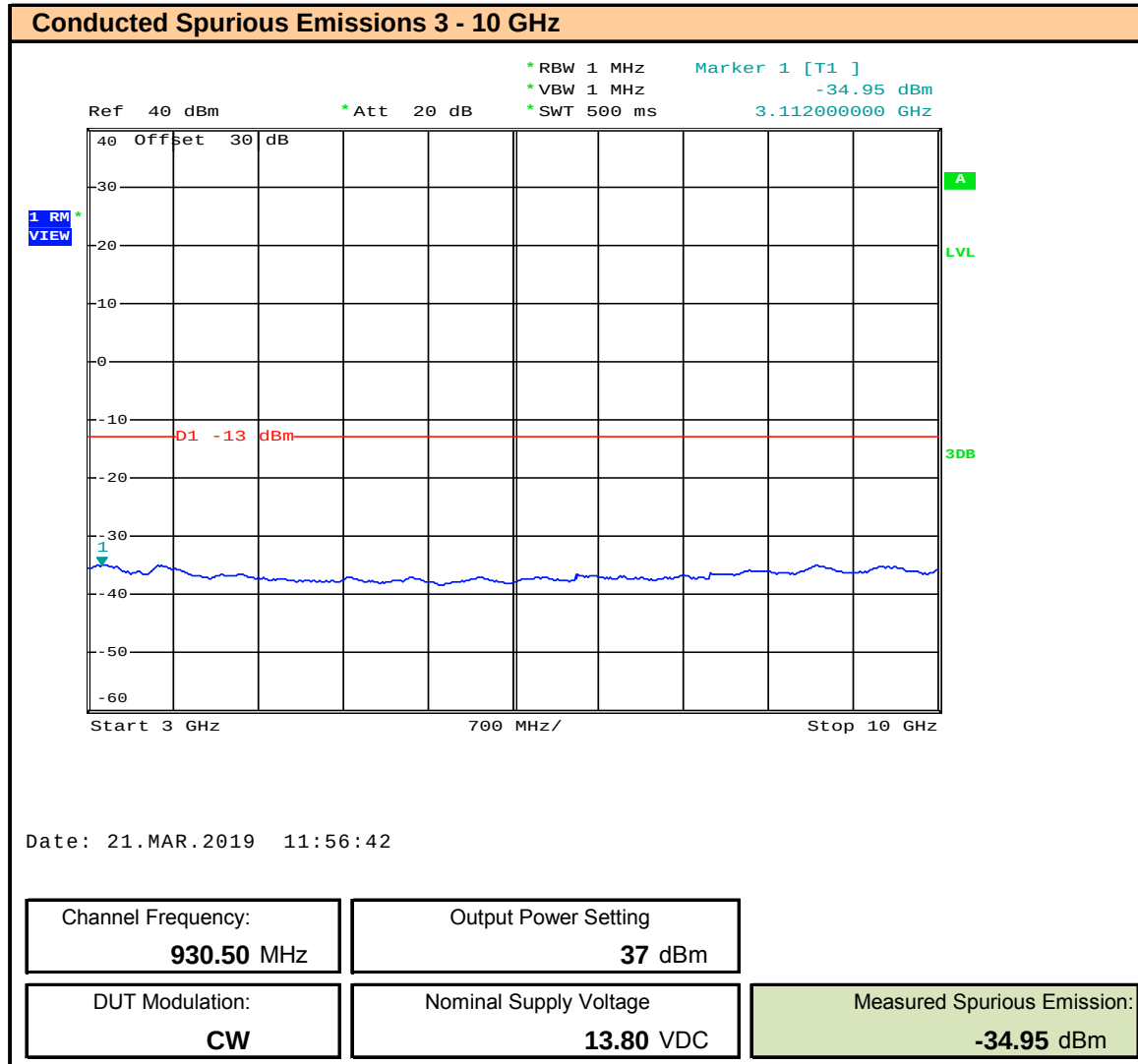
Plot 10.6 – Conducted Spurious Emissions 930.5MHz Channel, 3 – 10GHz
