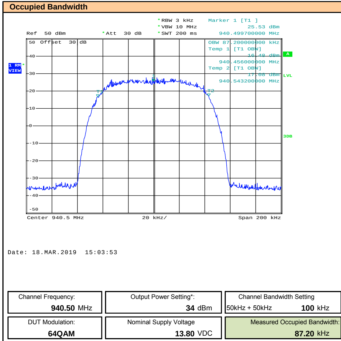
Plot 8.9 – Occupied Bandwidth – 940.5MHz, 100kHz BW, 64QAM
