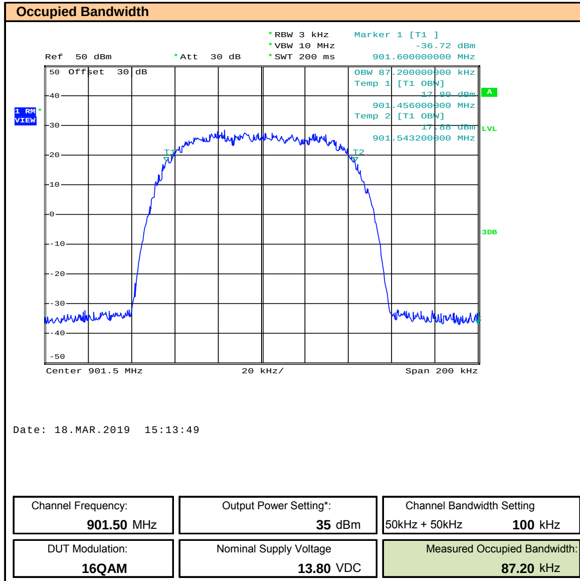
Plot 8.2 – Occupied Bandwidth – 901.5MHz, 100kHz BW, 16QAM
