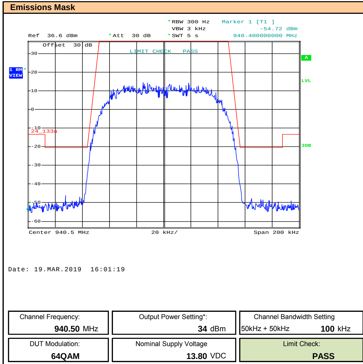
Plot 9.24 – Emissions Mask – 940.5, 100kHz BW, 64QAM
