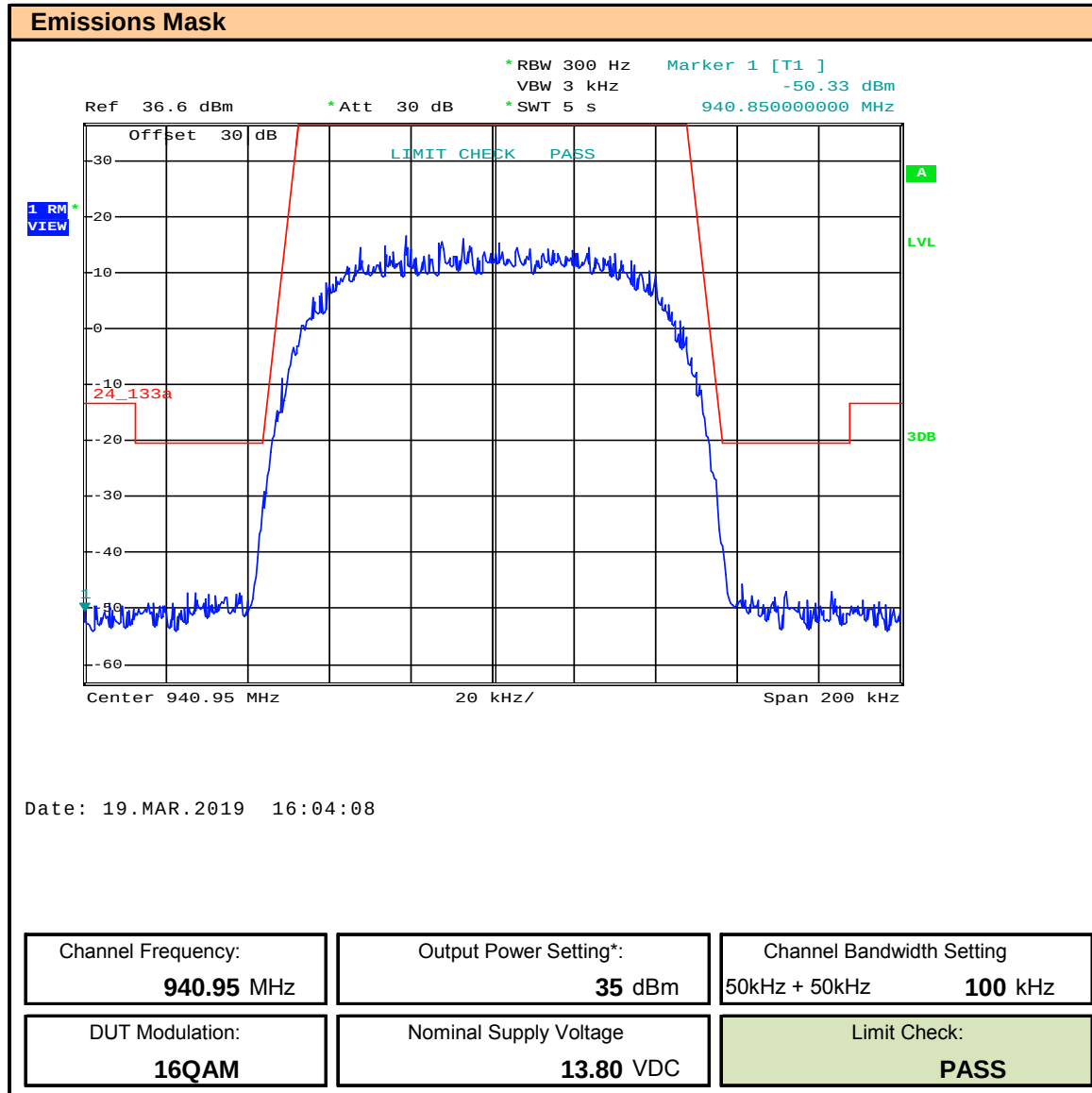
Plot 9.26 – Emissions Mask – 940.95, 100kHz BW, 16QAM
