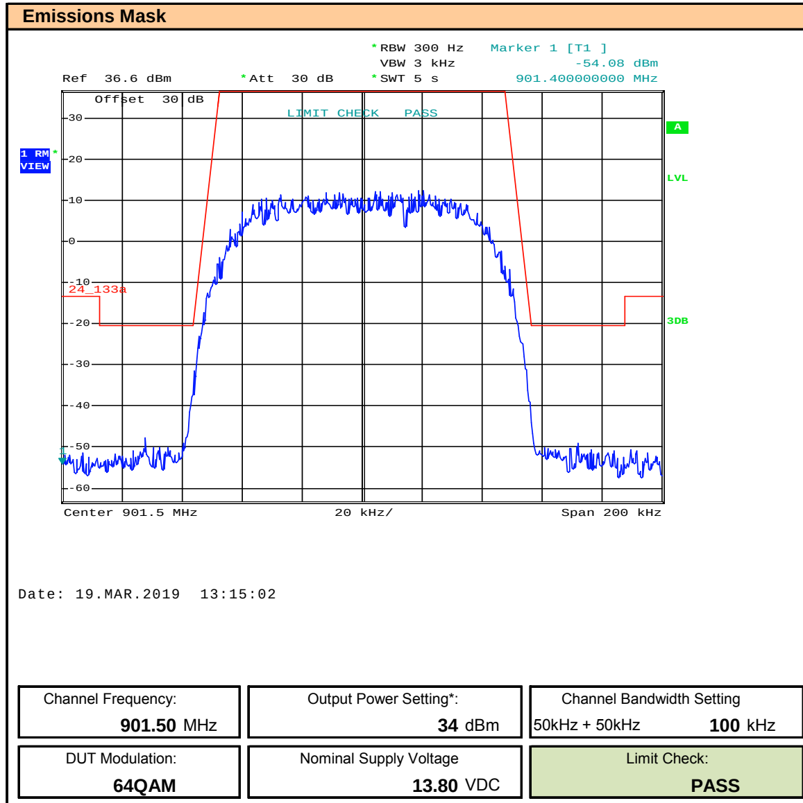
Plot 9.6 – Emissions Mask – 901.5, 100kHz BW, 64QAM
