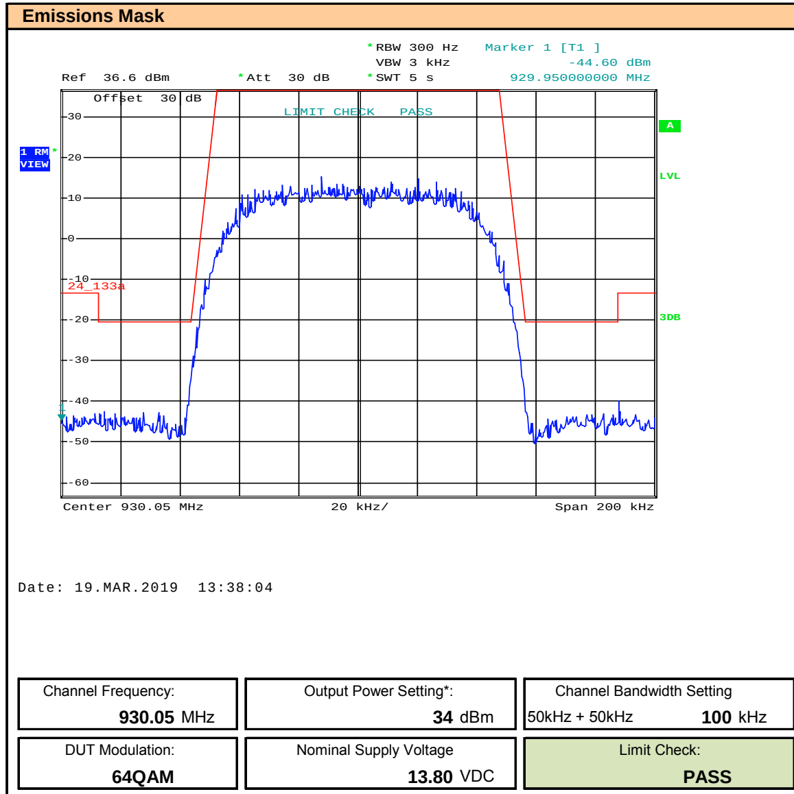
Plot 9.12 – Emissions Mask – 930.05, 100kHz BW, 64QAM
