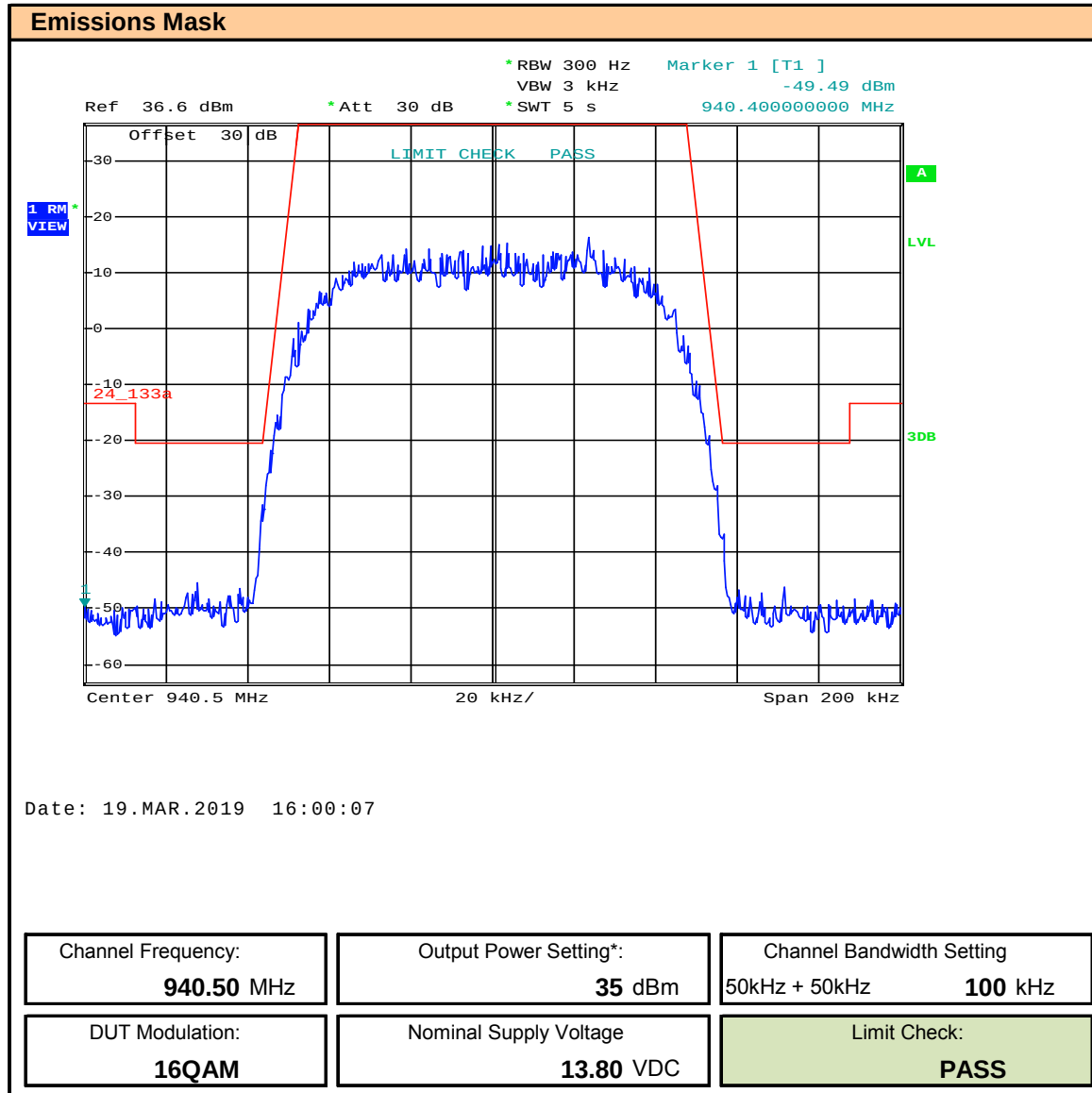
Plot 9.23 – Emissions Mask – 940.5, 100kHz BW, 16QAM
