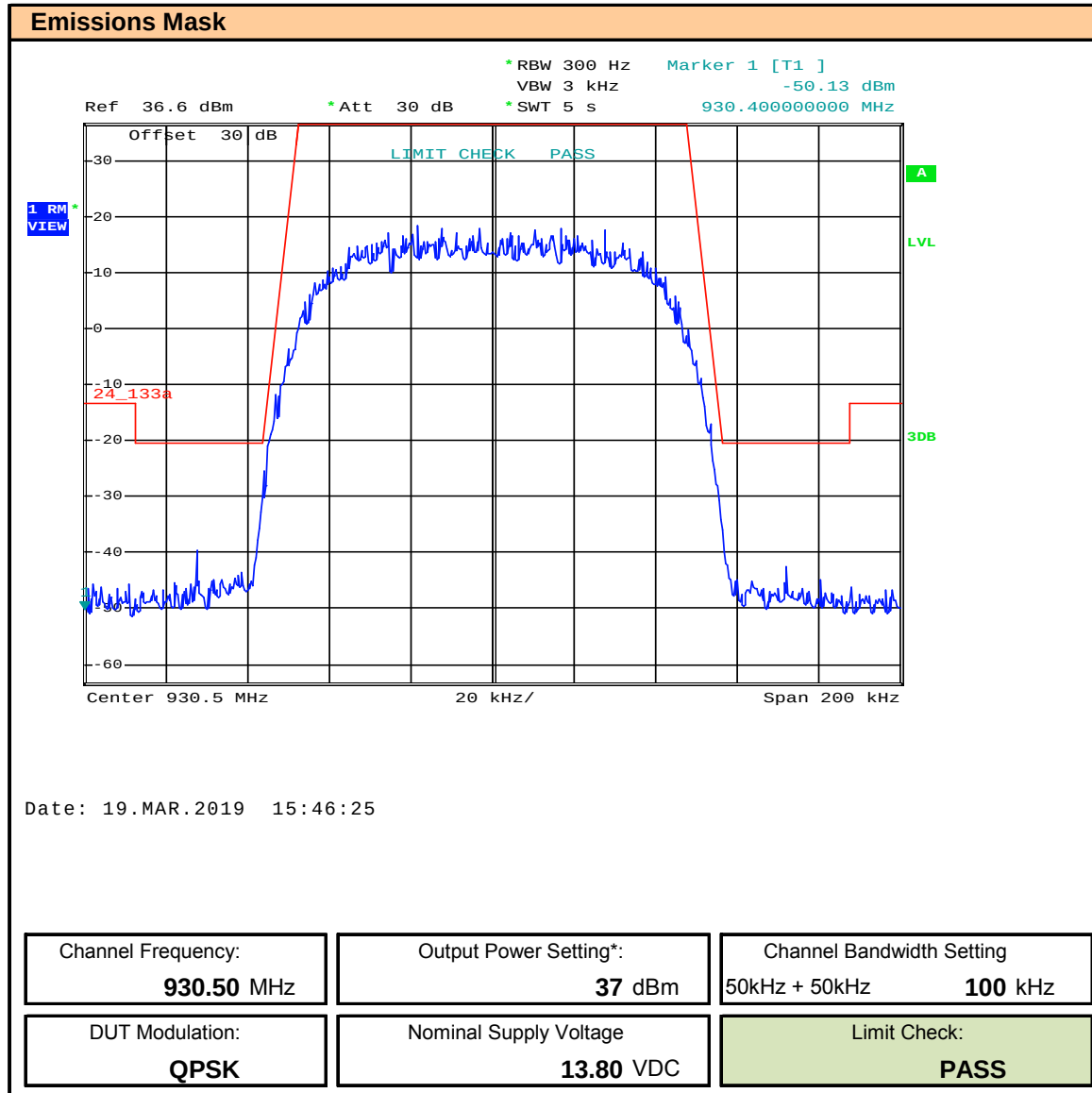
Plot 9.13 – Emissions Mask – 930.5, 100kHz BW, QPSK
