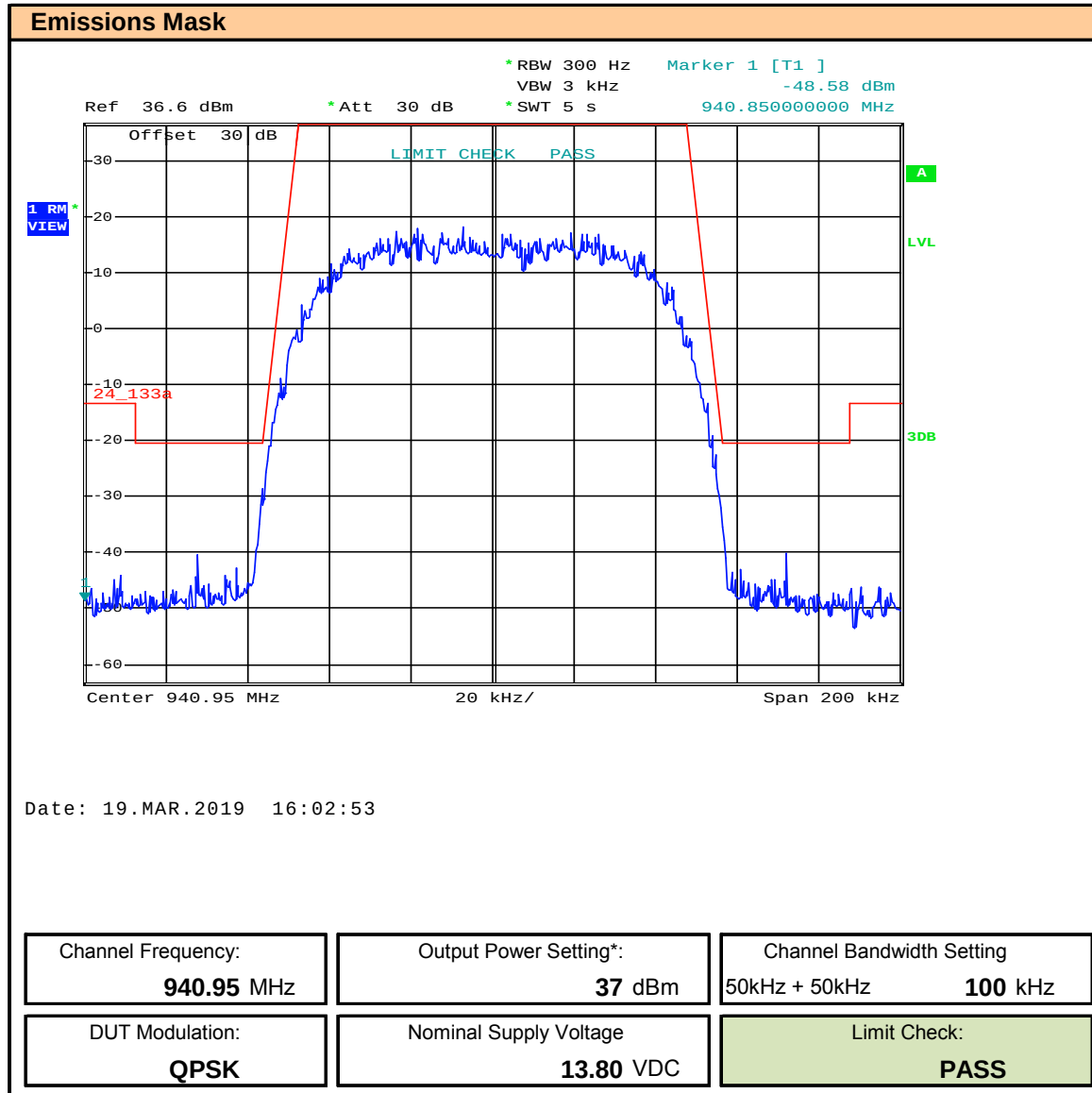
Plot 9.25 – Emissions Mask – 940.95, 100kHz BW, QPSK
