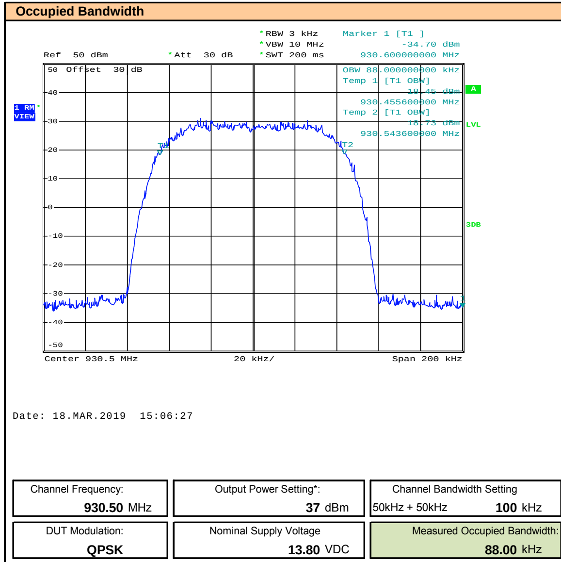
Plot 8.4 – Occupied Bandwidth – 930.5MHz, 100kHz BW, QPSK
