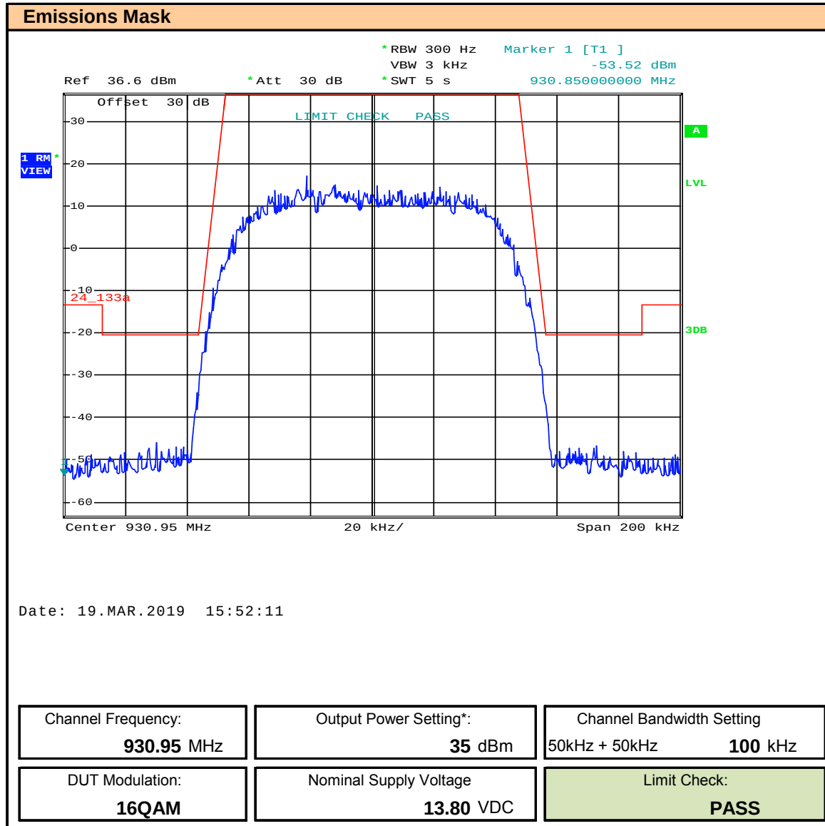
Plot 9.17 – Emissions Mask – 930.95, 100kHz BW, 16QAM
