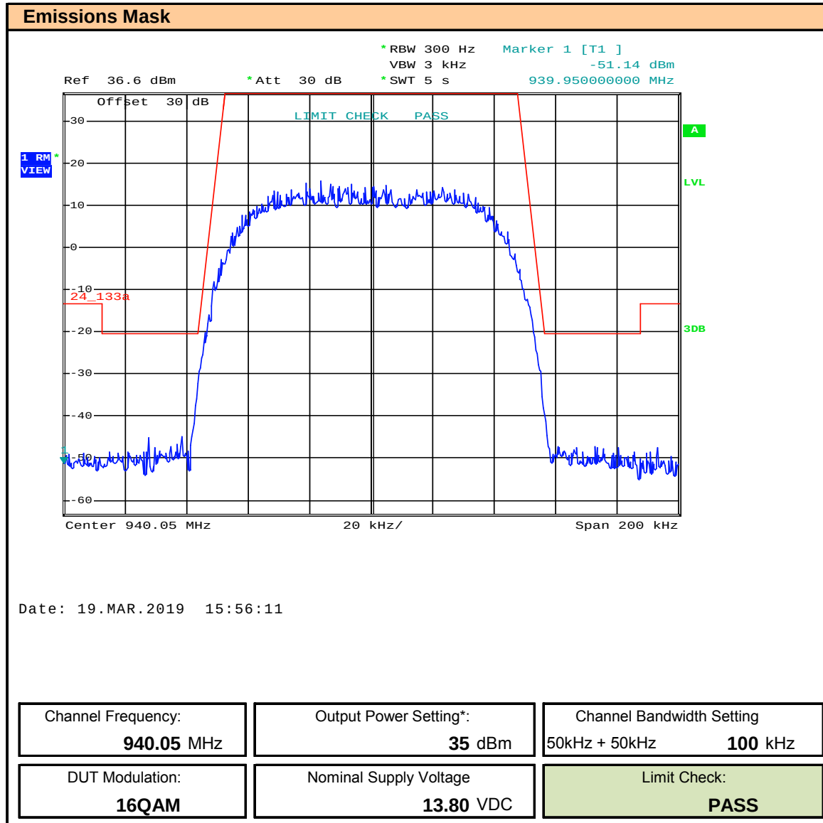
Plot 9.20 – Emissions Mask – 940.05, 100kHz BW, 16QAM
