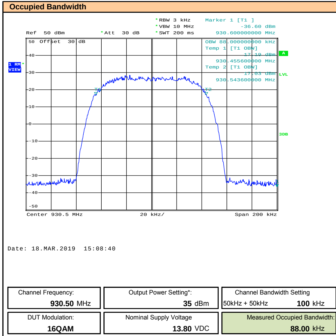
Plot 8.5 – Occupied Bandwidth – 930.5MHz, 100kHz BW, 16QAM
