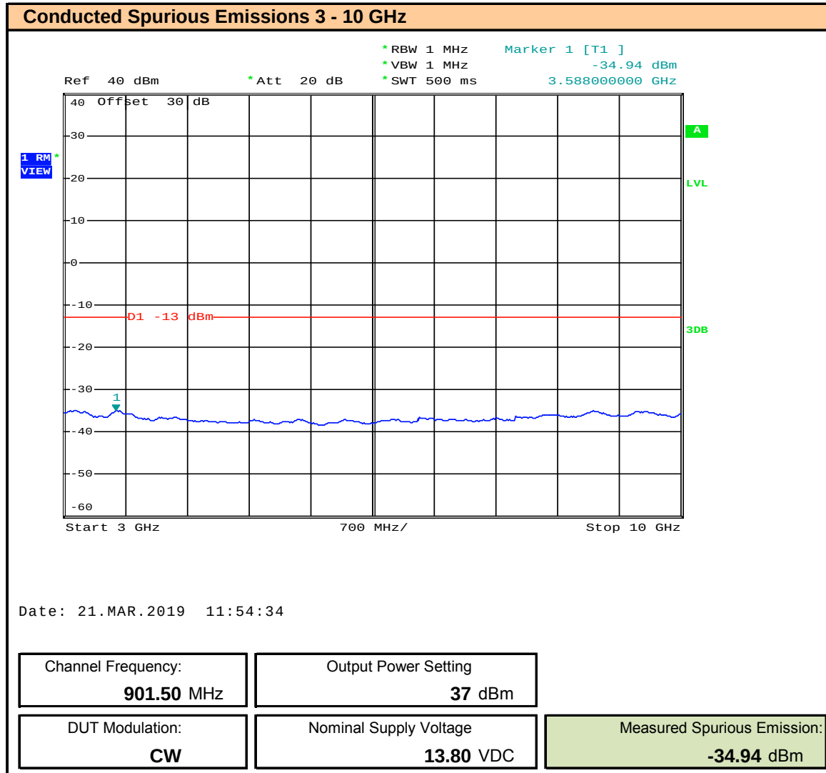
Plot 10.2 – Conducted Spurious Emissions 901.5MHz Channel, 3 – 10GHz
