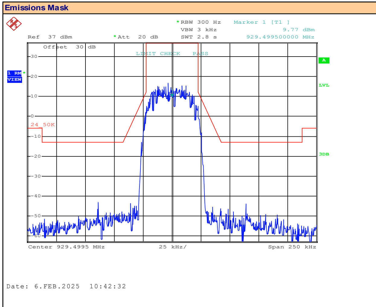
Plot 9.11 – Emissions Mask – 929.5, 50kHz BW, 64QAM
