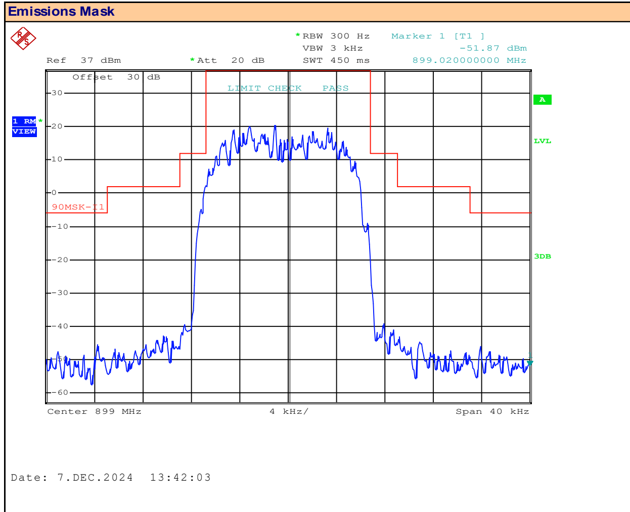
Plot 9.1 – Emissions Mask – 899MHz, 12.5kHz BW, QPSK
