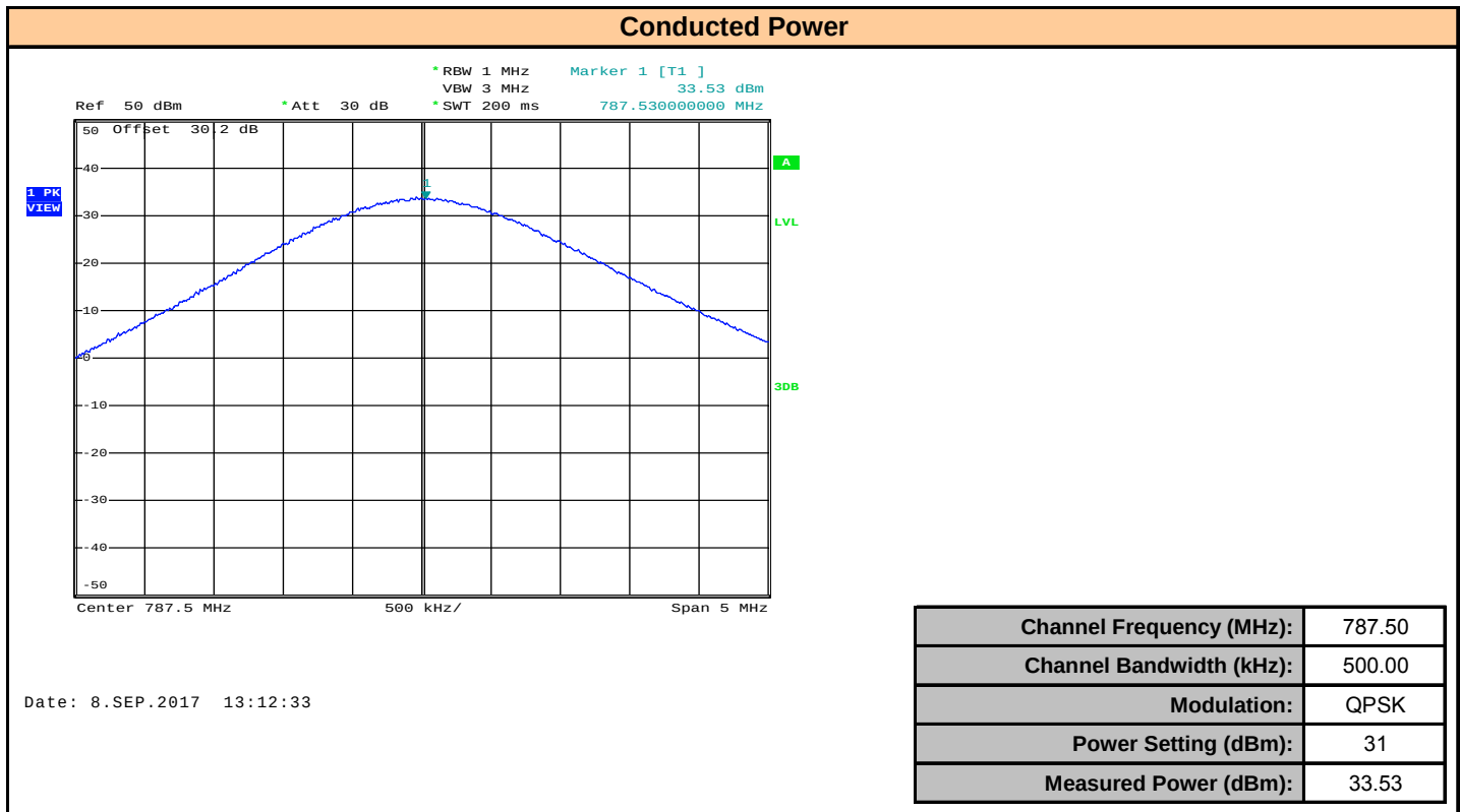
Plot 7.27 – Conducted Power 787.5MHz, 500kHz BW, QPSK
