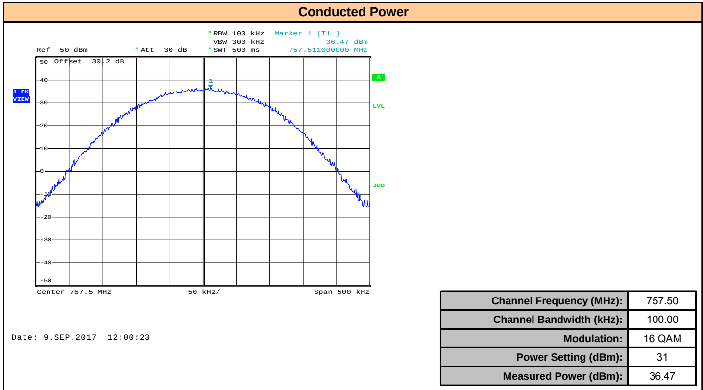
Plot 7.3 – Conducted Power 757.5MHz, 100kHz BW, 16 QAM
