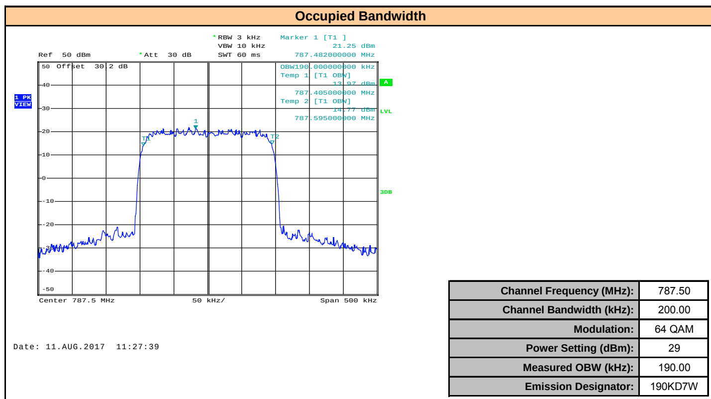
Plot 8.16 – Occupied Bandwidth 787.5MHz, 200kHz BW, 64 QAM
