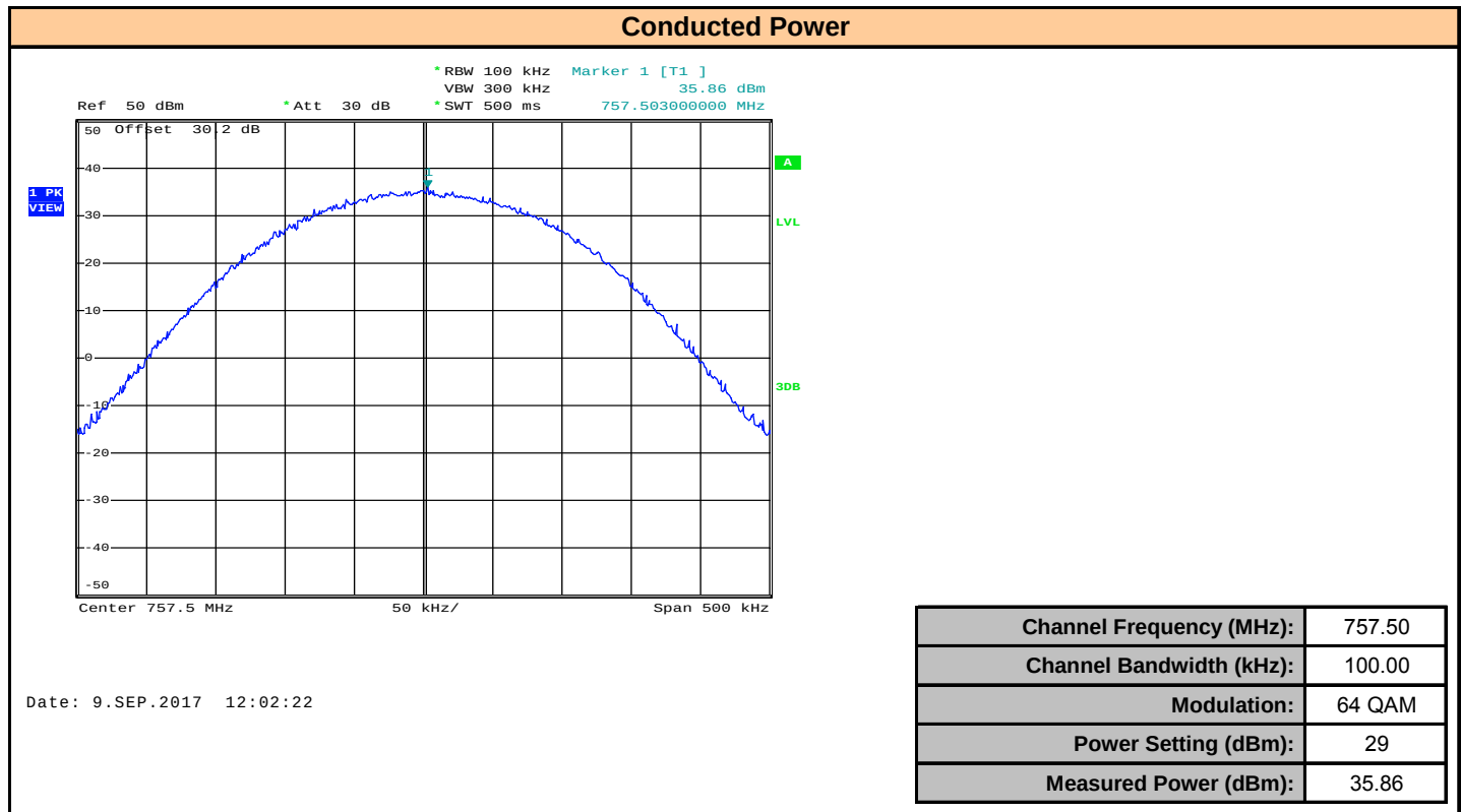
Plot 7.5 – Conducted Power 757.5MHz, 100kHz BW, 64 QAM
