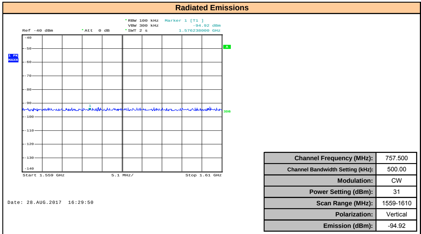
Plot 13.1 – Emission in the 1559 – 1610 MHz Band - Vertical
