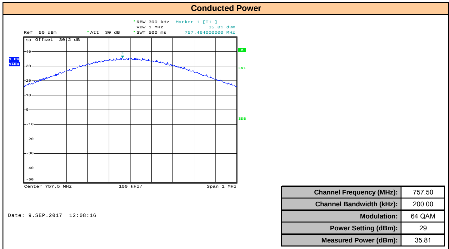
Plot 7.15 – Conducted Power 757.5MHz, 200kHz BW, 64 QAM
