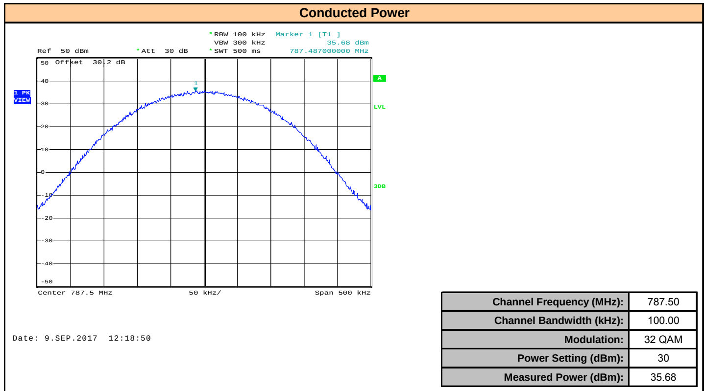
Plot 7.9 – Conducted Power 787.5MHz, 100kHz BW, 32 QAM
