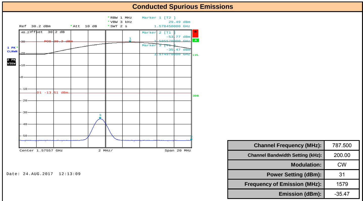
Plot 11.15 – Conducted Spurious Emission, 787.5MHz, 200kHz BW, CW, 2 nd Harmonic
