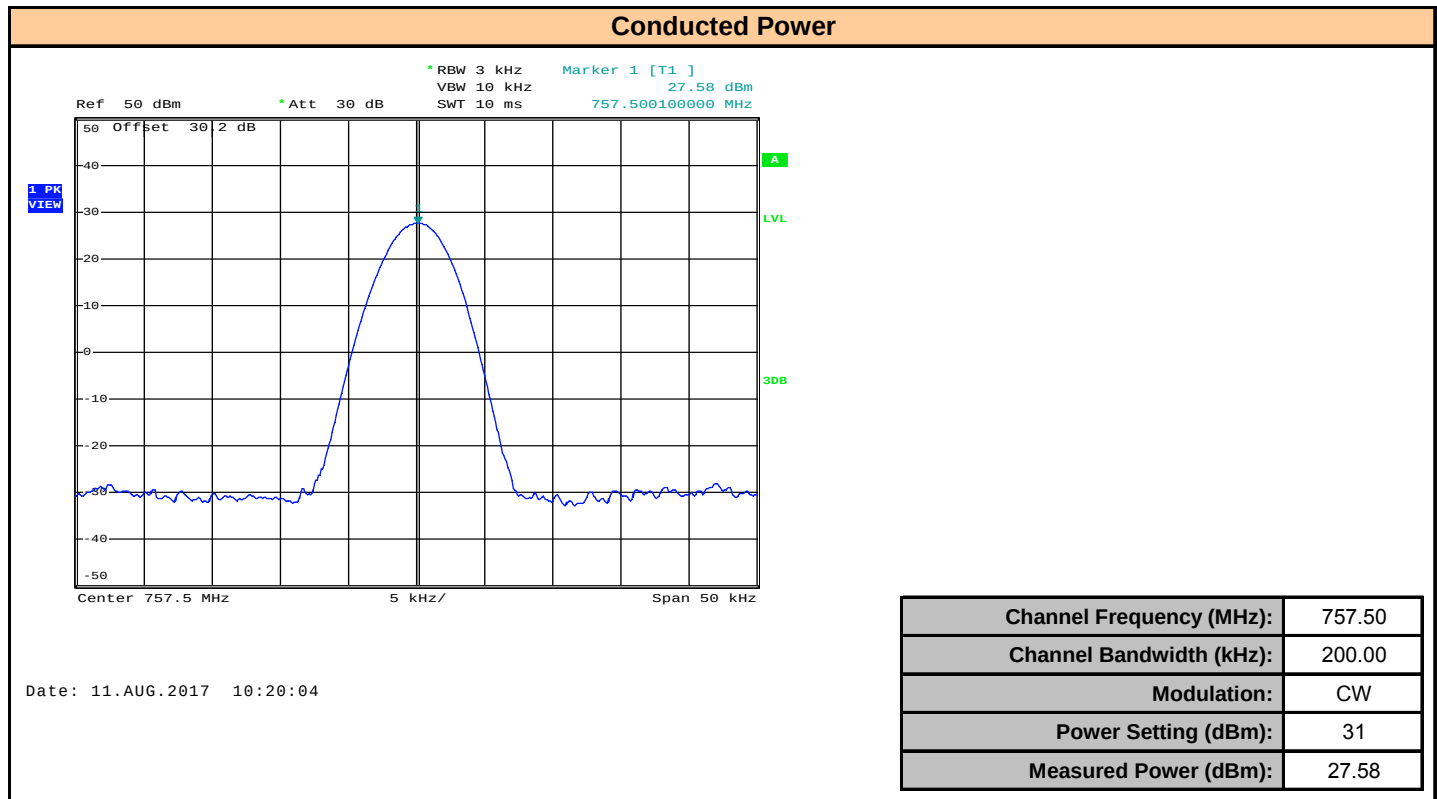
Plot 7.11 – Conducted Power 757.5MHz, 200kHz BW, CW
