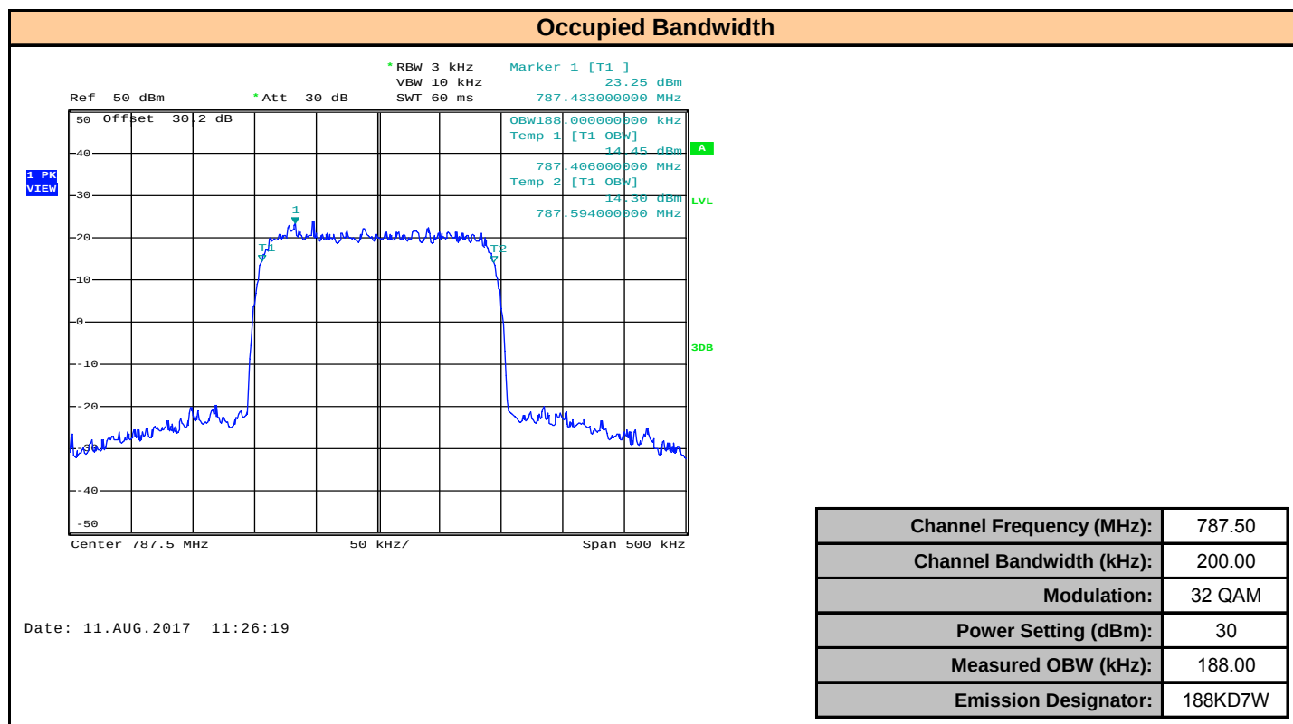
Plot 8.15 – Occupied Bandwidth 787.5MHz, 200kHz BW, 32 QAM
