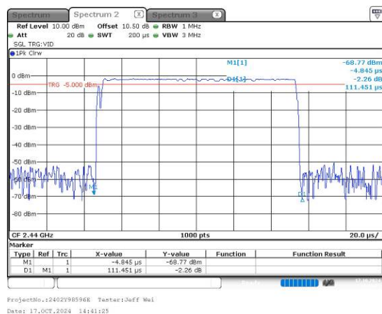
Pulse width
