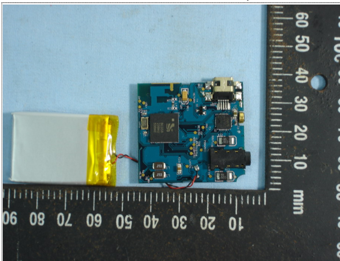
Rear View of Main board with battery
