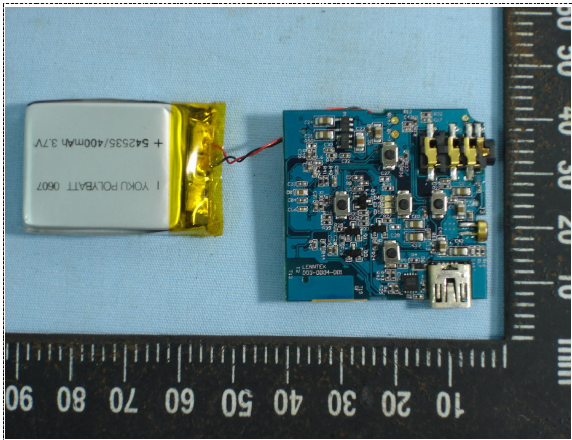
Front View of Main board with battery
