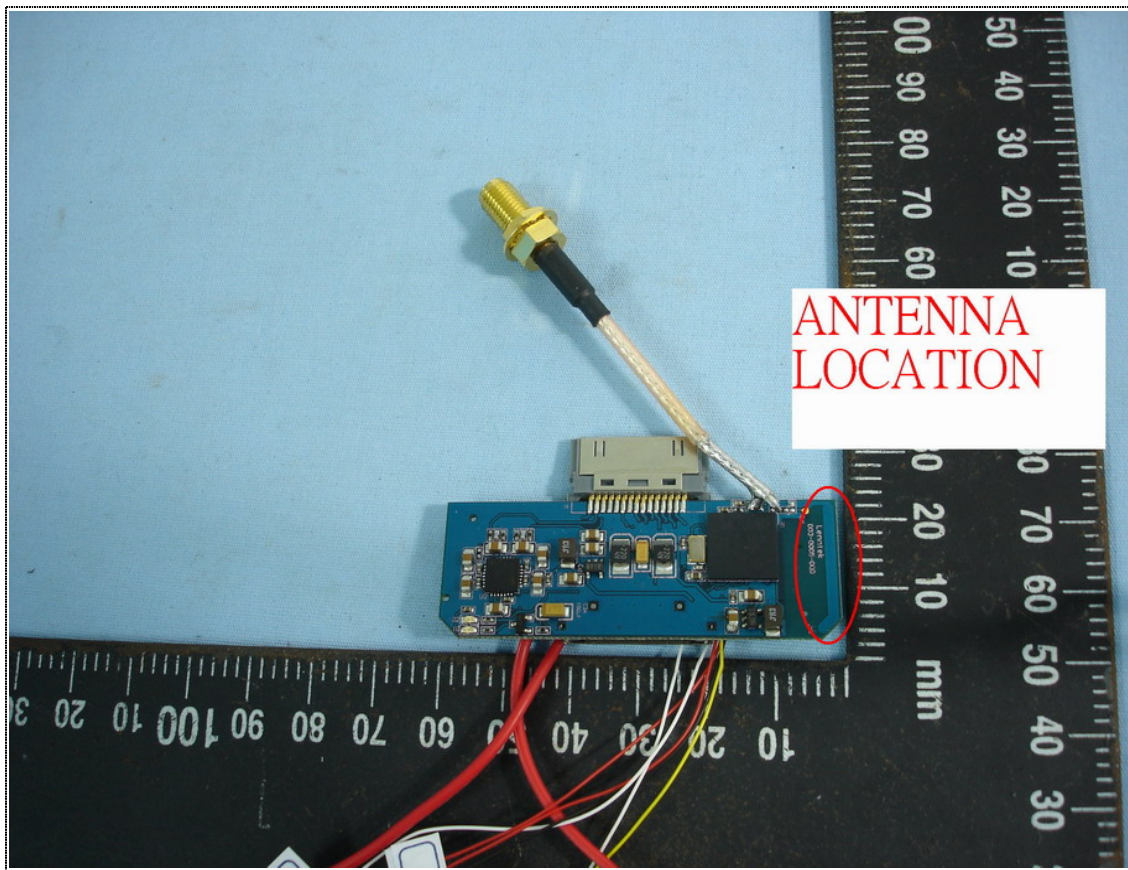
PCB Antenna Location
