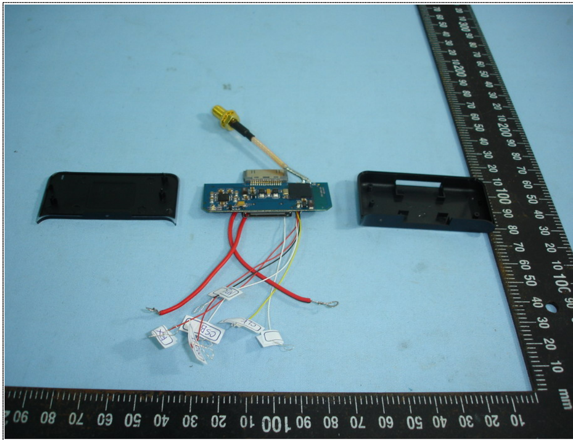
Inner view of Dongle
