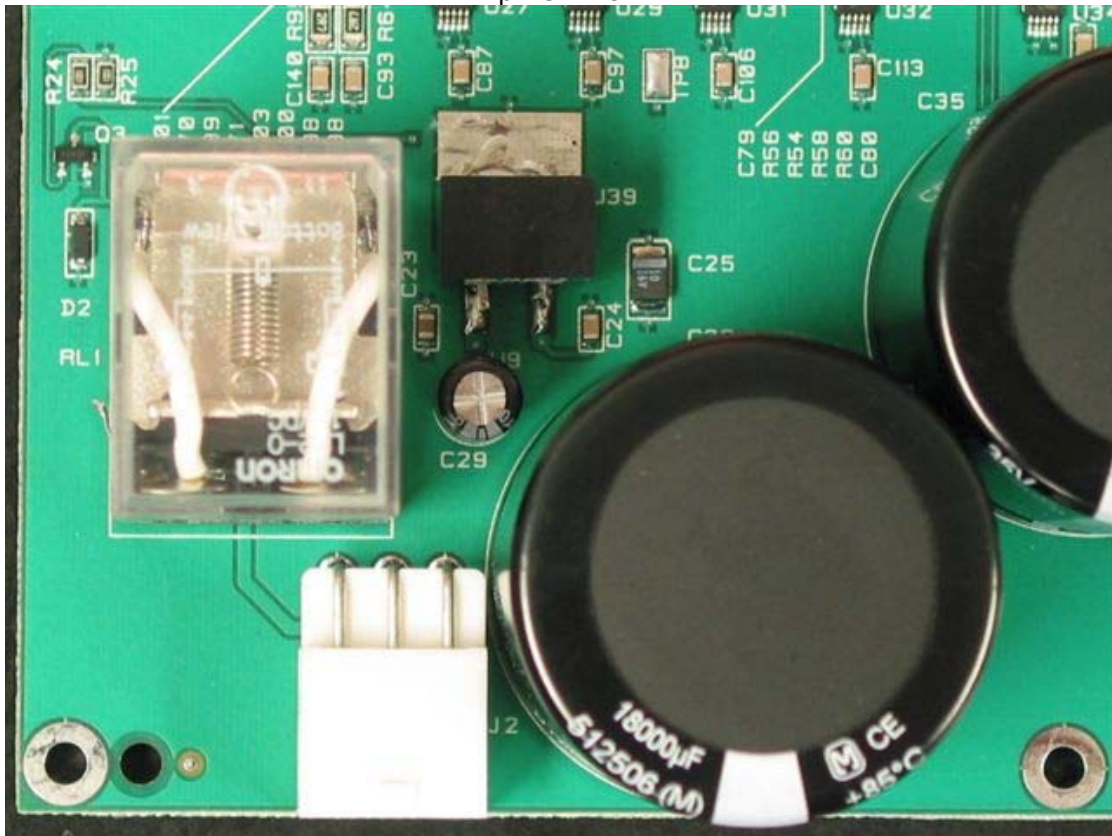
Amp PCB View 5
