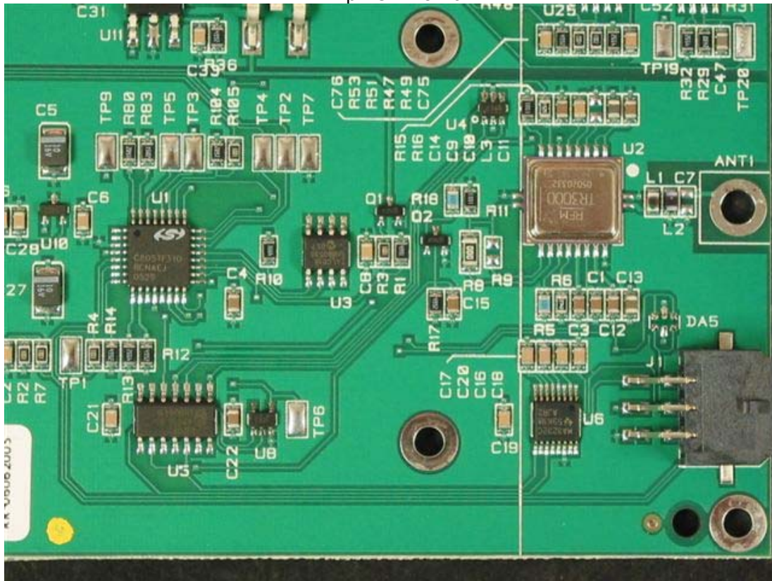
Amp PCB View 6
