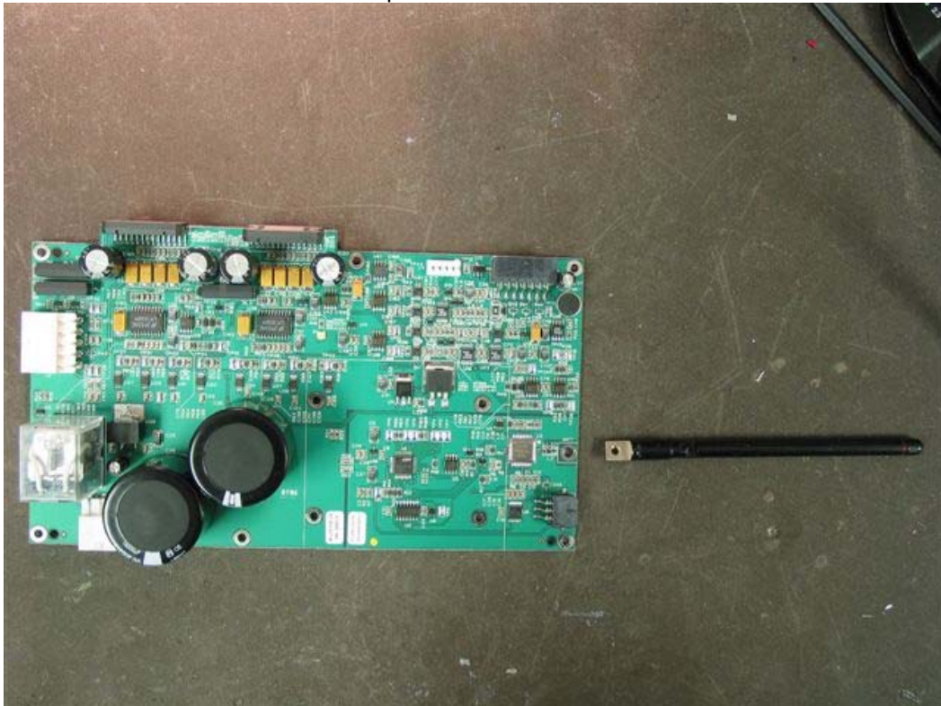
Amp PCB and Antenna
