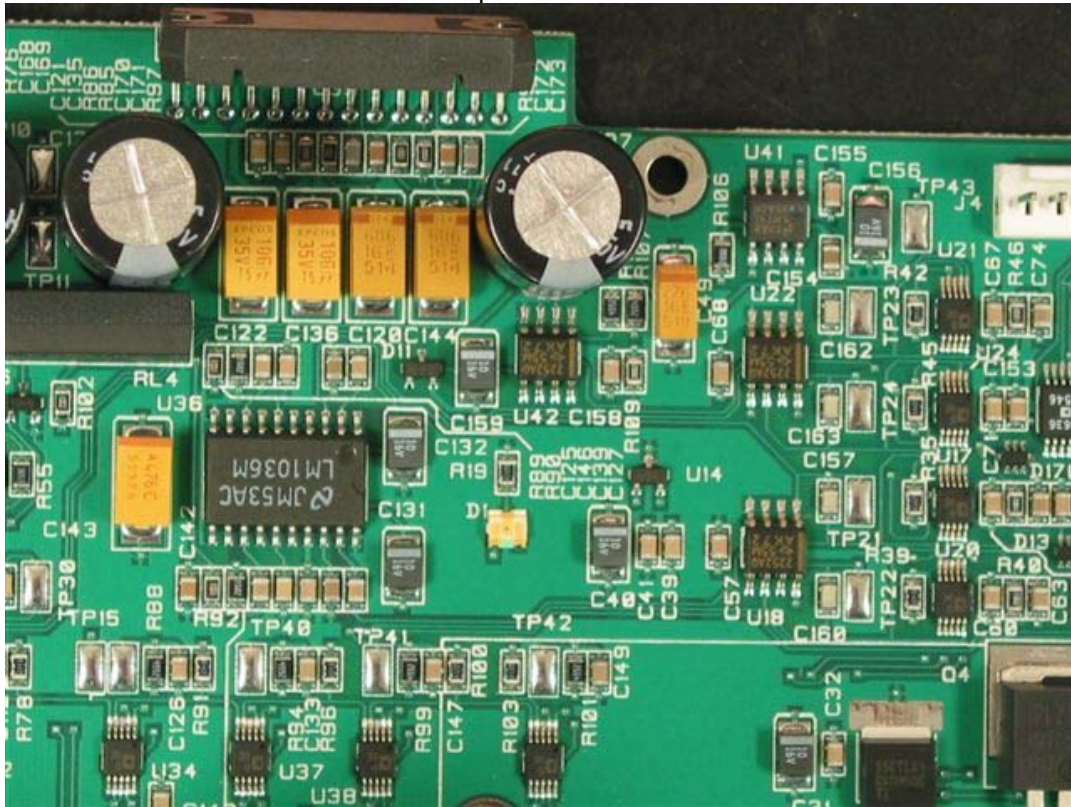
Amp PCB View 3
