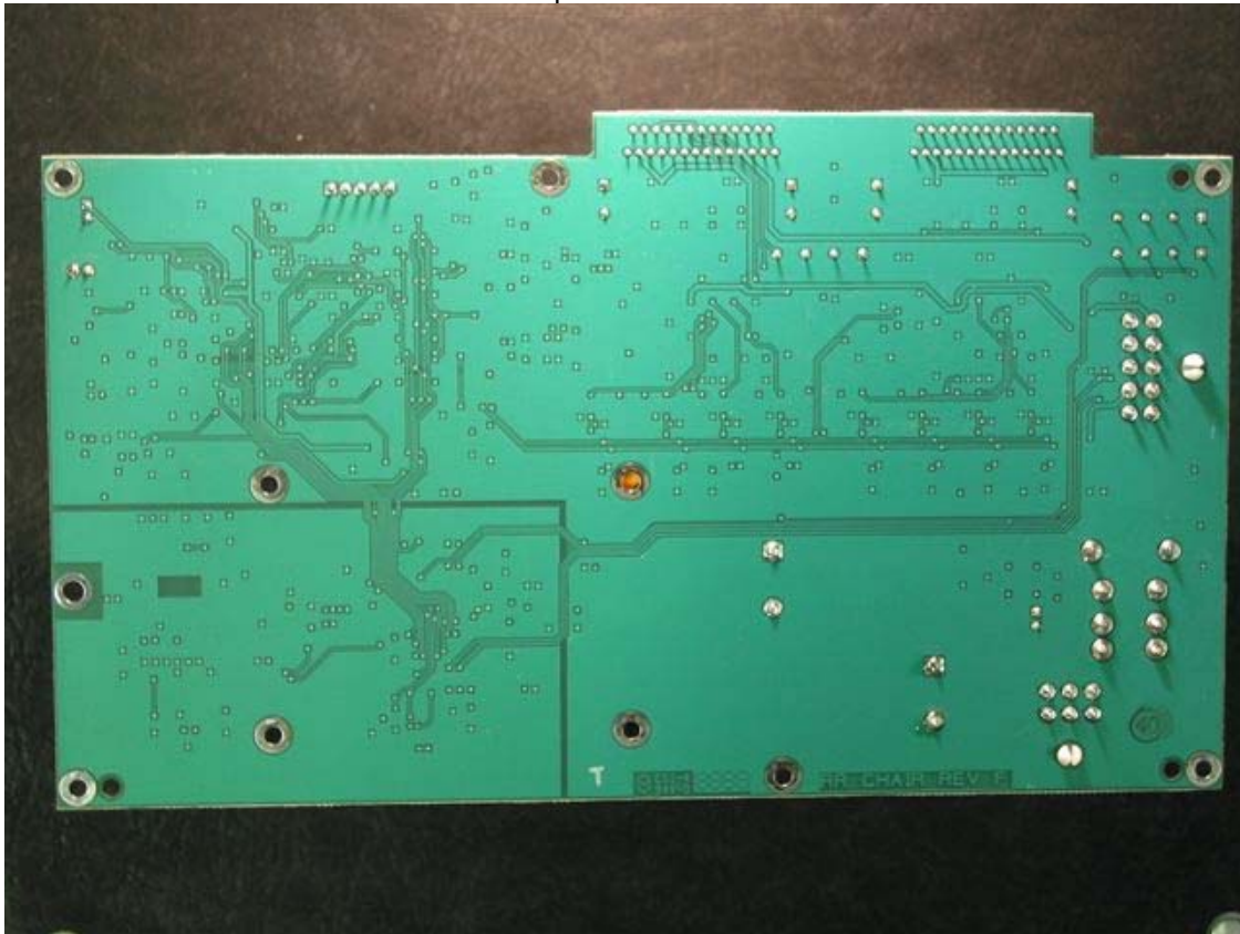
Amp PCB View 1
