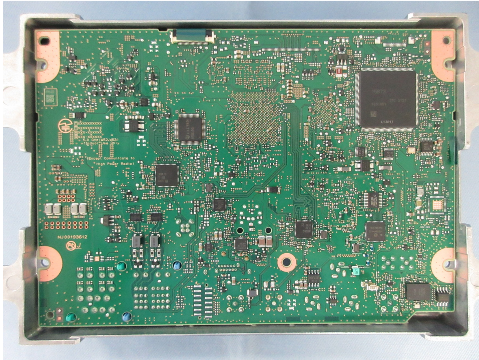
PCB-MAIN S-side
