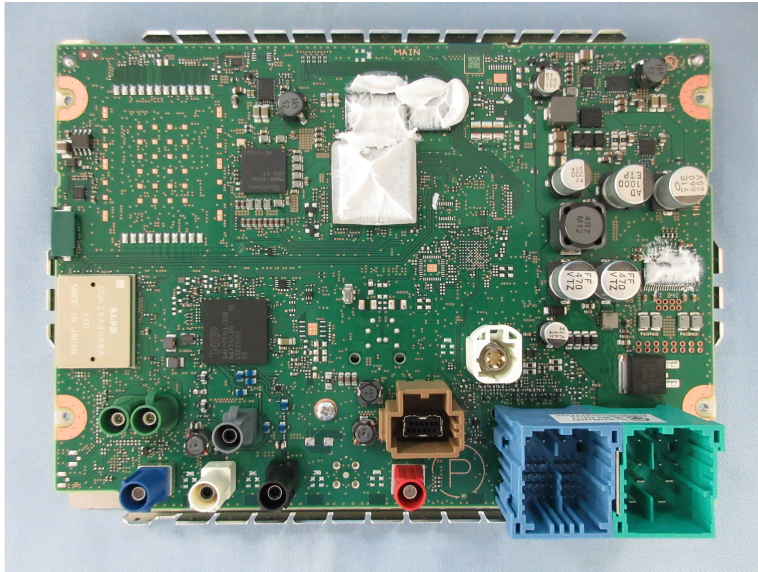
PCB-MAIN C-side
