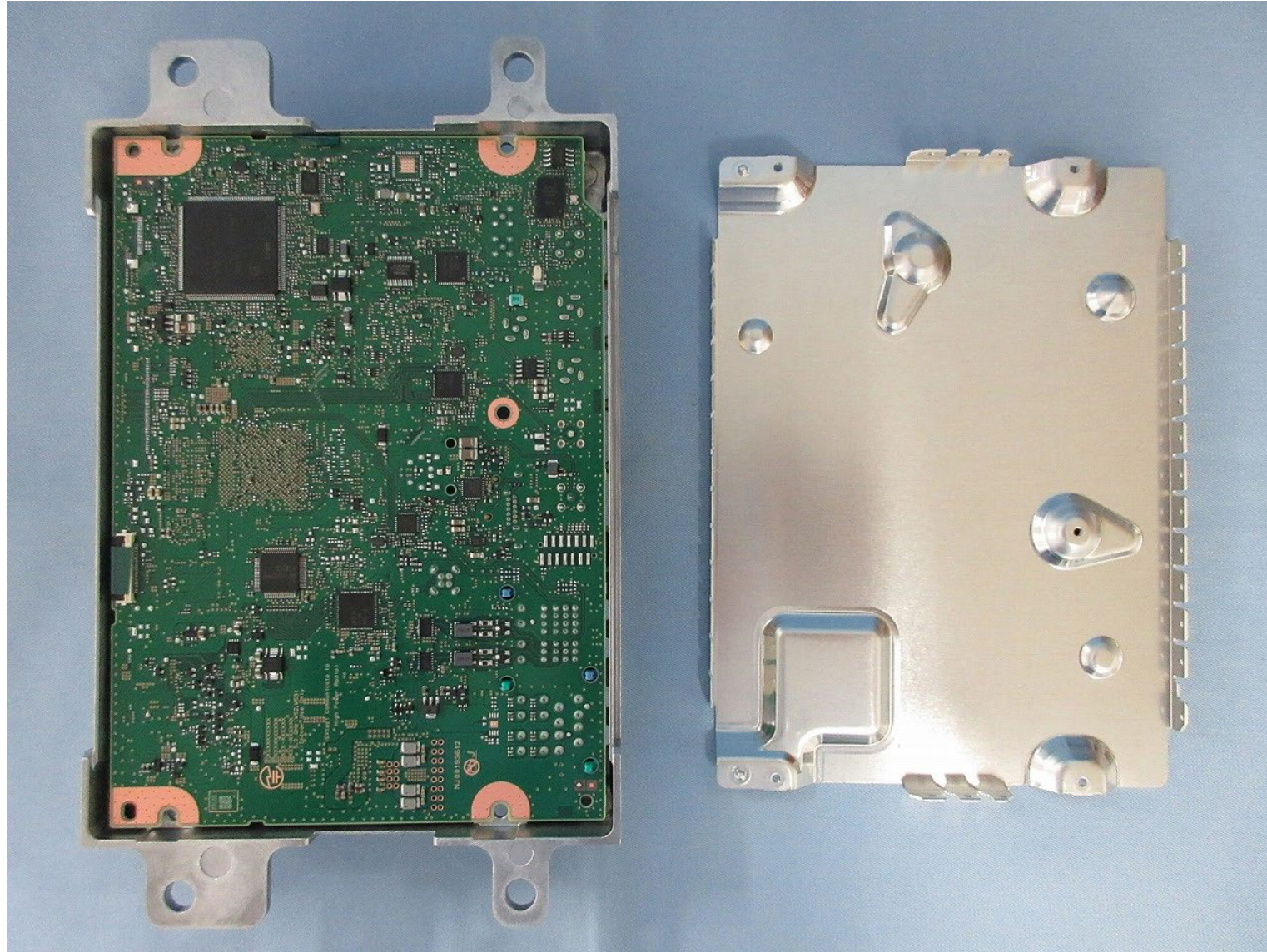
PCB-MAIN S-side
